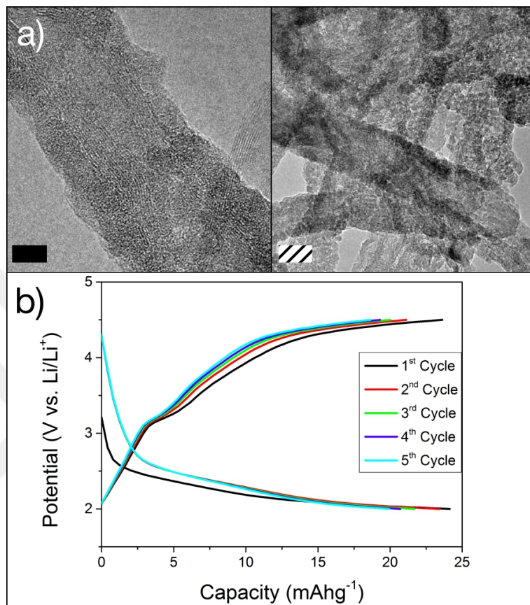
Figure 3.11: a) TEM images of A-100T cathode. Black and dashed bars indicate 5 and 10 nm in scale, respectively. b) Battery cycling performance of A-100T cathode at 100 mA g -1 current rate.
