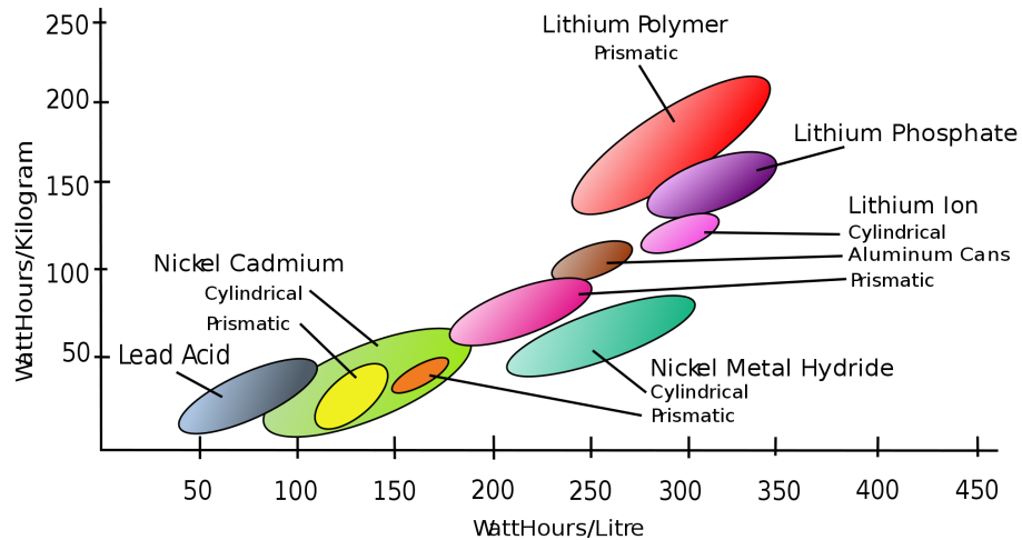
Figure 1.4: Graph of mass and volume energy densities of several secondary cells (by direction: down=heavier, up=lighter, right=powerful, left=weaker). [26]
