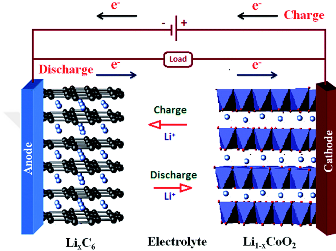
Figure 1.5: A schematic representation of the working mechanism of a simple LIB. [28]
