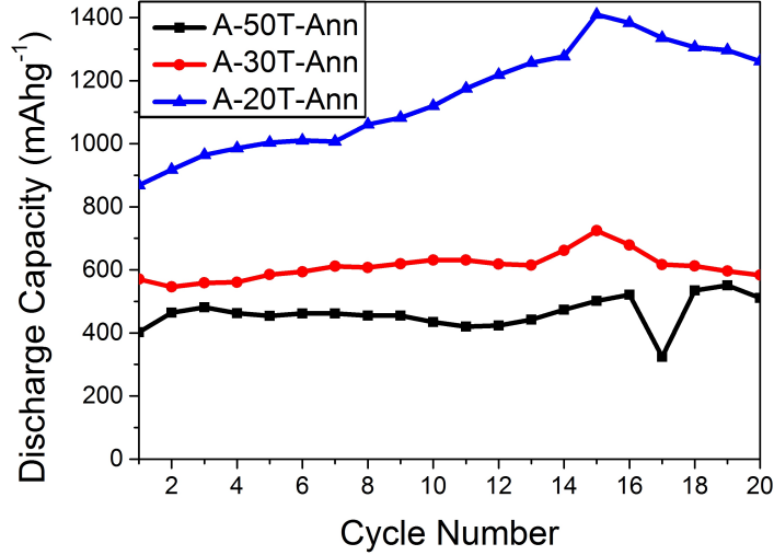
Figure 3.16: Discharge capacity retention comparison of A-50T-Ann, A-30T-Ann and A-20T-Ann cathodes on full 20 discharge and charge battery cycles at 100 \text{mA g}^{-1} current rate.
