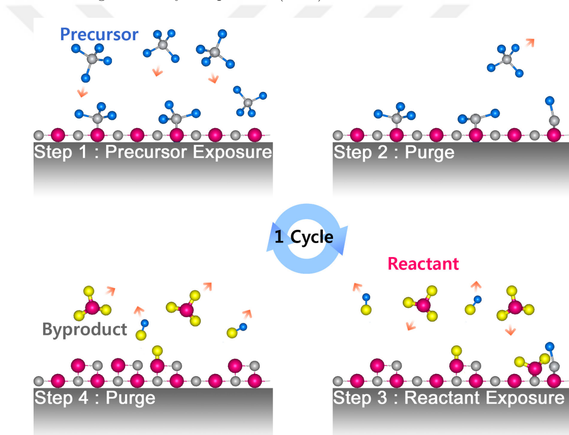
Figure 1.8: A schematic representation of one ALD cycle. [78]
