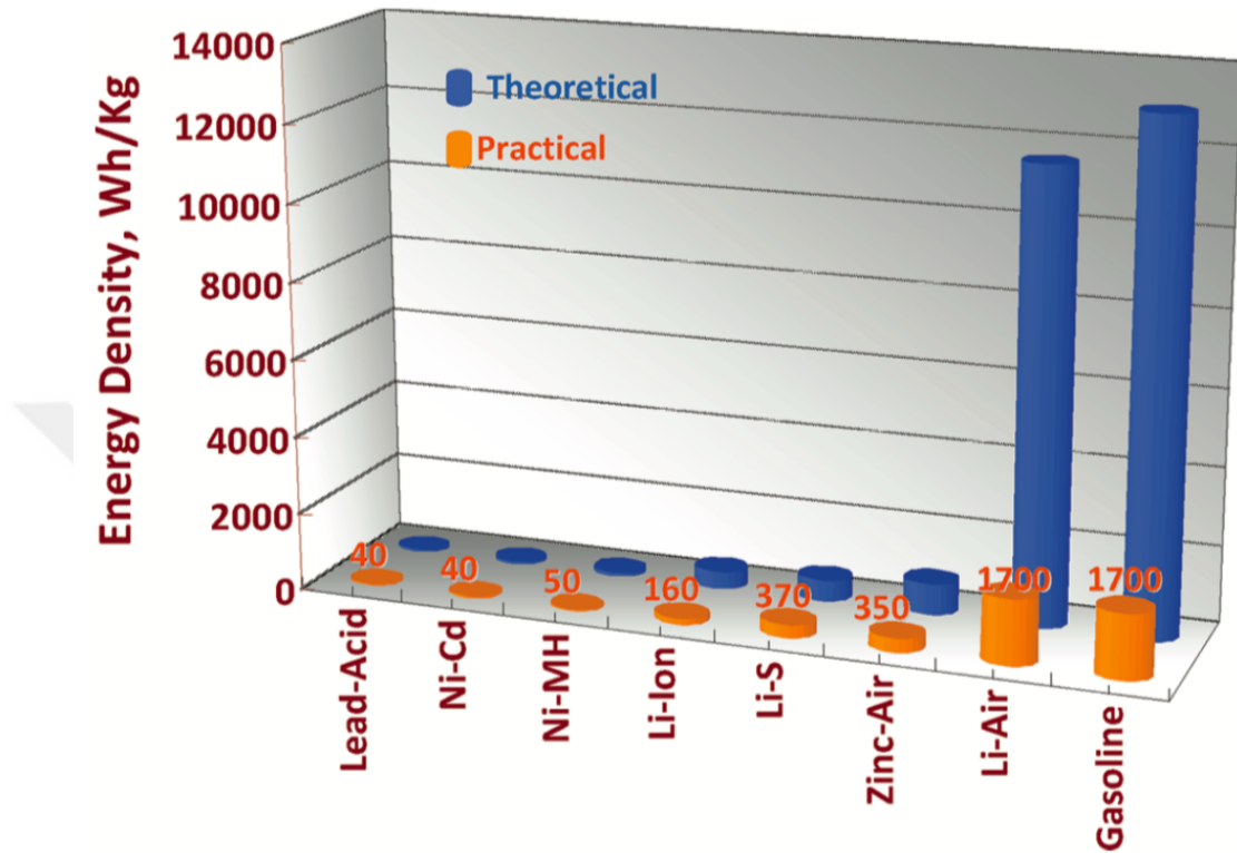
Figure 1.6: The gravimetric energy densities ( \text{Whkg}^{-1} ) for various types of rechargeable batteries compared to gasoline. The theoretical density is based strictly on thermodynamics and is shown as the blue bars while the practical achievable density is indicated by the orange bars and numerical values. For Li-air, the practical value is just an estimate. For gasoline, the practical value includes the average tank-to-wheel efficiency of cars. [36]
