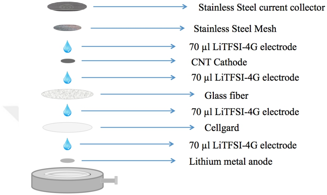
Figure 2.1: Schematic representation of Li-O 2 battery cell configuration.
