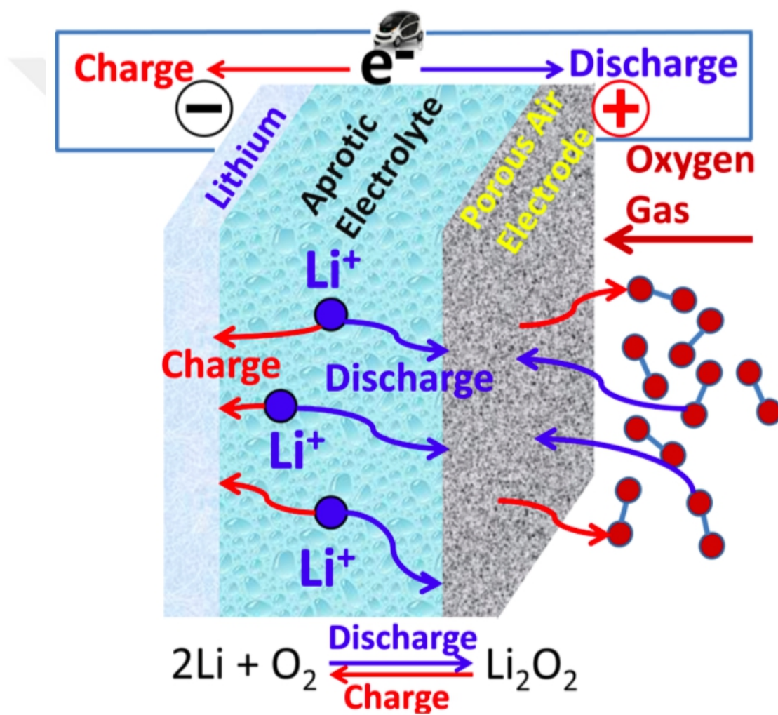
Figure 1.7: A schematic representation of an aprotic Li-O 2 battery. [40]
