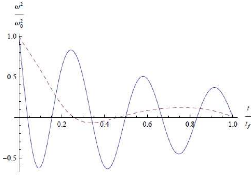
Fig. 4.2. \omega^2(t)/\omega_0^2 versus t/t_f . The system is decompressed by a factor of 4. The dashed (solid) curve is for L_1(t) ( L_2(t) with n = 3 ).
