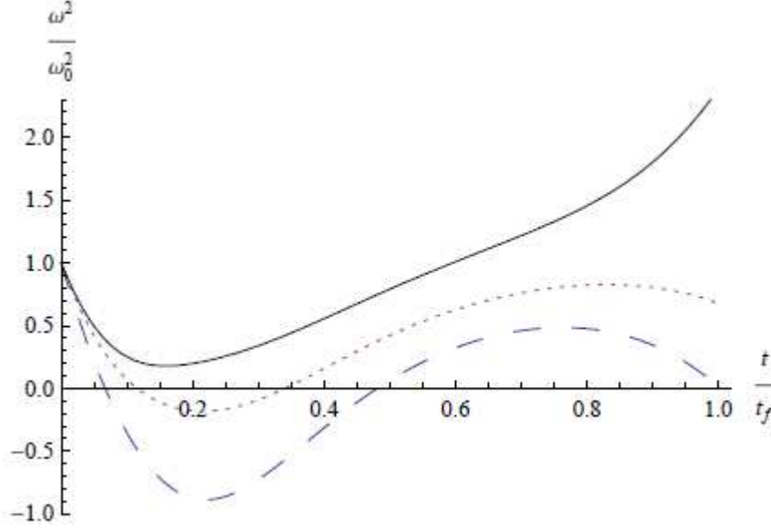
Fig. 4.1. \omega^2(t)/\omega_0^2 versus t/t_f for L_1(t) with \kappa = 4 in the TF regime. The solid, dotted and dashed curves are for \gamma = 0.4\omega_0 , \gamma = 0.3\omega_0 , \gamma = 0 , respectively.
