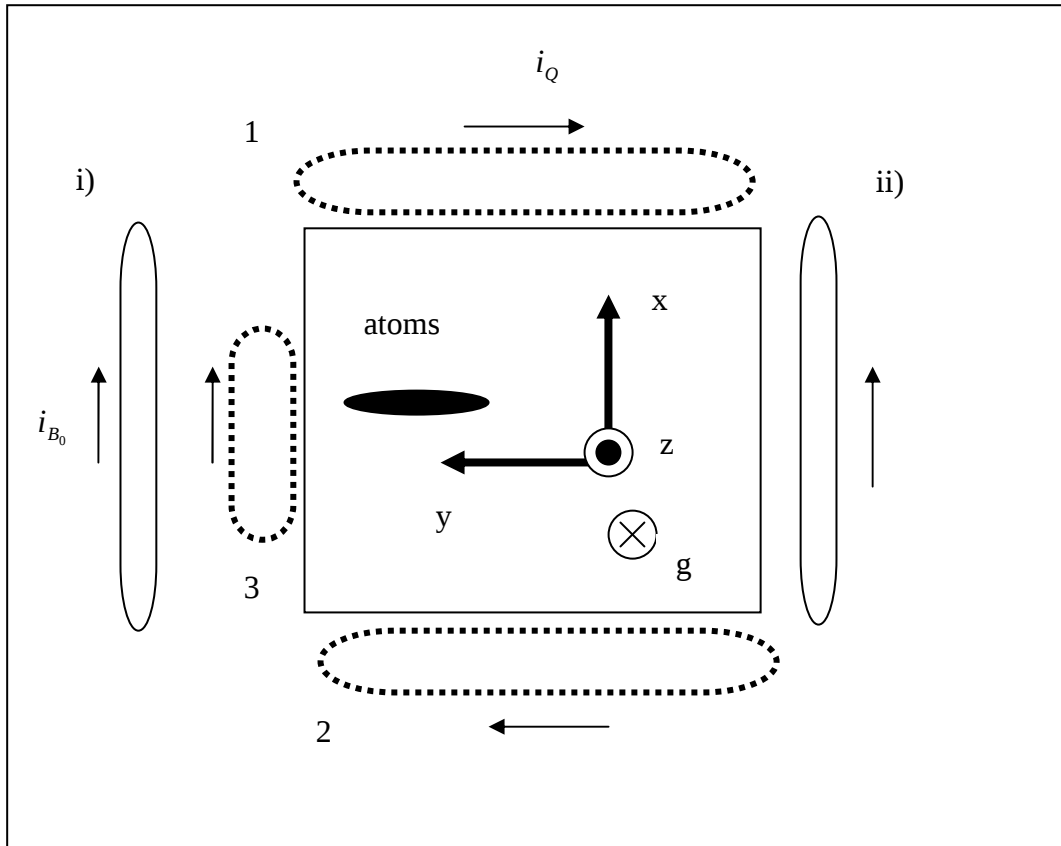
Fig. 3.2. Trapping geometry (figure in the horizontal plane). Ultracold ^{87}\text{Rb} atoms are trapped in an Ioffe-Pritchard-type magnetic trap created by current i_Q running through the three QUIC coils 1 , 2 , and 3 . An additional pair of coils ( i and ii ) produces a homogeneous field along y , which allows an independent tuning of the trap minimum field B_0 via the current i_{B_0} .
