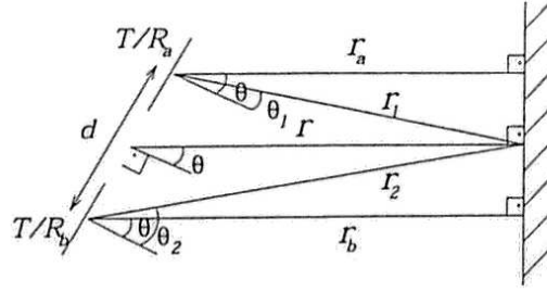
Figure A.1: Geometry of the problem with the given sensor pair when the target is a plane (adopted from [1]).
