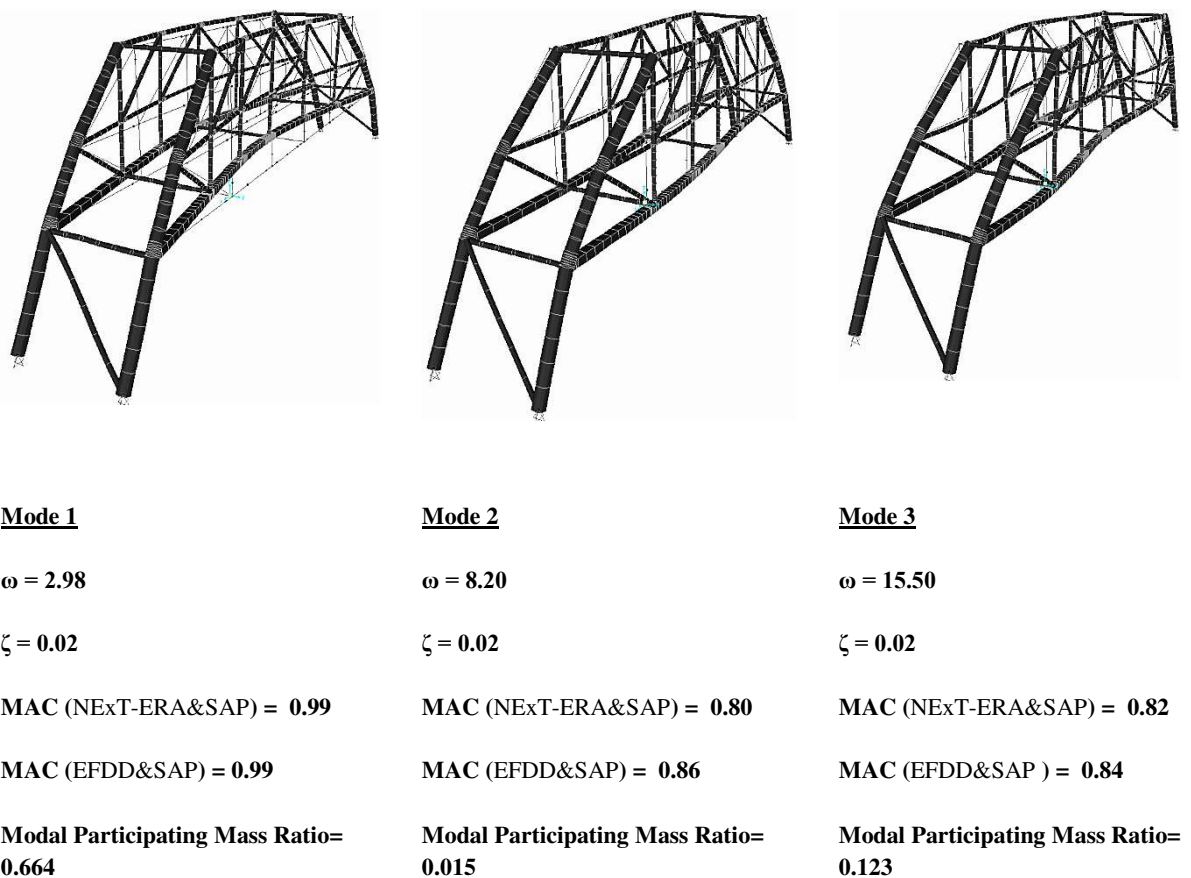
Figure 5.2 The first three modes obtained from the calibrated finite element model
