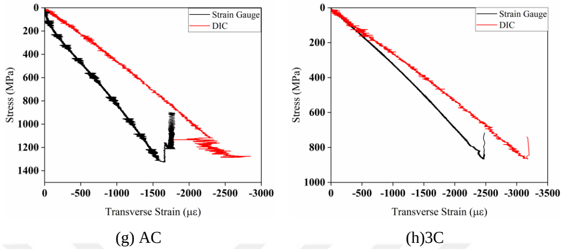
Fig. 3-14. Poisson's ratio evolution vs axial strain for (a) AC, (b) 13C, (c) 1C, (d)2C, (e) 3C and (f) AG, laminates; Transverse strain reduction during tests for (g) AC and (h) 3C specimens.
