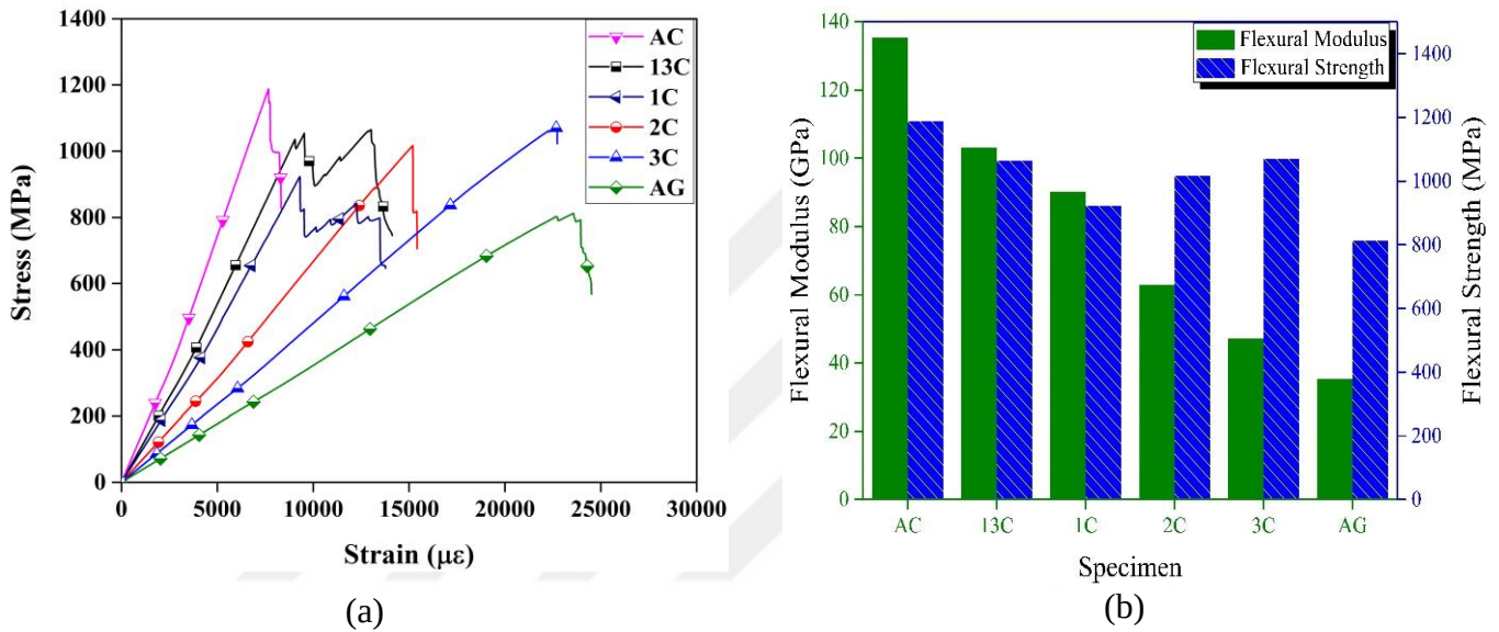
Fig. 1-6. (a) Flexural strain-stress curves (b) Flexural properties chart
