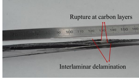
Fig. 1-11. Failure region of 2C specimen indicating fiber rupture in carbon plies and delamination of glass layers
