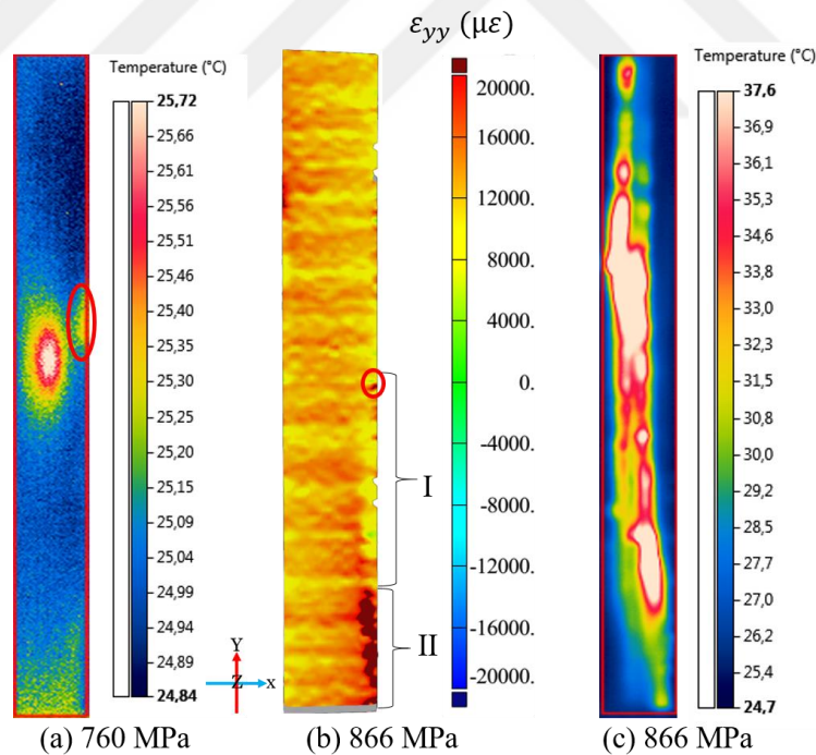
Fig. 3-9. (a) Thermal map corresponding to 760 MPa; (b) Axial strain map at 866MPa, and (c) thermal maps at 866MPa, for 3C laminate
