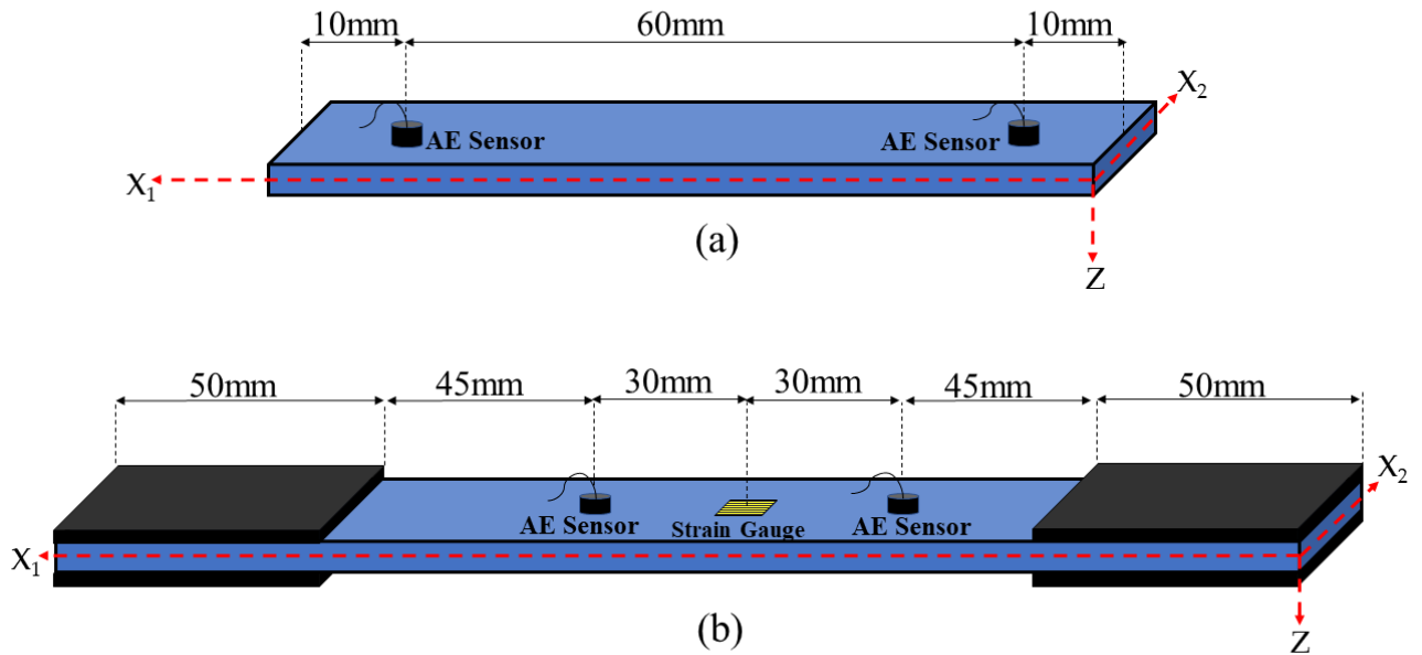
Fig. 1-2. Schematic of (a) Bending and (b) Tensile specimens
