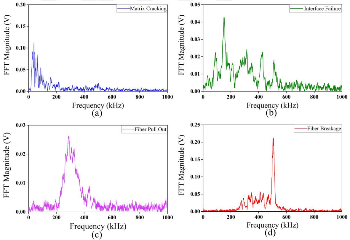
Fig. 1-21. Sample frequency domain magnitudes for each damage type (a) Matrix cracking, (b) Interface failure, (c) Fiber pull out, and (d) Fiber breakage
