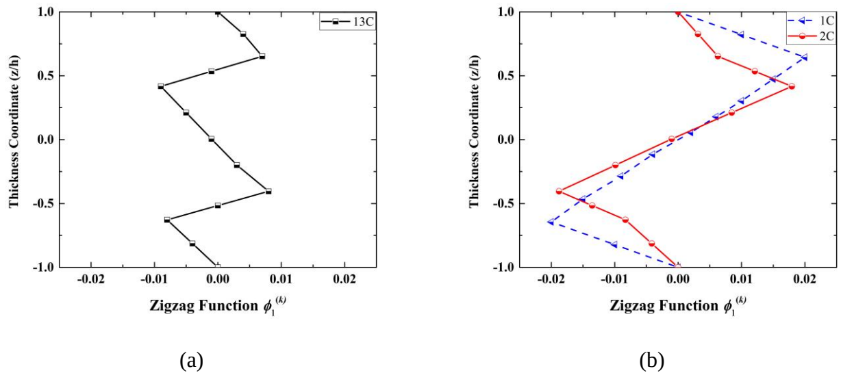
Fig. 1-12. Zigzag function values through the thickness for hybrid fiber samples (a) 13C (b) 1C and 2C
