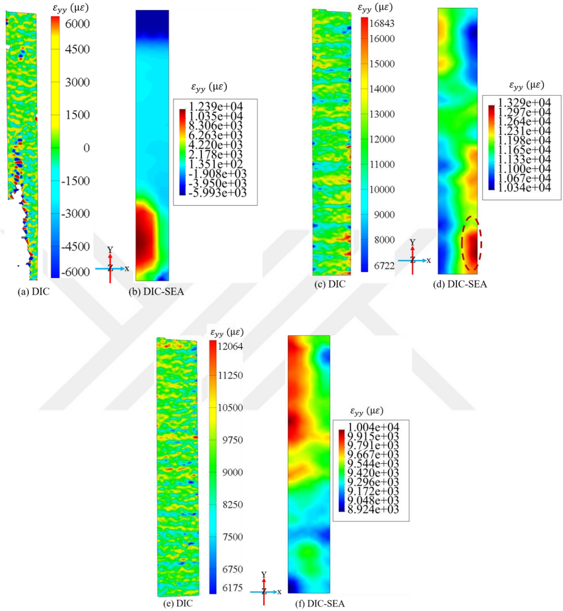
Fig. 3-13 Longitudinal strain maps obtained from DIC and DIC-SEA for a & b)AG; c & d)3C; e & f)13C laminates
