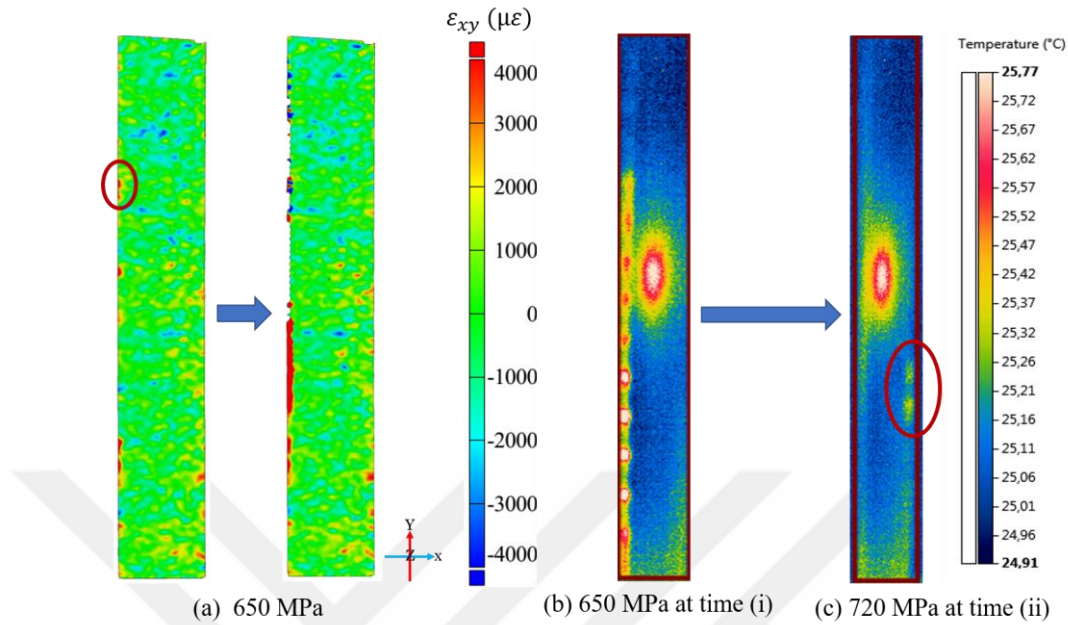
Fig. 3-7. (a) Axial strain maps for 1C sample at 650 MPa; Thermal maps corresponding to (b) 650, and (c) 720 MPa
