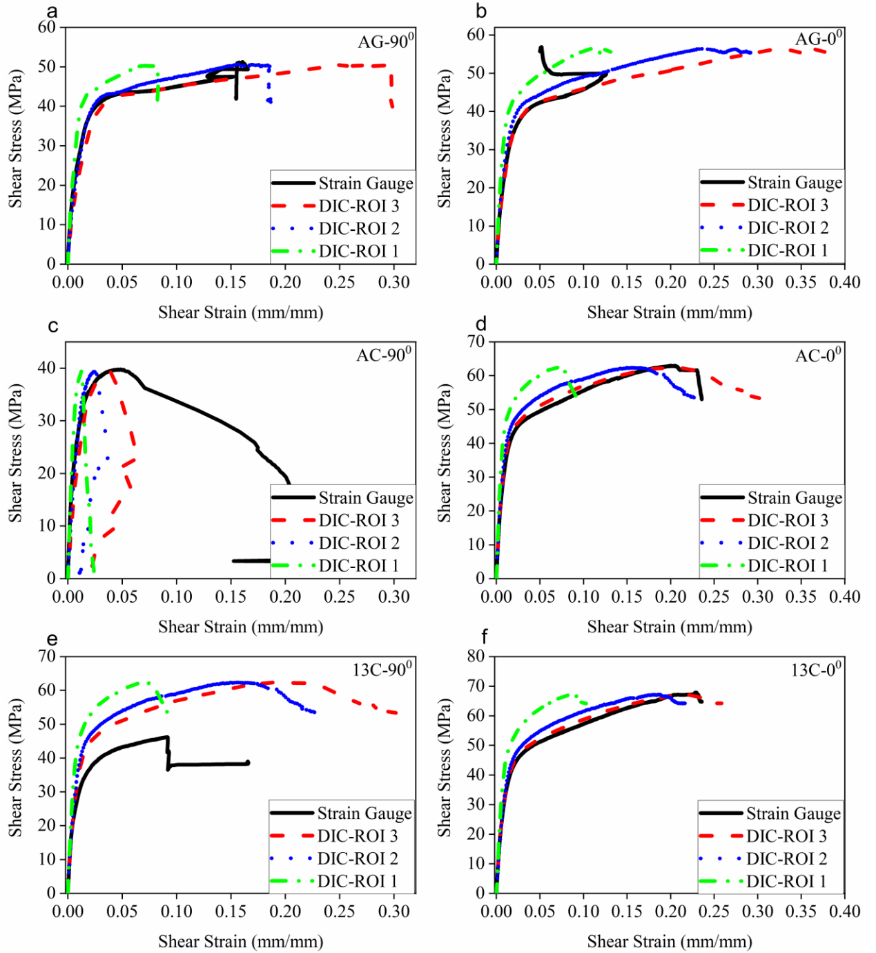
Fig. 2-4. Shear stress-strain curves obtained for various ROIs and strain gauge for (a)AG-90°, (b)AG-0°, (c)AC-90°, (d)AC-0°, (e)13C-90°, and (f)13C-0°
