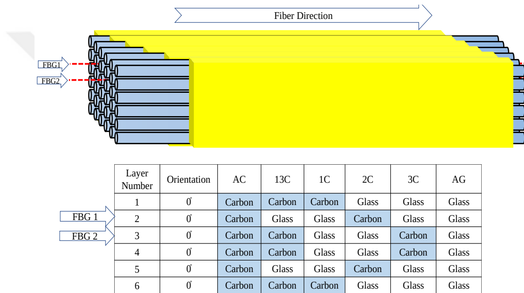
Fig. 3-1. Schematic of FBG positions and stacking sequence of various composites
