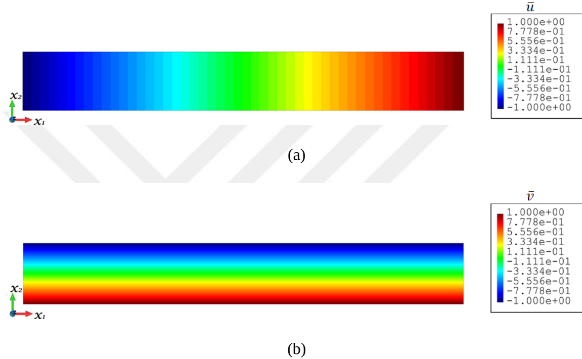
Fig. 1-13. Displacement results for tensile tests: In-plane displacements along (a) x_1 axis and (b) x_2 axis
