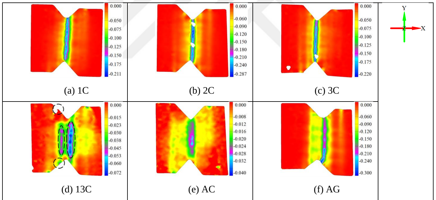
Fig. 2-6. DIC shear strain maps for 90° configurations for (a)1C, (b)2C, (c)3C, (d)13C, (e)AC, and (f)AG laminates
