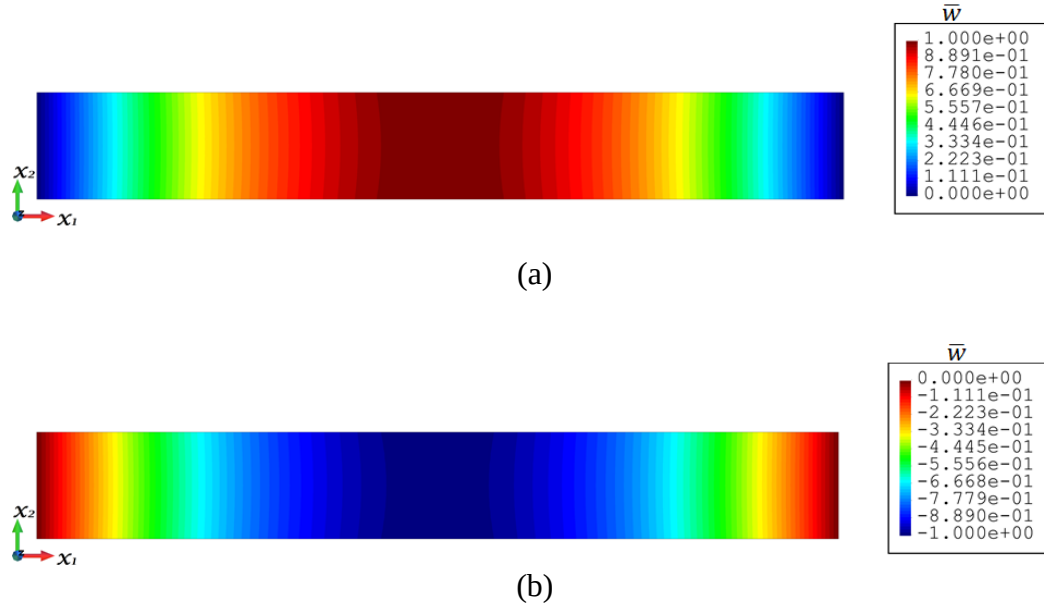
Fig. 1-14. Out of plane displacement for (a) 13C and 3C (b) 2C specimens
