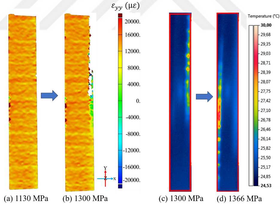
Fig. 3-6. Axial strain maps for 13C sample at (a) 1130, and (b) 1300 MPa; Thermal maps corresponding to (c) 1300, and (d) 1366 MPa
