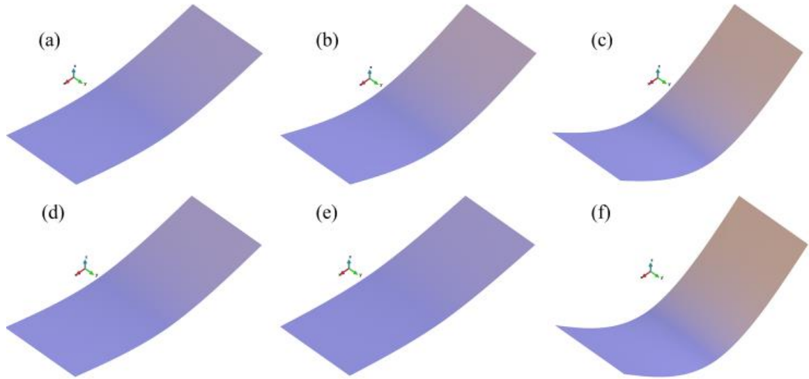
Fig. 1-18. Deformation results under flexural load [mf:10] (a) 1C, (b) 2C, (c) 3C, (d) 13C, (e) AC, (f) AG
