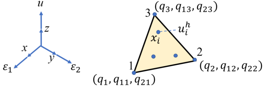
Fig. 3-3. A three-node triangular smoothing element depicted with its nodal DOF
