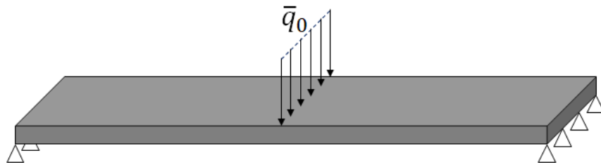
Fig. 1-5. Schematic of load distribution (a) Tensile Specimen (b) Bending specimen
