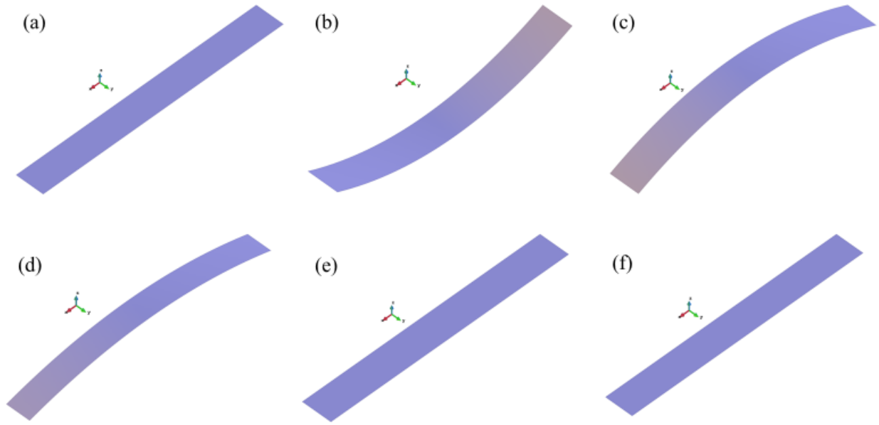
Fig. 1-15. Deformation results for tensile specimens (a) 1C [mf: 333], (b) 2C [mf:128], (c)3C [mf:204], (d)13C [mf:1030], (e) AC [mf:385], and (f) AG [mf:129]
