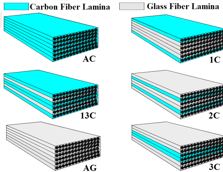
Fig. 1-1. Stacking sequence of produced composite plates and their nomenclature
