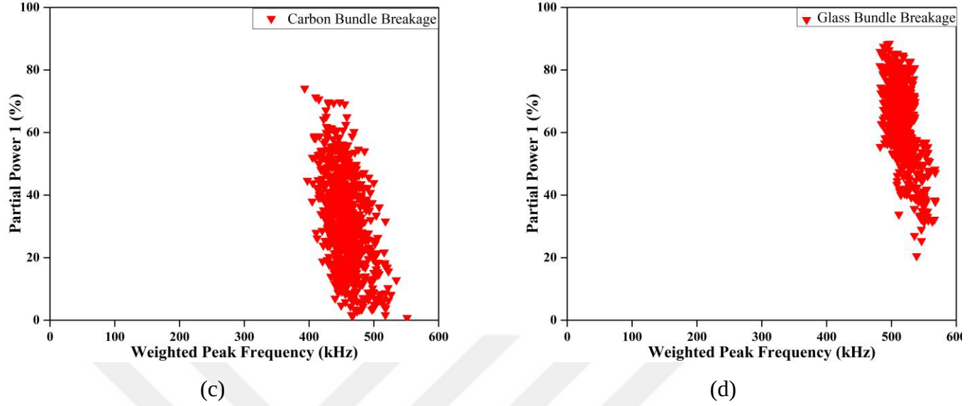
Fig. 1-20. (a) Clustering result of 2C bending hybrid sample, (b) clustering result of 2C tensile hybrid specimen, (c) AE results of carbon bundle, and (d) AE results of glass bundle
