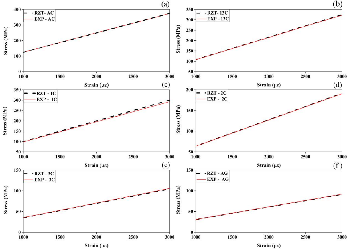
Fig. 1-19. Comparison of stress strain behavior of bending specimens between 1000-3000 \mu\epsilon . (a) AC, (b) 13C, (c) 1C, (d) 2C, (e) 3C, (f) AG
