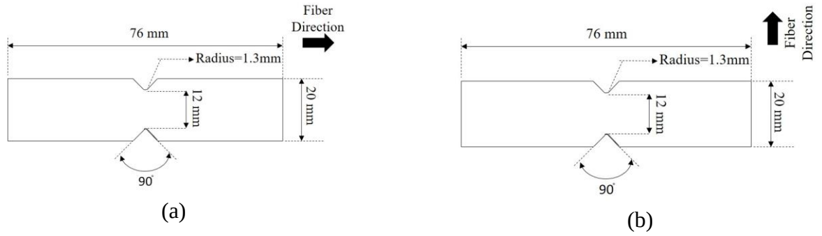
Fig. 2-1. Schematic of V-notch beam test samples in (a) 0° , (b) 90° configurations
