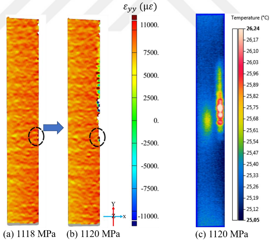
Fig. 3-5. Axial Strain field for AC specimen at (a) 1118 and (b)1120 MPa; (c) Thermal map prior to failure at 1120 MPa
