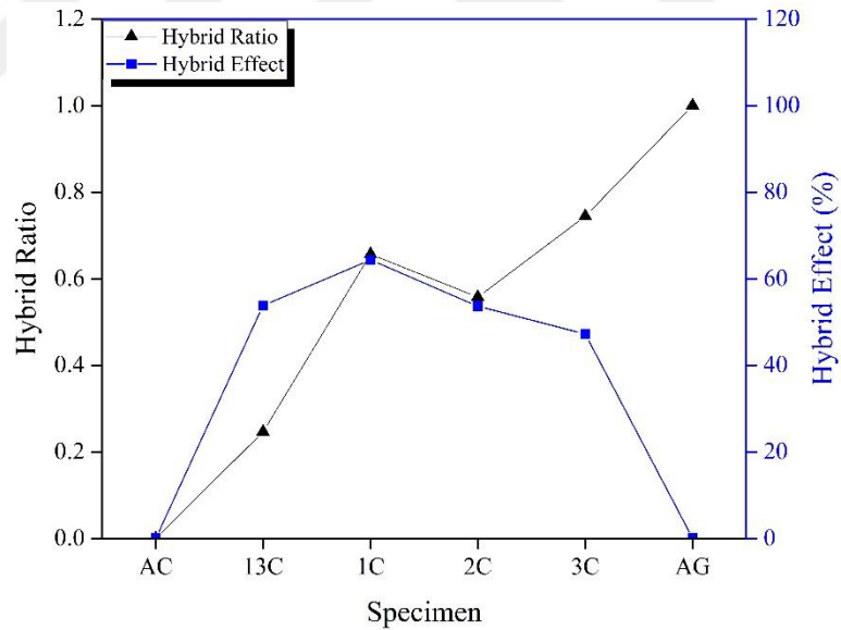
Fig. 1-10. Plot of Hybrid effect and hybrid ratio for each tensile specimen
