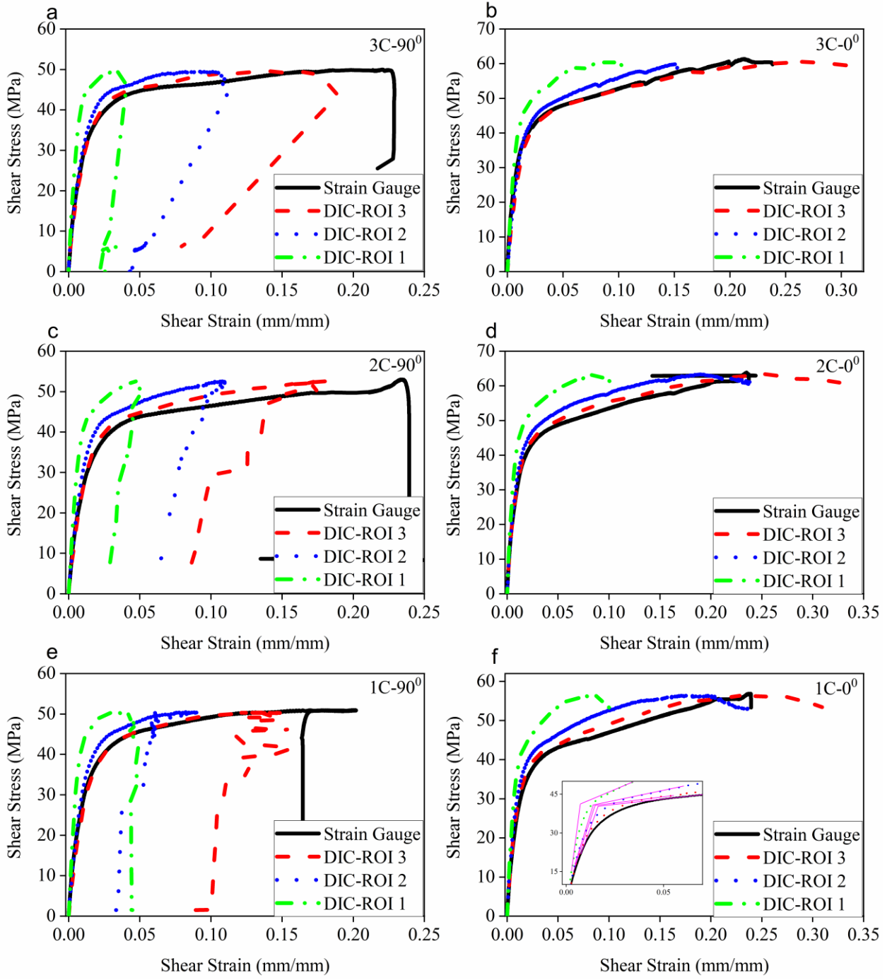
Fig. 2-3. Shear stress-strain curves obtained for various ROIs and strain gauge for (a)3C-90°, (b)3C-0°, (c)2C-90°, (d)2C-0°, (e)1C-90°, and (f)1C-0°
