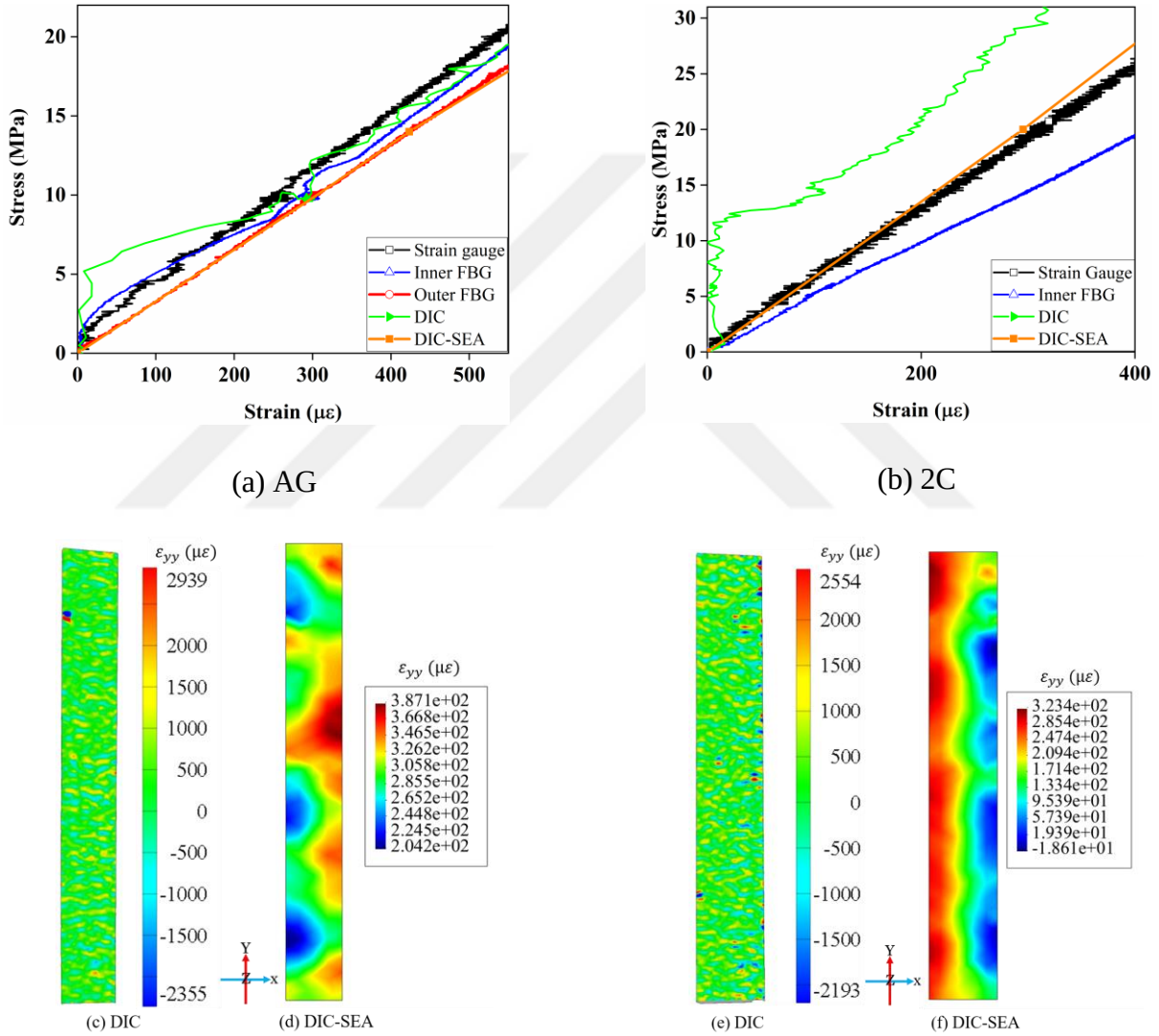
Fig. 3-12. Presence of data fluctuation at early stages of loading for (a) AG and (b) 2C samples; Full field longitudinal strain maps for AG sample obtained by (c) DIC and (d) DIC-SEA; Full field longitudinal strain maps for 2C sample obtained by (e) DIC and (f) DIC-SEA.
