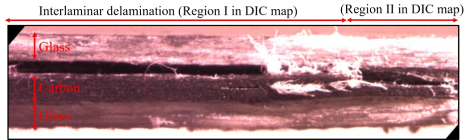
Fig. 3-10. Transfer of zone of interlaminar crack between carbon and glass plies in to the middle carbon layers as seen in 3C laminate
