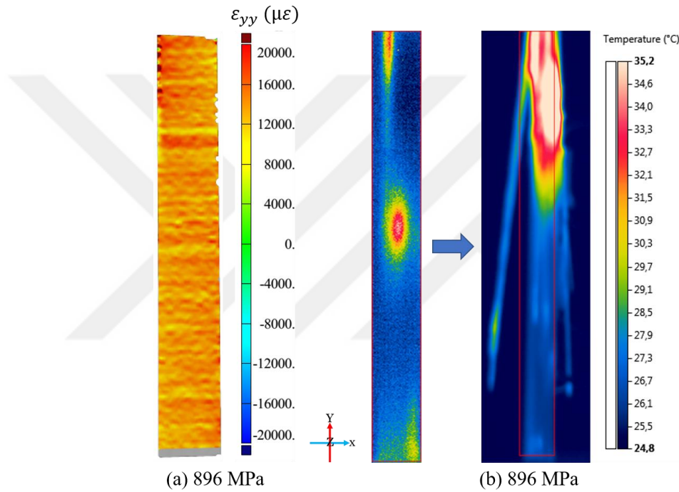
Fig. 3-8. (a) Axial strain map for 2C sample at 896 MPa; (b) Thermal maps at failure point corresponding to 896 MPa
