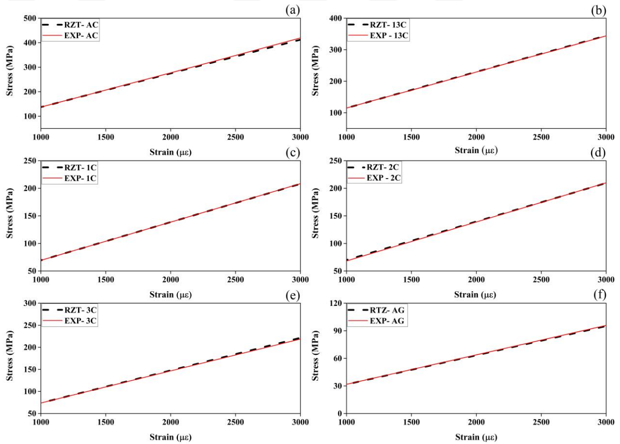
Fig. 1-16. Comparison of stress strain behavior tensile specimens between 1000\mu\epsilon and 3000\mu\epsilon . (a) AC (b) 13C (c) 1C (d) 2C (e) 3C (f) AG
