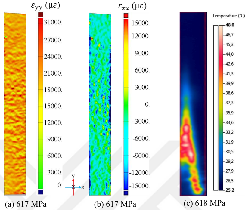
Fig. 3-11. (a) Axial strain map at 617 MPa, (b) Transverse strain map at 617 MPa, and (c) Thermal map at 618 MPa, for AG specimen
