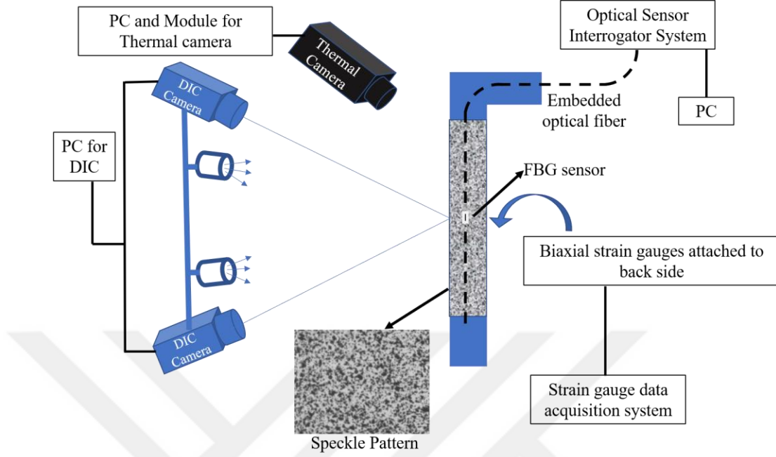
Fig. 3-2. Schematic of test set up for multi-instrument monitoring using DIC, Thermal Camera, Strain Gauge and embedded FBGs
