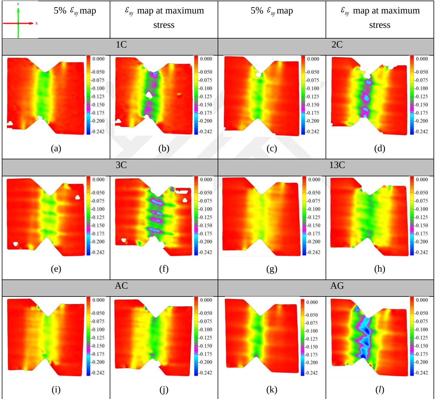
Fig. 2-5. strain maps for various laminates in 0^\circ direction at 5% \epsilon_{xy} strain and maximum load level
