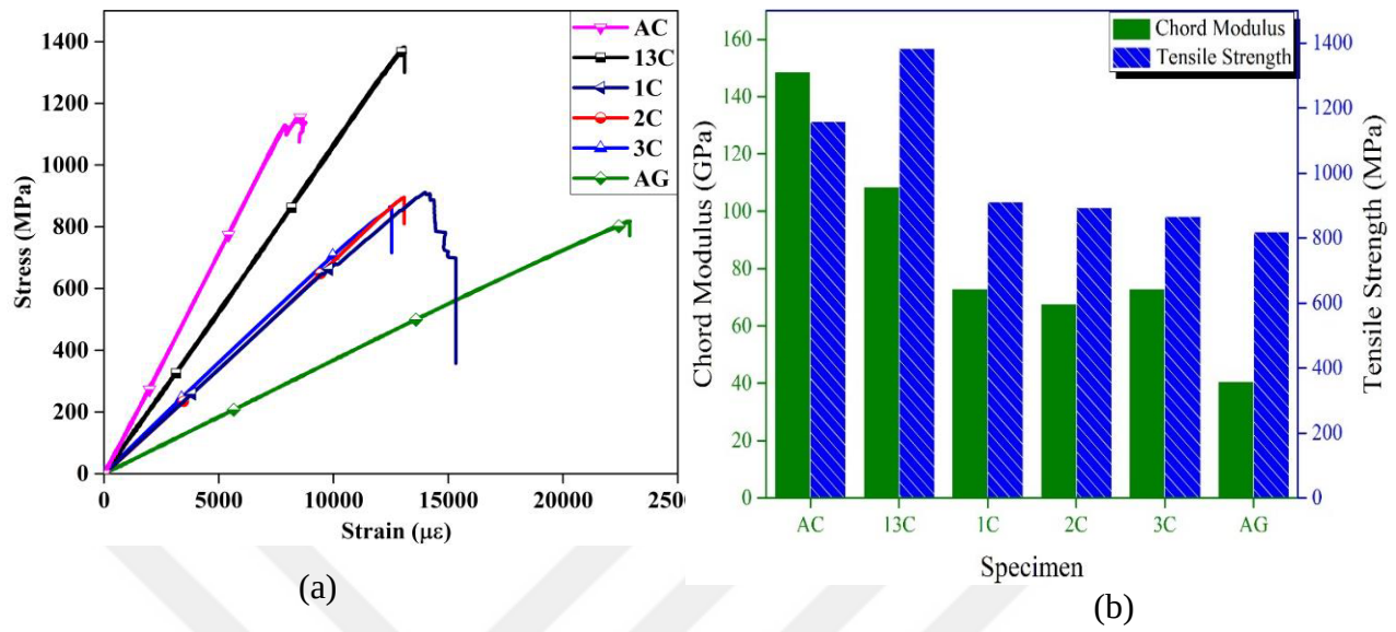
Fig. 1-9. (a) Tensile stress- strain curve of each laminates (b) strength and modulus of respective laminates
