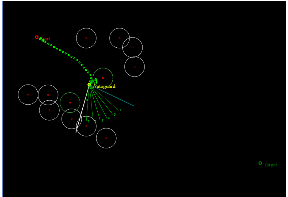
Figure 4.7: USV with autopilot case
