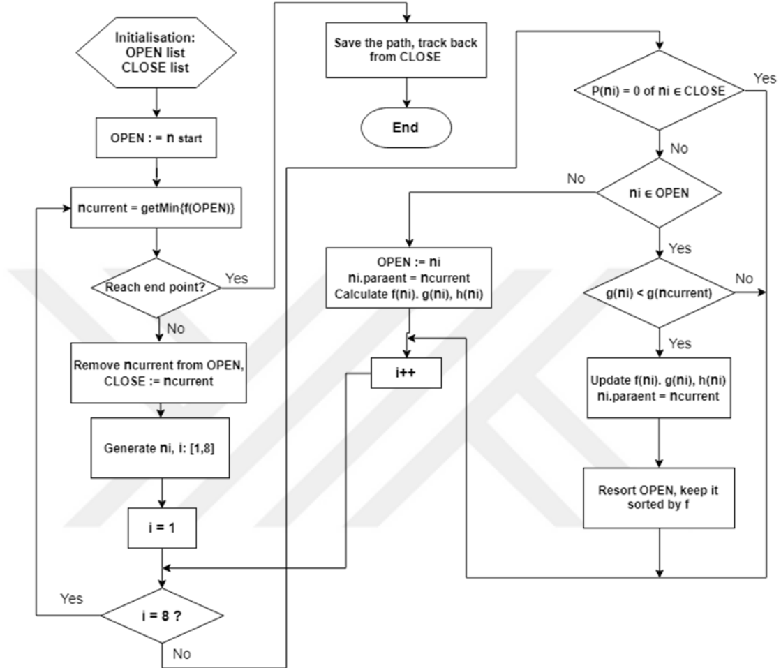
Figure 3.3: Flowchart of the conventional A* algorithm
