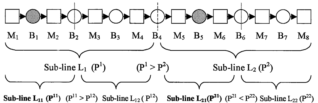
Figure 5. 5. Bisection of 8-machine production line until its final sub-lines
