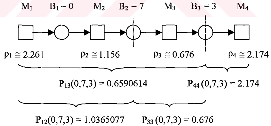
Figure 5. 10. Termination of LIBA
