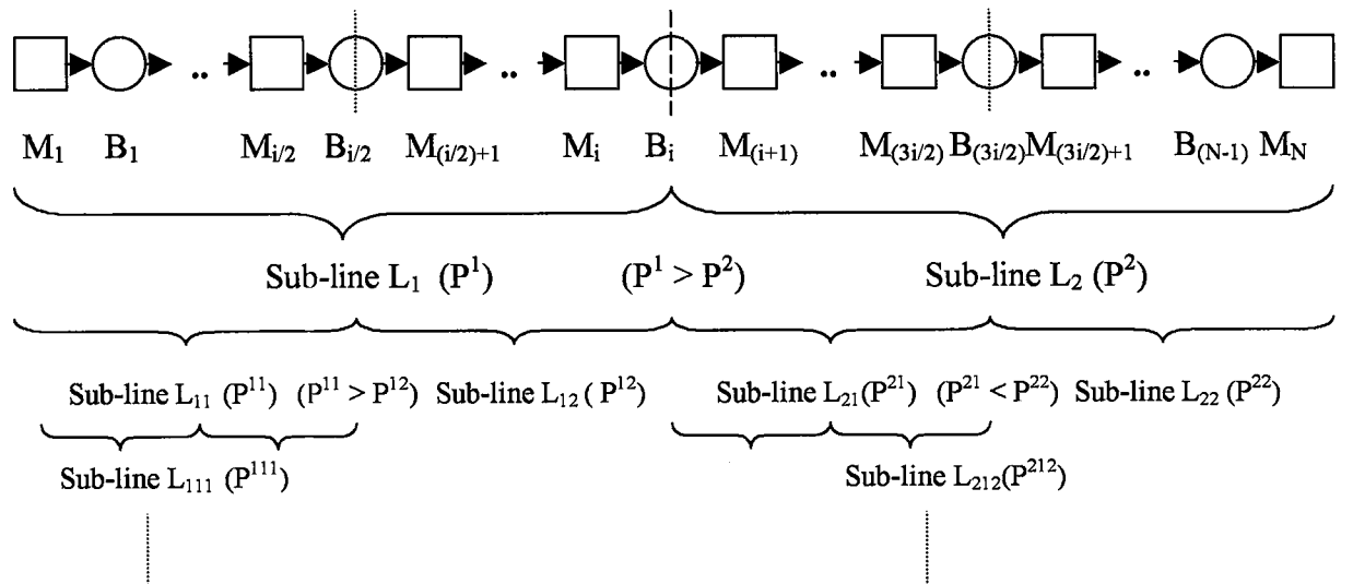
Figure 5. 4. Bisection procedure for determination of potential giver and receiver
