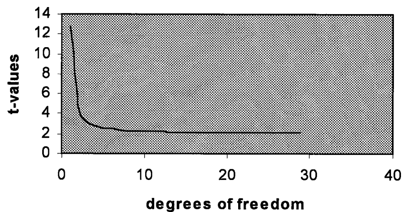
Chart5. 1. t -statistics versus the degrees of freedom for \alpha = 0.05 confidence level
