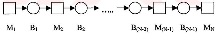
Figure 5. 1. The N -machine production line L
