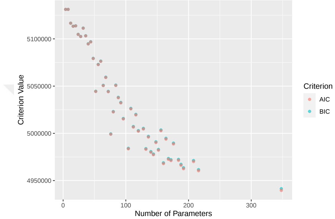
Figure 4.9: AIC and BIC criteria values using p -method, for different number of estimated parameters which depend on the cardinality of the attribute set R
