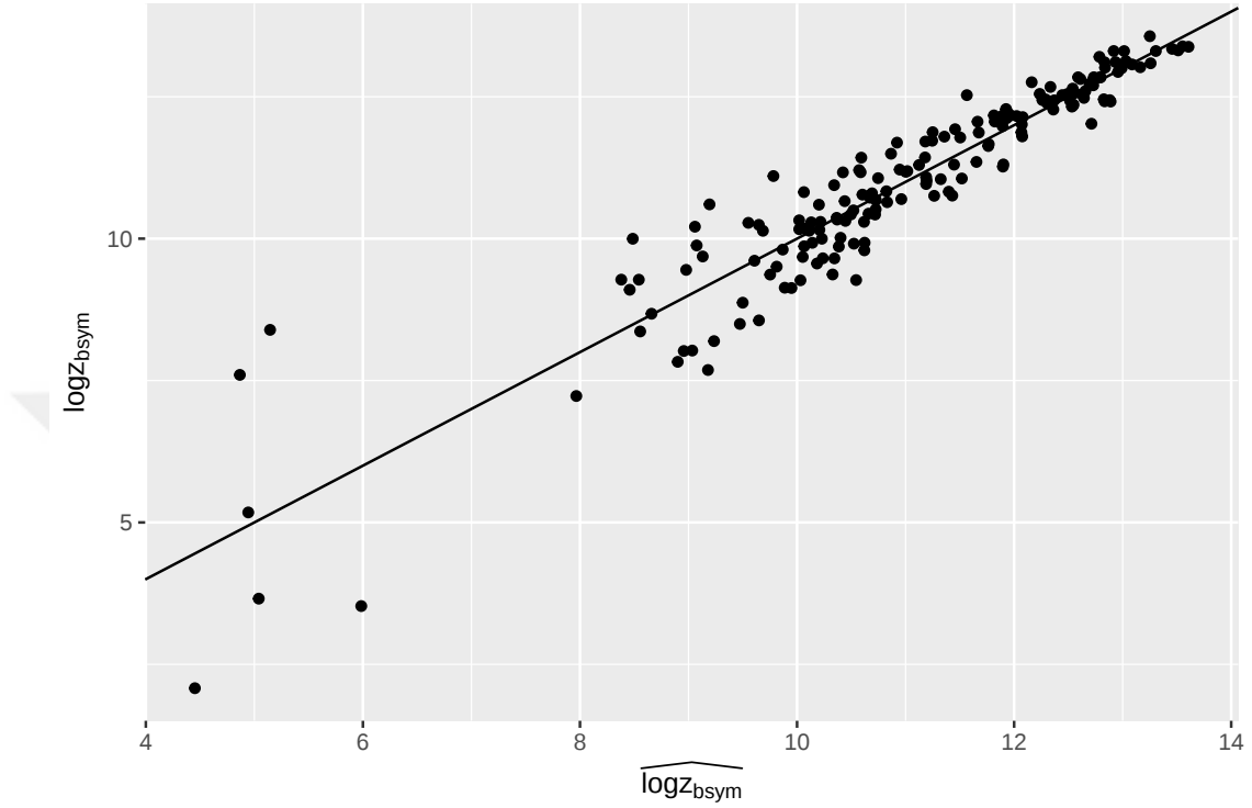
Figure 4.1: Plot of the fitted vs. observed values of the log normalized sales
