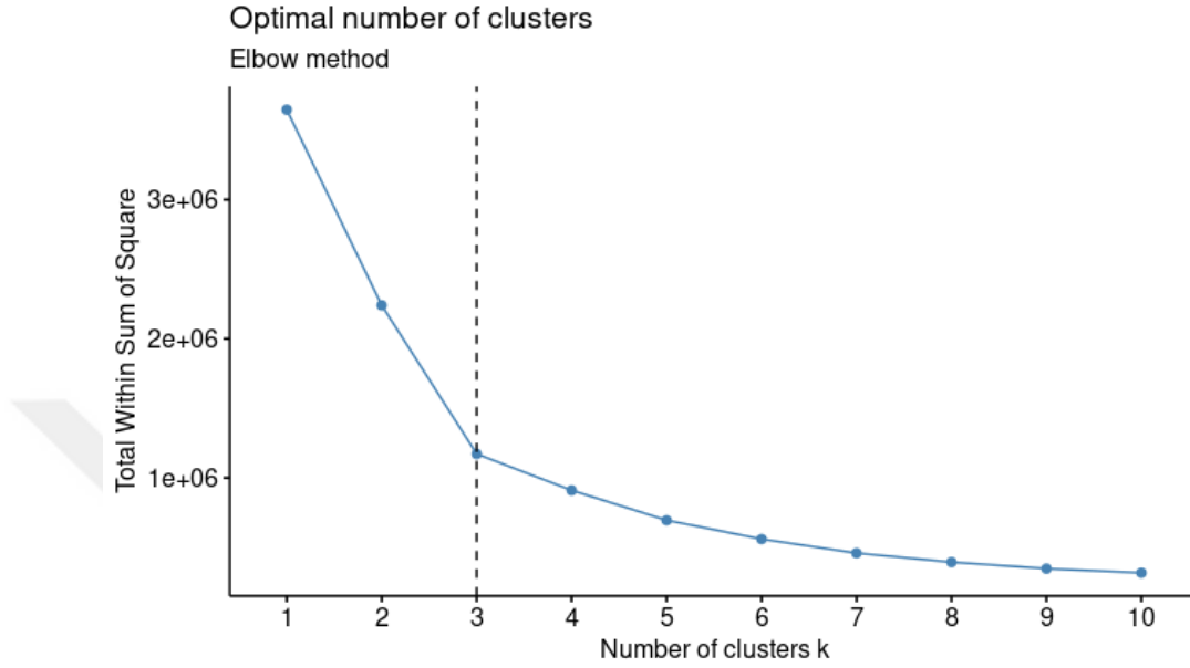
Figure 7.5: Optimal number of clusters using the Elbow method
