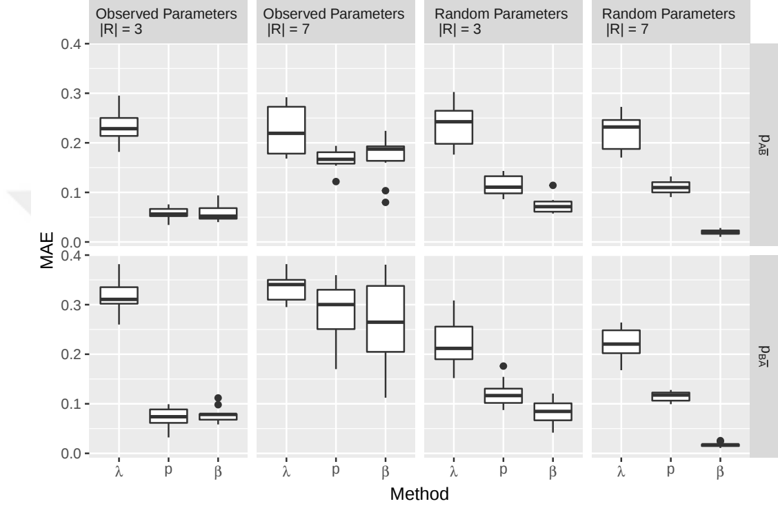
Figure 4.8: MAE comparison of all three methods
