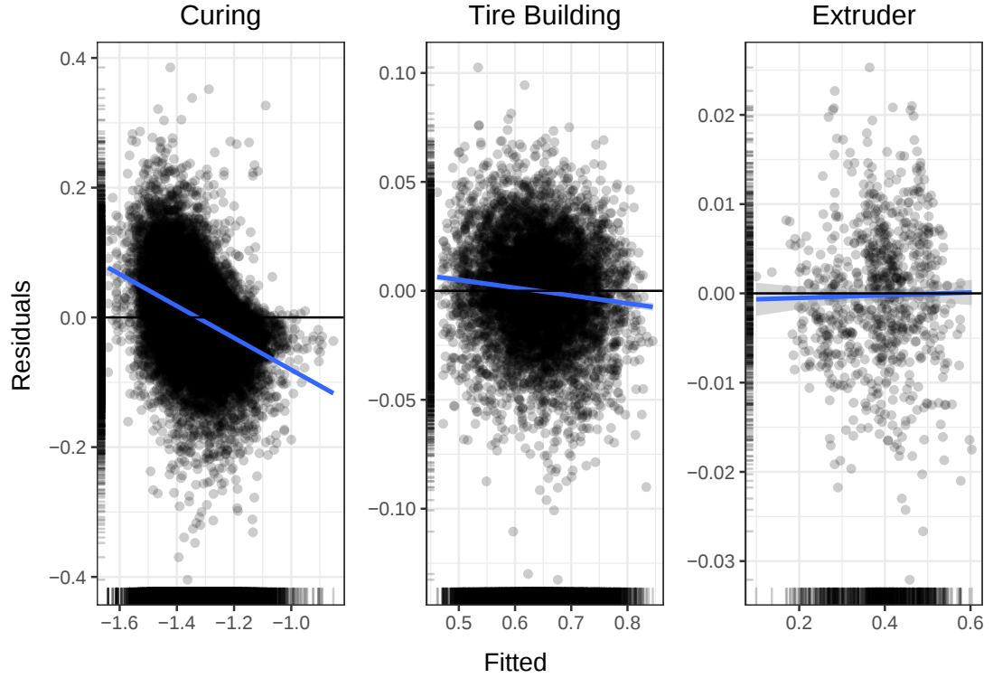
Figure 5.1: Residual Analysis plots of the machine learning models for the three machine groups
