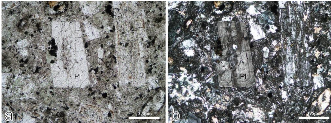
Figure 5.3 (a, b) Andesite. Hipocrystalline texture, P.N (plane nichols) ve C.N (crossed nichols) images, microlits are more dominated from volcanic glass and showing oscillatory concentric zoning in plagioclase. Pl: Plagioclase
