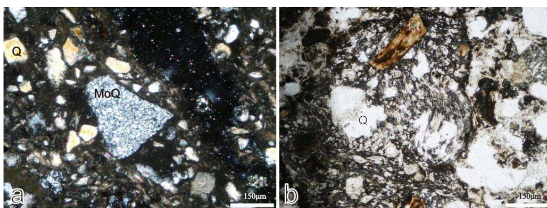
Figure 5.6 (a) Monolithic quartzs (MoQ) within ignimbrites, crossed nichols, rhyolitic lithic tuff. Quartz (Q) + Biotite (Bi) + Amphibole (Amp) + Pumice + Lithic fragments; (b) Cellular pumice within ignimbrite, Biotite and euhedral and embayed quartzs phenocrysts, crossed nichols.
