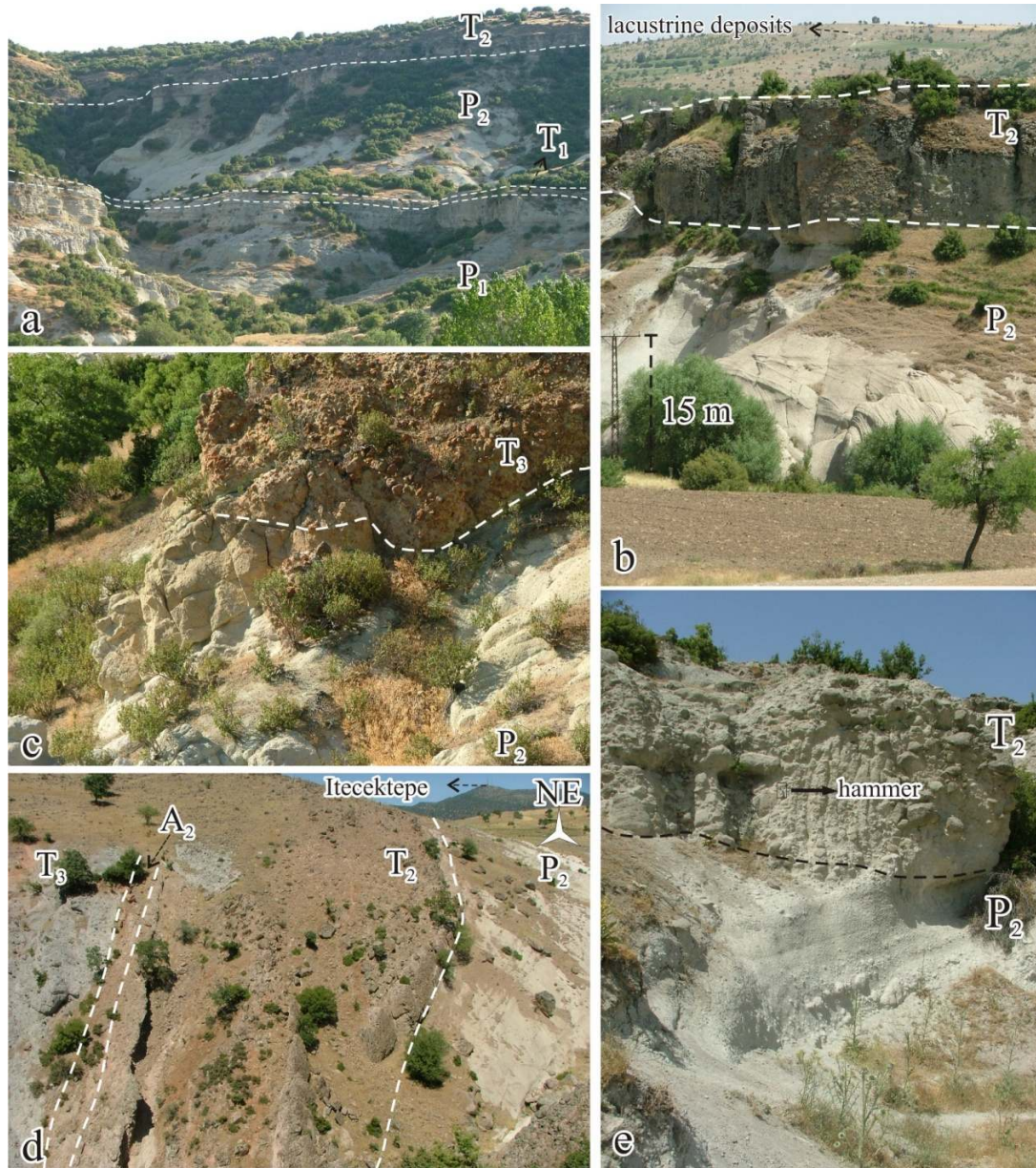
Figure 4.18 Field photographs of volcanic successions around the İtecektepe volcano. (a) Well-preserved exposure showing thick pyroclastic deposits ( P_1 and P_2 ; with T_1 and T_2 ); (b) interrelation between T_2 and P_2 , bottom level of the P_2 , displaying phreatomagmatic textures within surge deposits; (c) P_2 is terminated by T_3 , from Sec. 14 (see Figure 2 for location); (d) good-exposure from the western side of the volcano showing interrelation between P_2 and debris avalanche deposits, is divided by an ash fall ( A_2 ). The volcanic succession is truncated by a fault, which is placed at the eastern side of the photograph (not visible); (e) a dramatic transition from P_2 to T_2 .
