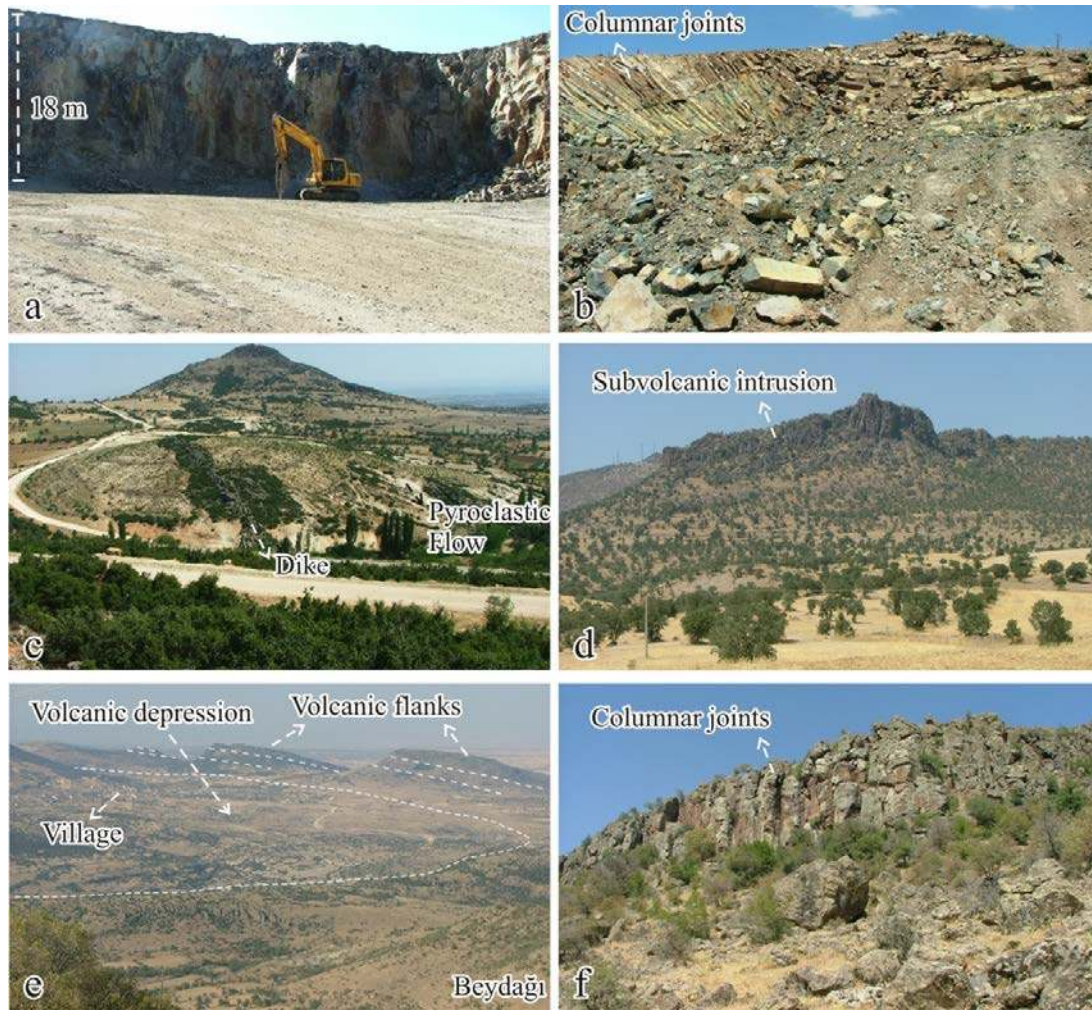
Figure 4.20 Field photographs showing the prominent volcanic edifices of the Elmadağ volcano. (a) Thick andesitic lava flow from the southern part of the volcano; (b) basaltic lavas showing columnar joints, in front of Mt. Beydağı; (c) NW–SE-trending latitic dike, which is cutting pyroclastic flow deposits at the inside of the volcanic depression; (d) subvolcanic intrusions, from southern part of the Mt. İtecektepe; (e) volcanic depression and volcanic flanks of the Beydağı, from Mt. Beydağı; (f) andesitic lavas showing columnar joints at the center of the volcano.
