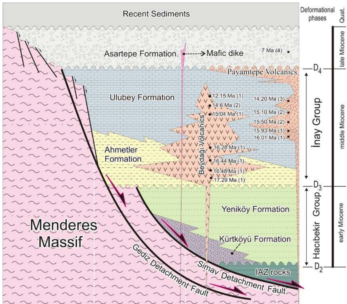
Figure 2.3 Tectono-stratigraphic columnar section of the NE-trending Uşak-Güre basin (D 2 -D 4 refers to deformation phase). Age data: (1) Karaoğlu et al. (2010); (2) Seyitoğlu (1997); (3) Innocenti et al. (2005); (4) Seyitoğlu et al. (2009).
