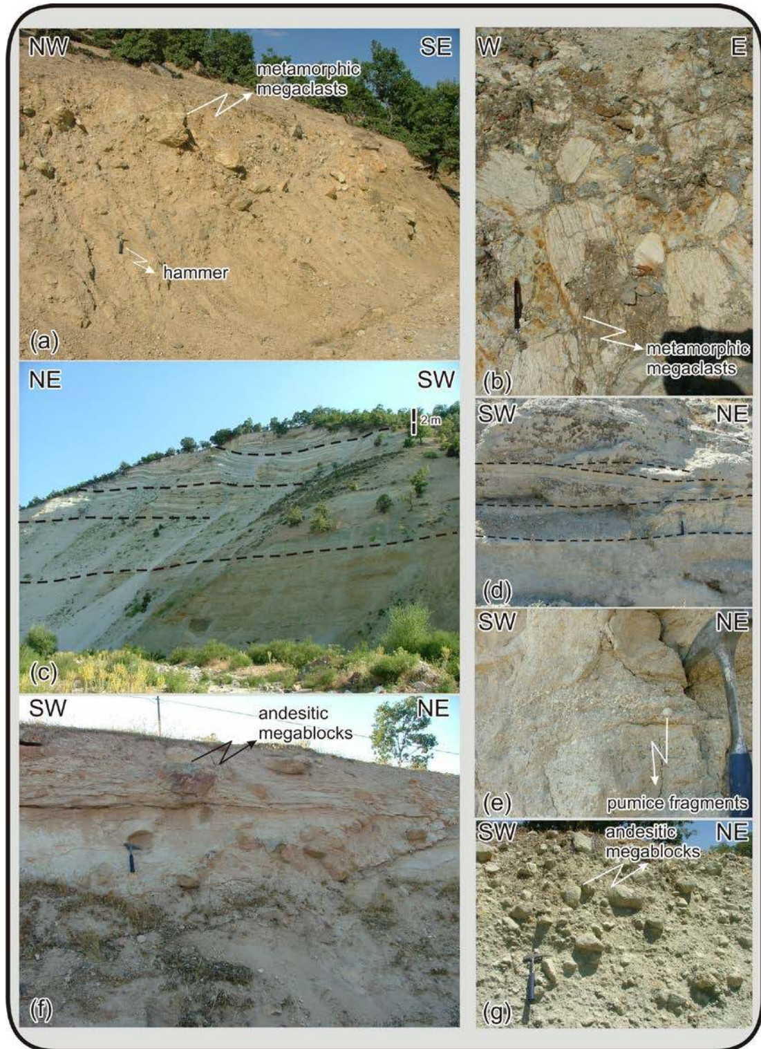
Figure 2.11 Three distinct members of the Ahmetler formation. (a) Photograph showing matrix-supported Merdivenlikuyu block member which reflecting basal layer of the Ahmetler formation, in the western margin of the Güre basin. (b) Close-up view of Merdivenlikuyu member showing subordinate matrix-supported metamorphic breccias and blocks, near the western margin. (c) Balçıklıdere member with siltstone and mudstone horizontal bedding, near Kıran village-western side
