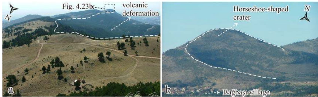
Figure 4.23 Volcanic depression structures over the Elmadağ volcano. (a) Photo was taken from NW to SE across the edifice; (b) one of the small-scale (ca. 300 m in diameter) horse shoe-shaped flank collapse of the Elmadağ volcano.
