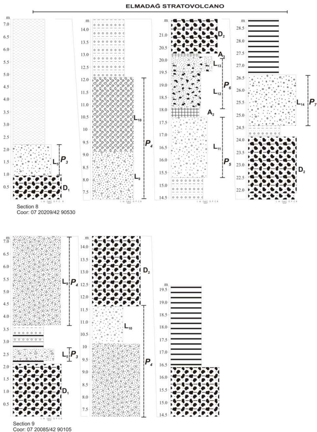
Figure 4.8 Typical columnar sections of the Elmadag stratovolcano (Sections 8–9 see Figure 2 for locations and Figure 4.7 for legend).
