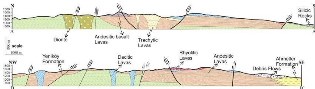
Figure 4.4 Geological cross-sections across the Elmadag stratovolcano (see Figure 4.3 for localities and legends).
