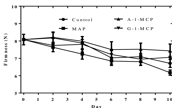
Figure 4.2. Changes in firmness of cucumbers stored at 23 \pm 1 °C
