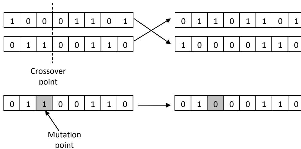
Figure 3.8: Crossover & Mutation
