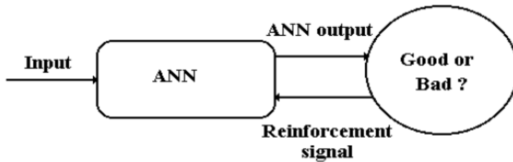
Figure 3.3: Reinforcement Learning
