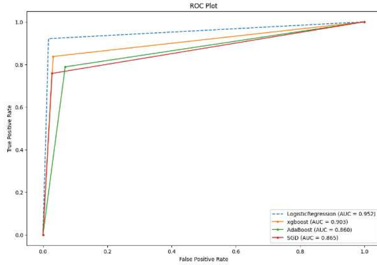
Figure 4.9 The ROC plot results for obtained ML models after applying 80:20 before applying SMOTE
