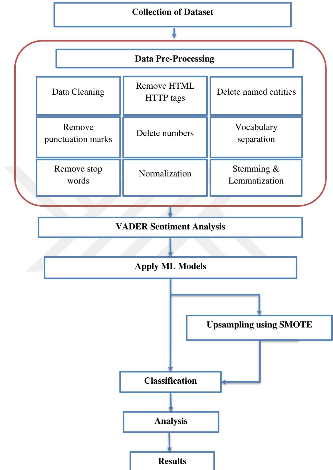
Figure 3.1 The proposed research framework
