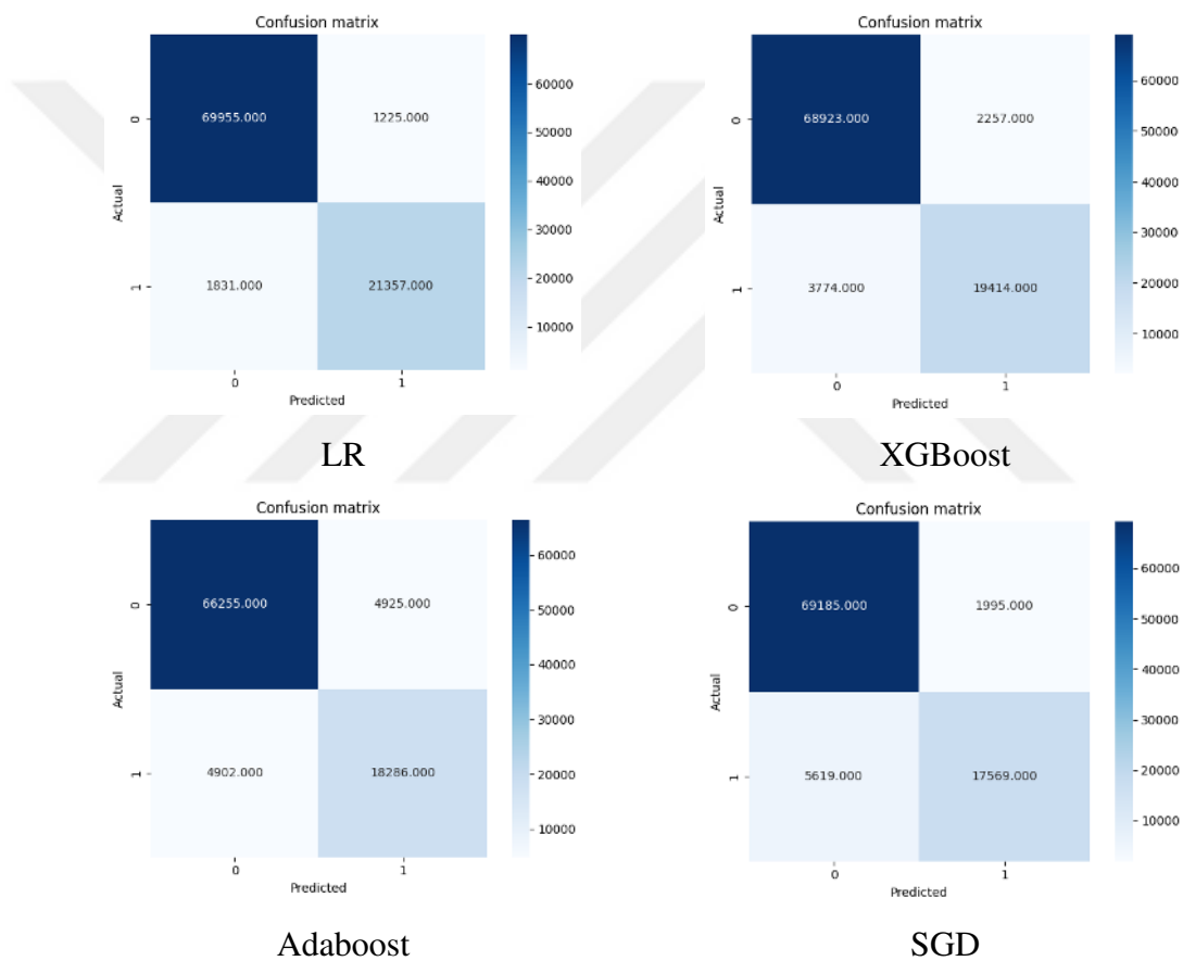
Figure 4.8 Confusion matrix for applied ML models
