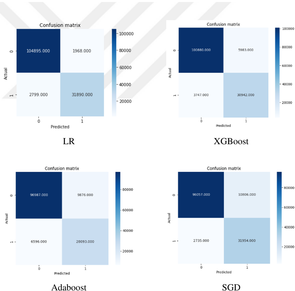
Figure 4.12 Confusion matrix for applied ML models
