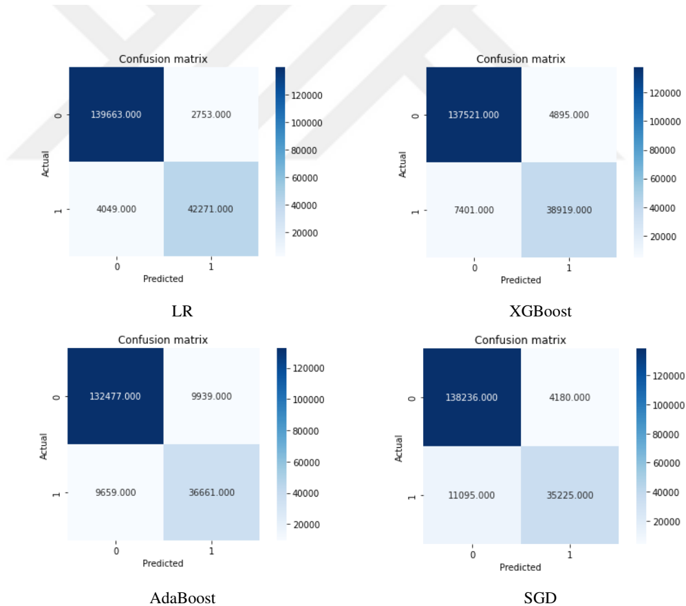
Figure 4.4 Confusion matrix for applied ML models
