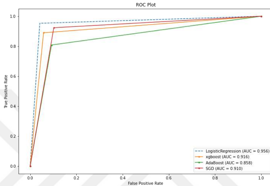
Figure 4.11 The ROC plot results for obtained ML models after applying 60:40 after applying SMOTE
