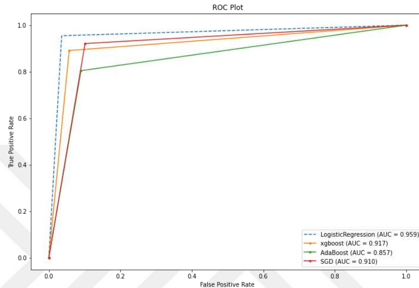
Figure 4.15 The ROC plot results for obtained ML models after applying 80:20 after applying SMOTE
