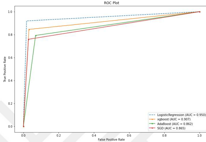
Figure 4.7 The ROC plot results for obtained ML models after applying 70:30 before applying SMOTE
