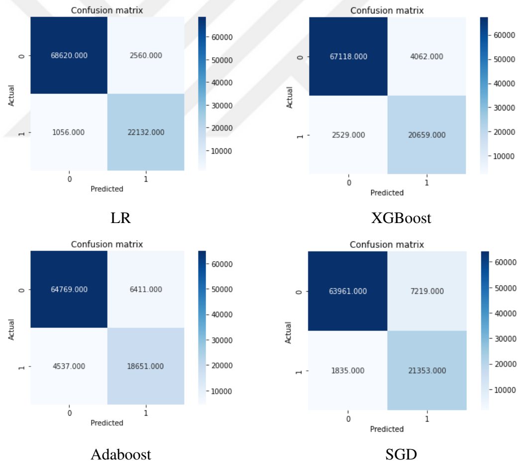
Figure 4.14 Confusion matrix for applied ML models
