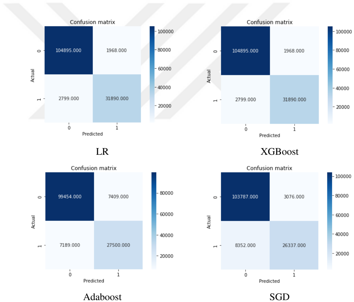
Figure 4.6 Confusion matrix for applied ML models
