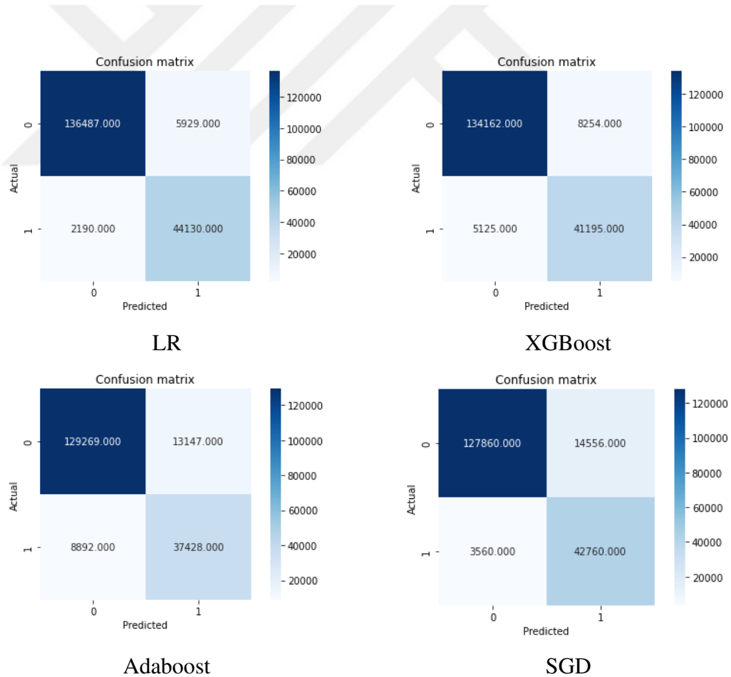
Figure 4.10 Confusion matrix for applied ML models
