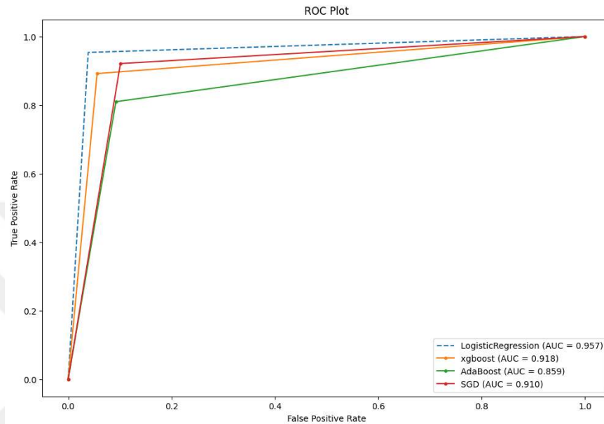
Figure 4.13 The ROC plot results for obtained ML models after applying 70:30 after applying SMOTE
