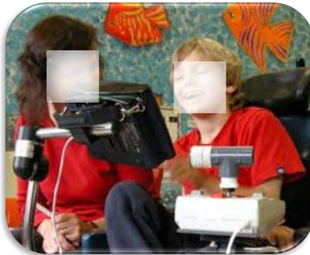
Figure 2.7 : AAC sample
