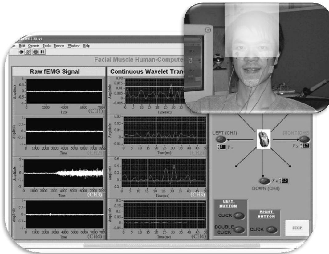
Figure 2.16 : Facial electromyography
