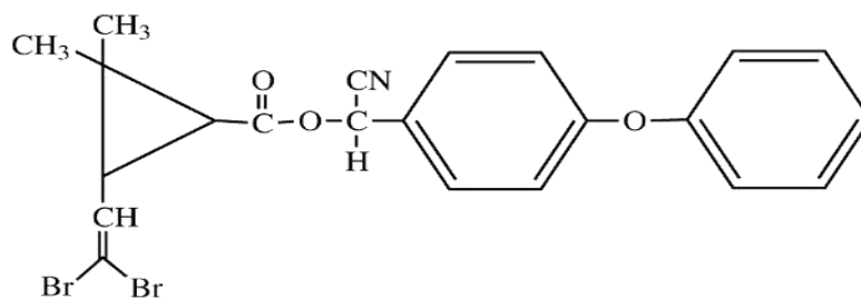
Figure 1.1 Molecular structure of deltamethrin, C_{22}H_{19}Br_2NO_3 .
