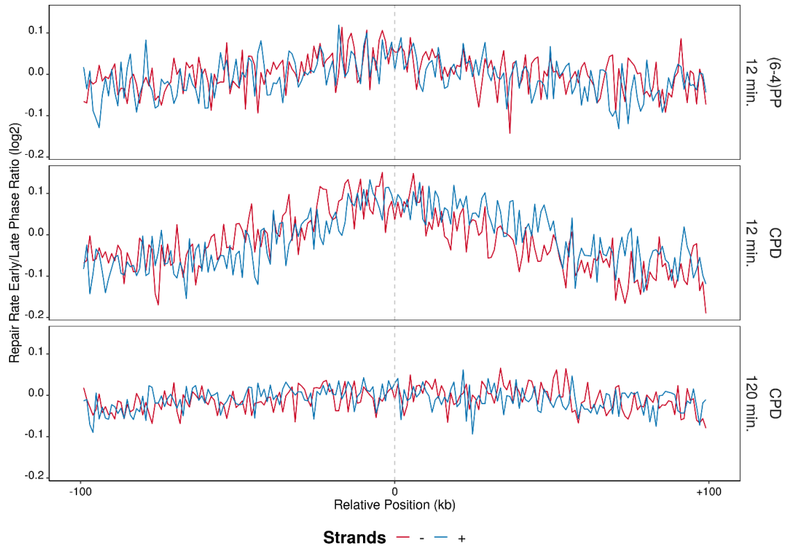
Figure 6.41 After log 2 -transformed repair rates (XR-seq/Damage-seq) are calculated, samples that are at early S phase of the cell cycle are further divided by the ones that are at the late S phase (early/late) in 200 kb windows with 1 kb intervals, which initiation zones are positioned at the center of the region. The blue lines are the plus strands and red lines are the minus strands. Analysis is performed on replicate B.
