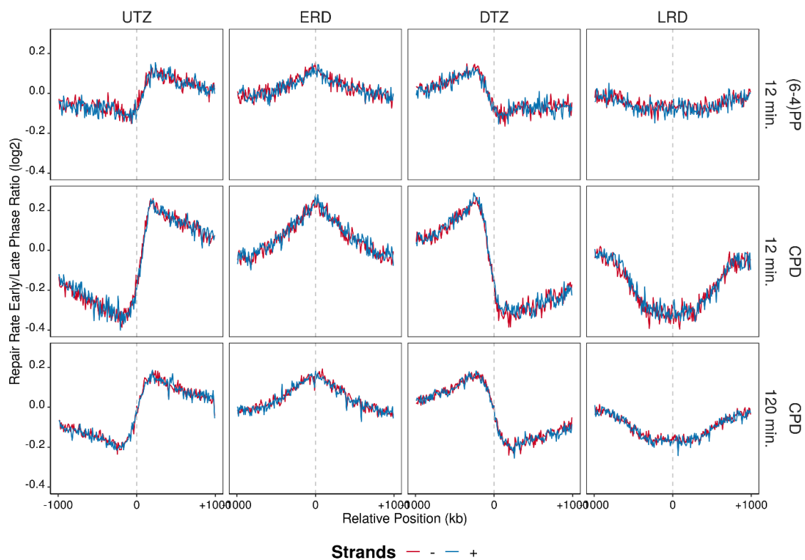
Figure 6.29 After log2-transformed repair rates (XR-seq/Damage-seq) are calculated, samples that are at early S phase of the cell cycle are further divided by the ones that are at the late S phase (early/late) in 2 Mb windows with 10 kb intervals, which replication domains are positioned at the center of the region. The blue lines are the plus strands and red lines are the minus strands. Analysis is performed on replicate B.
