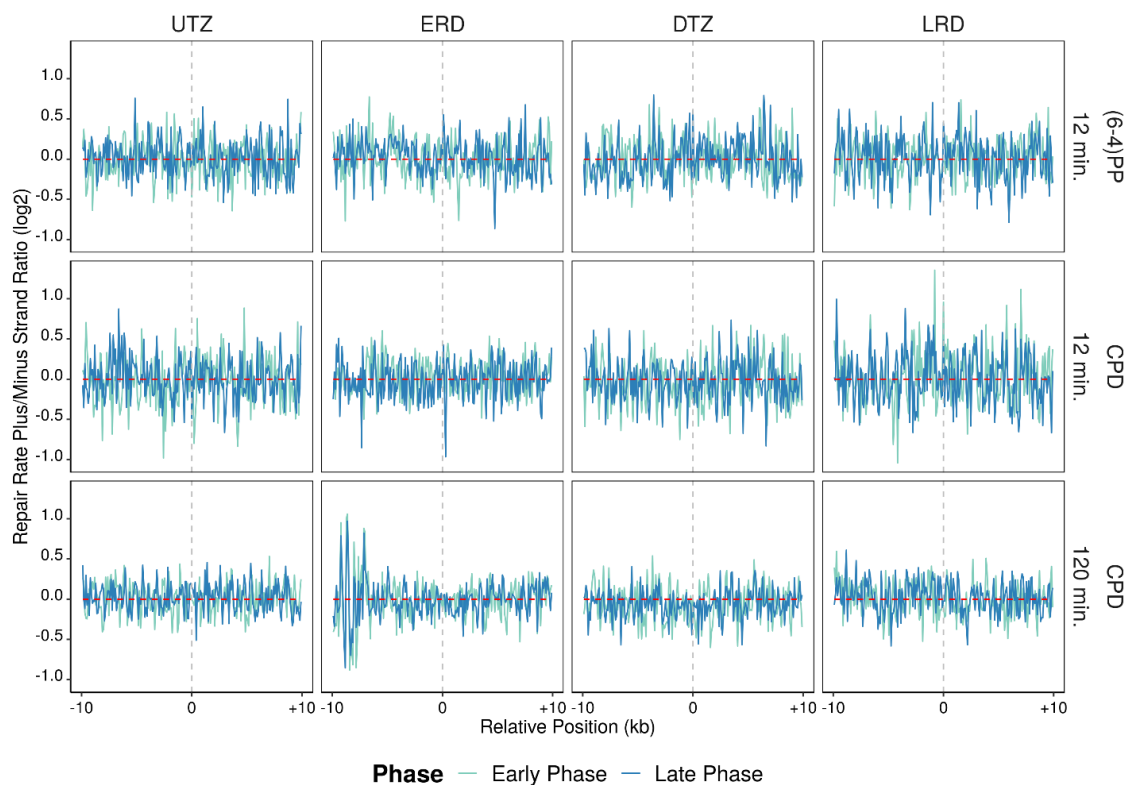
Figure 6.31 After log2-transformed repair rates (XR-seq/Damage-seq) are calculated, plus strands of the samples are further divided to minus strands (plus/minus) in 20 kb windows with 100 base pair intervals, which replication domains are positioned at the center of the region. Light blue lines are the early phase samples and dark blue lines are the late phase samples. Analysis is performed on replicate B.
