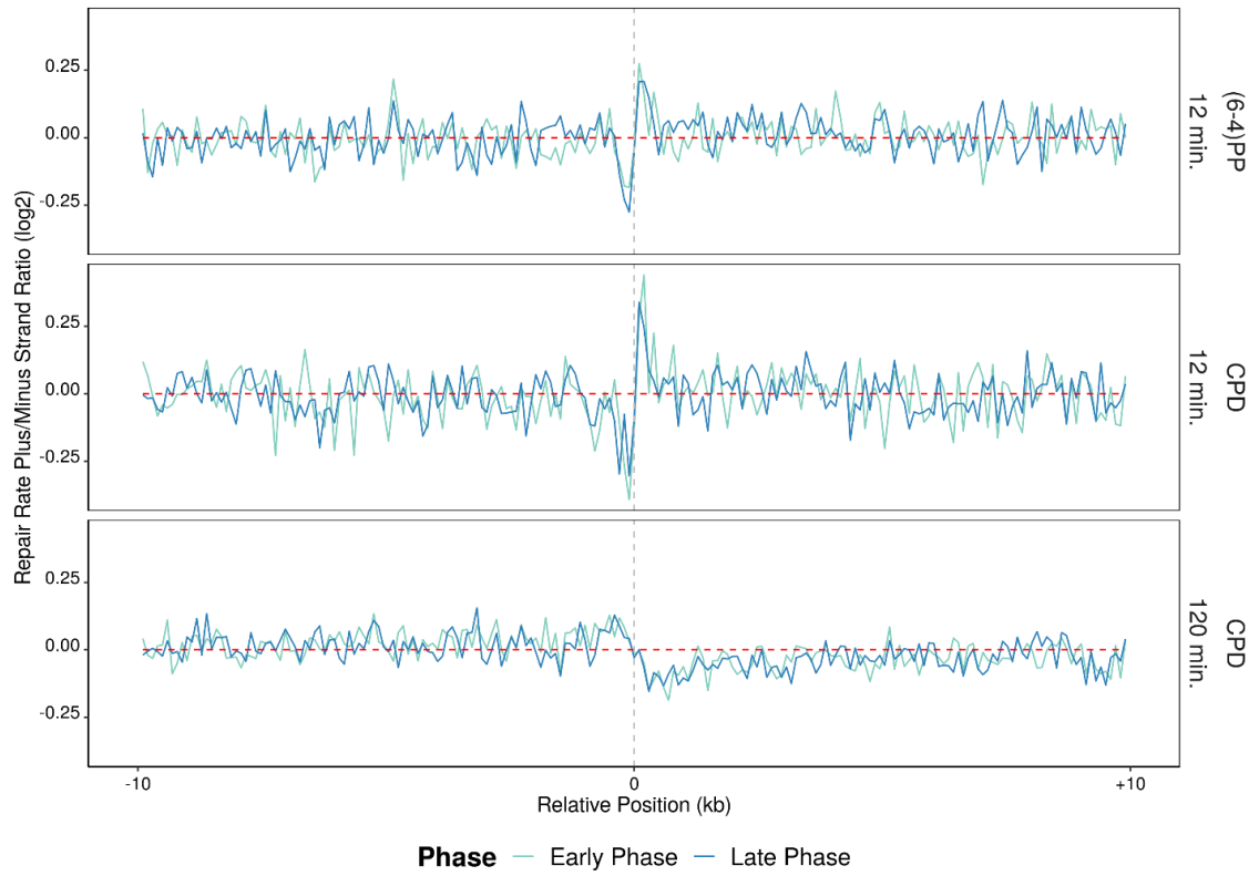
Figure 6.60 After log 2 -transformed repair rates (XR-seq/Damage-seq) are calculated, plus strands of the samples are further divided to minus strands (plus/minus) in 20 kb windows with 100 base pair intervals, which replication origins (SNS-seq) are positioned at the center of the region. Light blue lines are the early phase samples and dark blue lines are the late phase samples. Analysis is performed on replicate A.
