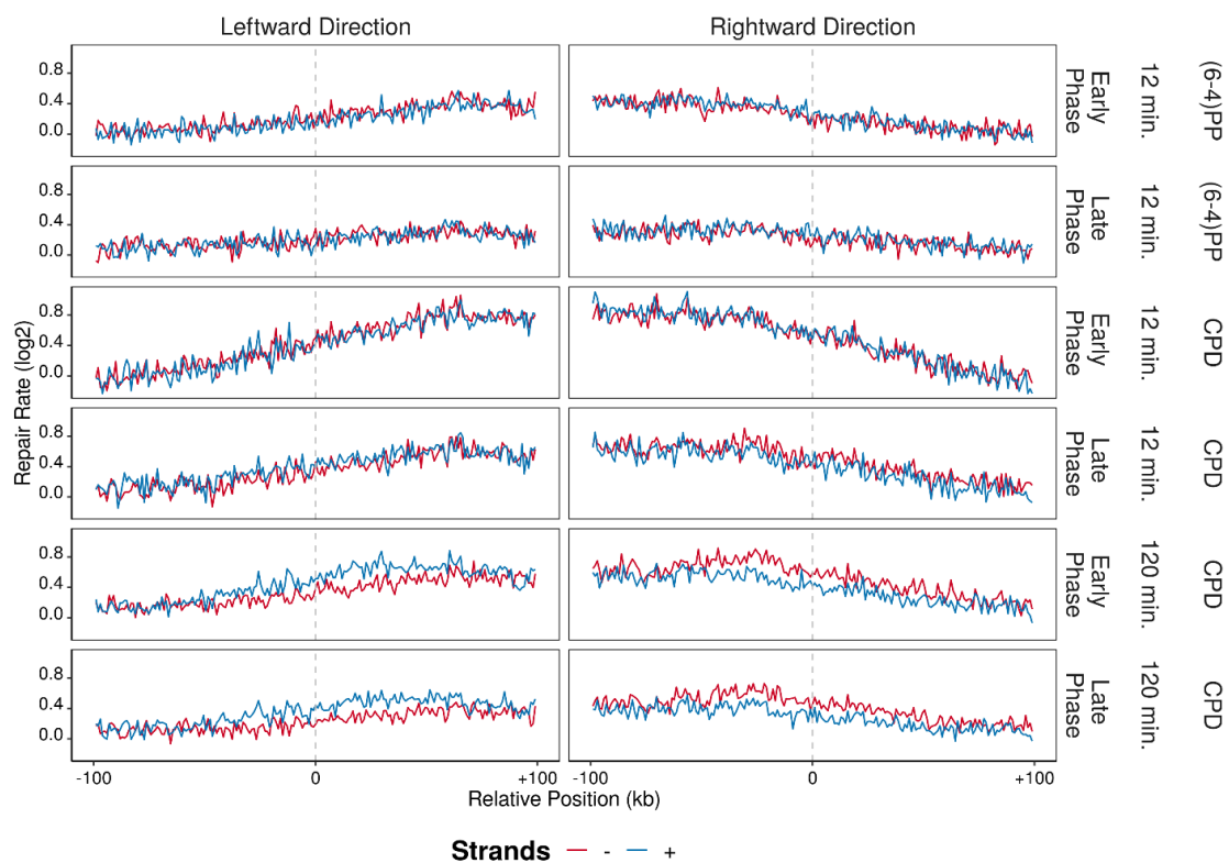
Figure 6.65 Repair rates (XR-seq/Damage-seq) of high RFD regions are calculated at both leftward and rightward directions and log2-transformed in 200 kb windows with 1 kb intervals. The blue lines are the plus strands and red lines are the minus strands. Analysis is performed on replicate B.
