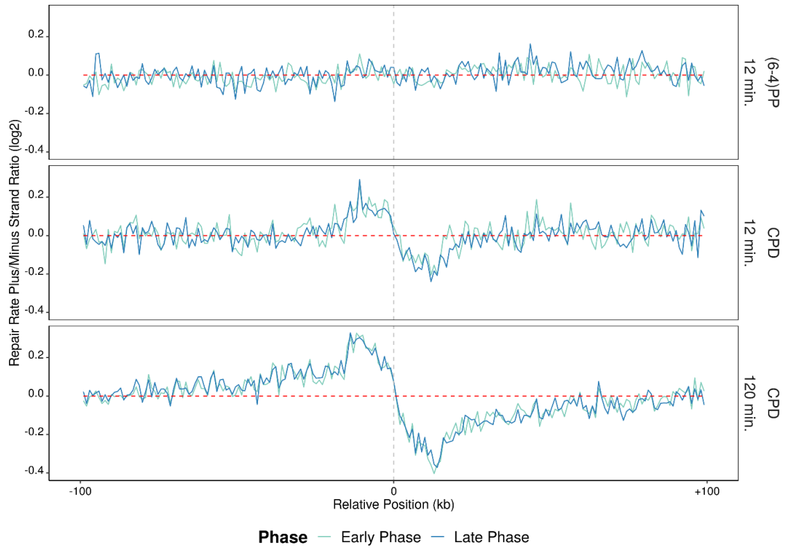
Figure 6.44 After log2-transformed repair rates (XR-seq/Damage-seq) are calculated, plus strands of the samples are further divided to minus strands (plus/minus) in 200 kb windows with 1 kb intervals, which initiation zones are positioned at the center of the region. Light blue lines are the early phase samples and dark blue lines are the late phase samples. Analysis is performed on replicate A.
