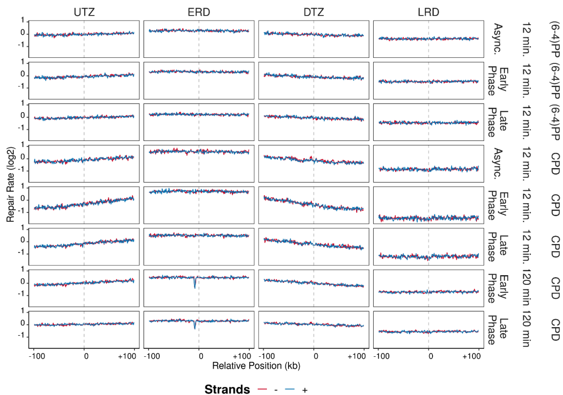
Figure 6.20 Repair rates (XR-seq/Damage-seq) are calculated and log2-transformed in 200 kb windows with 1 kb intervals, which replication domains are positioned at the center of the region. The blue lines are the plus strands and red lines are the minus strands. Analysis is performed on replicate A.
