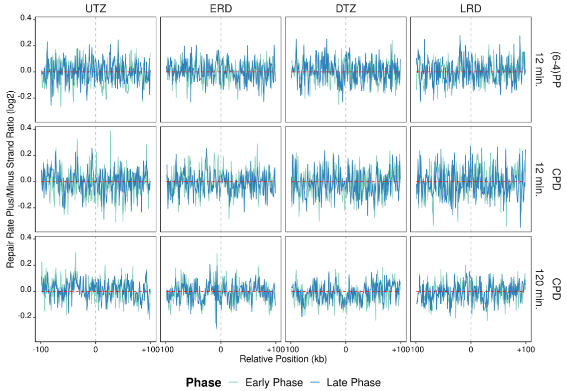
Figure 6.33 After log2-transformed repair rates (XR-seq/Damage-seq) are calculated, plus strands of the samples are further divided to minus strands (plus/minus) in 200 kb windows with 1 kb intervals, which replication domains are positioned at the center of the region. Light blue lines are the early phase samples and dark blue lines are the late phase samples. Analysis is performed on replicate B.
