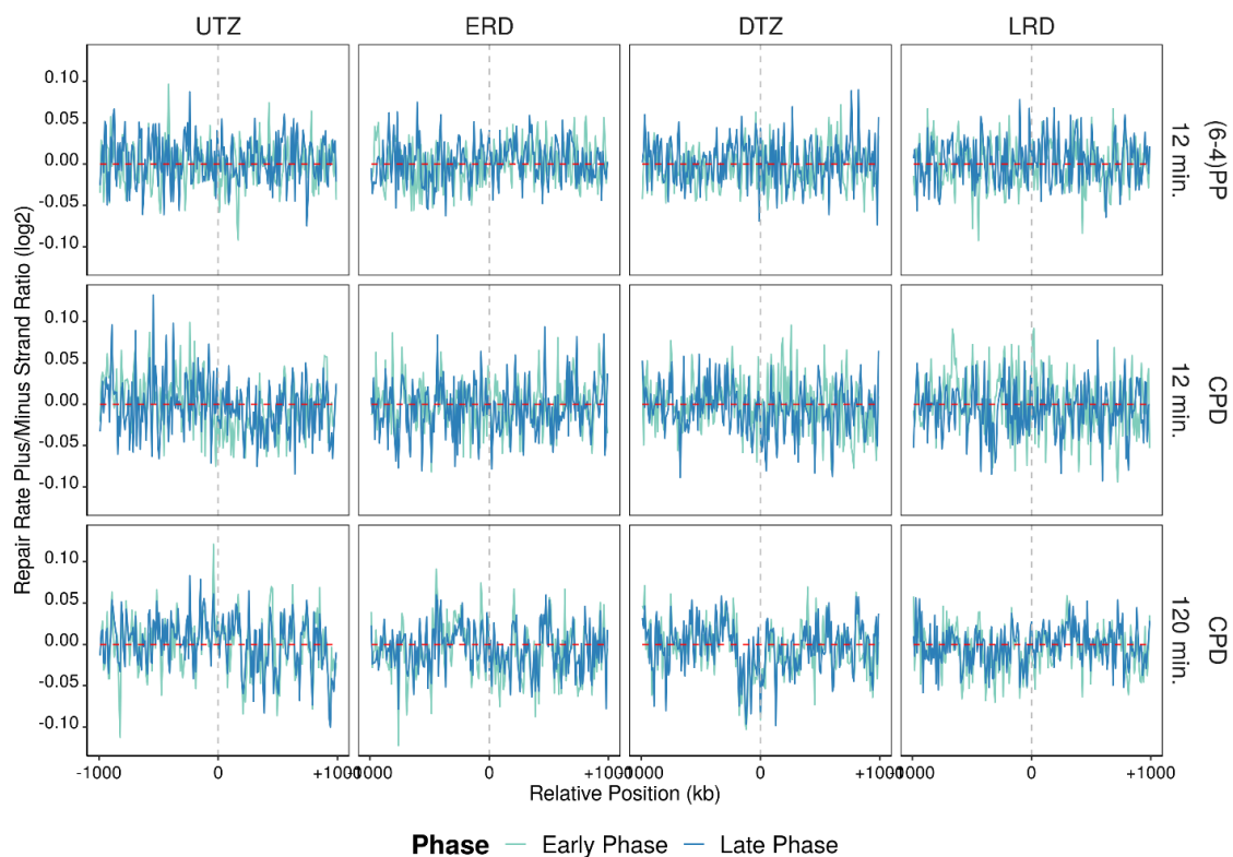
Figure 6.35 After log2-transformed repair rates (XR-seq/Damage-seq) are calculated, plus strands of the samples are further divided to minus strands (plus/minus) in 2 Mb windows with 10 kb intervals, which replication domains are positioned at the center of the region. Light blue lines are the early phase samples and dark blue lines are the late phase samples. Analysis is performed on replicate B.
