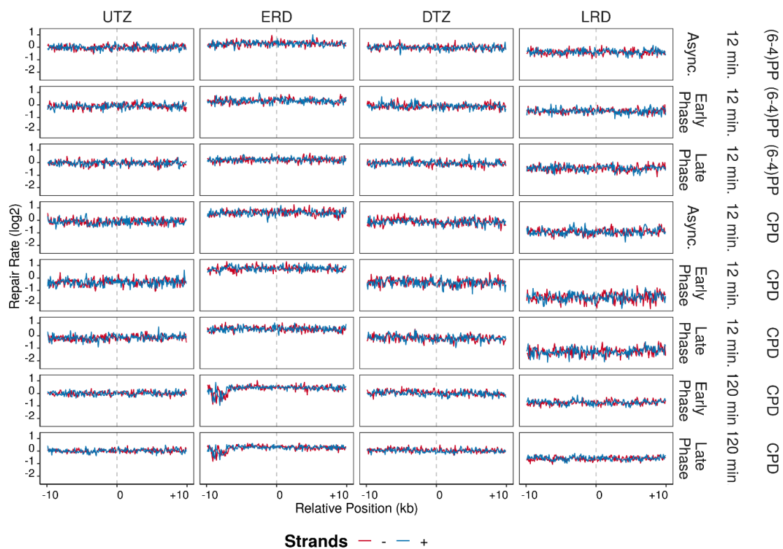
Figure 6.18 Repair rates (XR-seq/Damage-seq) are calculated and log2-transformed in 20 kb windows with 100 base pair intervals, which replication domains are positioned at the center of the region. The blue lines are the plus strands and red lines are the minus strands. Analysis is performed on replicate A.
