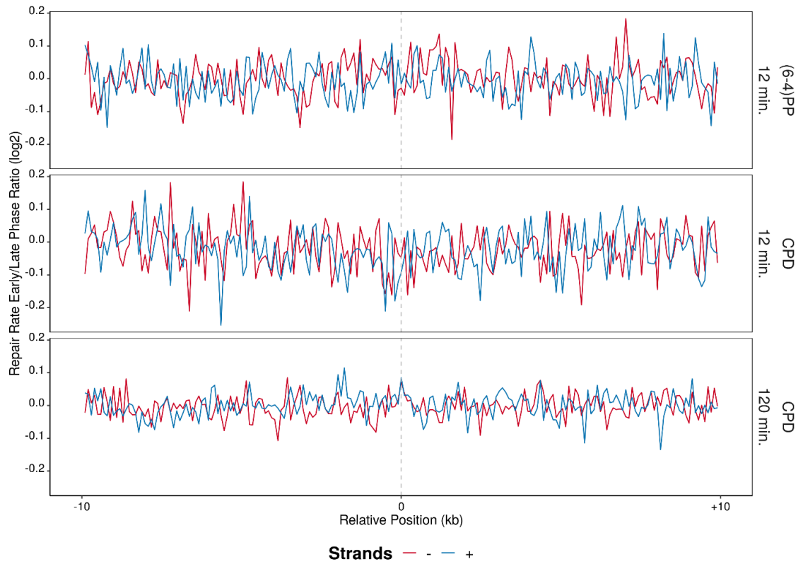
Figure 6.56 After log 2 -transformed repair rates (XR-seq/Damage-seq) are calculated, samples that are at early S phase of the cell cycle are further divided by the ones that are at the late S phase (early/late) in 20 kb windows with 100 base pair intervals, which replication origins (SNS-seq) are positioned at the center of the region. The blue lines are the plus strands and red lines are the minus strands. Analysis is performed on replicate A.
