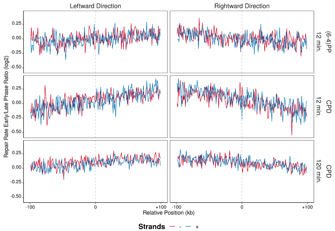
Figure 6.70 After log 2 -transformed repair rates (XR-seq/Damage-seq) of high RFD regions are calculated at both leftward and rightward directions, samples that are at early S phase of the cell cycle are further divided by the ones that are at the late S phase (early/late) in 200 kb windows with 1 kb intervals. The blue lines are the plus strands and red lines are the minus strands. Analysis is performed on replicate A.
