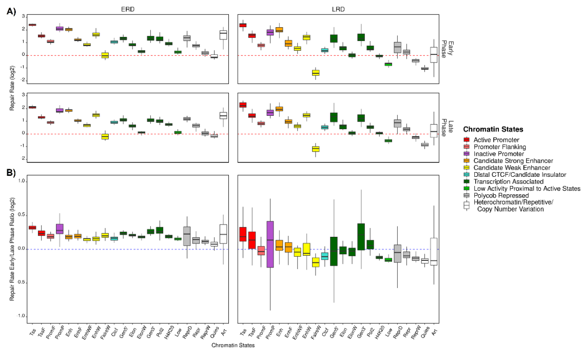
Figure 6.17 The effect of Chromatin States on repair efficiency of the replication domains. A) Repair rates (XR-seq/Damage-seq) of CPD samples at 120 minutes are calculated, log2-transformed B) and for every region, the repair rates at early S phase divided by repair rates at late S phase to layout the skewness of the repair rate to a phase of replication. The analysis is performed on replicate B.
