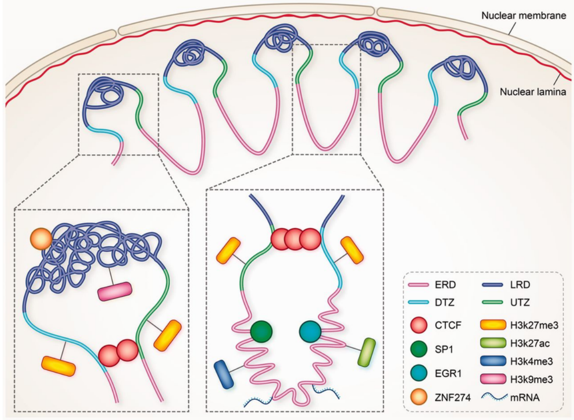
Figure 1.1 Model of replication domains and its chromatin organization (Liu et al., 2016).
