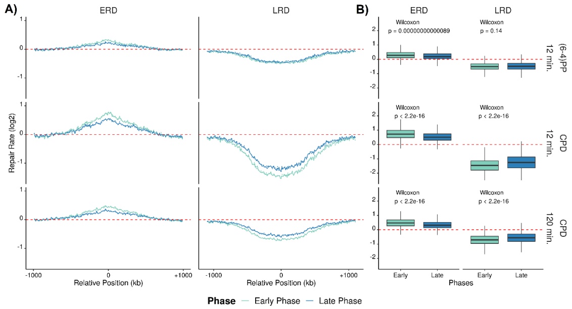
Figure 4.2 The shift of repair efficiency in replication domains during replication. A) Repair rates (XR-seq/Damage-seq) are calculated and log2-transformed in 2 Mb regions with 10 kb intervals, which early replication domains (ERDs, left) and late replication domains (LRDs, right) positioned at the center of the region. B) RPKM values of XR-seq samples are divided by Damage-seq samples (Repair Rate) for each ERD (left) and LRD (right) domains and log2-transformed. Wilcoxon test is used to assess the significance of difference between early and late S phases. The light blue lines are the early phase repair rate values and dark blue lines are the late phase repair rate values. Above the red horizontal dashed line demonstrates that repair is higher than damage, below demonstrates that damage is higher. Analysis is performed on replicate A.
