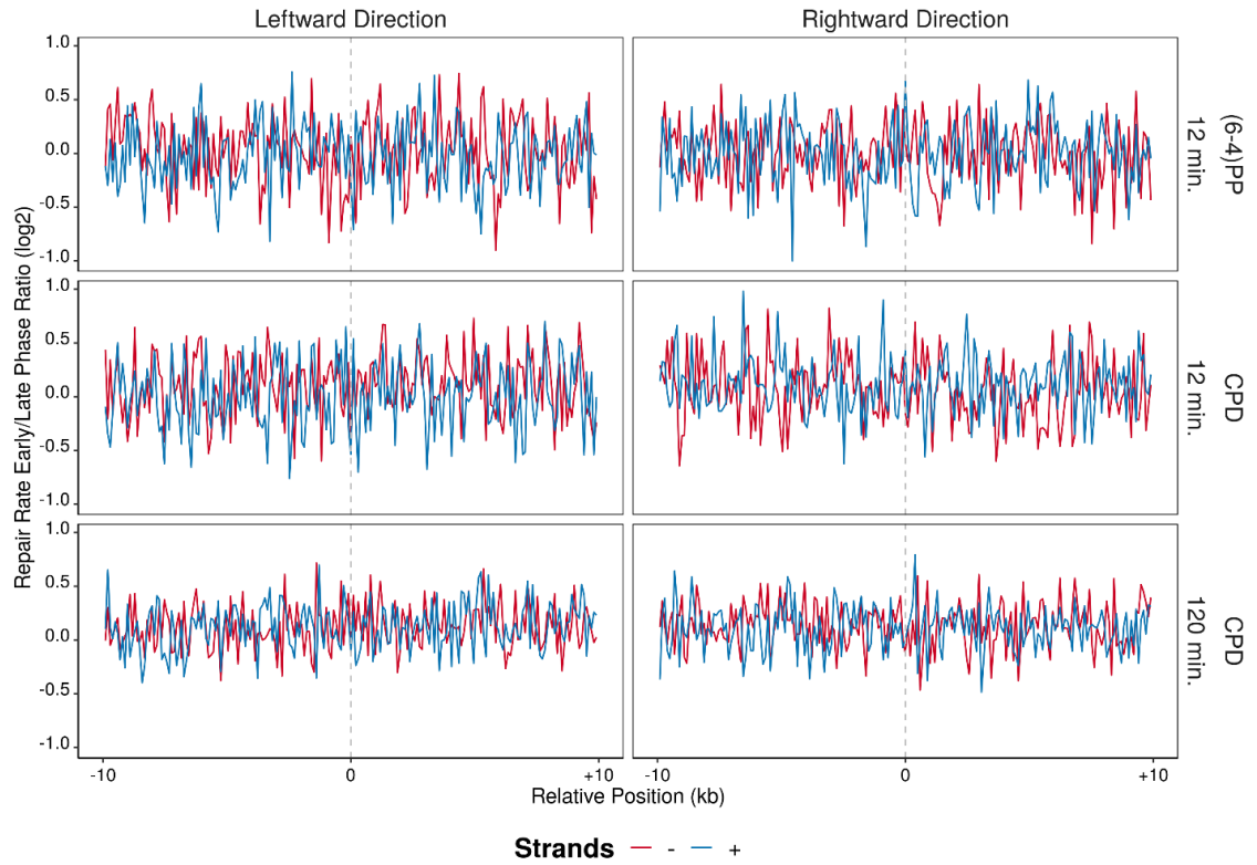
Figure 6.69 After log 2 -transformed repair rates (XR-seq/Damage-seq) of high RFD regions are calculated at both leftward and rightward directions, samples that are at early S phase of the cell cycle are further divided by the ones that are at the late S phase (early/late) in 20 kb windows with 100 base pair intervals. The blue lines are the plus strands and red lines are the minus strands. Analysis is performed on replicate B.
