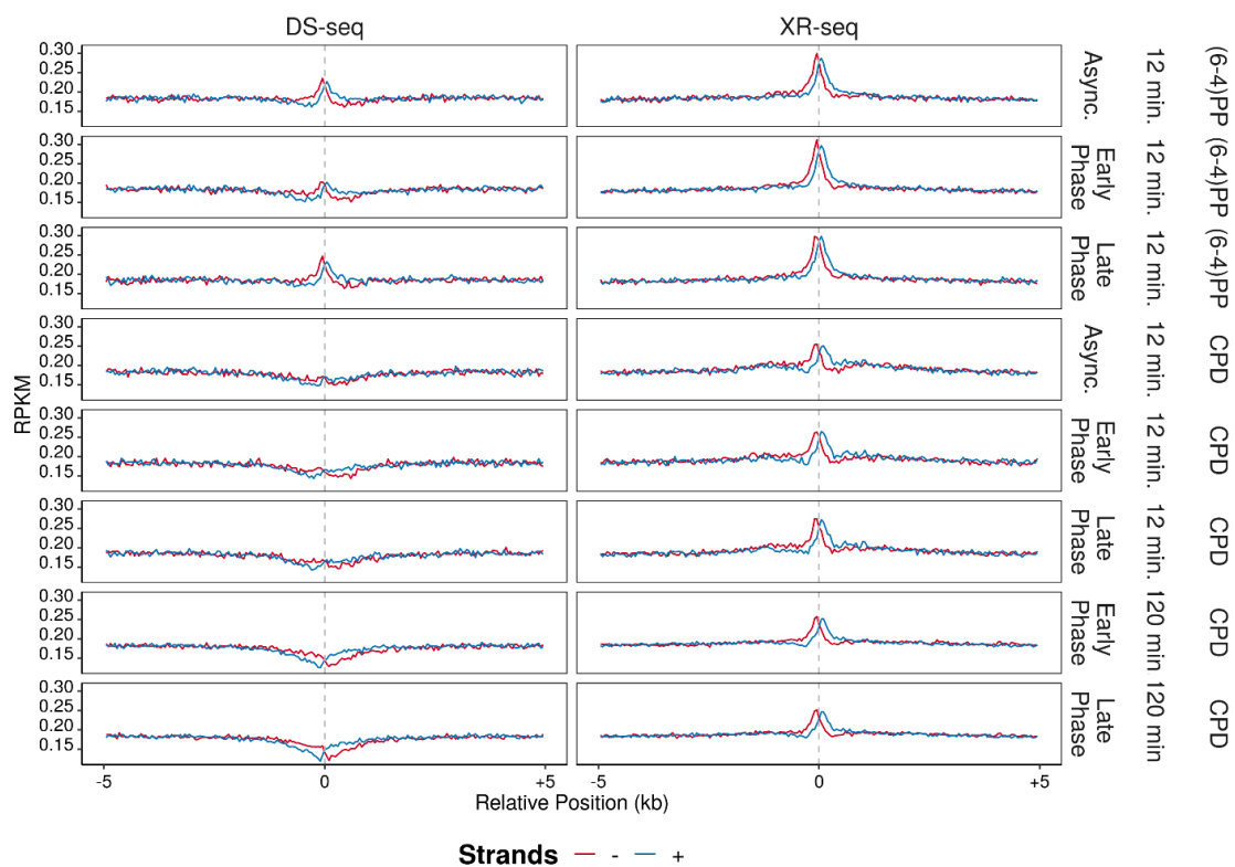
Figure 6.47 RPKM values of Damage-seq samples (left) and XR-seq samples (right) are calculated in 10 kb windows with 50 base pair intervals, which replication origins (SNS-seq) are positioned at the center of the region. Blue lines represent the plus strands and red lines represent the minus strands. Gray vertical dashed line shows the center of the region. Analysis is performed on replicate B.
