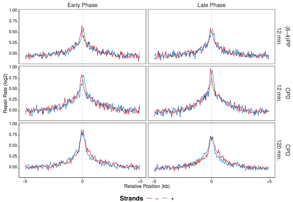
Figure 6.51 Repair rates (XR-seq/Damage-seq) are calculated and log2-transformed in 10 kb windows with 50 base pair intervals, which replication origins (SNS-seq) are positioned at the center of the region. The blue lines are the plus strands and red lines are the minus strands. Analysis is performed on replicate B.
