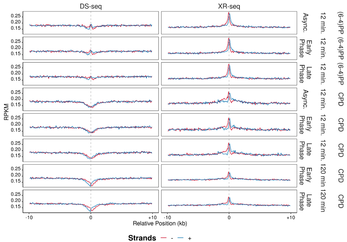
Figure 6.48 RPKM values of Damage-seq samples (left) and XR-seq samples (right) are calculated in 20 kb windows with 100 base pair intervals, which replication origins (SNS-seq) are positioned at the center of the region. Blue lines represent the plus strands and red lines represent the minus strands. Gray vertical dashed line shows the center of the region. Analysis is performed on replicate A.
