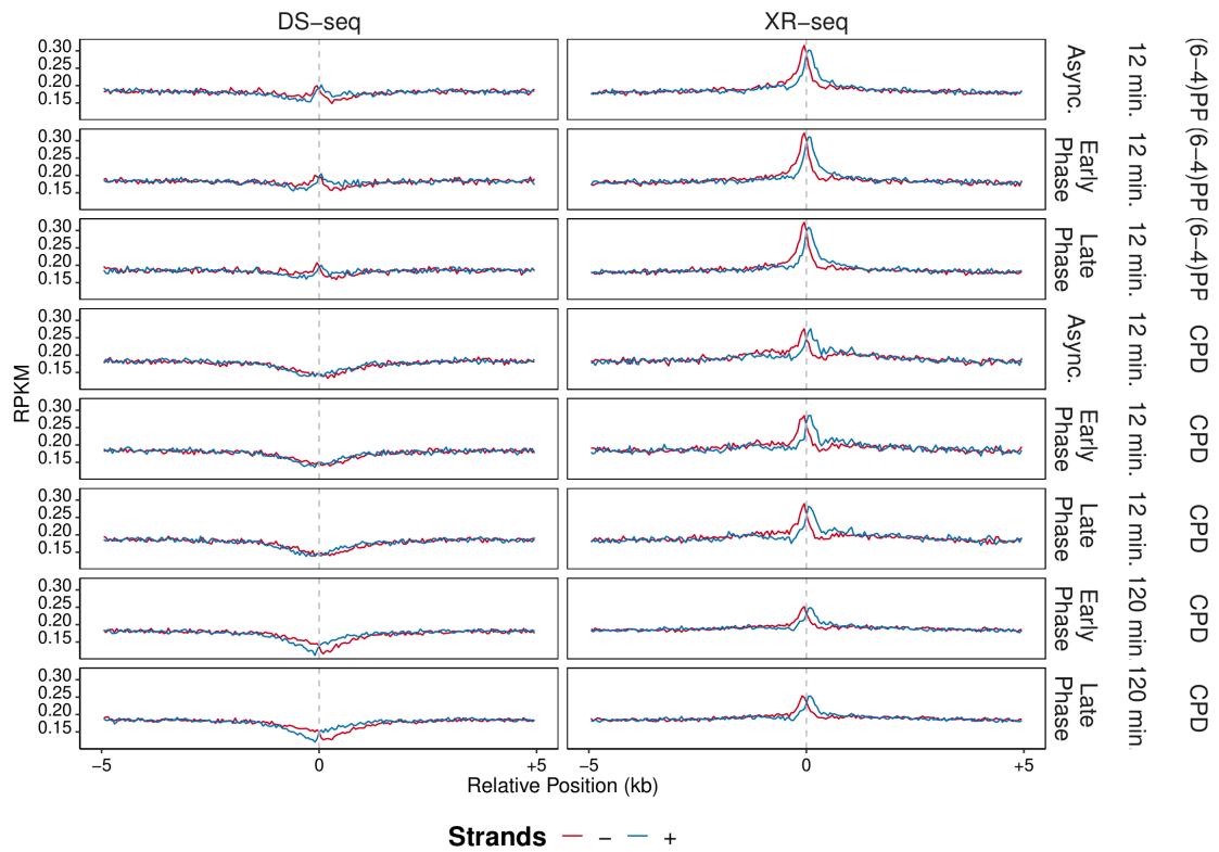
Figure 6.46 RPKM values of Damage-seq samples (left) and XR-seq samples (right) are calculated in 10 kb windows with 50 base pair intervals, which replication origins (SNS-seq) are positioned at the center of the region. Blue lines represent the plus strands and red lines represent the minus strands. Gray vertical dashed line shows the center of the region. Analysis is performed on replicate A.
