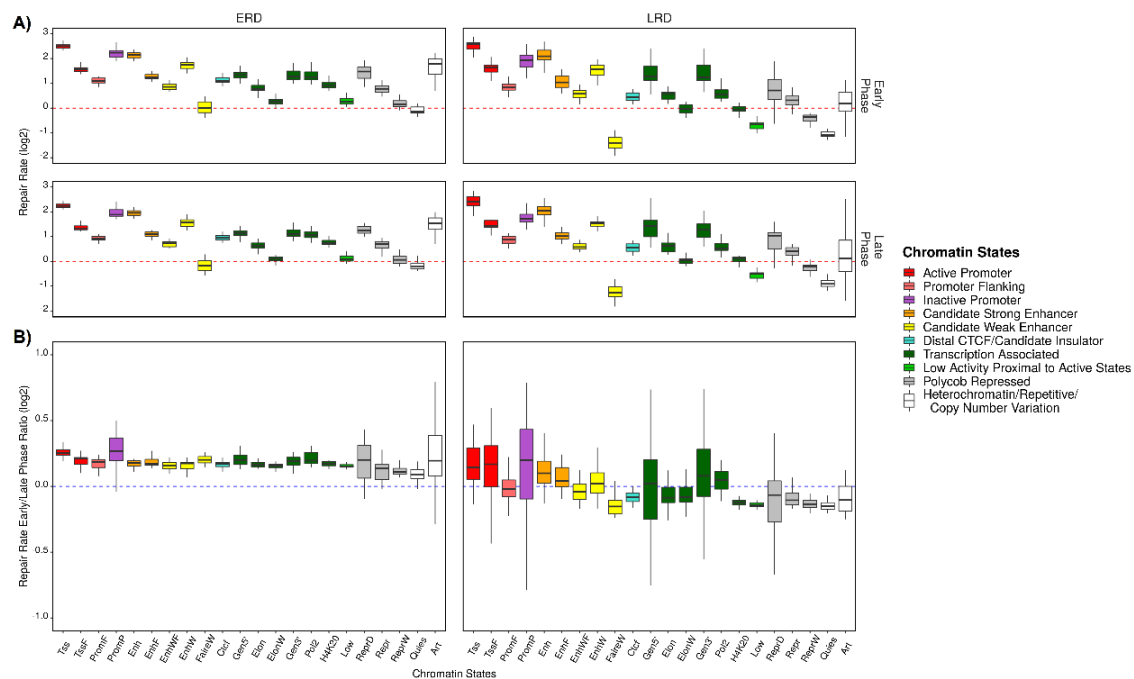
Figure 6.16 The effect of Chromatin States on repair efficiency of the replication domains. A) Repair rates (XR-seq/Damage-seq) of CPD samples at 120 minutes are calculated, log2-transformed, B) and for every region, the repair rates at early S phase divided by repair rates at late S phase to layout the skewness of the repair rate to a phase of replication. The analysis is performed on replicate A.
