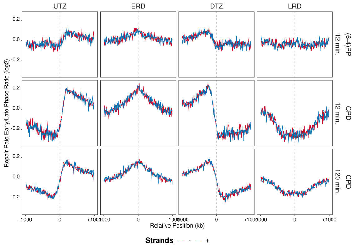
Figure 6.28 After log2-transformed repair rates (XR-seq/Damage-seq) are calculated, samples that are at early S phase of the cell cycle are further divided by the ones that are at the late S phase (early/late) in 2 Mb windows with 10 kb intervals, which replication domains are positioned at the center of the region. The blue lines are the plus strands and red lines are the minus strands. Analysis is performed on replicate A.
