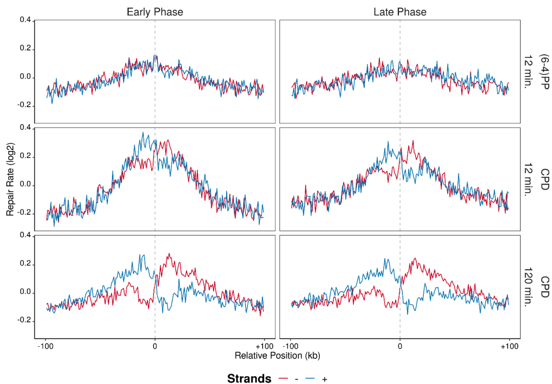
Figure 6.36 Repair rates (XR-seq/Damage-seq) are calculated and log2-transformed in 200 kb windows with 1 kb intervals, which initiation zones are positioned at the center of the region. The blue lines are the plus strands and red lines are the minus strands. Analysis is performed on replicate A.
