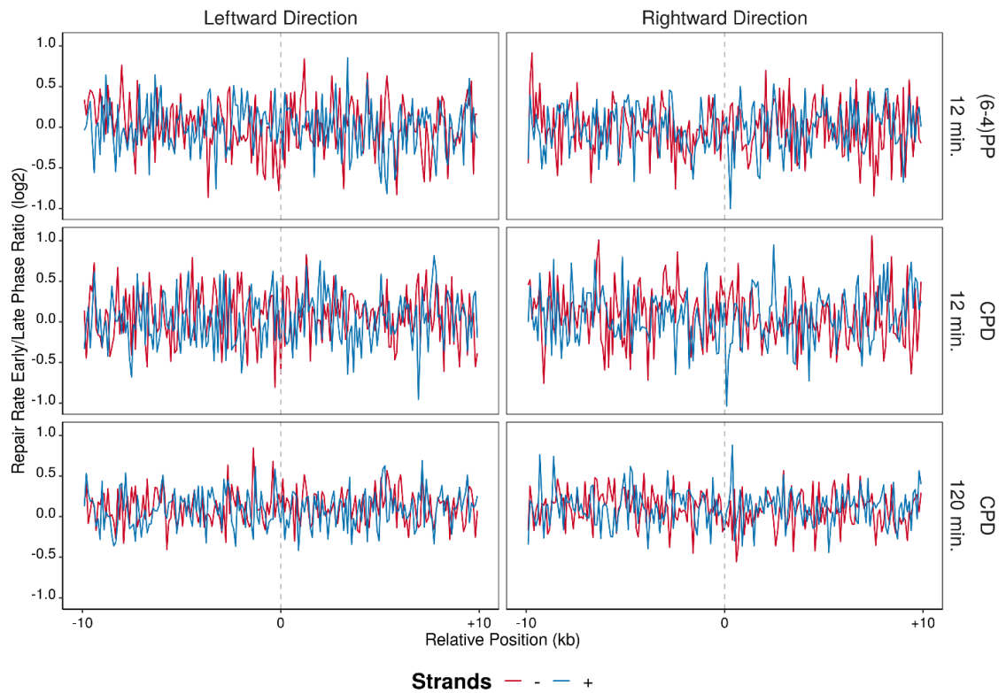
Figure 6.68 After log 2 -transformed repair rates (XR-seq/Damage-seq) of high RFD regions are calculated at both leftward and rightward directions, samples that are at early S phase of the cell cycle are further divided by the ones that are at the late S phase (early/late) in 20 kb windows with 100 base pair intervals. The blue lines are the plus strands and red lines are the minus strands. Analysis is performed on replicate A.
