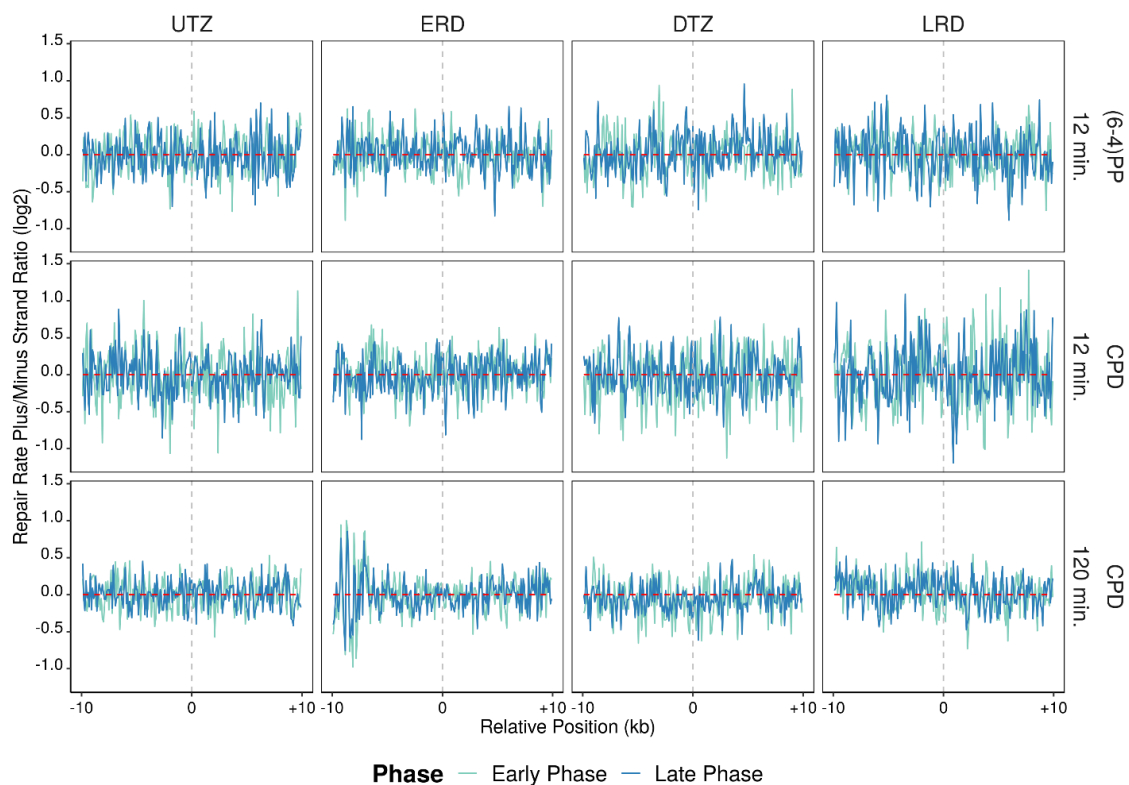
Figure 6.30 After log2-transformed repair rates (XR-seq/Damage-seq) are calculated, plus strands of the samples are further divided to minus strands (plus/minus) in 20 kb windows with 100 base pair intervals, which replication domains are positioned at the center of the region. Light blue lines are the early phase samples and dark blue lines are the late phase samples. Analysis is performed on replicate A.
