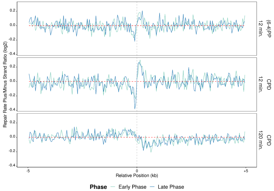
Figure 6.59 After log 2 -transformed repair rates (XR-seq/Damage-seq) are calculated, plus strands of the samples are further divided to minus strands (plus/minus) in 10 kb windows with 50 base pair intervals, which replication origins (SNS-seq) are positioned at the center of the region. Light blue lines are the early phase samples and dark blue lines are the late phase samples. Analysis is performed on replicate B.
