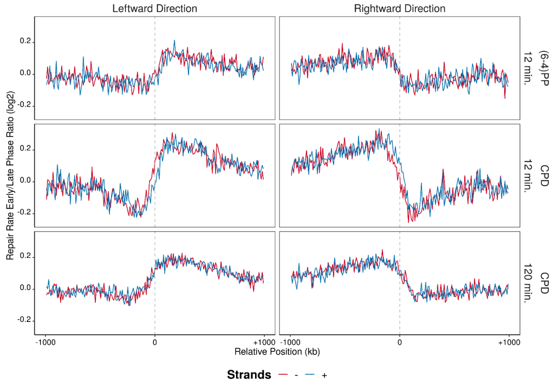
Figure 6.73 After log2-transformed repair rates (XR-seq/Damage-seq) of high RFD regions are calculated at both leftward and rightward directions, samples that are at early S phase of the cell cycle are further divided by the ones that are at the late S phase (early/late) in 2 Mb windows with 10 kb intervals. The blue lines are the plus strands and red lines are the minus strands. Analysis is performed on replicate B.
