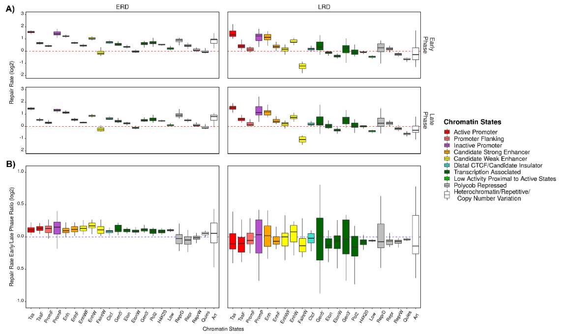
Figure 6.14 The effect of Chromatin States on repair efficiency of the replication domains. A) Repair rates (XR-seq/Damage-seq) of (6-4)PP samples at 12 minutes are calculated, log2-transformed, B) and for every region, the repair rates at early S phase divided by repair rates at late S phase to layout the skewness of the repair rate to a phase of replication. The analysis is performed on replicate B.
