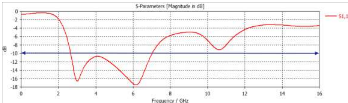
Figure 3.6: The S_{11} for the Primary M-MSA Design.
