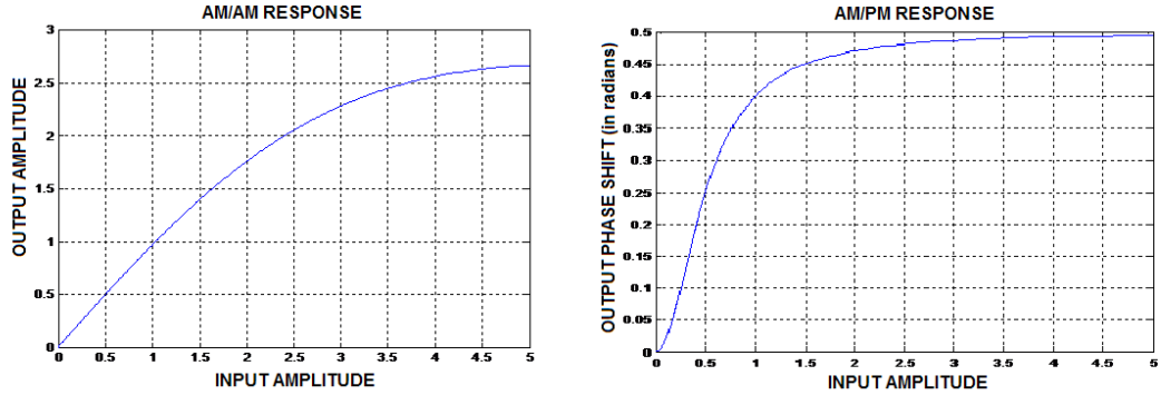
Figure 4.3: AM/AM and AM/PM characteristics of a Saleh Model
