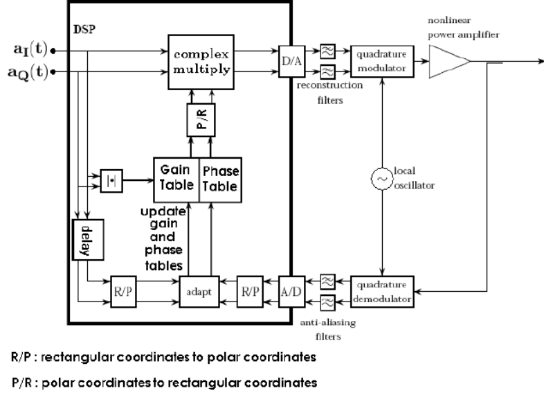
Figure 2.18: Polar Predistorter
