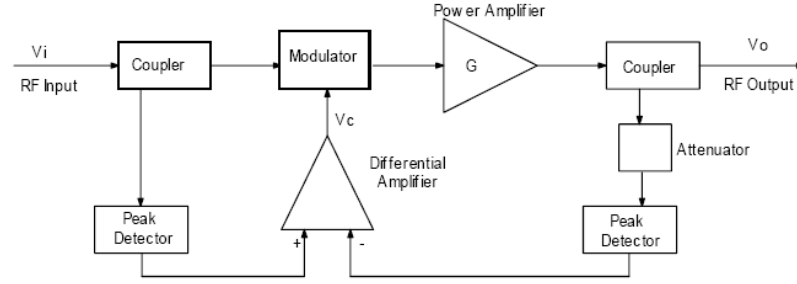
Figure 2.3: Envelope Feedback to Linearize Power Amplifier [1]
