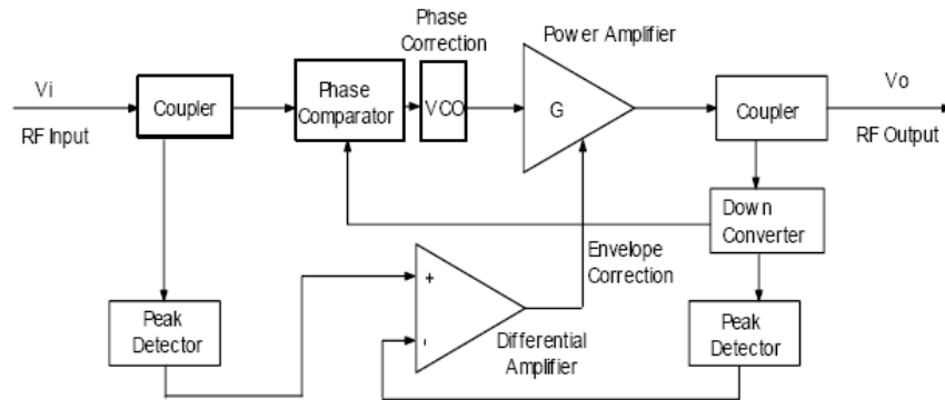
Figure 2.4: Polar Feedback to Linearize Power Amplifier [20]
