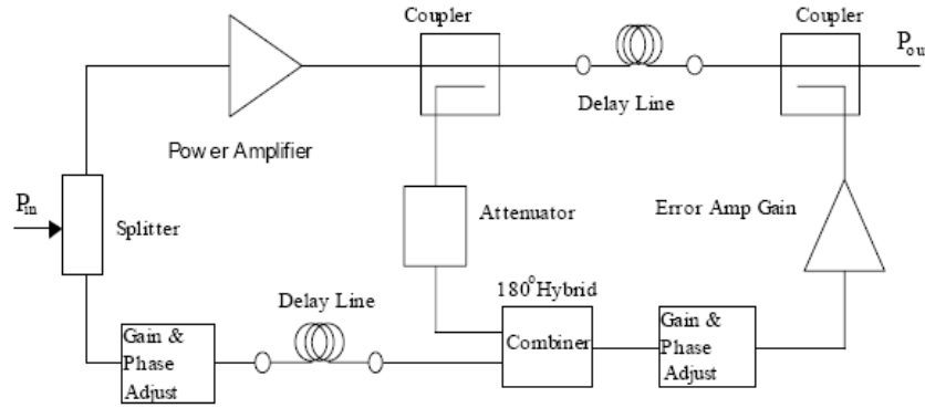
Figure 2.6: Feedforward Technique to Linearize Power Amplifier [12]
