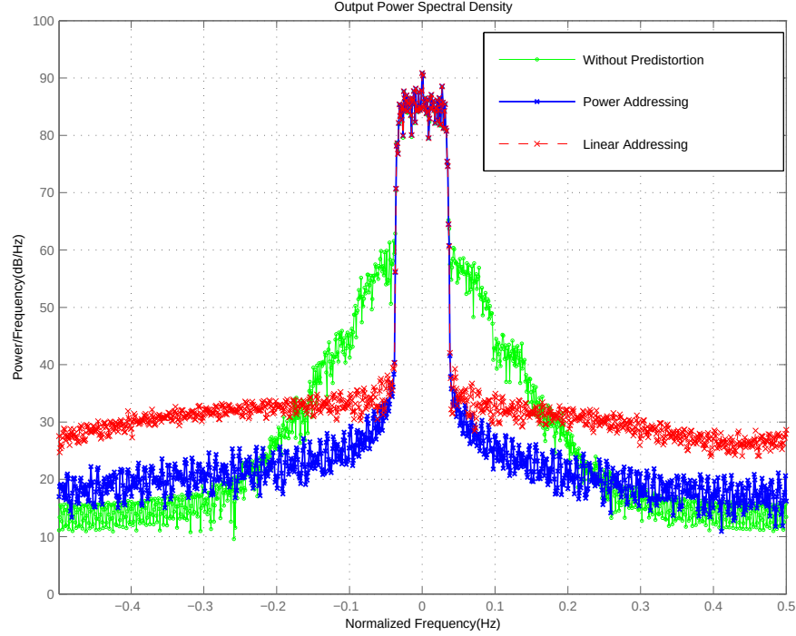
Figure 5.2: Sensitivity to Table Addressing
