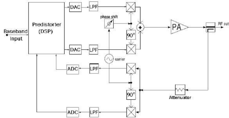
Figure 2.13: Adaptive Digital Baseband Predistortion [14]
