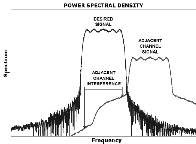
Figure 3.4: Adjacent Channel Interference
