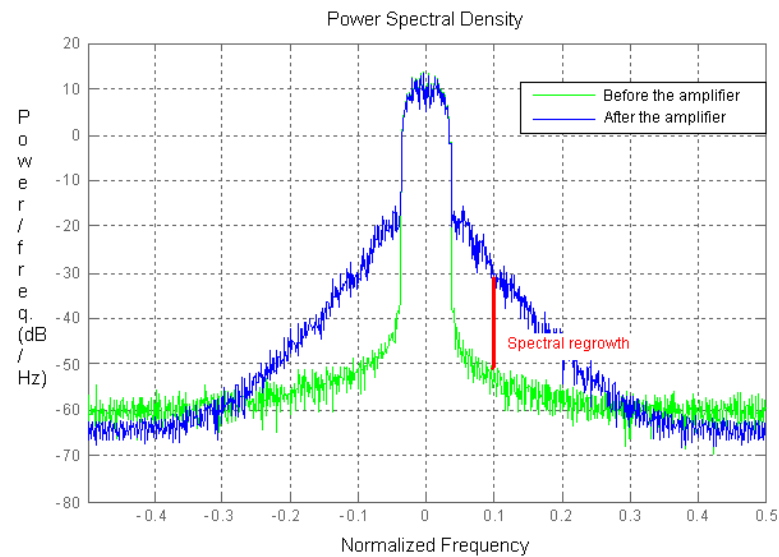
Figure 3.3: Spectral Regrowth
