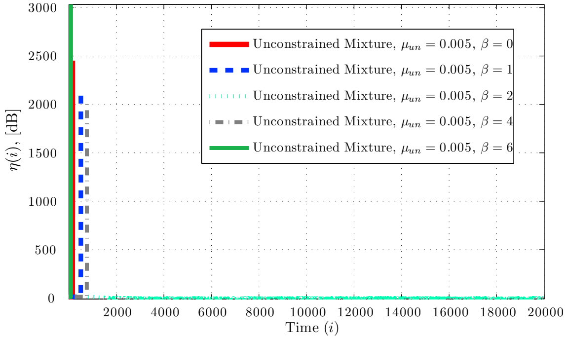
Figure 4.20: Example 2: Evolution of global mean-square deviation (MSD) (3.29) for adaptive diffusion LMS with unconstrained mixture combiner function with constant \mu_{un} = 0.005 .
