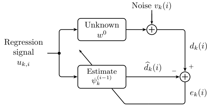
Figure 2.1: Block-diagram of the adaptive filtering procedure.
