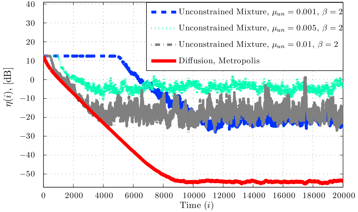
Figure 4.19: Example 2: Evolution of global mean-square deviation (MSD) (3.29) for adaptive diffusion LMS with unconstrained mixture combiner function with constant \beta = 2 .
