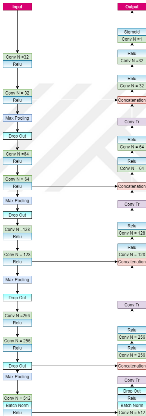
Figure 4.4: Bilnet1
