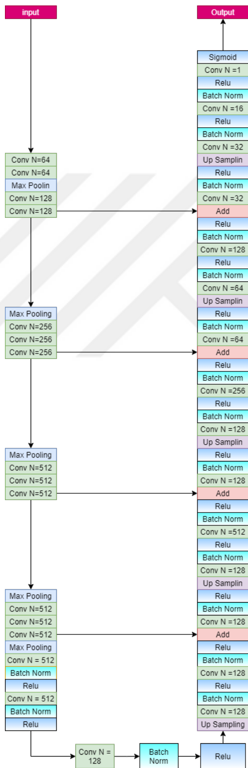
Figure 4.3: Original U-Net
