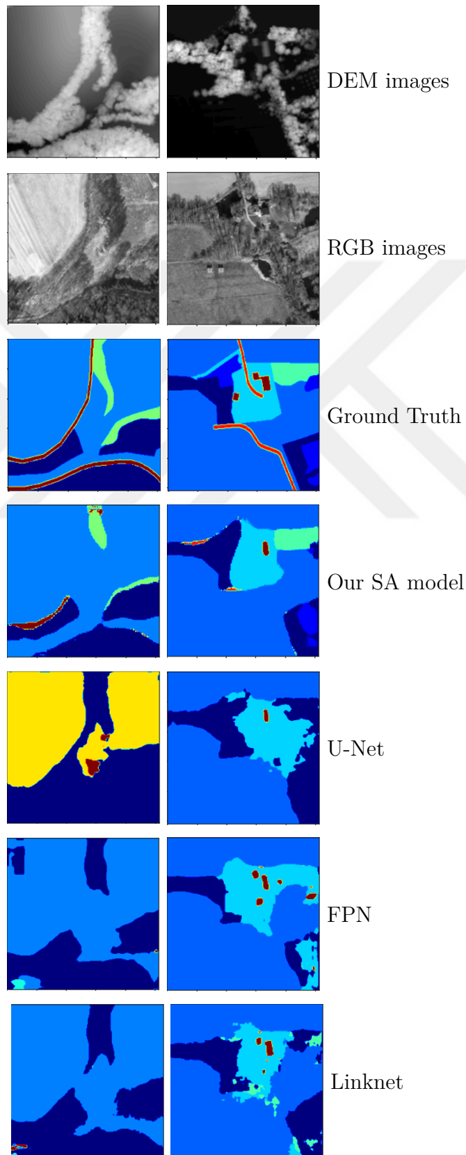
Figure 5.10: Comparison qualitative results in GeoNRW dataset
