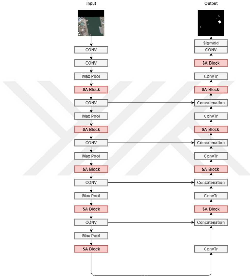
(a) Architecture of our model
