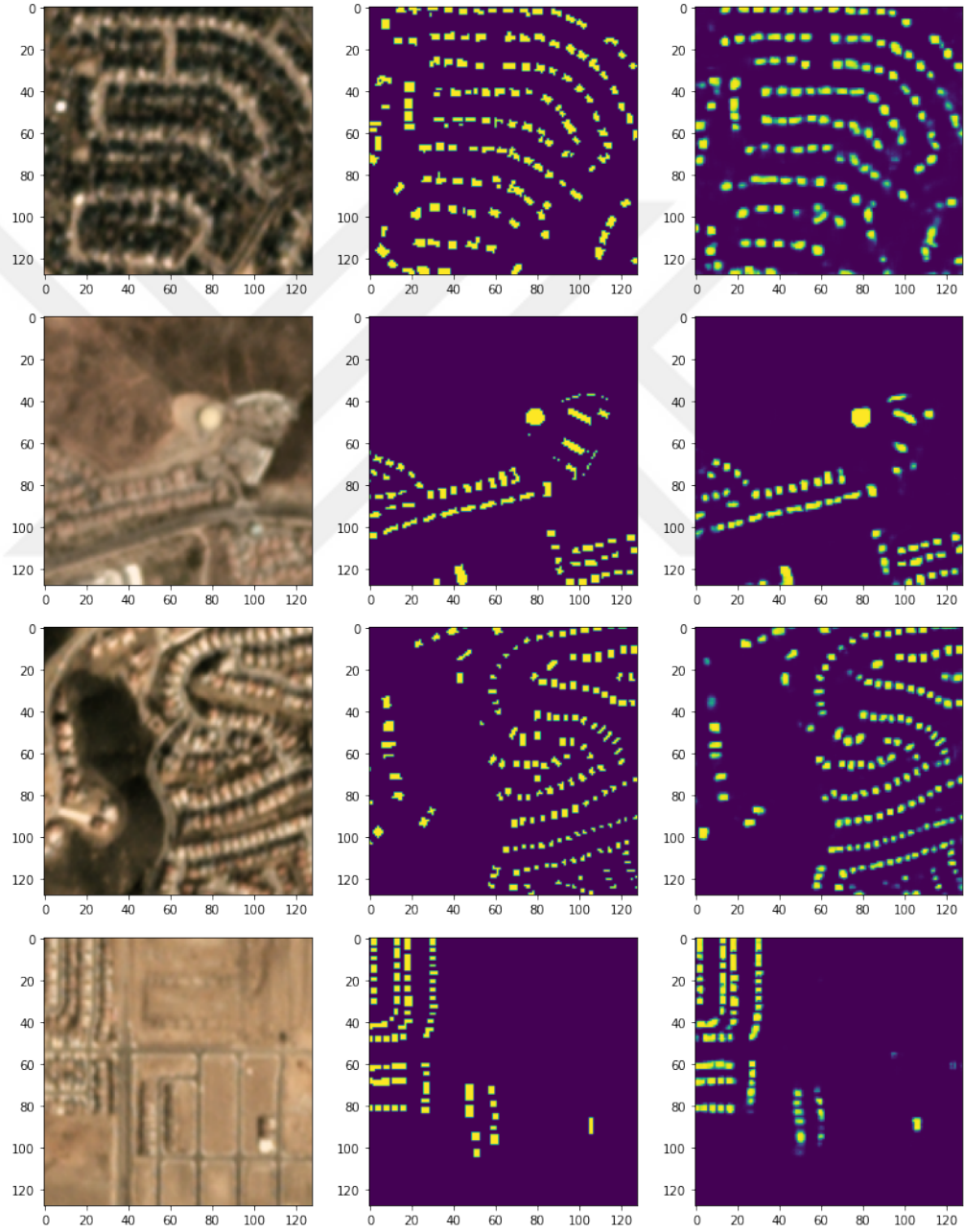
Figure 5.8: Prediction of proposed model On SpaceNet7
