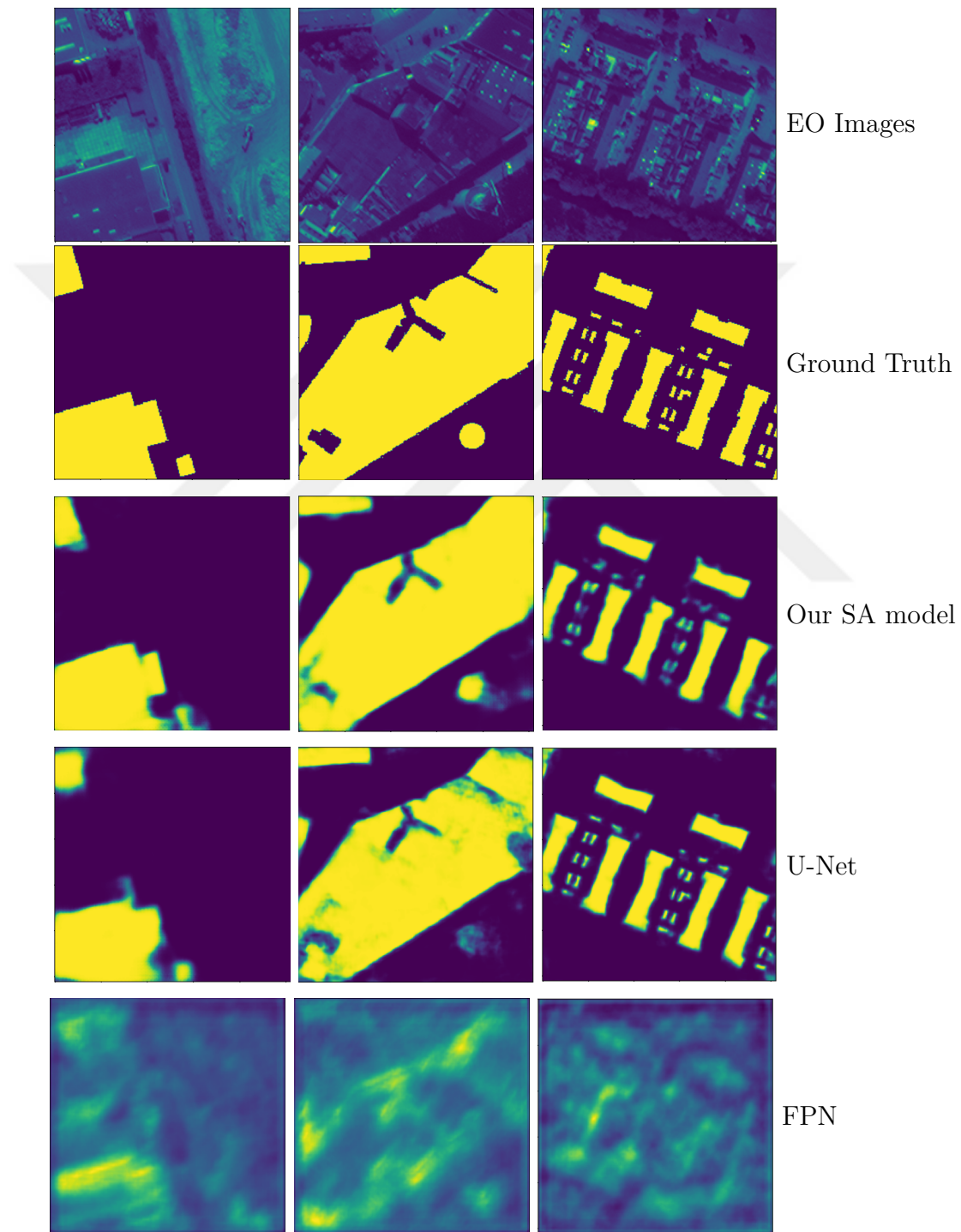
Figure 5.7: Prediction of proposed model vs U-Net model with EO images
