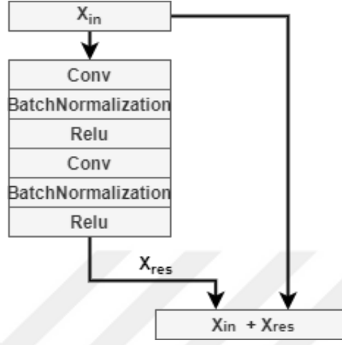
(a) Residual Block
