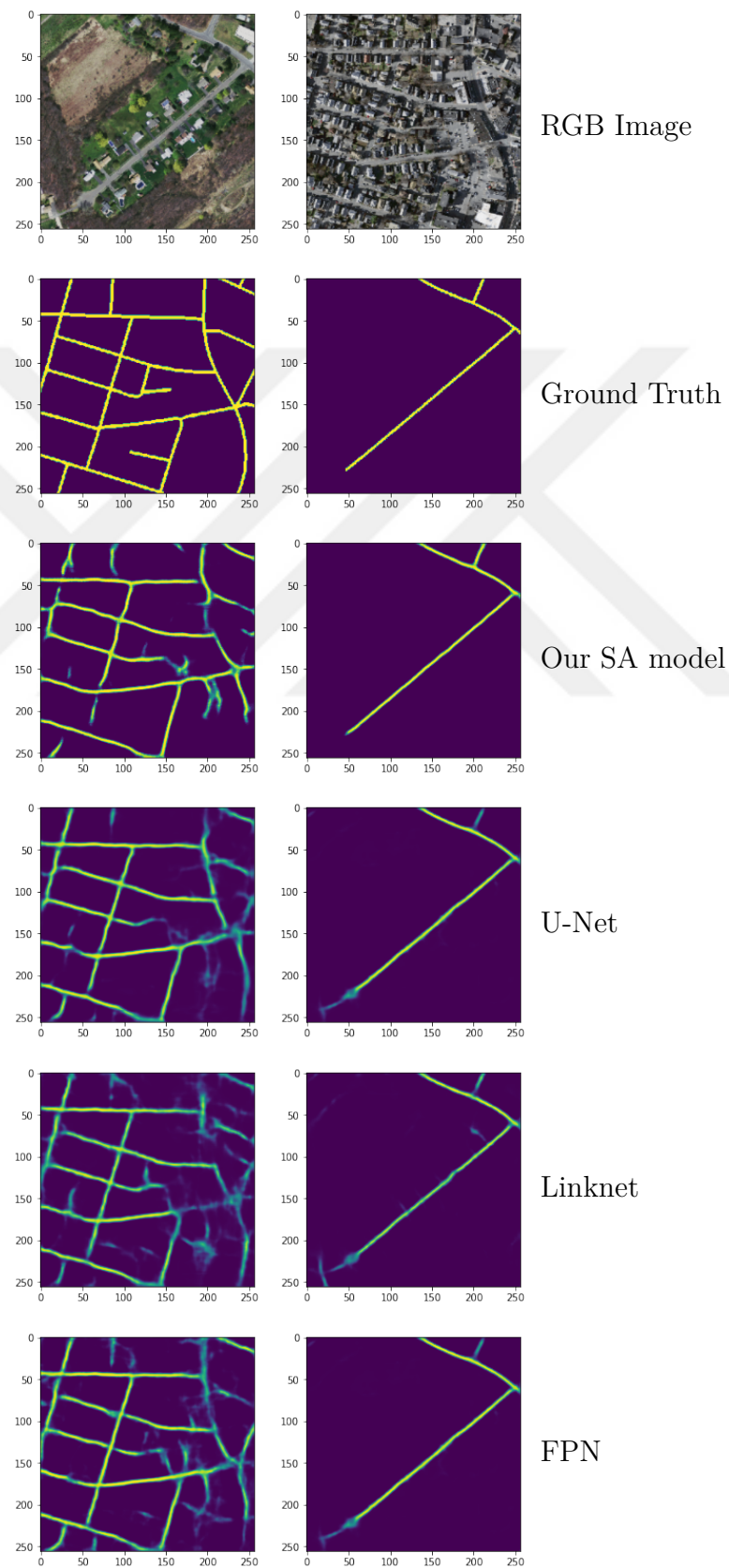
Figure 5.9: Comparison qualitative results in Massachusetts dataset
