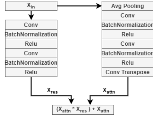
(c) Squeeze-and-attention(SA)
