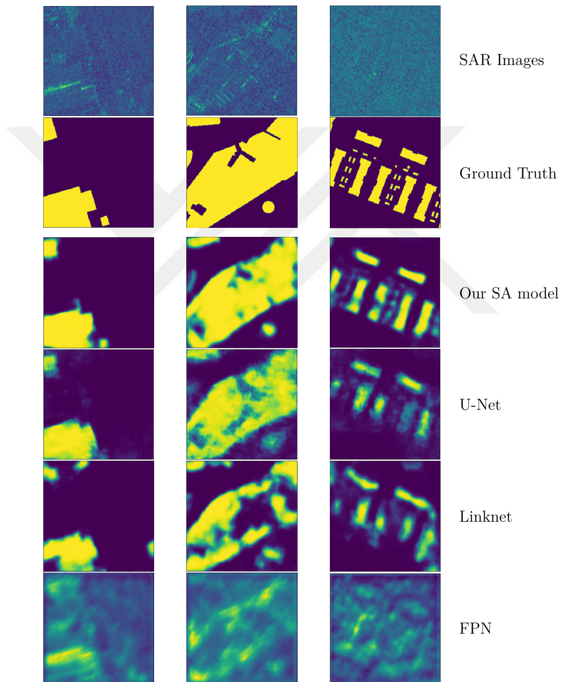
Figure 5.6: Comparative analysis of predicted samples from various networks.
