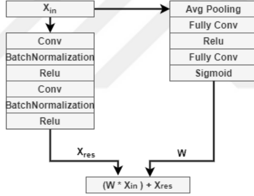
(b) Squeeze-and-excitation(SE)
