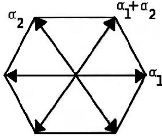
Figure 2.2: A Picture of \Delta for \Sigma_3
