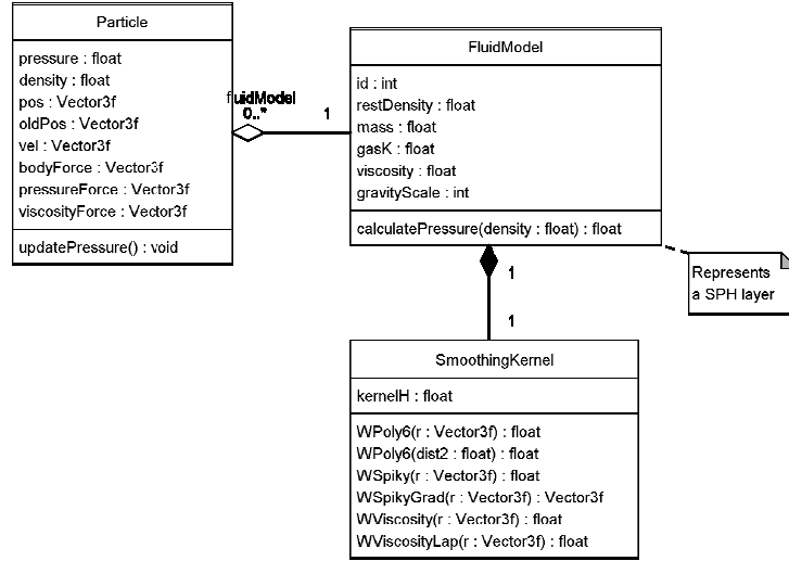
Figure A.1.1: The Particle model
