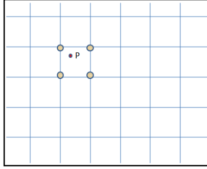
Figure 3.1: Grid approximation
