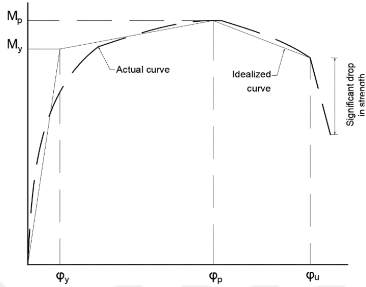
Figure 4.4. Actual versus idealized monotonic moment-curvature relationship
