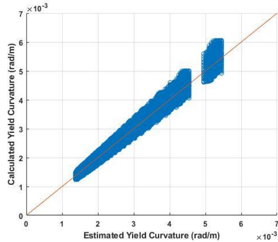
Figure 4.15. Effective yield curvature goodness of fit scatter plot for rectangular sections.
