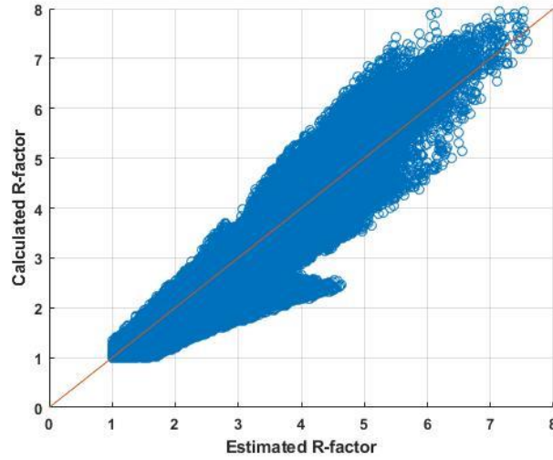
Figure 5.10. R-factor goodness of fit scatter plot for rectangular piers of pinned tip in the short direction.
