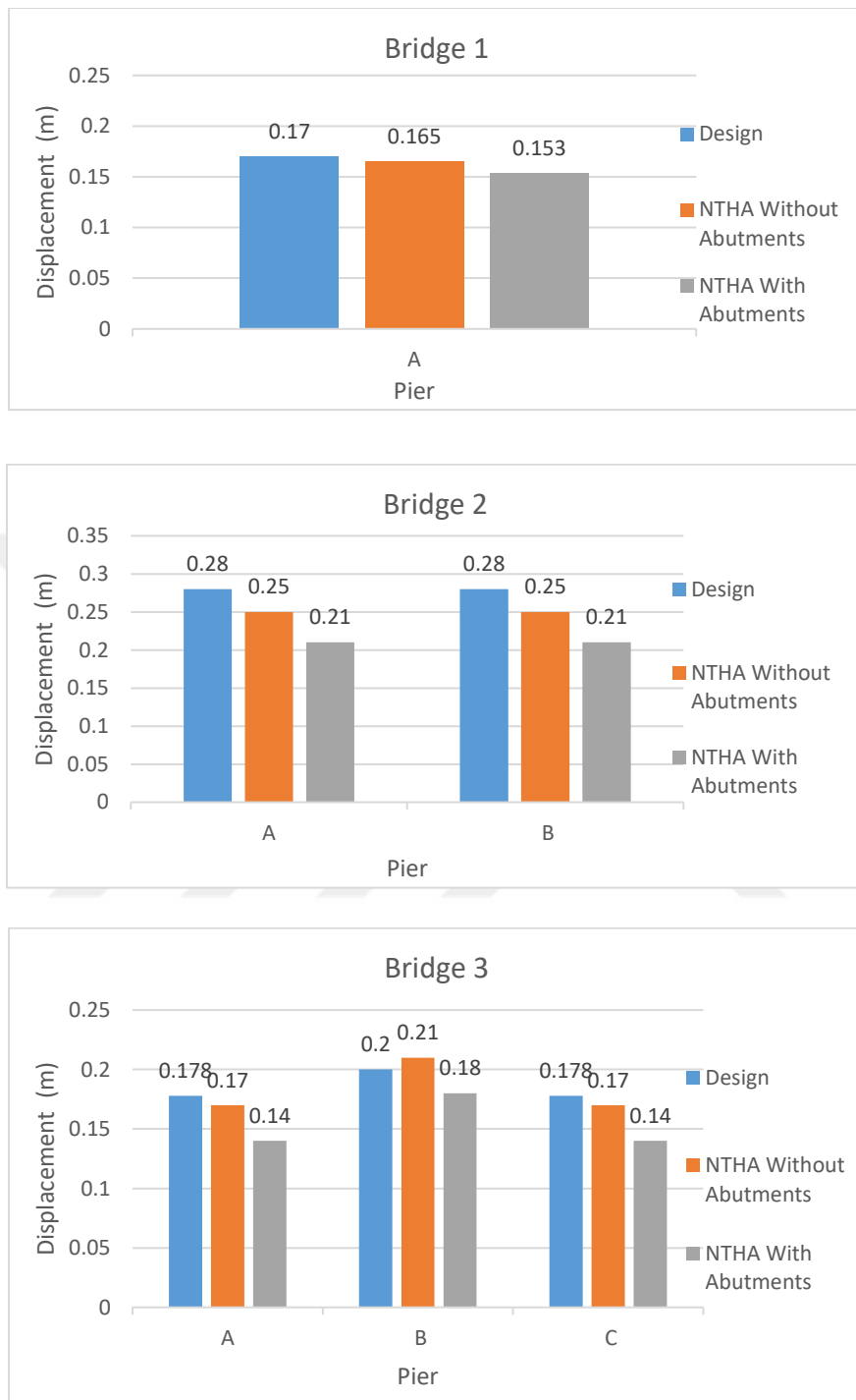
Figure 6.8. Comparison between design tip displacements and averaged tip displacements of piers from NTHA corresponding to the upper-performance level in longitudinal direction.
