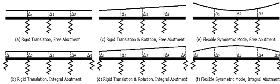
Figure 6.2. Plan views of possible inelastic displacement patterns for continuous bridges [38].
