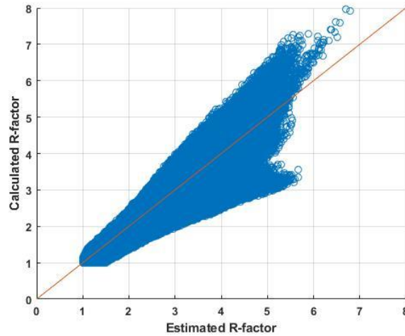
Figure 5.18. R-factor goodness of fit scatter plot for rectangular piers of fixed tip in the long direction.
