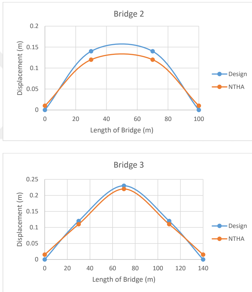
Figure 6.7. Comparison between design tip displacements and averaged tip displacements of piers from NTHA corresponding to the upper performance level in transverse direction.
