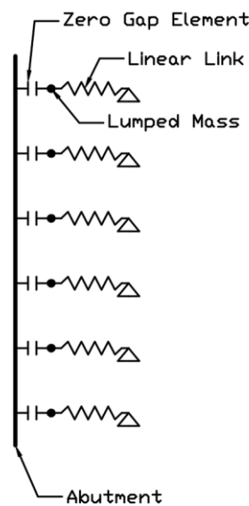
Figure 6.6. Modeling of backfill soil-structure interaction.
