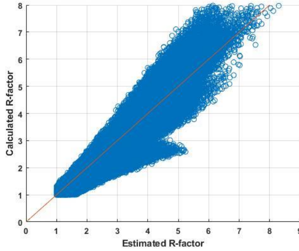
Figure 5.4. R-factor goodness of fit scatter plot for circular piers of pinned tip.
