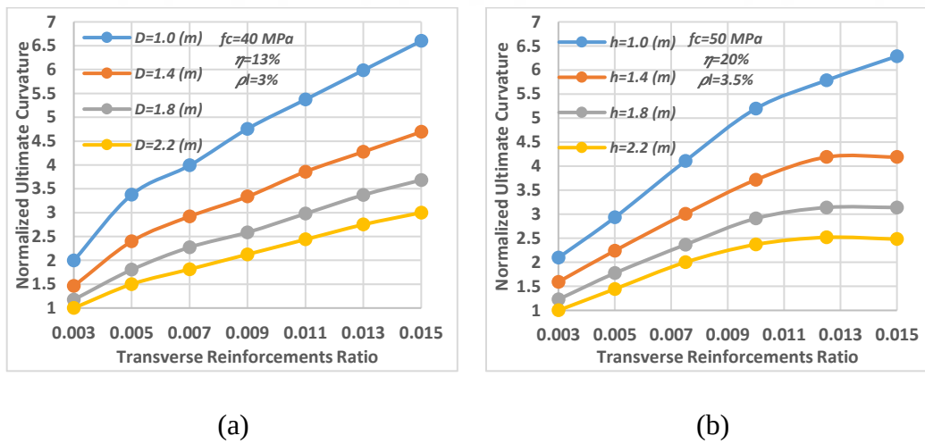
Figure 4.9. Effects of transverse reinforcements on ultimate curvature. (a) Circular sections, (b) Rectangular sections.
