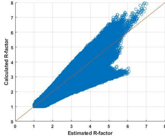
Figure 5.12. R-factor goodness of fit scatter plot for rectangular piers of fixed tip in the short direction.
