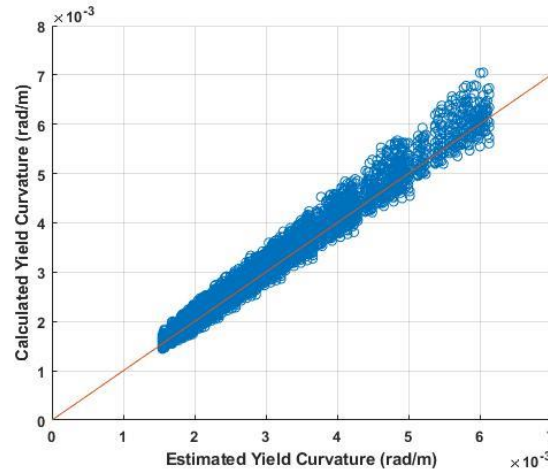
Figure 4.13. Effective yield curvature goodness of fit scatter plot for circular sections.
