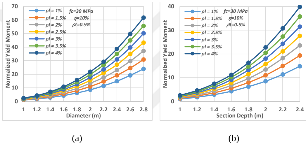
Figure 4.10. Effects of section diameter/depth and longitudinal reinforcements on yield moment. (a) Circular sections, (b) Rectangular sections.
