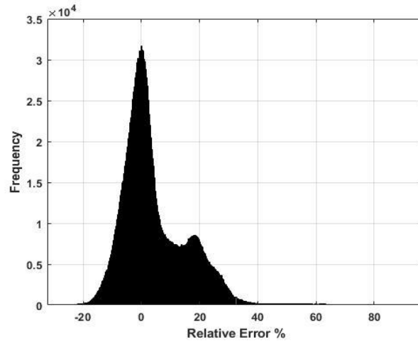
Figure 5.11. Relative error distribution of the estimated R-factor values for rectangular piers of pinned tip in the short direction.
