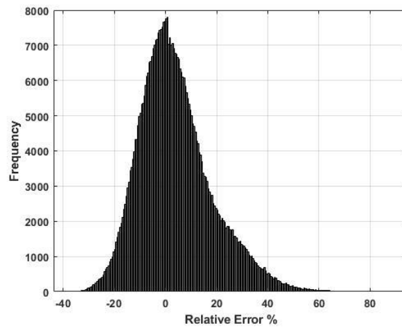
Figure 5.9. Relative error distribution of the estimated R-factor values for circular piers of elastomeric bearing connected tip.
