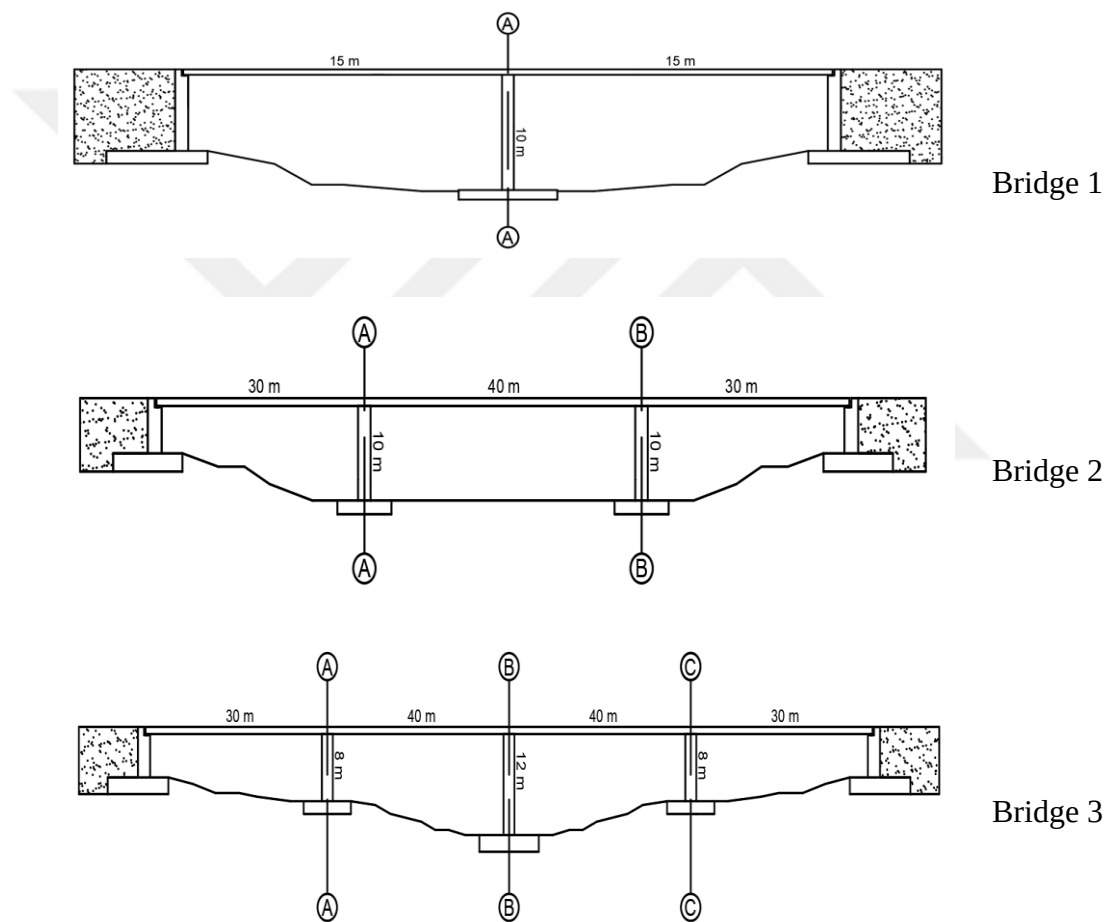
Figure 6.3. Design examples of continuous bridge structures.
