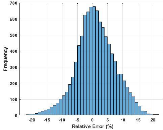
Figure 4.22. Relative error distribution of the estimated yield moment values for circular sections.
