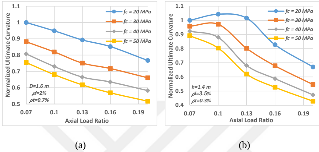
Figure 4.8. Effects of axial load and characteristic strength of concrete on ultimate curvature. (a) Circular sections, (b) Rectangular sections.
