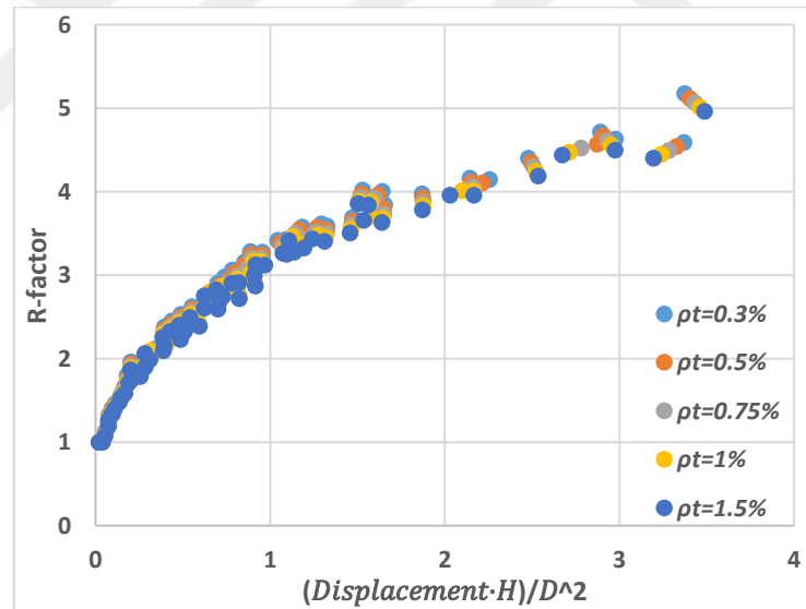
Figure 5.3. Effect of transverse reinforcements on R-factor.
