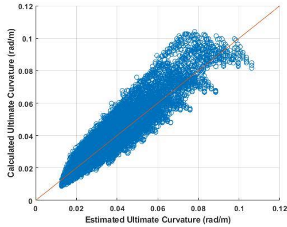
Figure 4.17. Ultimate curvature goodness of fit scatter plot for circular sections.
