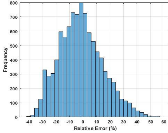
Figure 4.18. Relative error distribution of the estimated ultimate curvature values for circular sections.
