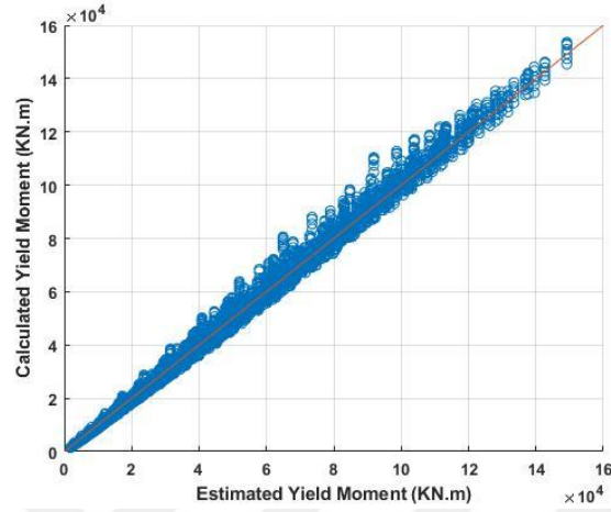
Figure 4.21. Yield moment capacity goodness of fit scatter plot for circular sections.
