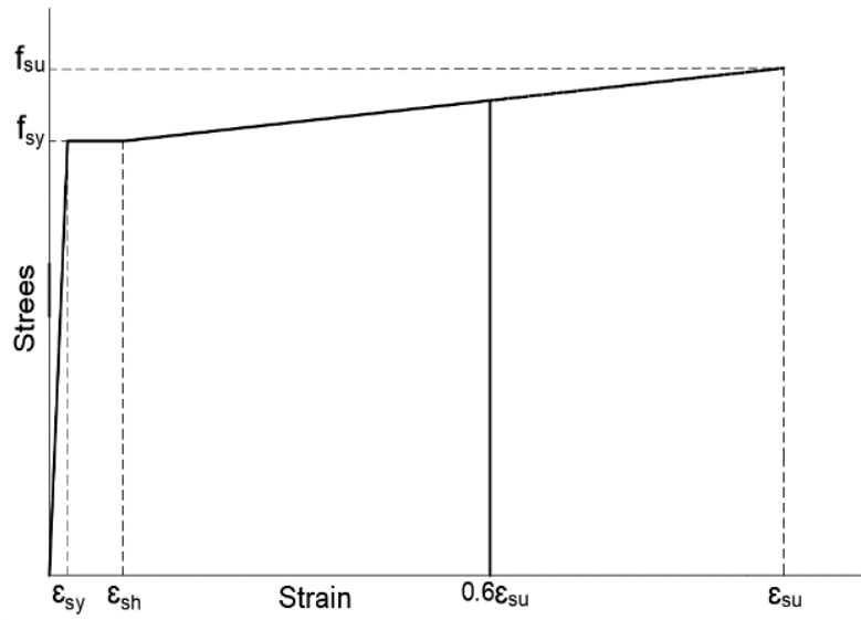
Figure 4.3. Stress-strain relationship of reinforcing steel.
