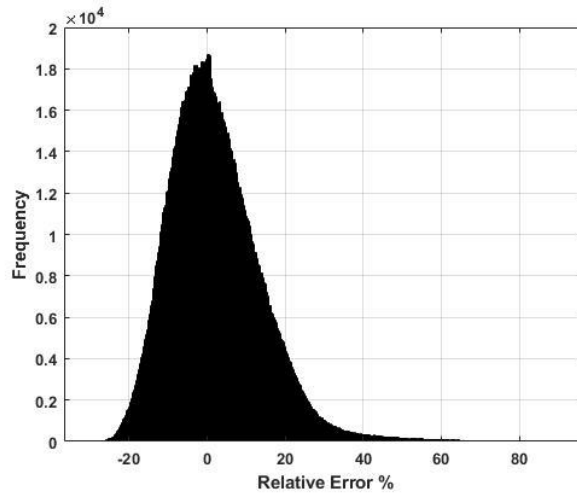
Figure 5.15. Relative error distribution of the estimated R-factor values for rectangular piers of elastomeric bearing connected tip in the short direction.
