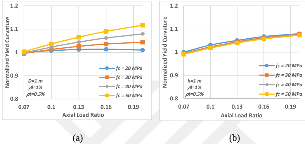
Figure 4.6. Effects of axial load and characteristic strength of concrete on the normalized effective yield curvature. (a) Circular sections, (b) Rectangular sections.
