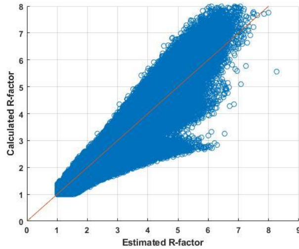
Figure 5.6. R-factor goodness of fit scatter plot for circular piers of fixed tip.
