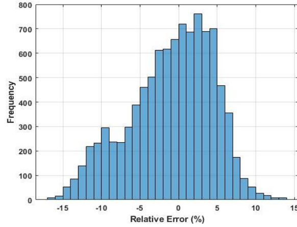
Figure 4.14. Relative error distribution of the estimated effective yield curvature values for circular sections.
