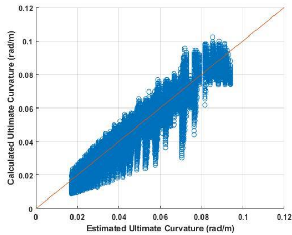
Figure 4.19. Ultimate curvature goodness of fit scatter plot for rectangular sections.
