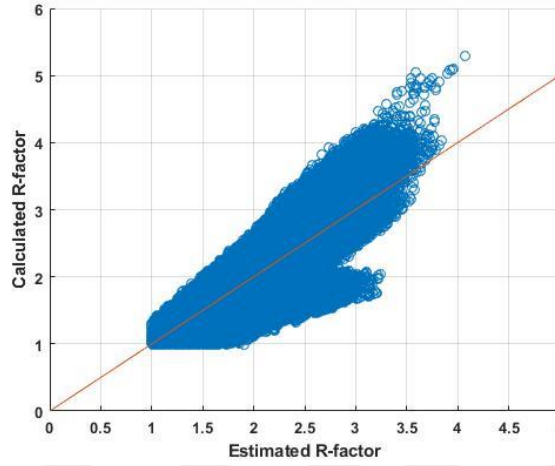
Figure 5.14. R-factor goodness of fit scatter plot for rectangular piers of elastomeric bearing connected tip in the short direction.
