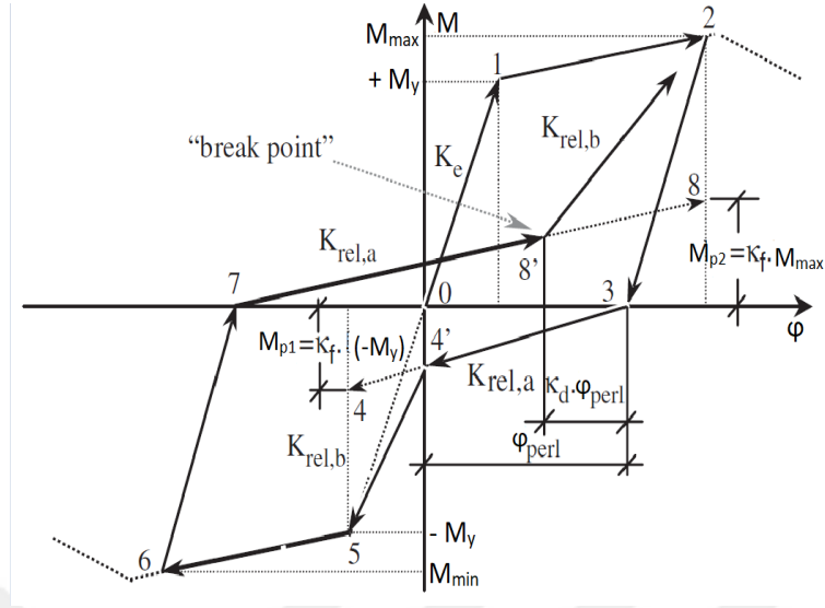
Figure 5.2. IMK pinching hysteretic model.
