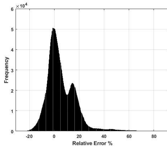
Figure 5.13. Relative error distribution of the estimated R-factor values for rectangular piers of fixed tip in the short direction.
