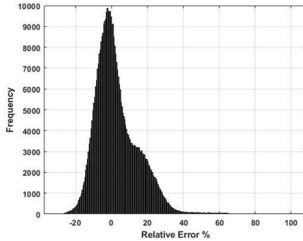
Figure 5.5. Relative error distribution of the estimated R-factor values for circular piers of pinned tip.
