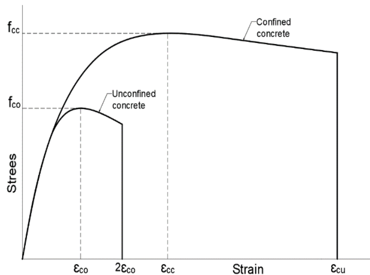
Figure 4.2. Stress-strain relationship of confined and unconfined concrete.
