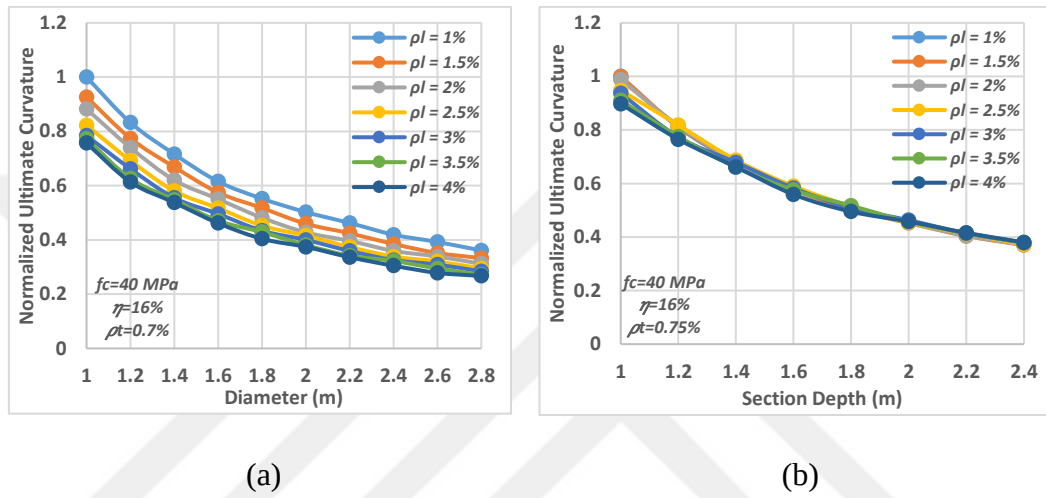
Figure 4.7. Effects of section diameter/depth and longitudinal reinforcements on the normalized ultimate curvature. (a) Circular sections, (b) Rectangular sections.
