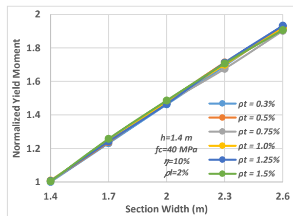
Figure 4.12. Section width versus normalized yield moment of rectangular sections for various transverse reinforcements ratios.
