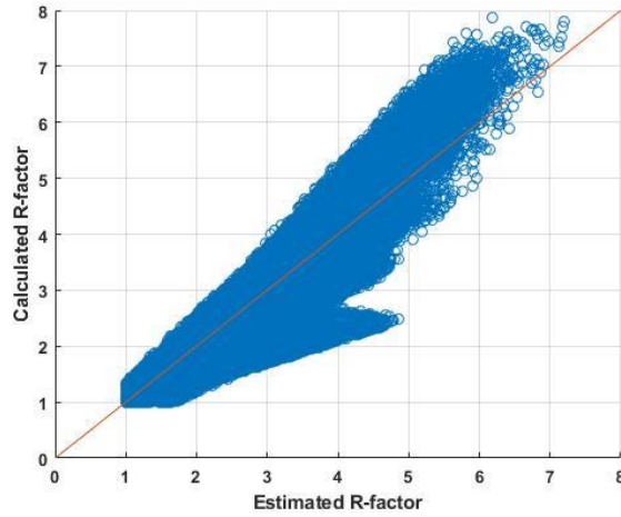
Figure 5.16. R-factor goodness of fit scatter plot for rectangular piers of pinned tip in the long direction.
