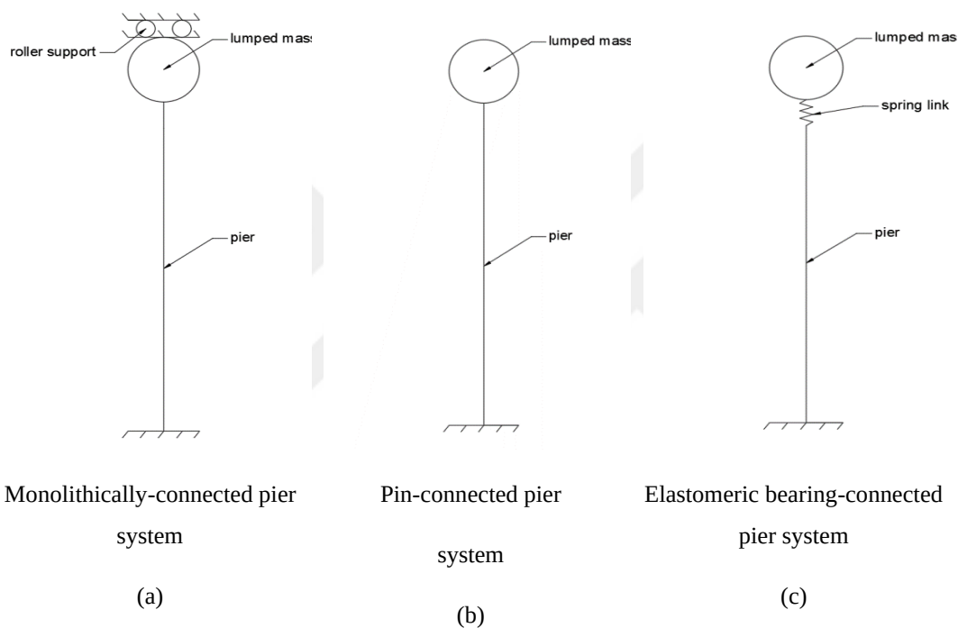
Figure 5.1. SDOF systems of piers
