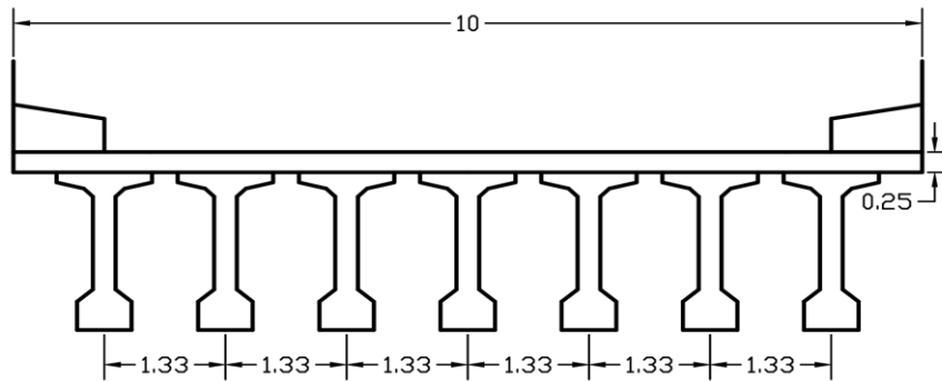
Figure 6.4. Cross-section of superstructure.
