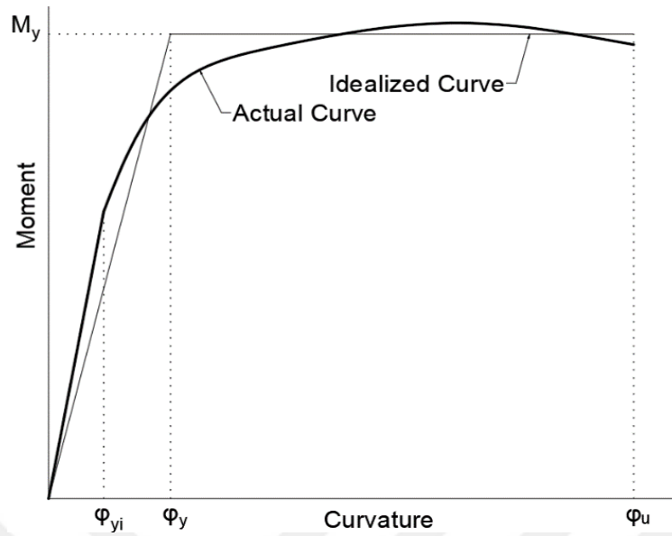
Figure 4.1. Actual versus idealized monolithic moment-curvature relationship.
