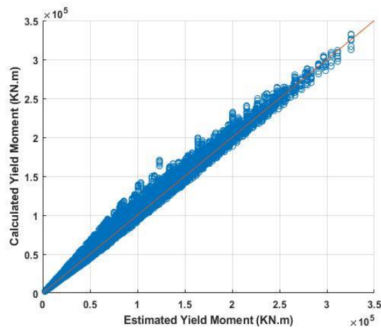
Figure 4.23. Yield moment capacity goodness of fit scatter plot for rectangular sections.
