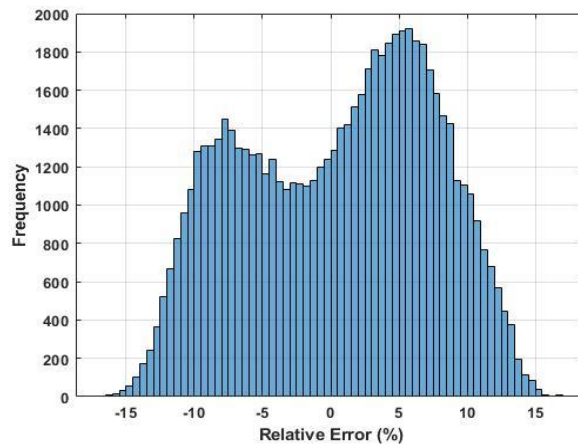
Figure 4.16. Relative error distribution of the estimated effective yield curvature values for rectangular sections.
