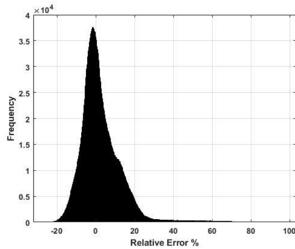
Figure 5.17. Relative error distribution of the estimated R-factor values for rectangular piers of pinned tip in the long direction.
