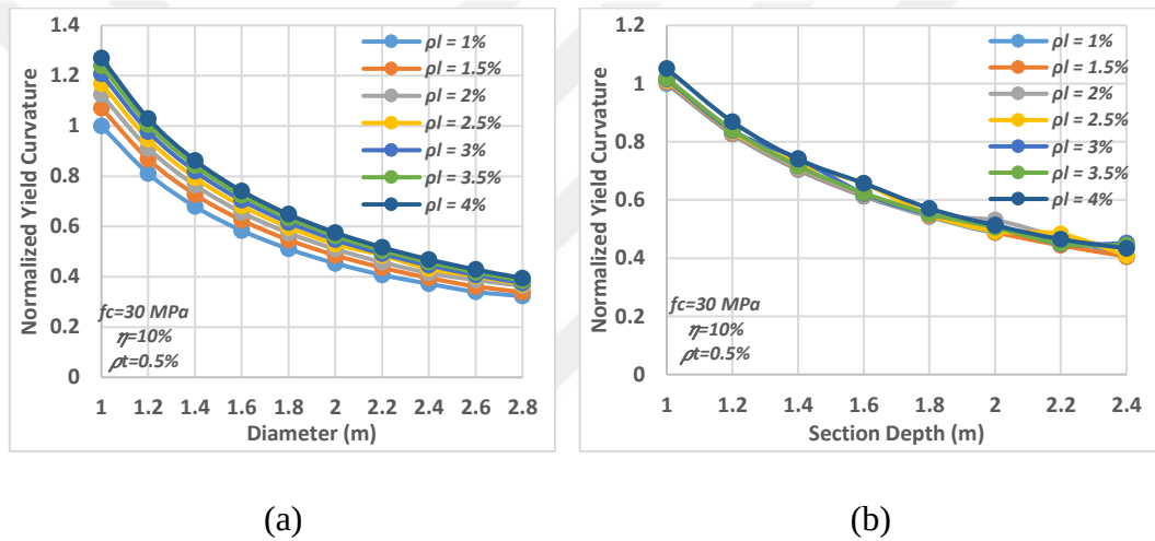
Figure 4.5. Effects of section diameter/depth and longitudinal reinforcements on the normalized effective yield curvature. (a) Circular sections, (b) Rectangular sections.
