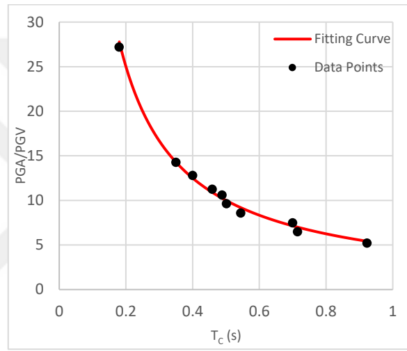
Figure 3.2. The second corner periods T_c of the smoothed response spectra versus the average PGA/PGV ratios of the ground motions groups, fitting curve of the plotted points.
