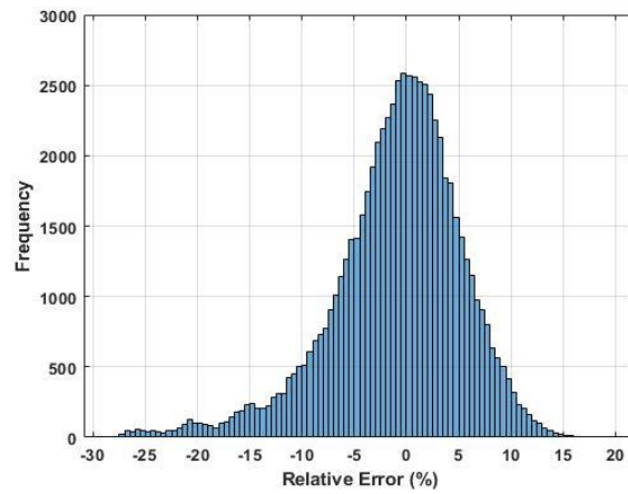
Figure 4.24. Relative error distribution of the estimated yield moment values for rectangular sections.
