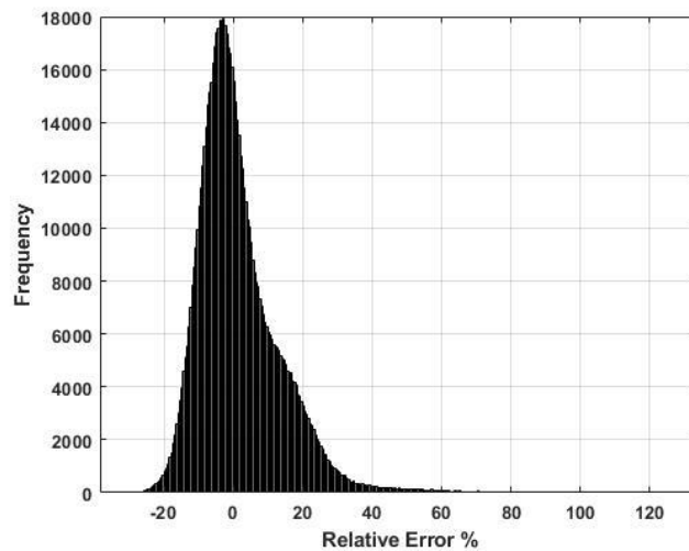
Figure 5.7. Relative error distribution of the estimated R-factor values for circular piers of fixed tip.
