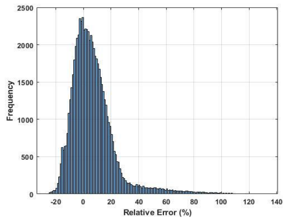
Figure 4.20. Relative error distribution of the estimated ultimate curvature values for rectangular sections.
