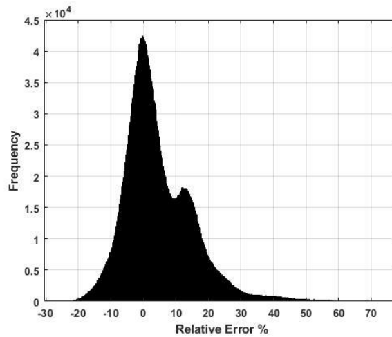
Figure 5.19. Relative error distribution of the estimated R-factor values for rectangular piers of fixed tip in the long direction.
