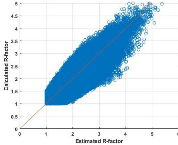
Figure 5.8. R-factor goodness of fit scatter plot for circular piers of elastomeric bearing connected tip.
