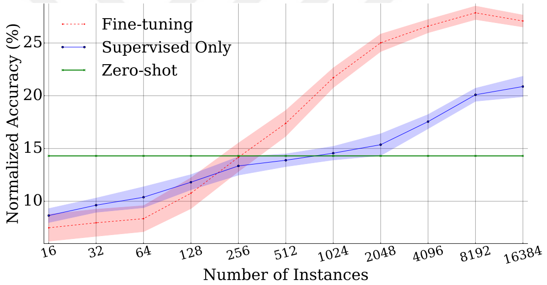
Figure 4.4: Performance comparison of the proposed framework with fine-tuning and supervised-only methods on zero-shot test classes. Fine-tuning and supervised-only results are derived at different points when the number of instances is increasing. The x -axis is shown in log-scale.
