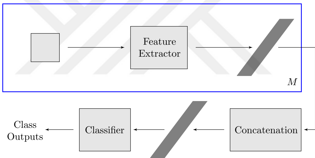
Figure 5.1: Basic multisource model. Feature-level fusion vector of multiple images acquired from M different sources is used for class identification. Note that plate notation is used for the illustration of different image source domains.
