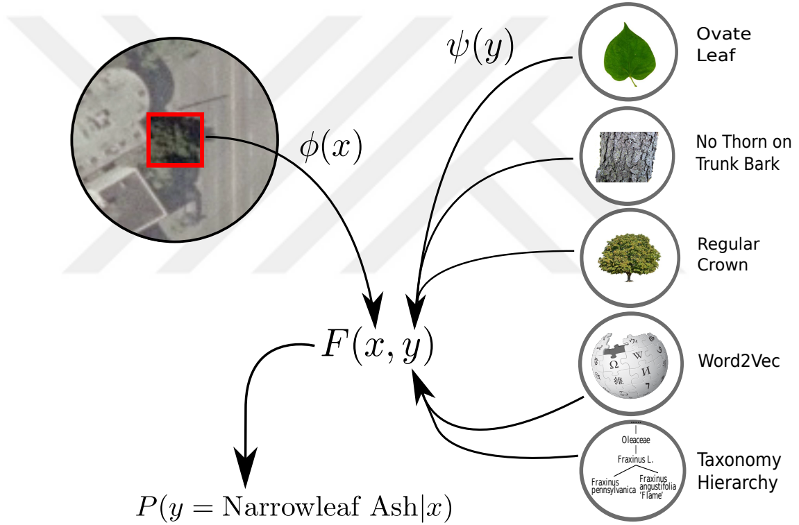
Figure 4.1: Our proposed framework learns the compatibility function F(x, y) between image embedding \phi(x) and class embeddings \psi(y) based on attributes, word-embeddings from a natural language model, and a hierarchical scientific taxonomy. The learned compatibility function is then used in recognizing instances of unseen classes by leveraging their class embedding vectors.
