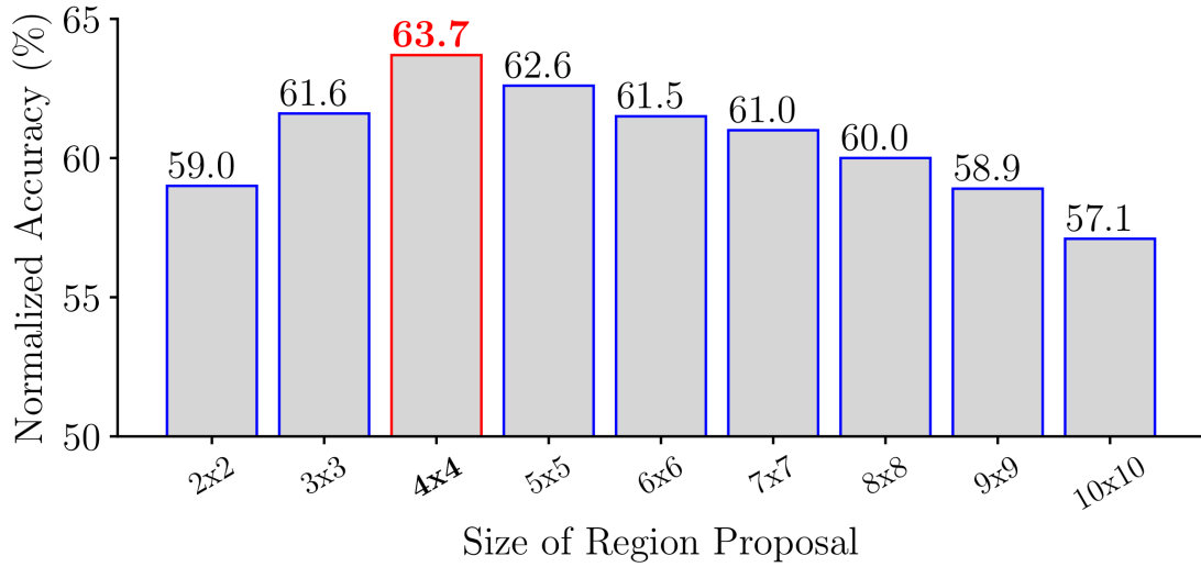
Figure 5.4: Effect of region proposal size on classification performance. The y-axis is shown in the range of [50 - 65] when the size of region proposal is increasing from 2 \times 2 to 10 \times 10 .
