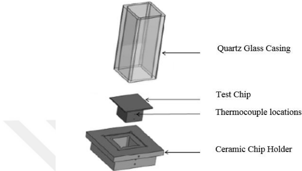
Figure 5.3. The copper test section with the ceramic chip holder assembly
