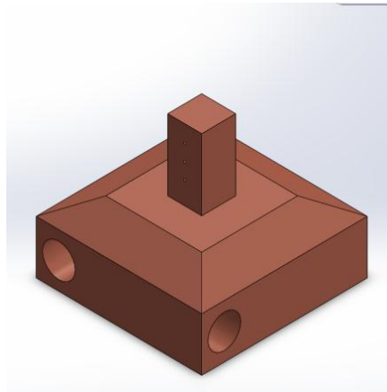
Figure 5.2. Heater block
