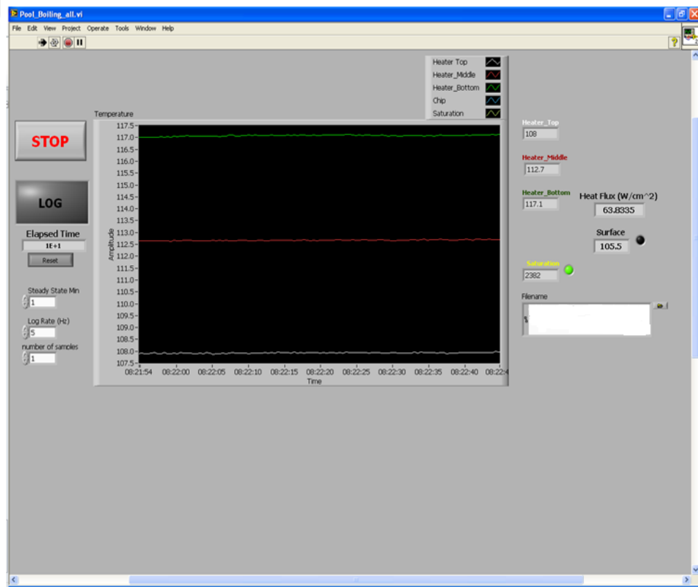
Figure 5.17. LabVIEW virtual instrument
