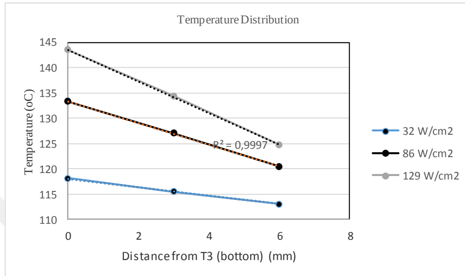
Figure 5.20. Heat loss study showing variation of temperature over the distance for a plain chip
