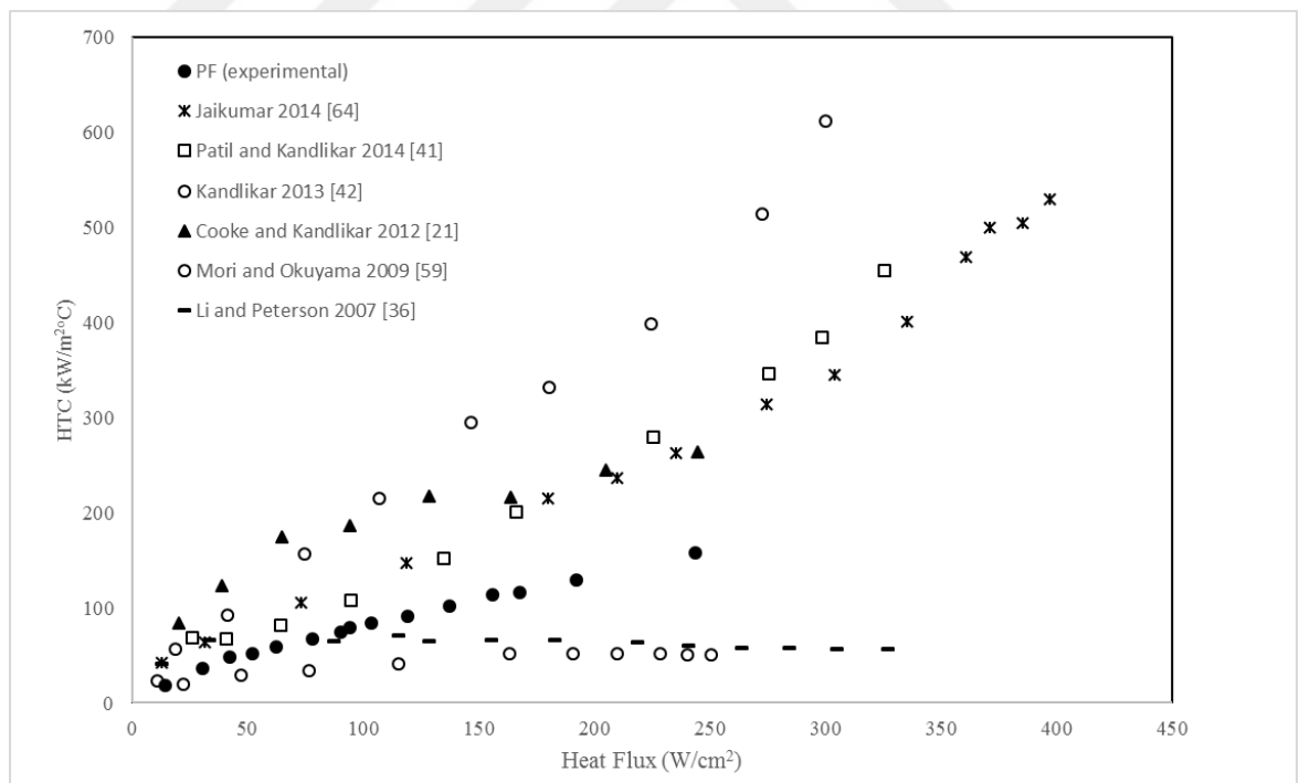
Figure 6.18. Comparison of best performing chip with other enhancements available in the literature [21,36,41, 42,59,64]
