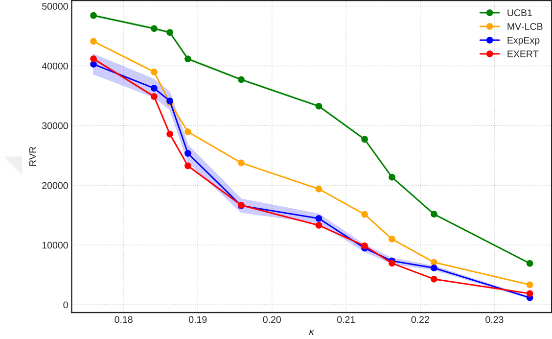
Figure 4.4: The RVR as a function of \kappa for \rho = 0.2 .
