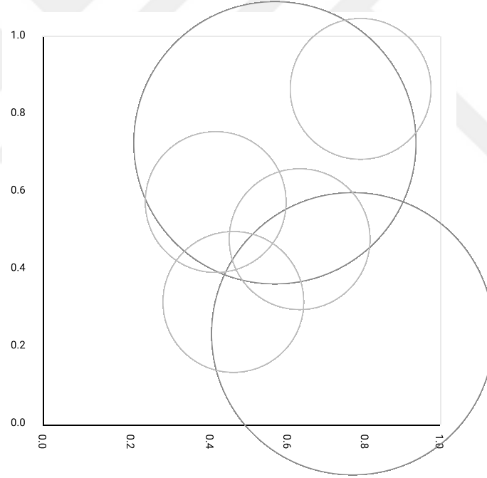
Figure 3.1: A Possible Cover of the 2-Dimensional Context Space 4
