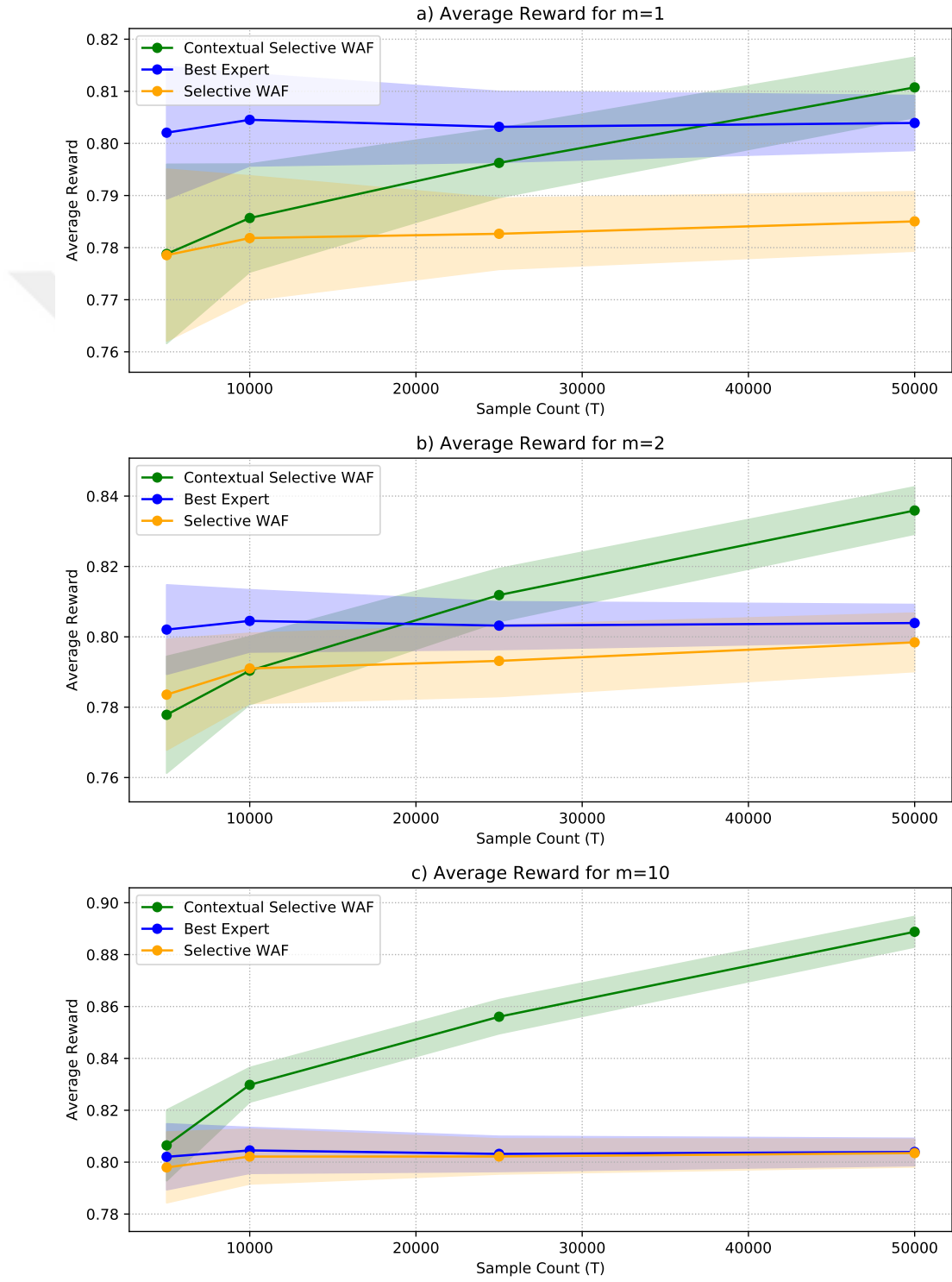
Figure 3.4: The average reward as a function of T for CinC Dataset
