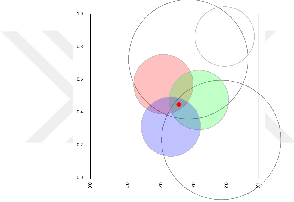
Figure 3.2: An Example of Relevant Balls in Contextual Zooming
