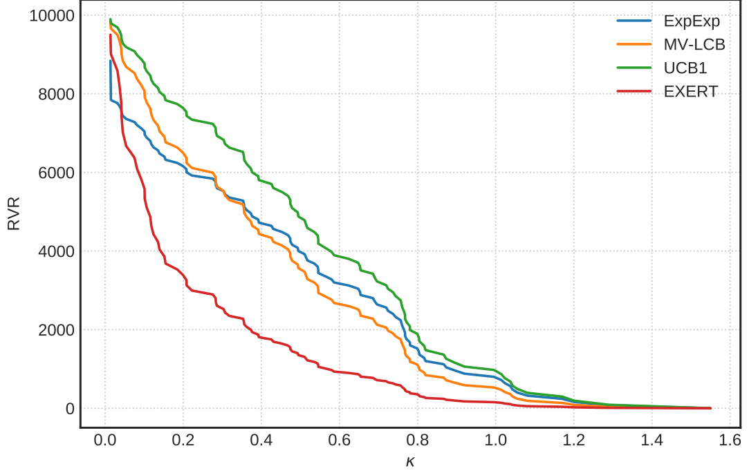
Figure 4.2: RVR at T = 10000 for different \kappa values for the variance minimization problem.
