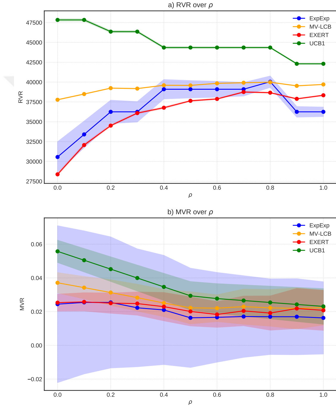
Figure 4.3: The RVR and MVR as a function of \rho .
