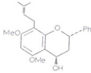
tephrowatsonin A
