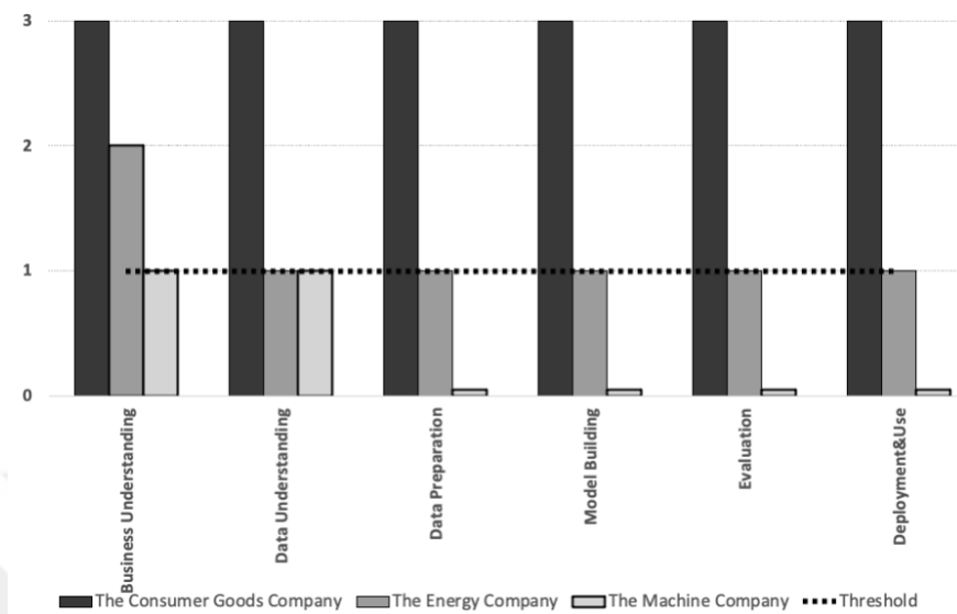
Figure 5-2. ML - 1 Assessment
