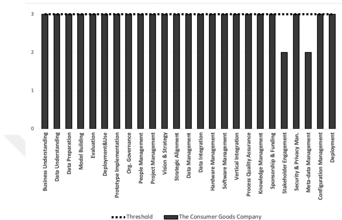
Figure 5-4. ML - 3 Assessment
