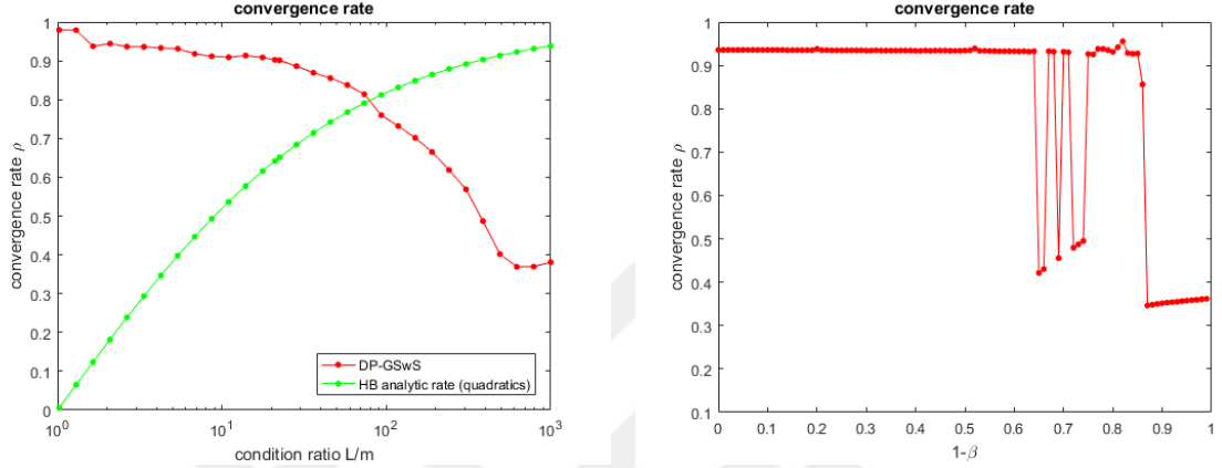
Figure 4.1: Convergence Rate for different \kappa values
