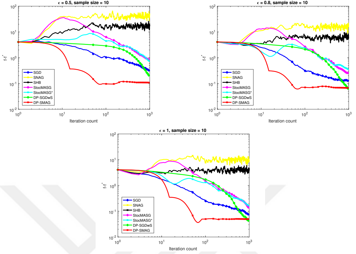
Figure 4.17: Comparison of Stochastic Algorithms For Sample Size = 10
