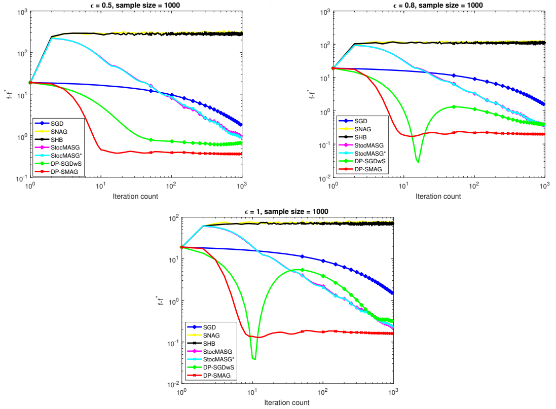
Figure 4.24: Comparison of Stochastic Algorithms For Sample Size = 1000 on MNIST
