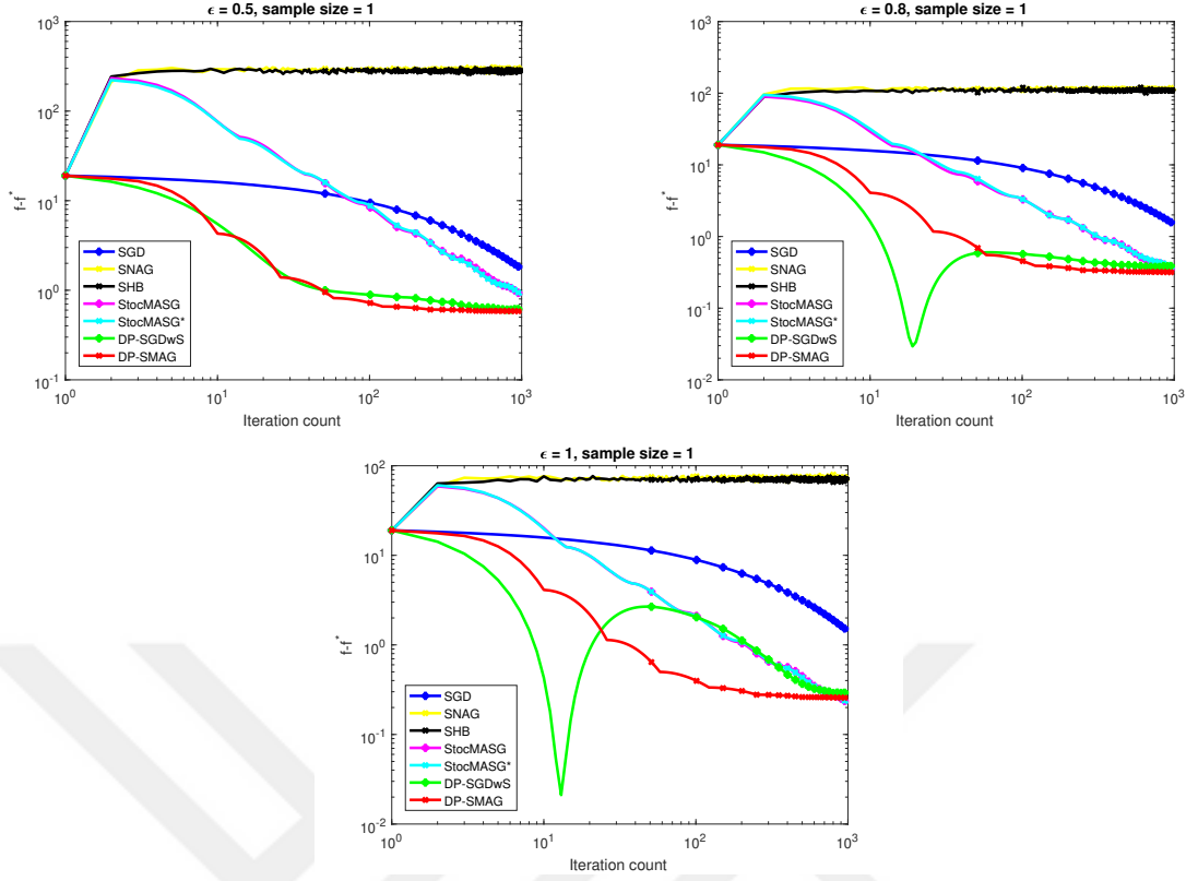
Figure 4.21: Comparison of Stochastic Algorithms For Sample Size = 1 on MNIST
