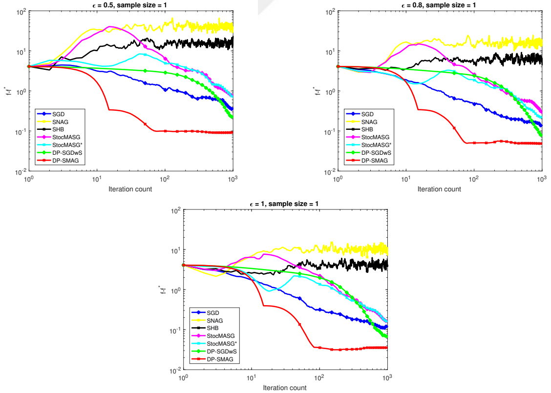
Figure 4.16: Comparison of Stochastic Algorithms For Sample Size = 1
