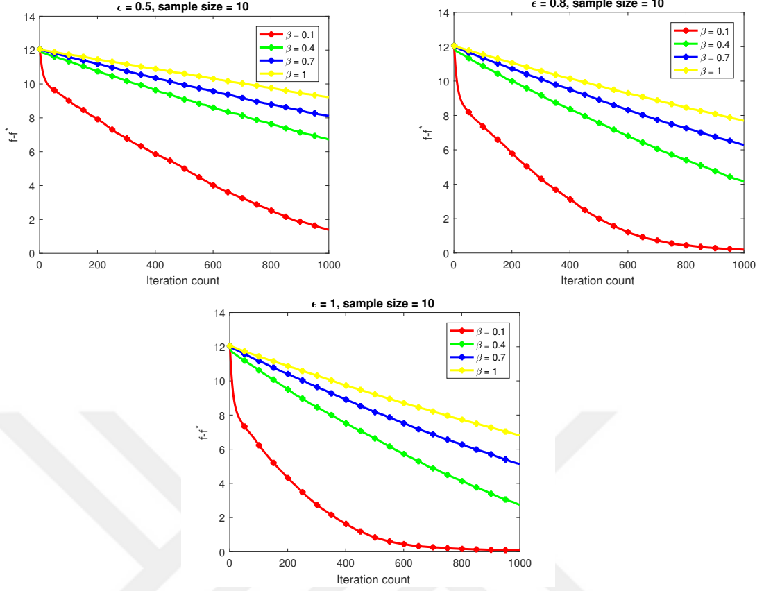
Figure 4.9: DP-SGDwS Results for Sample Size = 10
