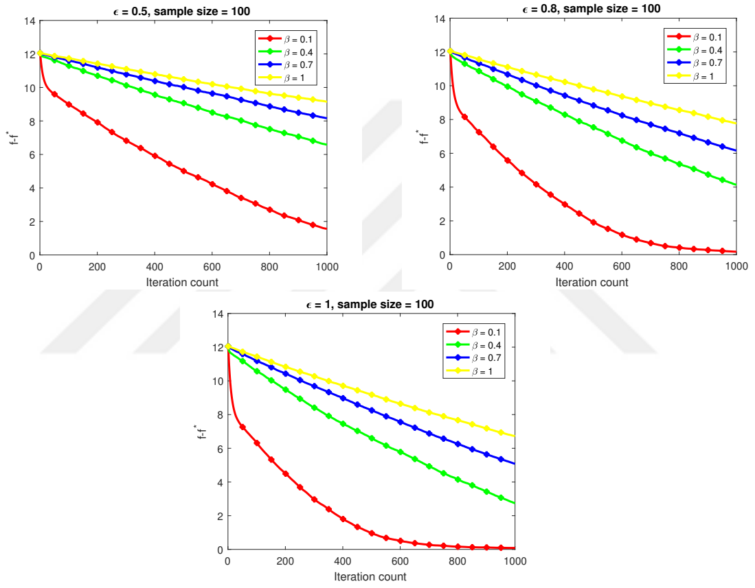
Figure 4.10: DP-SGDwS Results for Sample Size = 100
