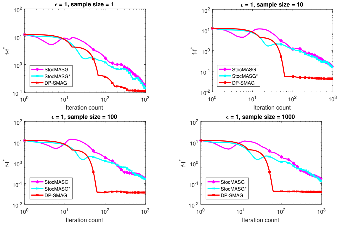
Figure 4.14: Advantage of DP-SMAG For Epsilon = 1
