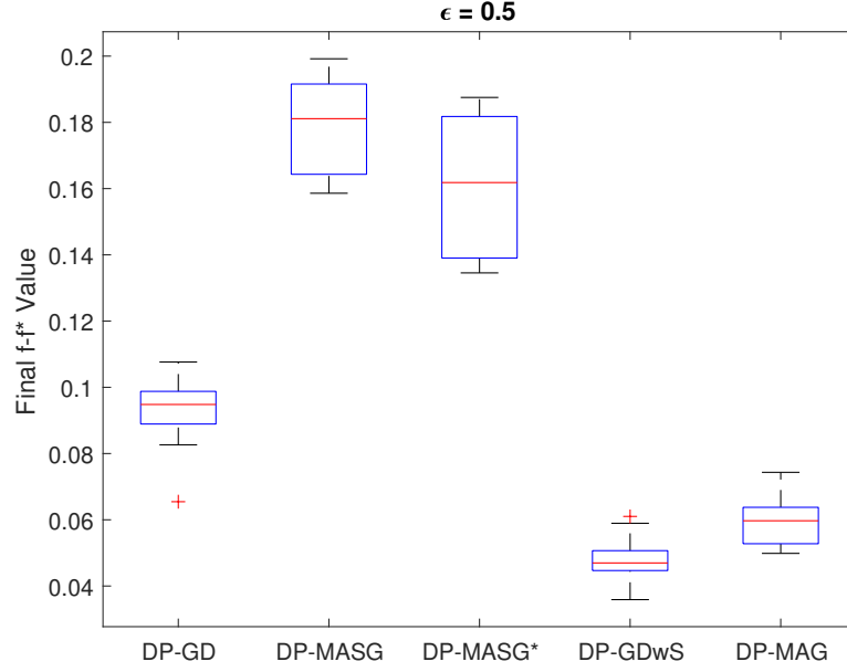
Figure 4.7: Deterministic DP - Comparisons for Different Datasets
