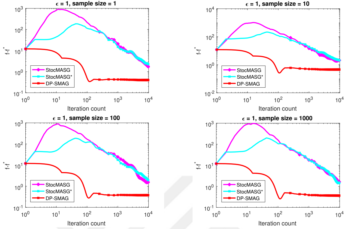
Figure 4.15: Advantage of DP-SMAG For 10^4 Iterations
