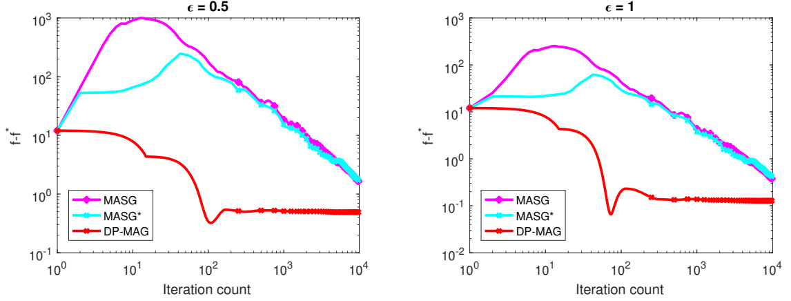
Figure 4.5: Advantage of DP-MAG for 10^4 iterations
