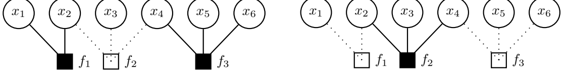
Figure 3.1: Incremental optimization of a partially separable objective by two proxy objectives f_1(x) + f_3(x) and f_2(x) . At each step, we pick a subset of functions and ignore the remainings. The black and white squares represent the chosen and omitted functions, respectively. By careful selection of subsets, we can process each proxy objective in parallel and obtain an approximation to the true solution. Based on this scheme, we present a second order algorithm.
