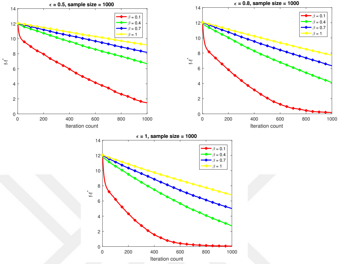
Figure 4.11: DP-SGDwS Results for Sample Size = 1000
