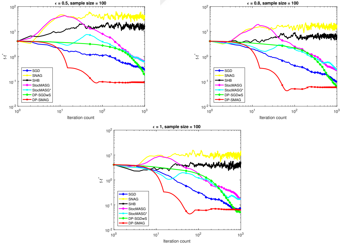
Figure 4.18: Comparison of Stochastic Algorithms For Sample Size = 100
