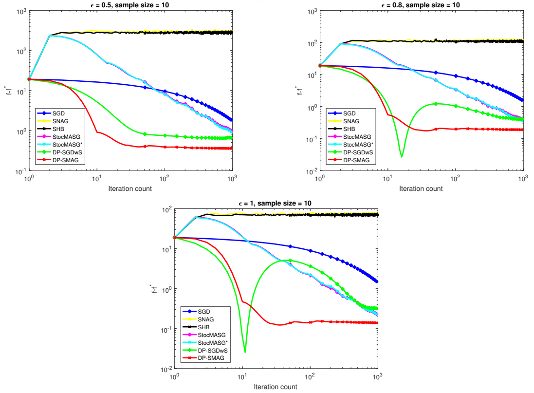
Figure 4.22: Comparison of Stochastic Algorithms For Sample Size = 10 on MNIST
