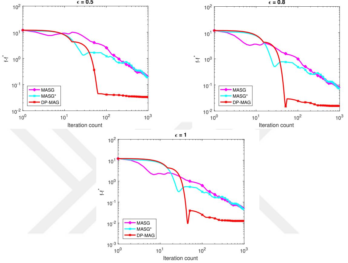
Figure 4.4: Advantage of DP-MAG
