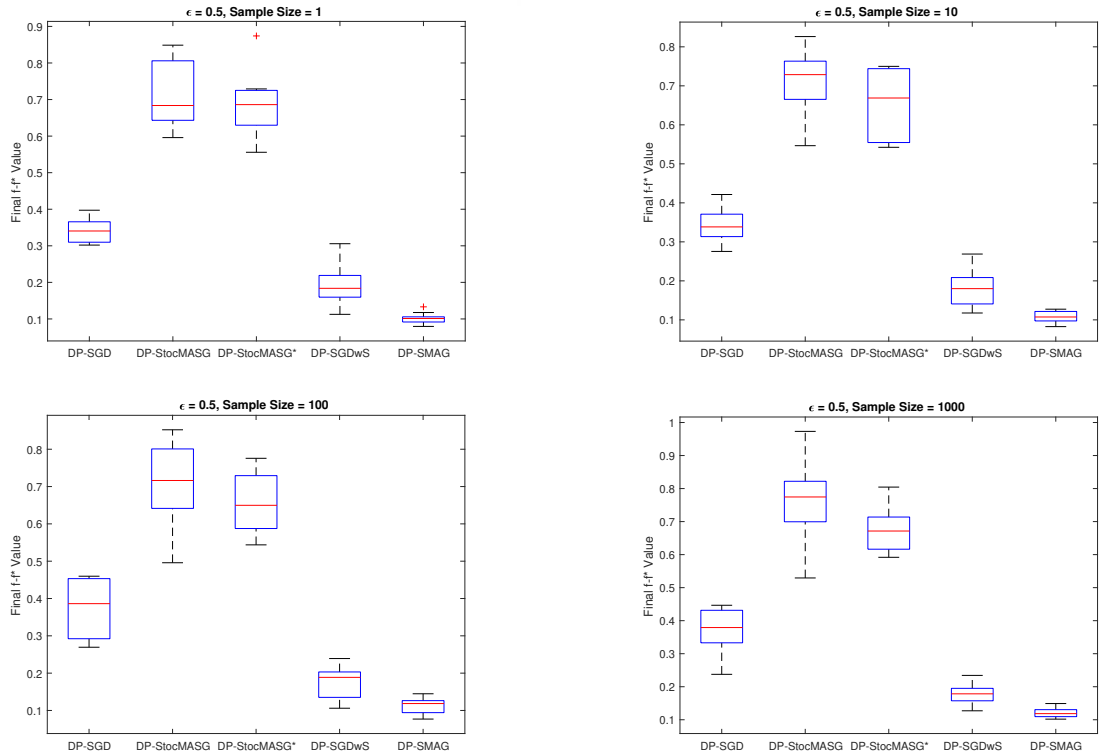
Figure 4.20: Comparison of Stochastic Algorithms For Different Datasets
