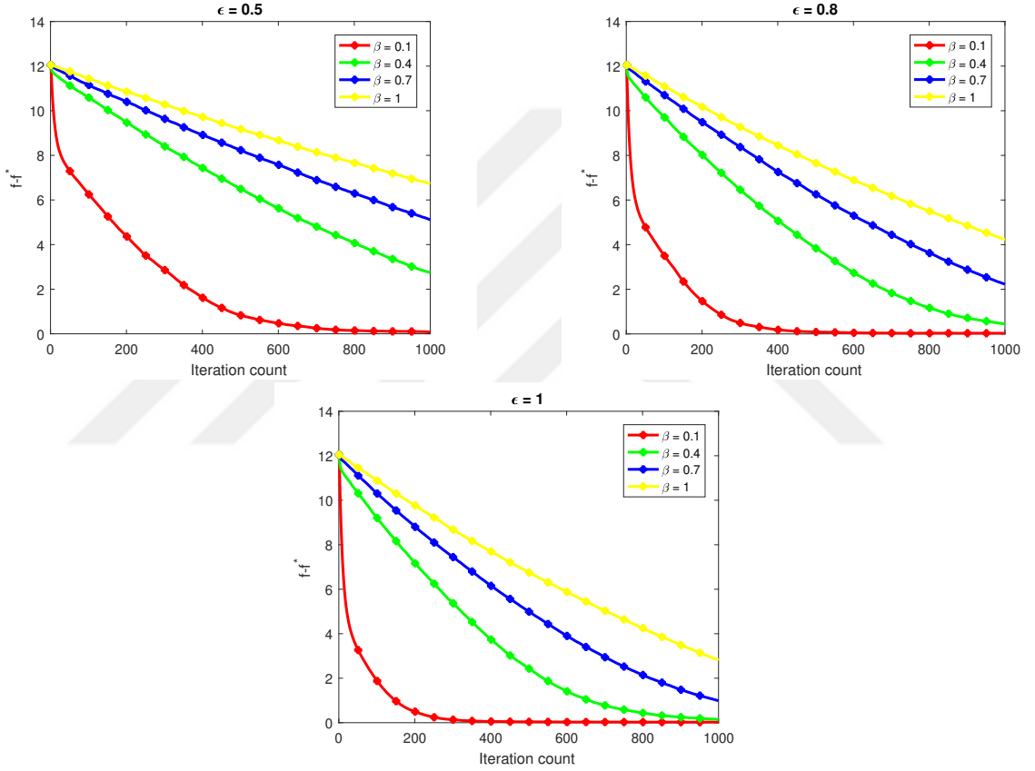
Figure 4.2: Results of DP-GDwS for \epsilon = 0.5, 0.8, 1
