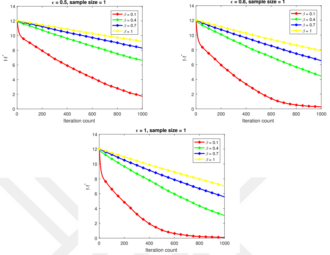
Figure 4.8: DP-SGDwS Results for Sample Size = 1
