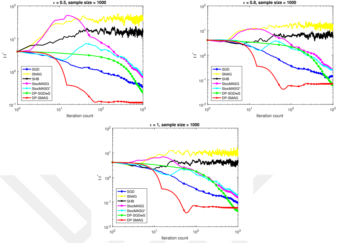
Figure 4.19: Comparison of Stochastic Algorithms For Sample Size = 1000
