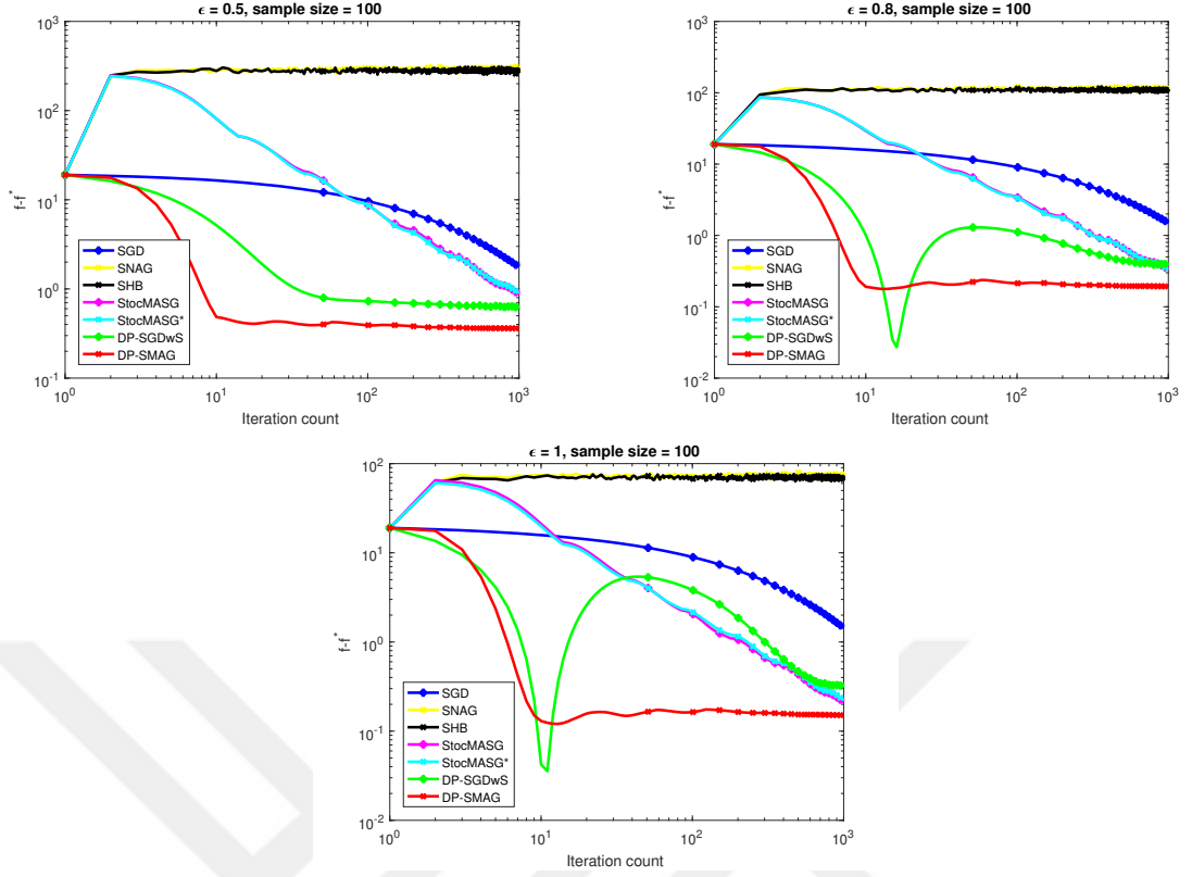
Figure 4.23: Comparison of Stochastic Algorithms For Sample Size = 100 on MNIST
