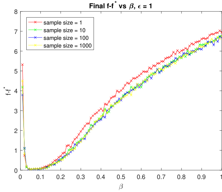
Figure 4.12: Results of DP-SGDwS for \epsilon = 1
