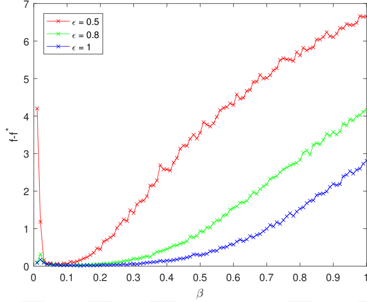
Figure 4.3: Results of DP-GDwS for \epsilon = 0.5, 0.8, 1
