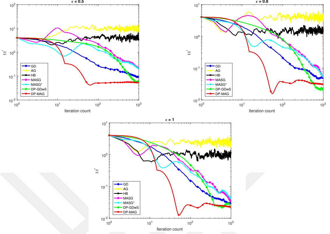
Figure 4.6: Deterministic DP - Comparisons
