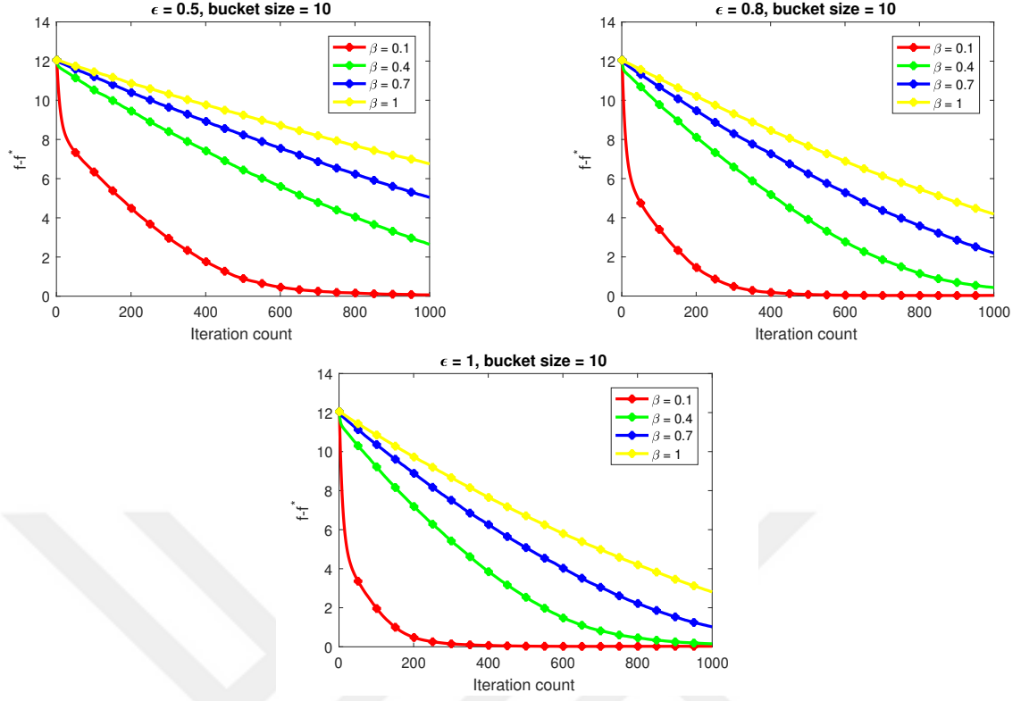
Figure 4.13: DP-onlineGDwS Results for Bucket Size = 10
