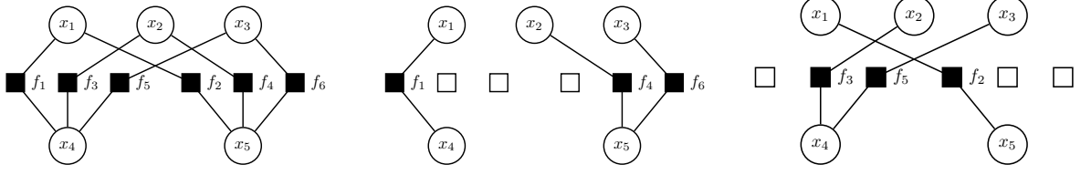
Figure 3.2: (Left) The factor graph of the problem in Example 3.0.1. (Middle and Right) A partitioning of function index set as \mathcal{I} = \cup_{k=1}^K S_k where S_k = S_{k,1} \cup \dots \cup S_{k,B_k} for k = 1, \dots, K . In this example K = 2 and with number of blocks B_1 = B_2 = 2 . (Middle) First subset ( k = 1 ) with S_1 = S_{1,1} \cup S_{1,2} = \{1\} \cup \{4, 6\} and \alpha_{1,1} = \{1, 4\} , \alpha_{1,2} = \{2, 3, 5\} , (Right) Second subset ( k = 2 ) with S_2 = S_{2,1} \cup S_{2,2} = \{3, 5\} \cup \{2\} , \alpha_{2,1} = \{2, 3, 4\} and \alpha_{2,2} = \{1, 5\} .
