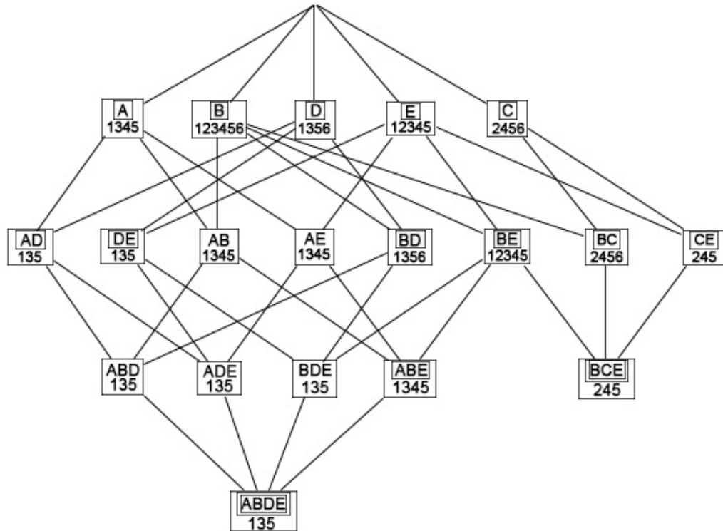
Figure 3.2: Closed Frequent Itemsets
