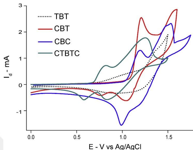
Figure 3.3. Cyclic voltammograms of TBT , CBT , CBC and CTBTC monomers (in 0.1 M TBABF 4 -DCM)
