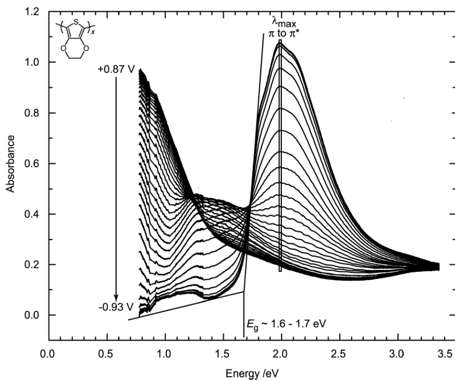
Figure 1.10. Absorption spectra of PEDOT film. [24]
