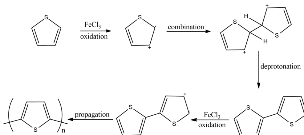
Scheme 1.4. Chemical oxidative polymerization with Ferric Chloride as an oxidant
