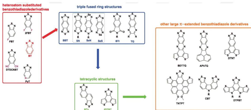
Figure 1.15. Common Benzothiadiazole derivatives in the literature [31]
