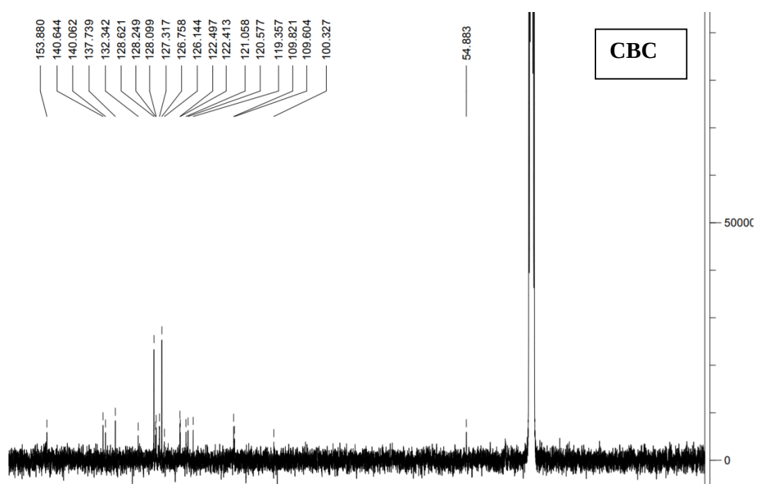
Figure A.2. ^{13}\text{C} NMR of CBC monomer.
