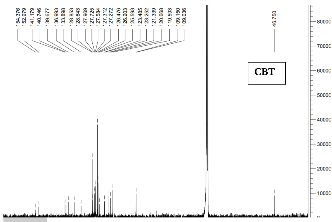
Figure A.4. ^{13}\text{C} NMR of CBT monomer
