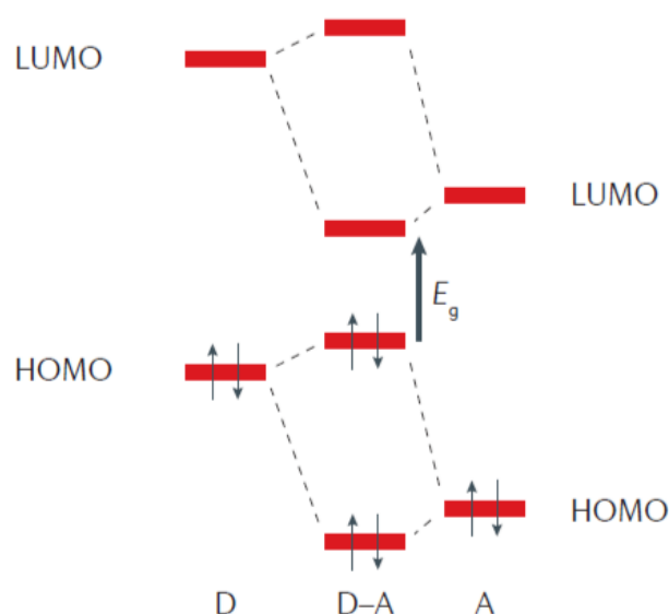
Figure 1.7. Molecular orbital representation of Donor-Acceptor approach
