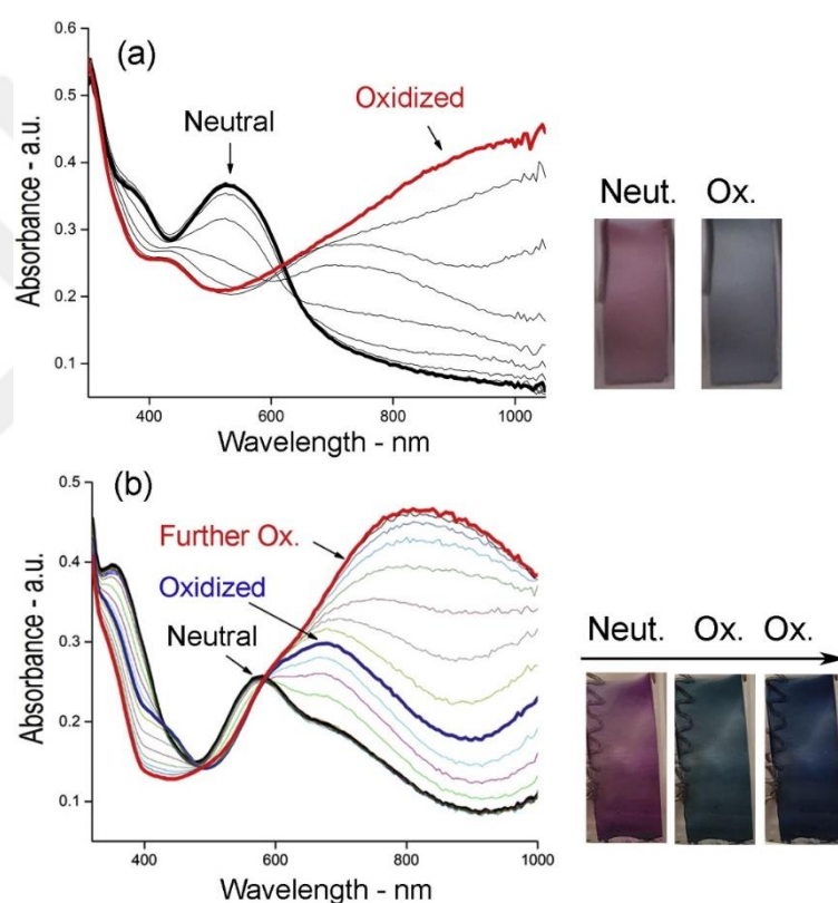
Figure 3.8. UV-Vis Spectra and photos of the films of a) PCBT and b) PCTBTC during oxidation (scan rate 20 mV/s)
