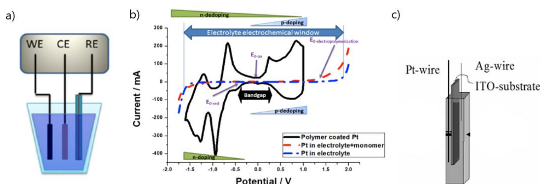
Figure 1.9. a) Electrochemical cell illustration of the three-electrode system b) Potential window of the electrolyte (blue line), oxidation of the monomer during polymerization (red line), and the voltammetric response of the doped conducting polymer (black line) [22]
