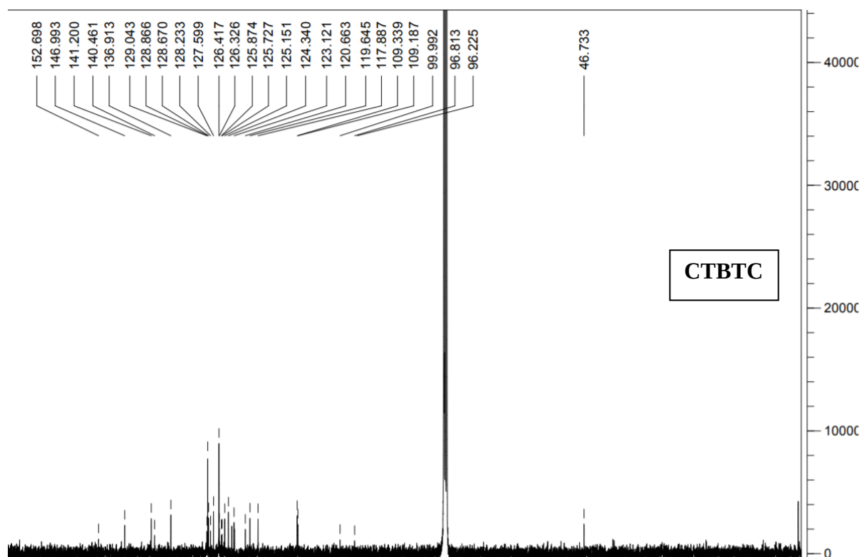
Figure A. 6. ^{13}\text{C} NMR of CTBTC monomer
