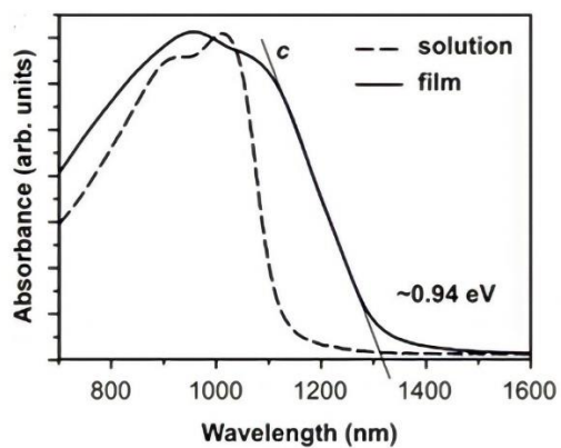
Figure 1.11. Determination of \lambda_{\text{onset}} by extrapolation of transition angle to the baseline [16]
