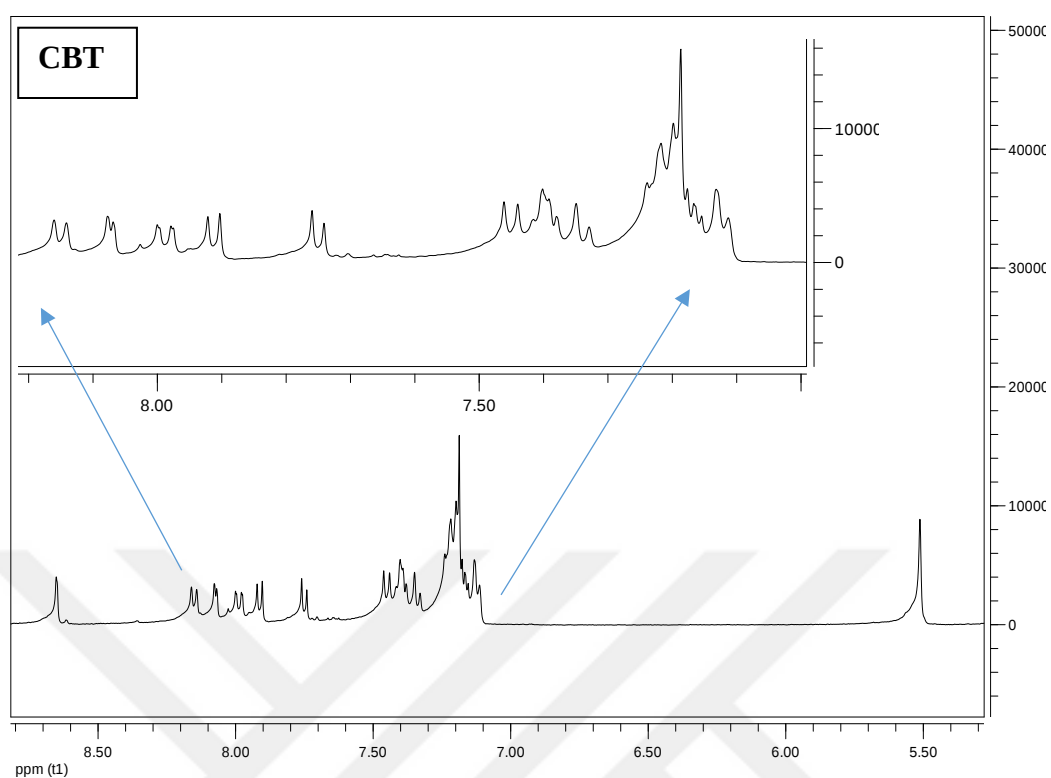
Figure A.3. ^1\text{H} NMR of CBT monomer
