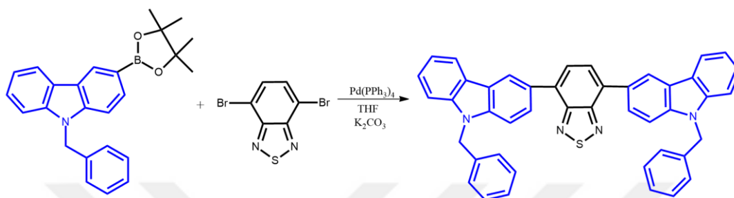
Scheme 2. 1. Chemical reaction route for synthesis of CBC monomer
