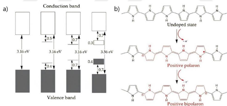
Figure 1.5. a) Valence and conduction band representation b) Illustration of doping process of PPy [3]
