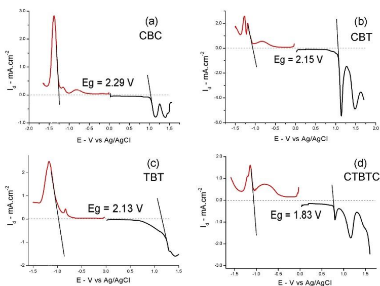
Figure 3.4. Differential pulse voltammograms of the monomers recorded in 0.1 M TBABF 4 electrolytic medium during n-doping and p-doping in the voltage range of a)-1.65 and 1.65 V for CBC monomer b) -1.50 and 1.65 V for CBT monomer c) -1.50 and 1.50 V for TBT monomer d) -1.60 and 1.65 V for CTBTC monomer.
