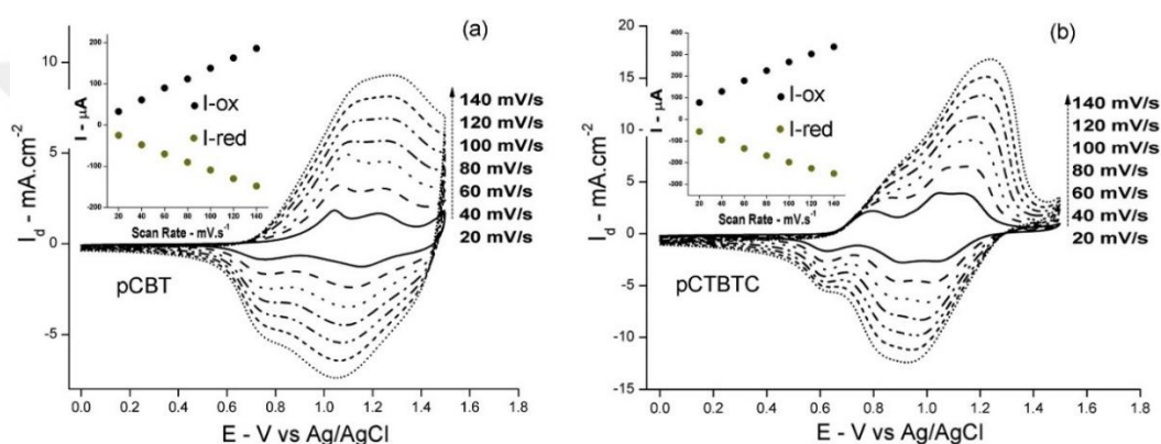
Figure 3.6. Scan rate dependence of a) PCBT and b) PCTBTC between 0.0 V and 1.50 V, at the scan rates from 20 mV/s to 140 mV/s with 20 mV increments. Insets: The anodic and the cathodic peak currents of polymer films vs. scan rate.
