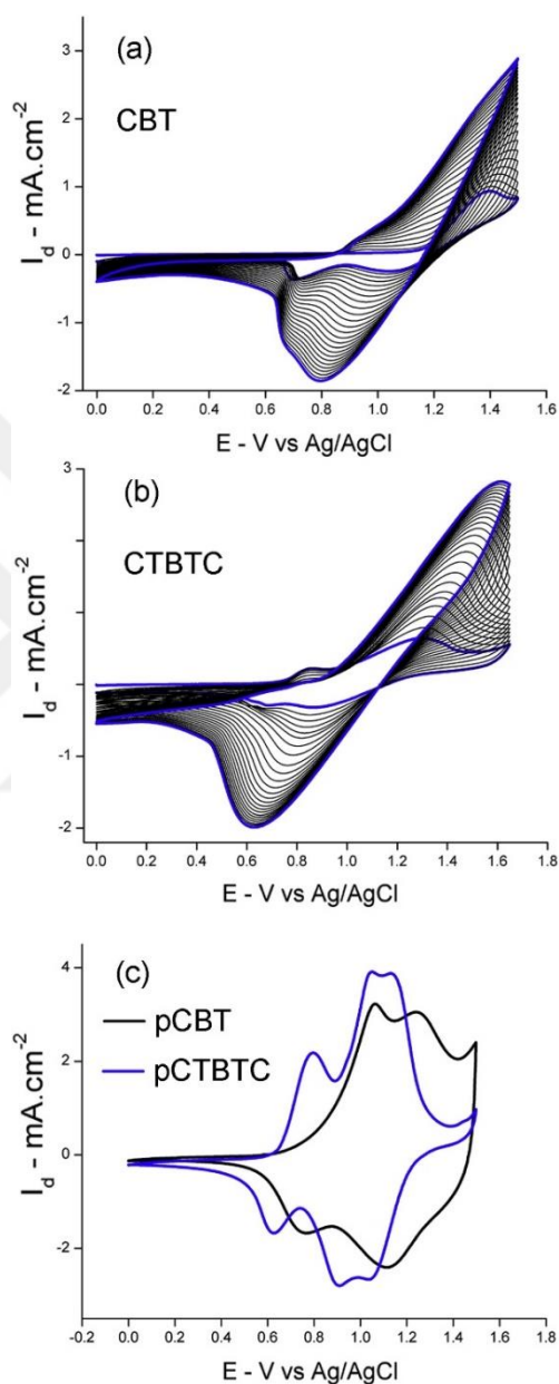
Figure 3.5. Cyclic voltammograms of the monomers during electropolymerizations of a) CBT (between 0.0 V and 1.5 V) b) CTBTC (between 0.0 and 1.65 V) in 0.1 M TBABF 4 /DCM electrolytic medium studied with the scan rate of 100 mV/s. c) cyclic voltammogram of the resulting polymer films at a scan rate of 40 mV/s.
