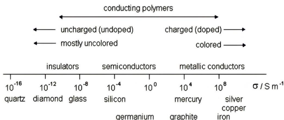
Figure 1.3. Electrical conductivity range of conducting polymers
