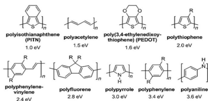
Figure 1.6. Bandgap values of some conjugated polymers [16]
