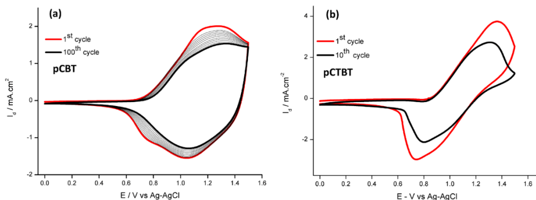
Figure 3.7. Cyclic voltammograms of polymer films upon many cycles a) PCBT upon 100 cycles, b) PCTBTC upon 10 cycles.
