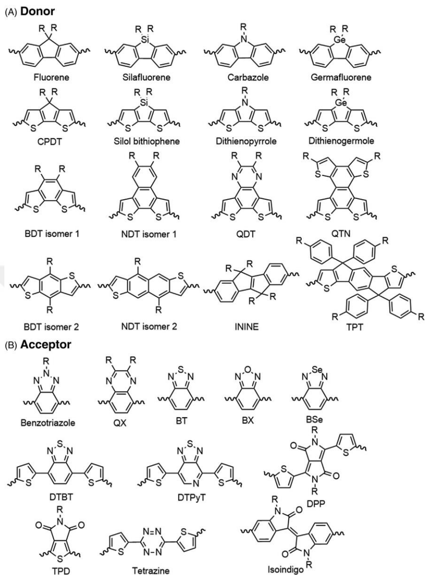
Figure 1.8. Typical a) donor and b) acceptor moieties [20].
