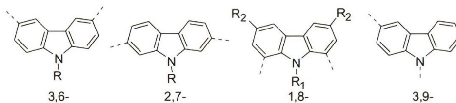
Figure 1.12. Carbazole derivatives
