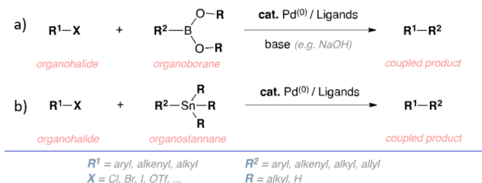
Scheme 1.3. Routes of a) Suzuki and b) Stille Cross-Coupling reactions
