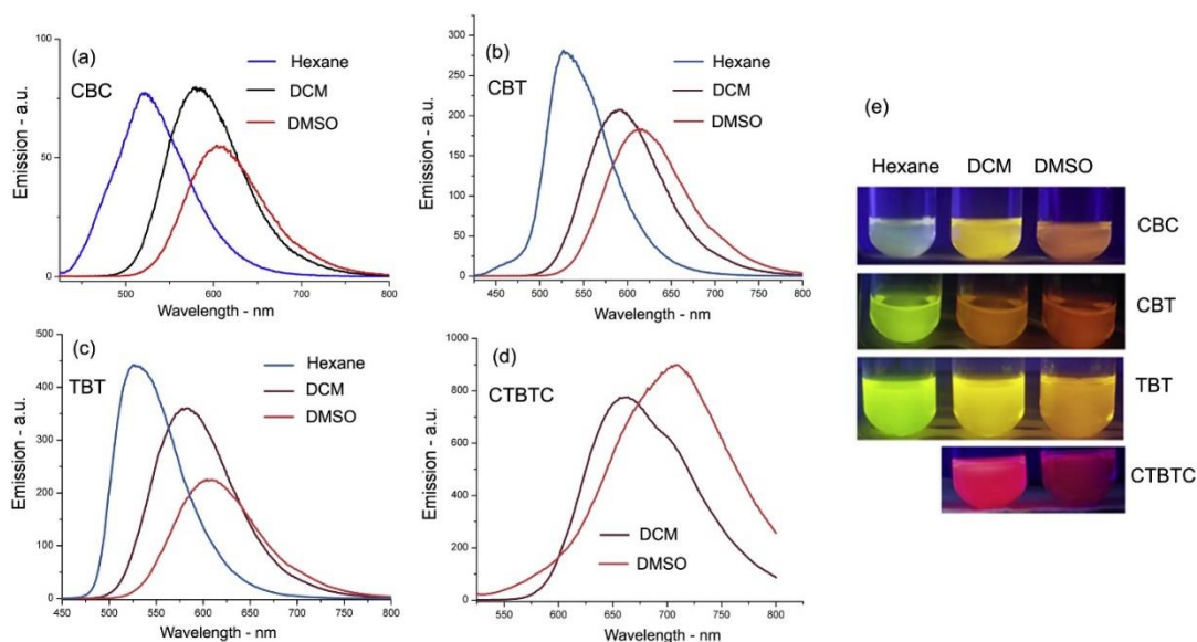
Figure 3.2. Fluorescence spectra of the monomers in Hexane, DCM and DMSO a) CBC , b) CBT , c) TBT , d) CTBTC e) monomer solutions in different solvents under UV light
