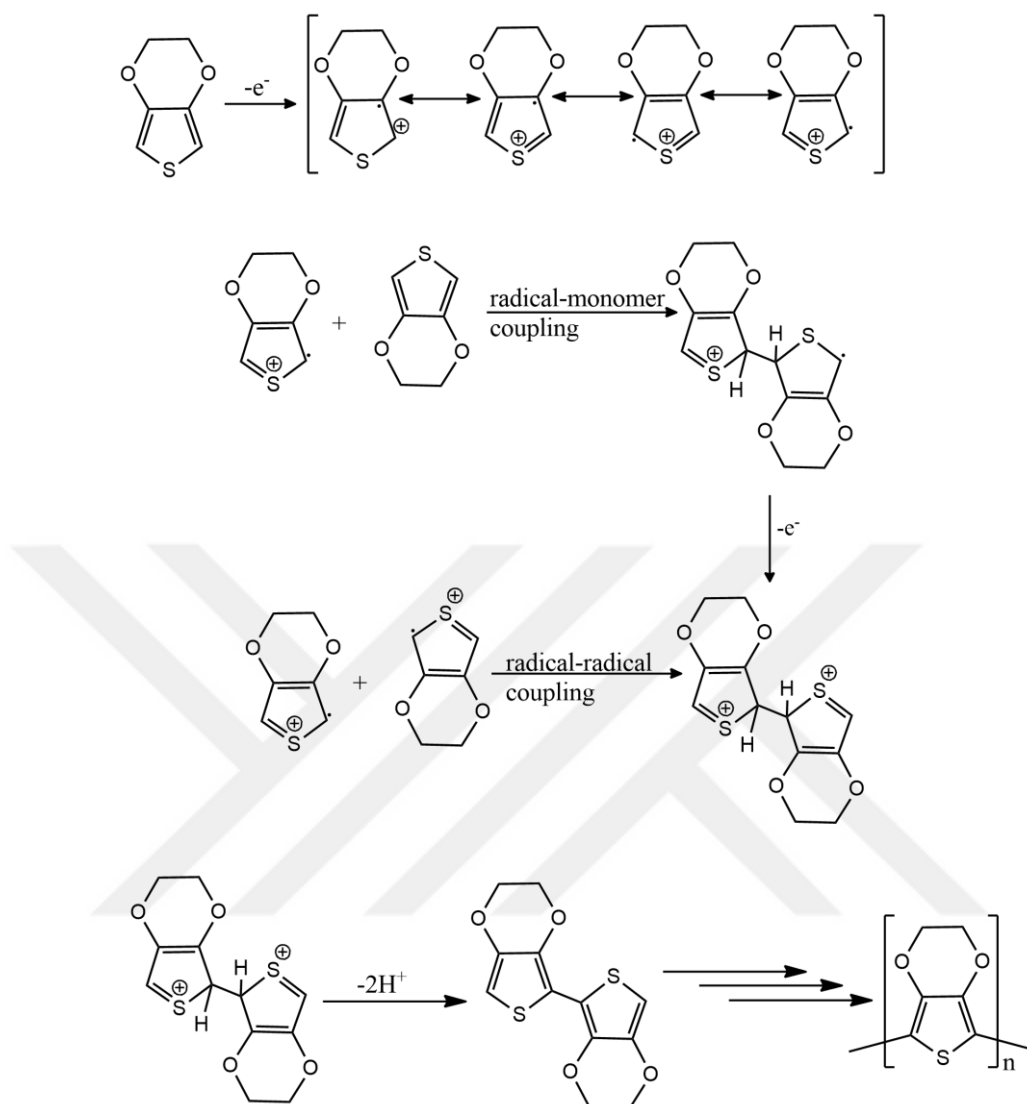
Scheme 1.5. Electrosynthesis mechanism of PEDOT [23]
