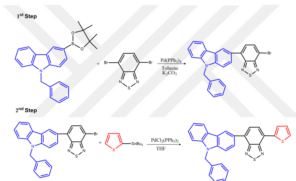
Scheme 2. 2. Chemical reaction route for synthesis of CBT monomer
