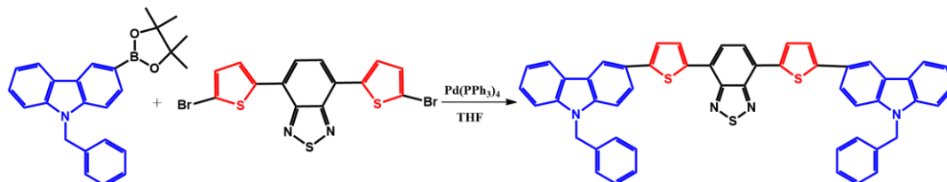
Scheme 2. 3. Chemical reaction route for synthesis of CTBTC monomer
