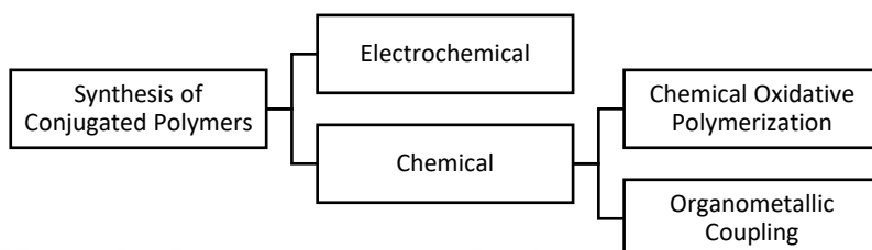
Scheme 1.1. Synthesis of conjugated polymers
