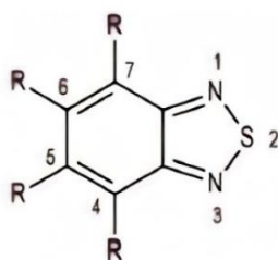
Figure 1.14. 2,1,3-Benzothiadiazole (B)
