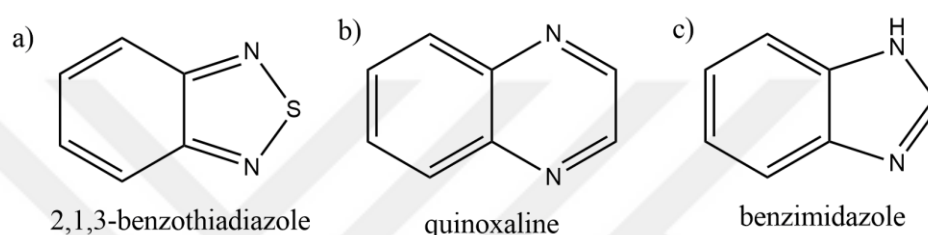
Figure 1.13. Chemical structures of a) 2,1,3-Benzothiadiazole, b)Quinoxaline, c)Benzimidazole
