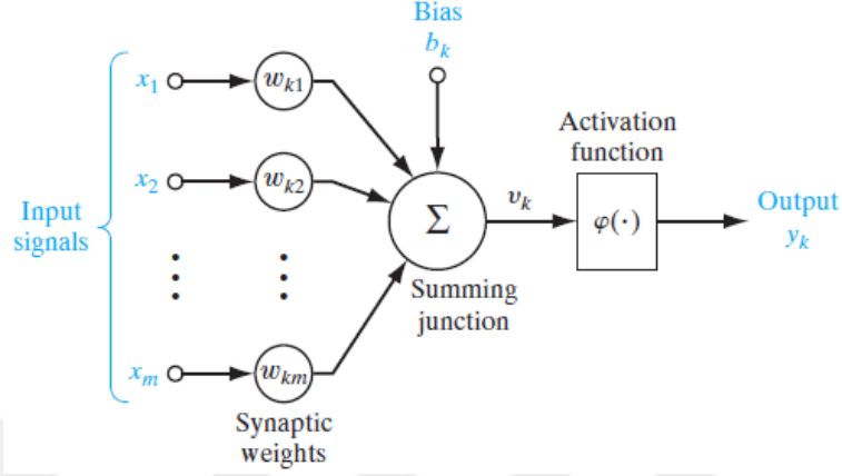
Figure 2.1: Perceptron model. 1
