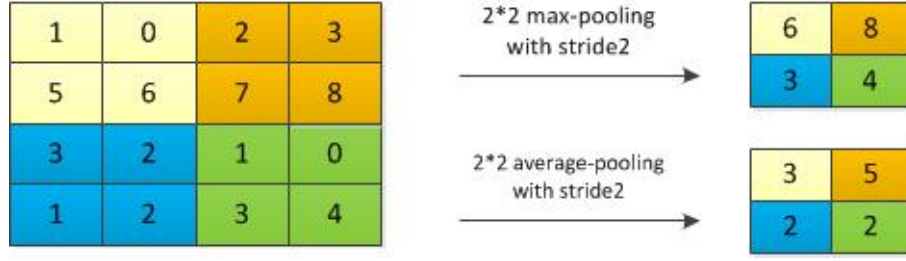
Figure 2.7: Examples of non-overlapping pooling. Top : Max-pooling operation. Bottom : Average-pooling operation.
