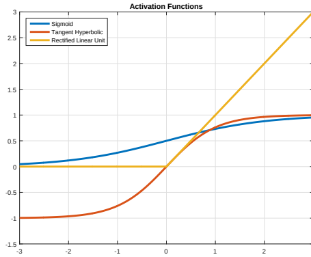
Figure 2.2: Activation functions sigmoid, tangent hyperbolic and rectified linear unit.
