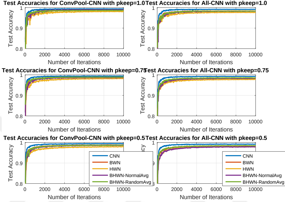
Figure 4.2: Test accuracy results for different dropout probabilities.
