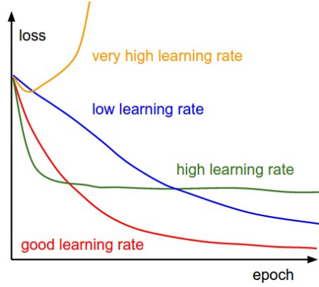
Figure 3.4: Effects of different learning rates [3].
