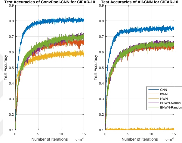
Figure 4.4: Test accuracy results for different activation functions at FC layer.
