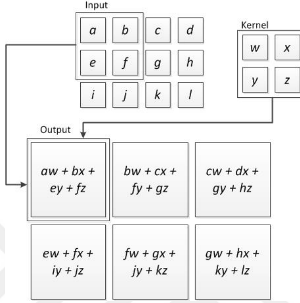
Figure 2.5: An example of 2-D convolution operation without kernel flipping [1].
