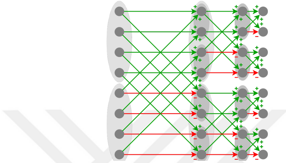
Figure 3.1: Fast Hadamard Transform algorithm of a vector of length 8. 1
