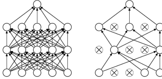
Figure 2.4: Left: A classical neural network with 2 hidden layers. Right: A thinned network after dropout is applied. 2
