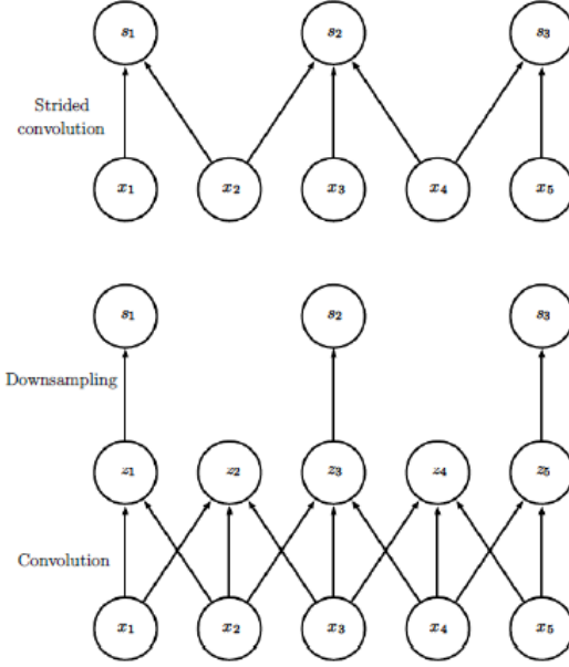
Figure 3.3: Top : Strided convolution with a stride of 2. Bottom : Convolution with unit stride followed by downsampling. 2
