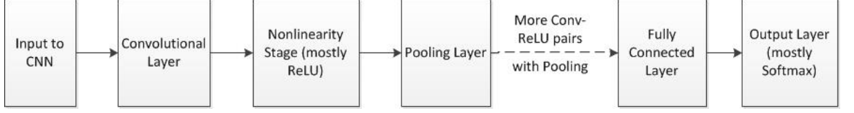
Figure 2.6: An example of standard CNN with its major components.
