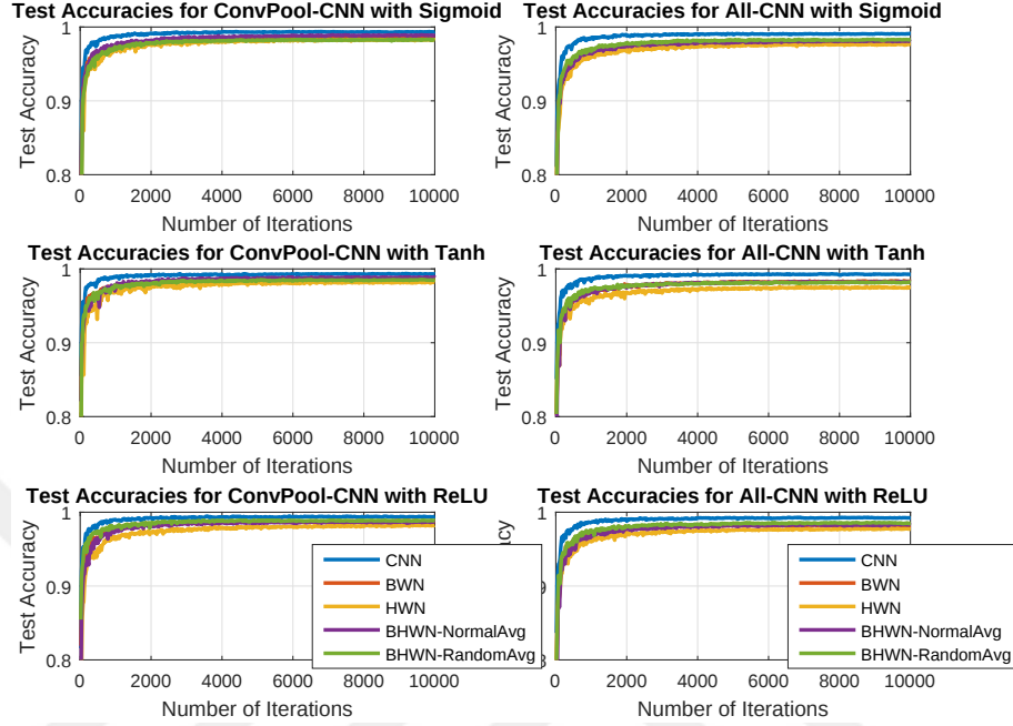
Figure 4.3: Test accuracy results for different activation functions at FC layer.
