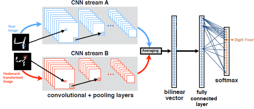
Figure 3.2: Our approach to combine BWN and HIN: The architecture of BWHIN [2].
