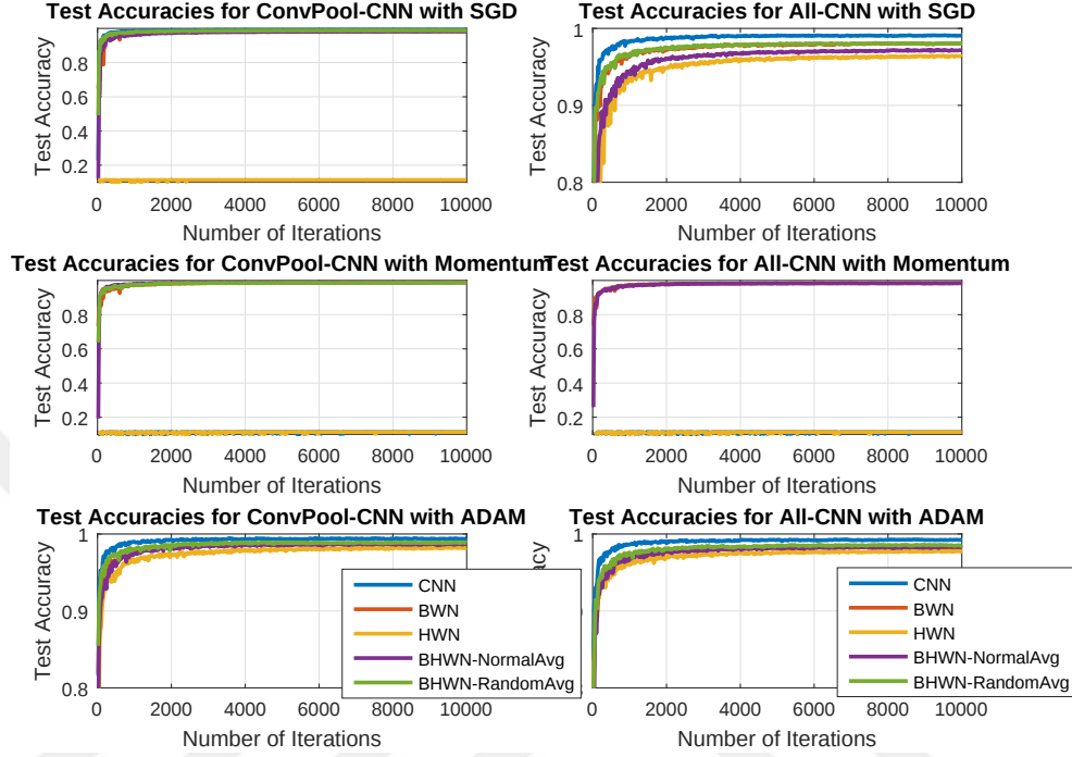
Figure 4.1: Test accuracy results for different optimizers.
