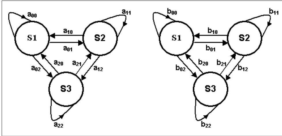
Figure 2.4: Markov model \lambda_1 corresponding to VOC plume (left) and the Markov model \lambda_2 of ordinary moving objects (right). Transition probabilities a_{ij} and b_{ij} are estimated off-line.
