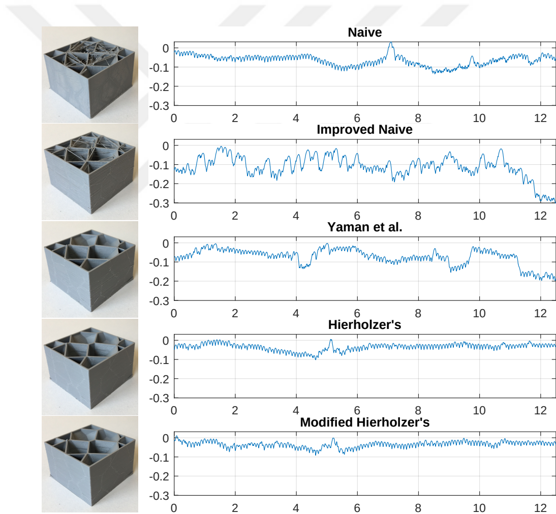
Figure 4.37: 3D printed boxes, and a sample surface roughness profile measured on an edge in the height direction. Both axes are in mm.
