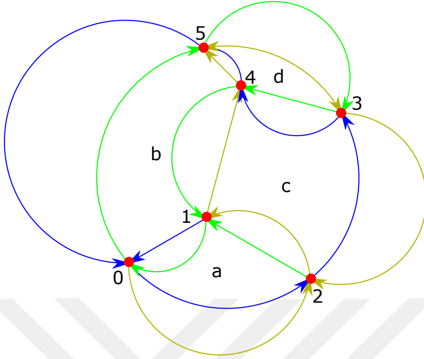
Figure 3.5: Subpaths are enlarged using available connections. Note that the green subpath is reversed during the enlargement.
