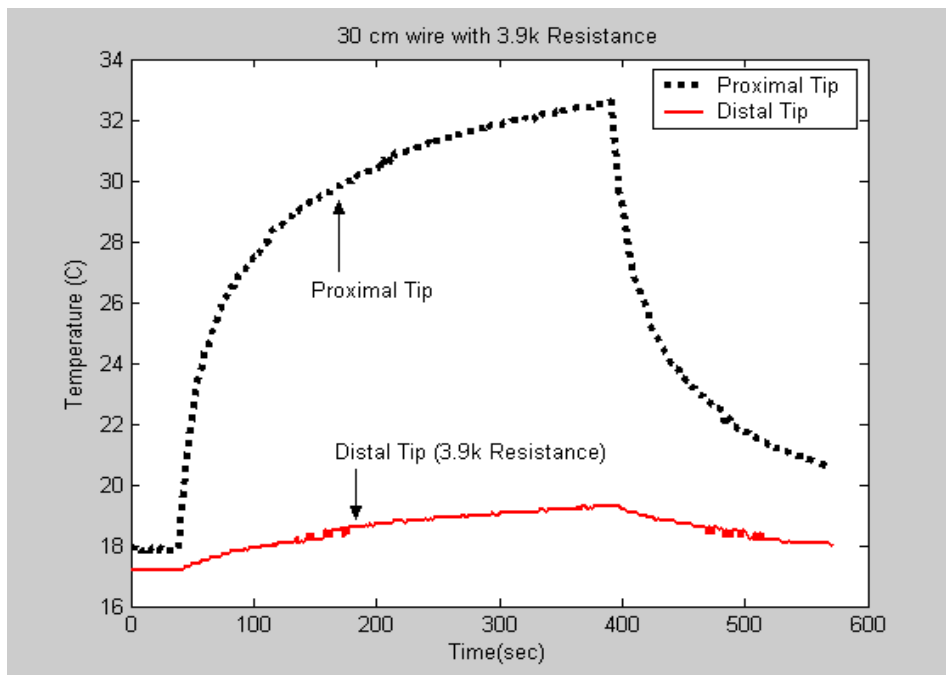
Figure 40. Temperature rise versus time at the distal and proximal electrode of the 30 cm wire 3.9 kΩ resistance placed on the distal electrode of the wire
