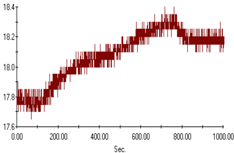
Figure 44. Heating experiment result of IPG model with CSC
