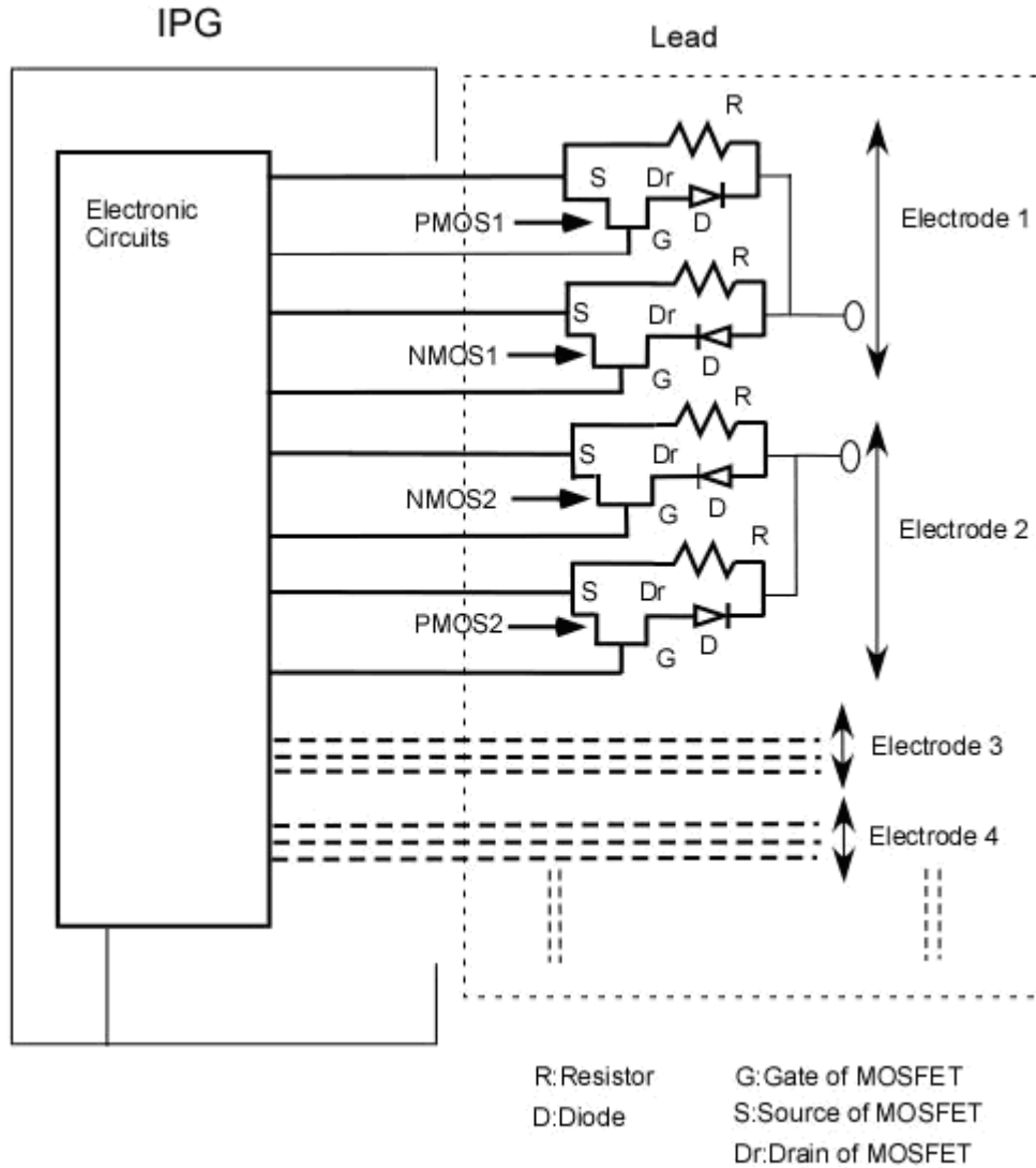
Figure12. Multi electrode pacing mode TDC Implementation-2 with capability of programming positive and negative pulses.
