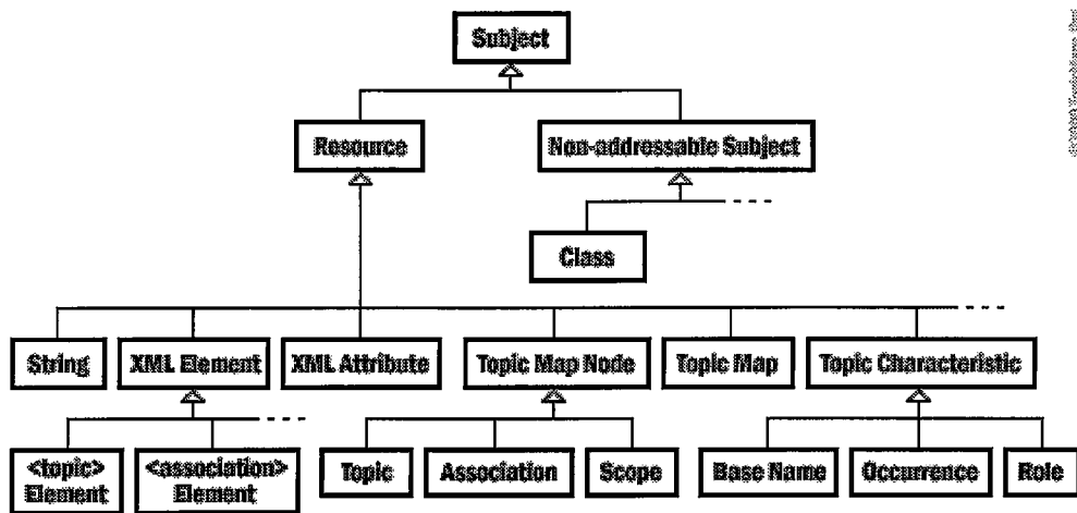
Figure 2.1: Class hierarchy for XTM conceptual model
