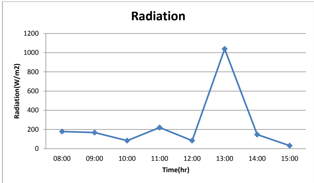
Figure 5-23: Hourly Changing Of Irradiance on January 8 th
