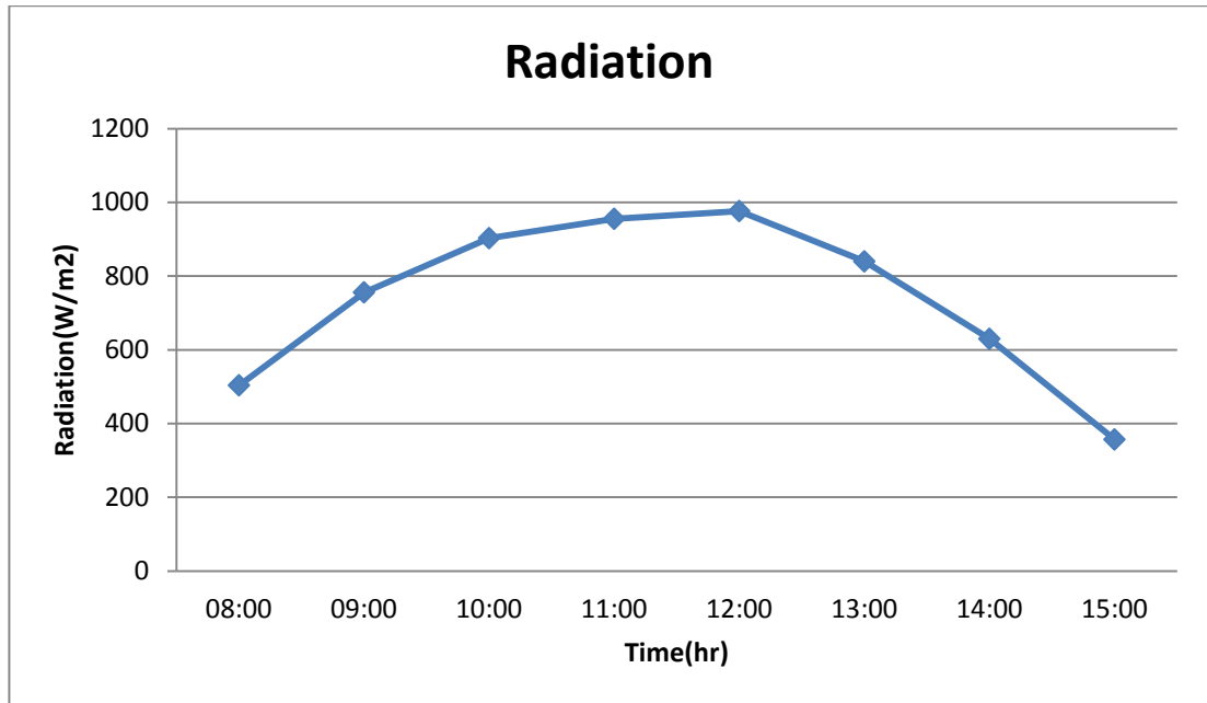
Figure 5-8: Variation of Irradiance during December 29 th
