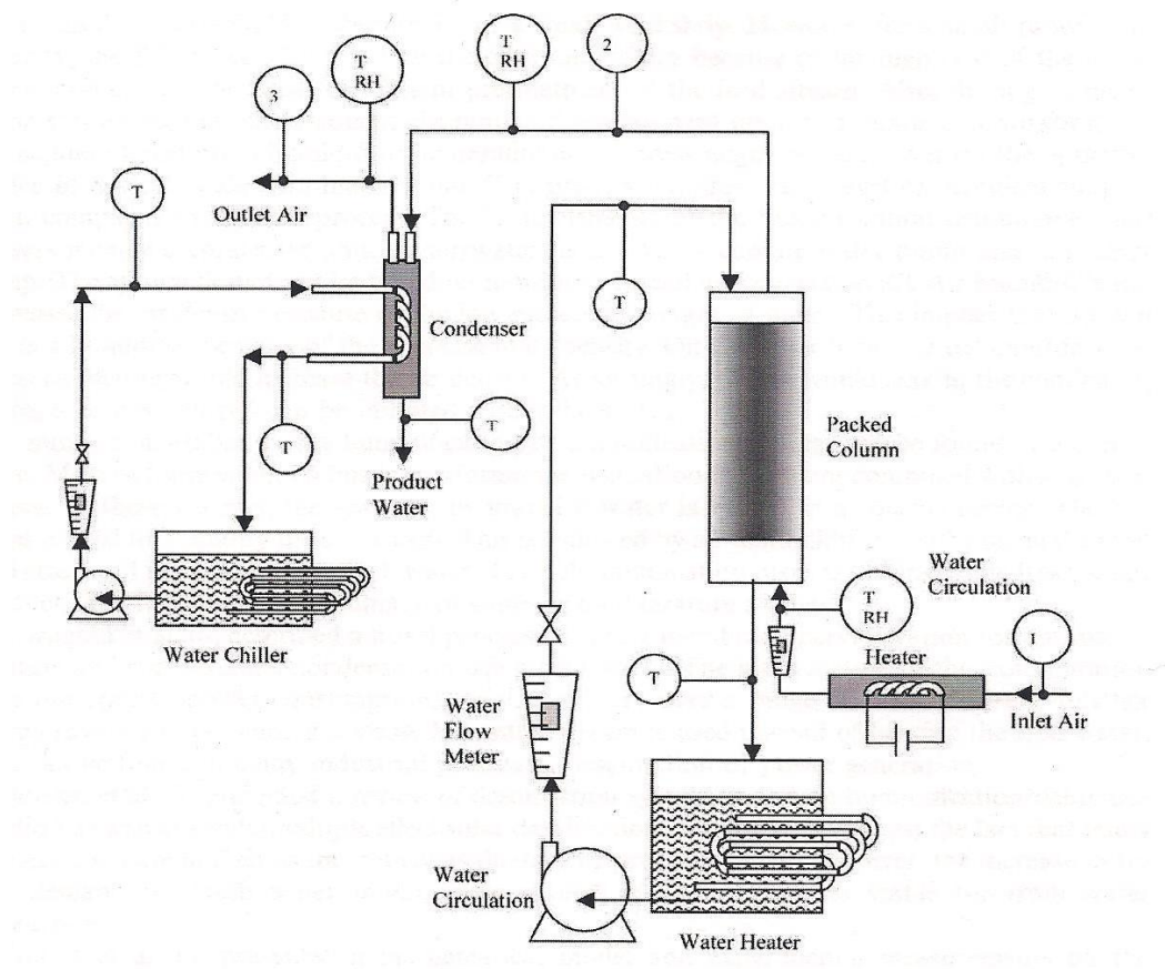
Figure 2-12: A Schematic of Experimental Unit [2].
