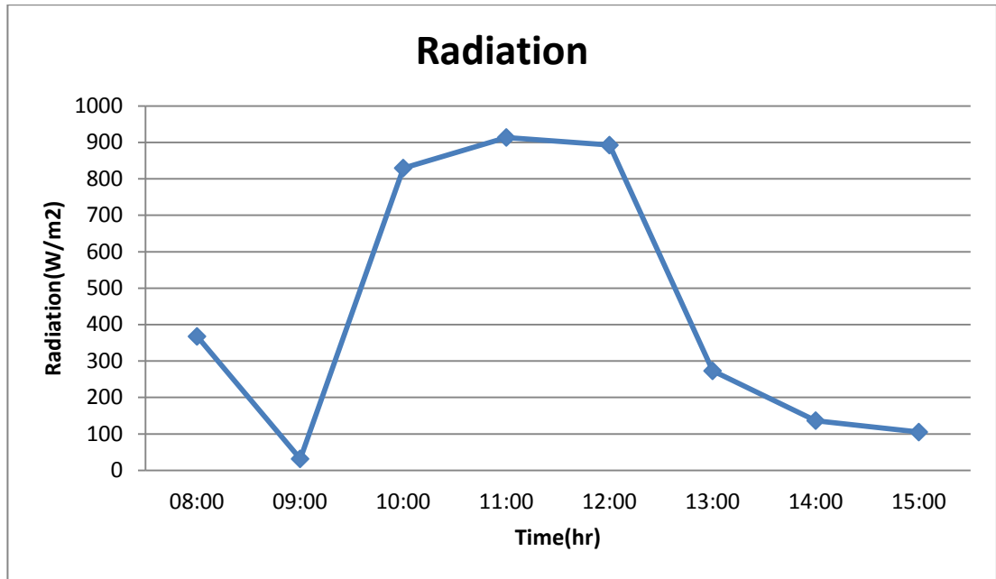
Figure 5-20: Variation of Insolation on January 7 th
