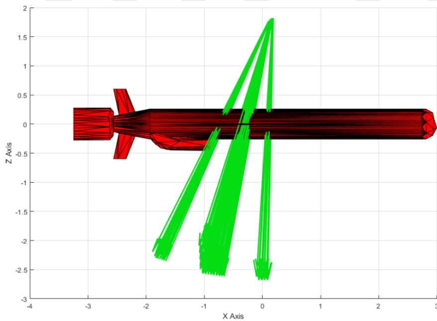
Figure 3.5: Scattering of Striking Fragments at Detonation Point 12 on XZ Axis for the 1 st Scenario
