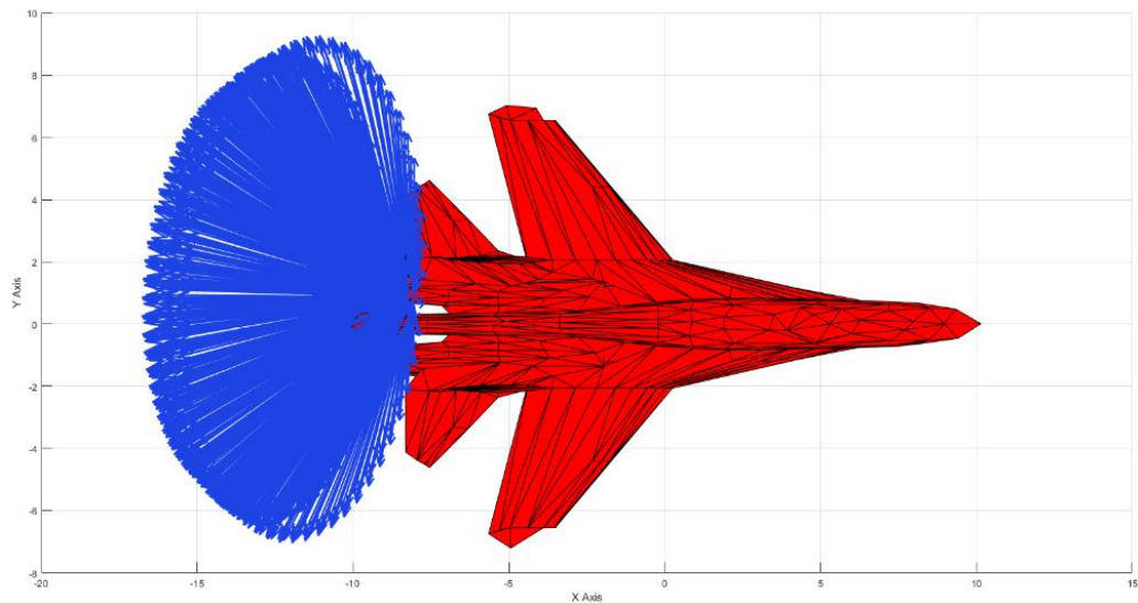
Figure 3.17: Scattering of All Fragments at Detonation Point 76 on XY Axis for the 2 nd Scenario
