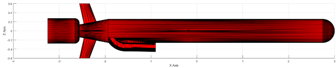
Figure 2.29: The Side View of the Cruise Missile with 10000 Triangles in Total
