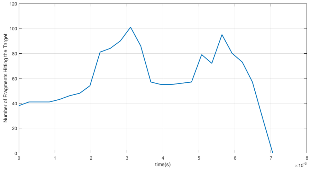
Figure 3.10: The Number of Fragments Hitting The Target vs Time for the 1 st Scenario
