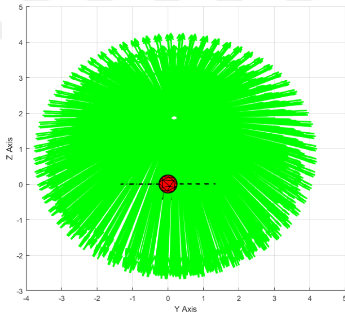
Figure 3.9: Scattering of All Fragments at Detonation Point 12 on YZ Axis for the 1 st Scenario
