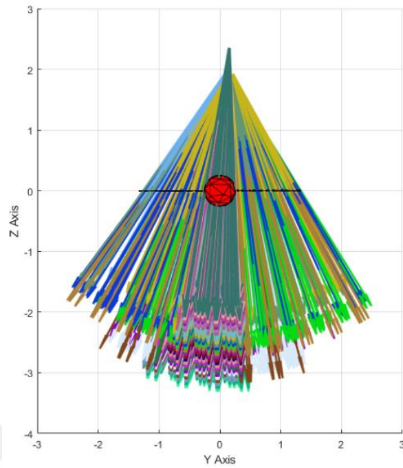
Figure 3.3: Scattering of Striking Fragments at All Detonation Points on YZ Axis for the 1 st Scenario
