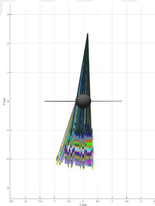
Figure 3.27: Scattering of Striking Fragments at All Detonation Points on YZ Axis for the 1 st Scenario by Using the Sphere Tool
