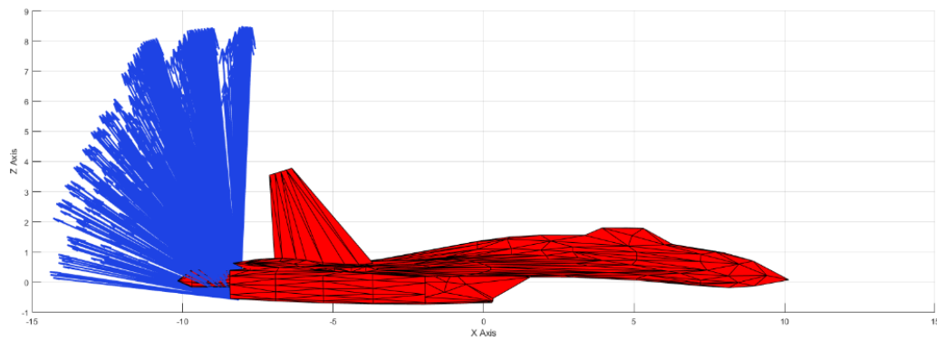
Figure 3.15: Scattering of Striking Fragments at Detonation Point 76 on XZ Axis for the 2 nd Scenario
