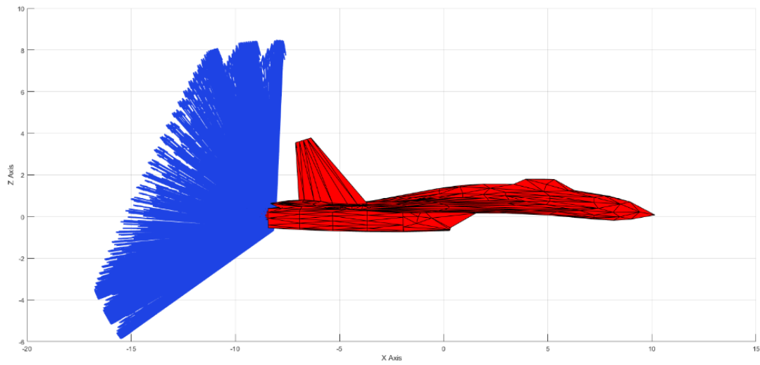
Figure 3.18: Scattering of All Fragments at Detonation Point 76 on XZ Axis for the 2 nd Scenario
