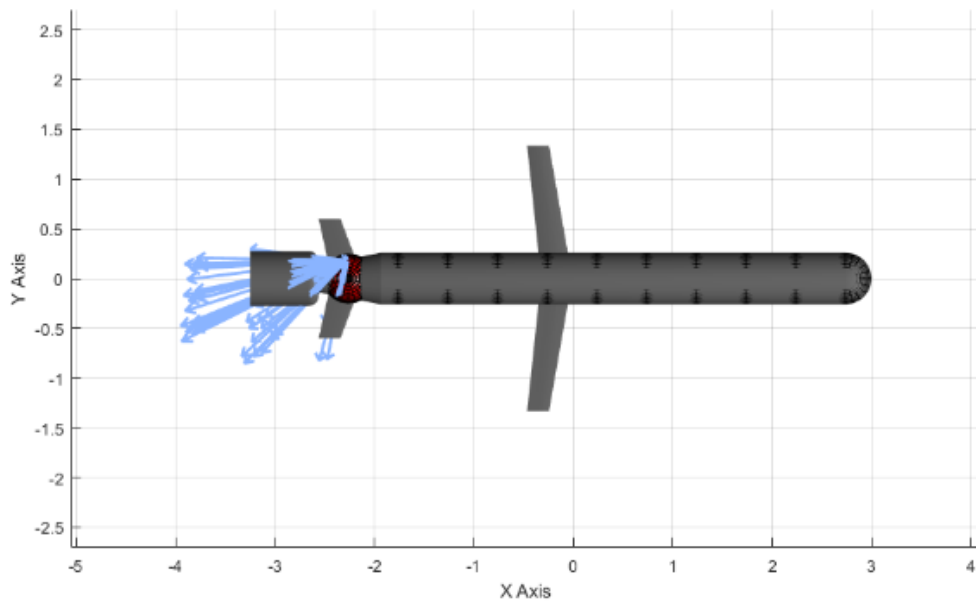
Figure 3.28: Scattering of Striking Fragments at Detonation Point 22 on XY Axis for the 1 st Scenario by Using the Sphere Tool
