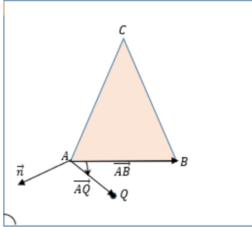
Figure 2.41: Point Q is Outside the Triangle
