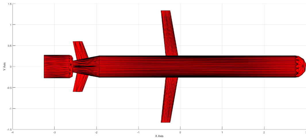
Figure 2.16: The Top View of the Cruise Missile with 1500 Triangles in Total
