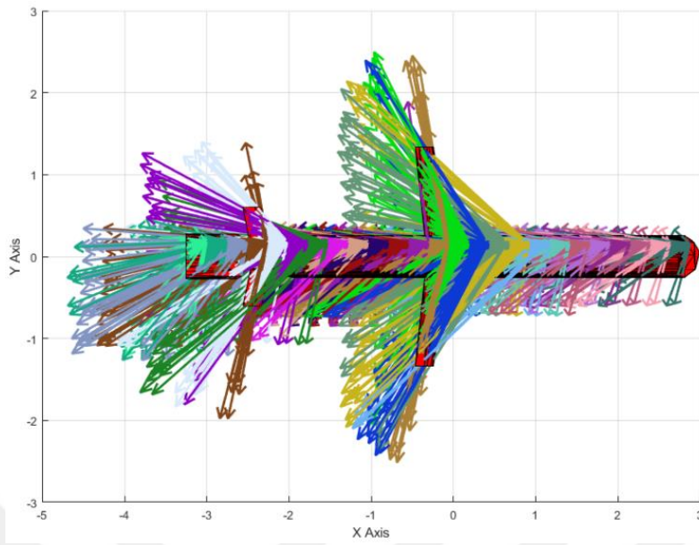
Figure 3.1: Scattering of Striking Fragments at All Detonation Points on XY Axis for the 1 st Scenario
