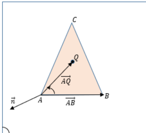
Figure 2.40: Point Q is Inside the Triangle
