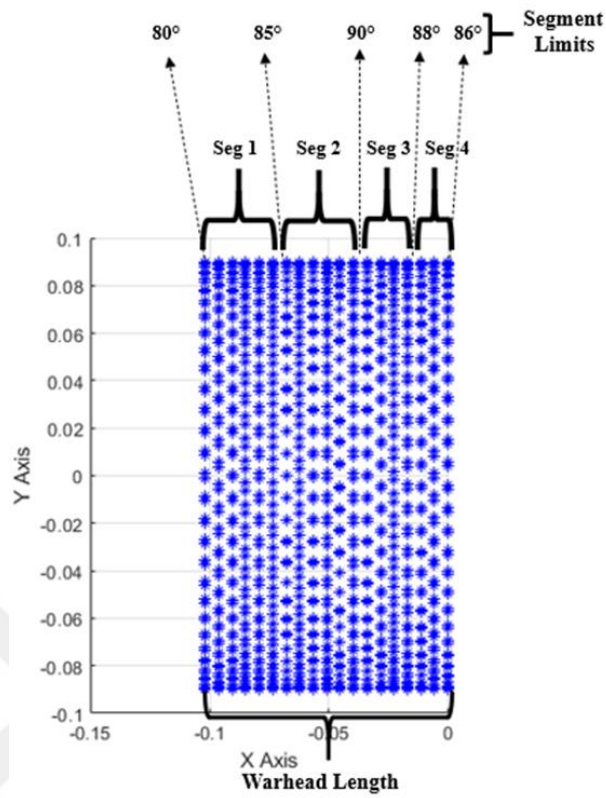
Figure 2.37: Representation of Some Warhead Parameters on the XY Axis of the Warhead Model
