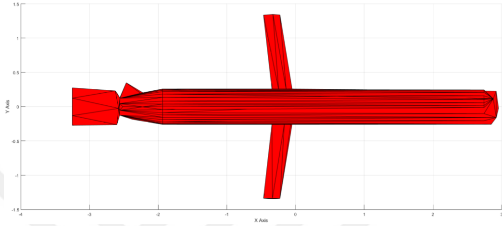
Figure 2.4: The Top View of the Cruise Missile with 250 Triangles in Total
