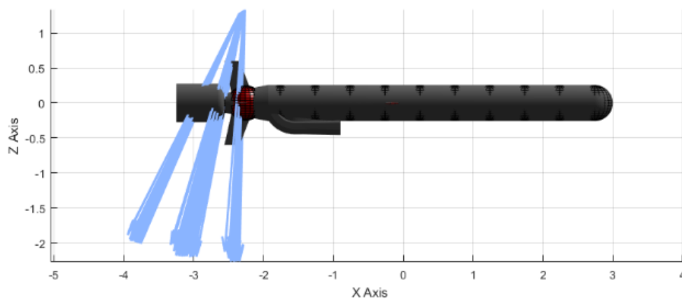
Figure 3.29: Scattering of Striking Fragments at Detonation Point 22 on XZ Axis for the 1 st Scenario by Using the Sphere Tool
