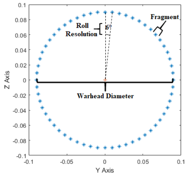
Figure 2.38: Representation of Some Warhead Parameters on One Ring
