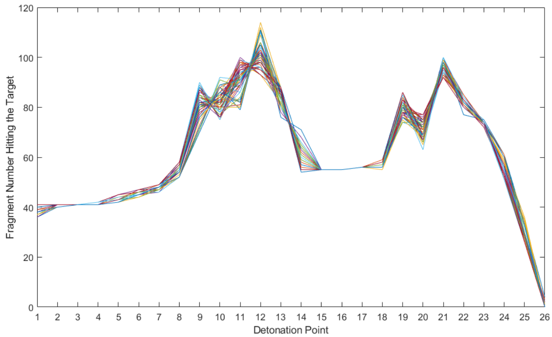
Figure 3.22: Fragment Number Hitting the Target vs Detonation Point for 50 Runs
