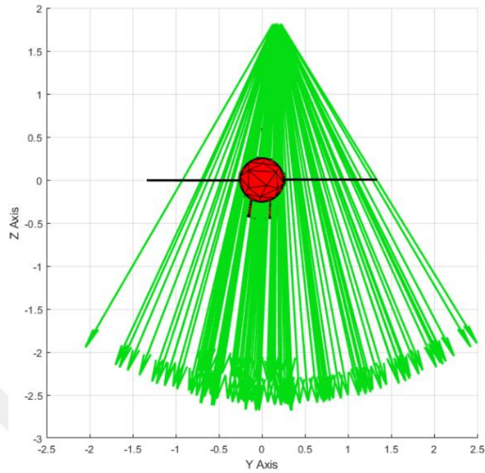
Figure 3.6: Scattering of Striking Fragments at Detonation Point 12 on YZ Axis for the 1 st Scenario
