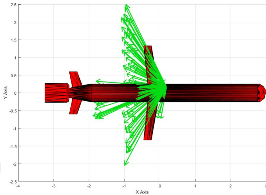
Figure 3.4: Scattering of Striking Fragments at Detonation Point 12 on XY Axis for the 1 st Scenario
