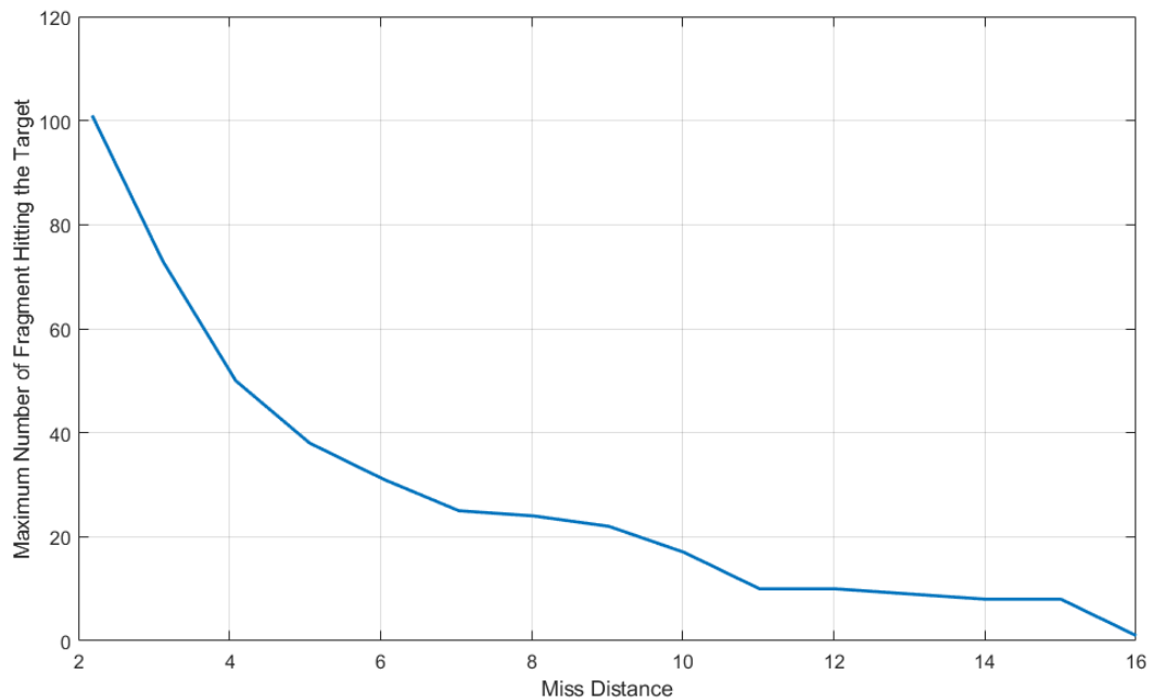
Figure 3.21: Maximum Number of Fragment Hitting the Target vs Miss Distance
