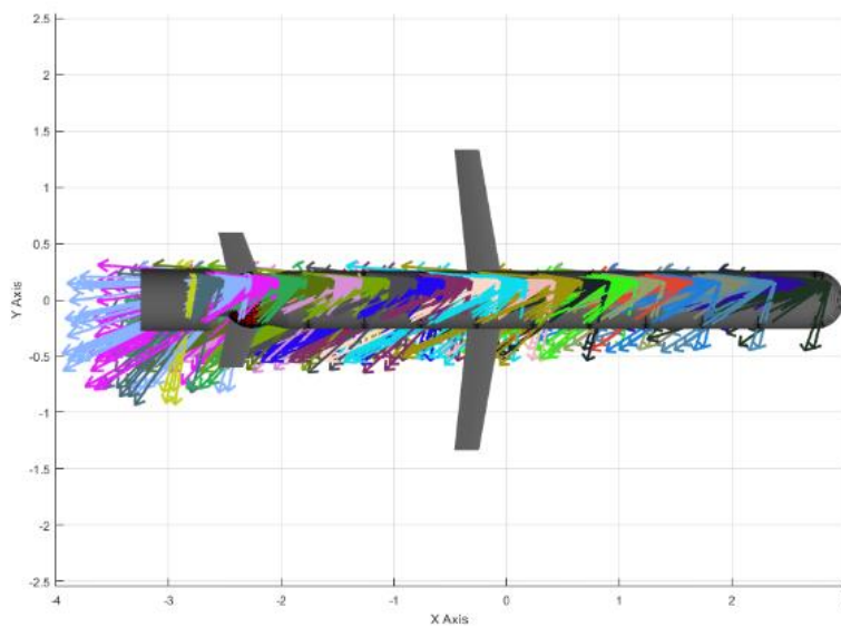
Figure 3.25: Scattering of Striking Fragments at All Detonation Points on XY Axis for the 1 st Scenario by Using the Sphere Tool
