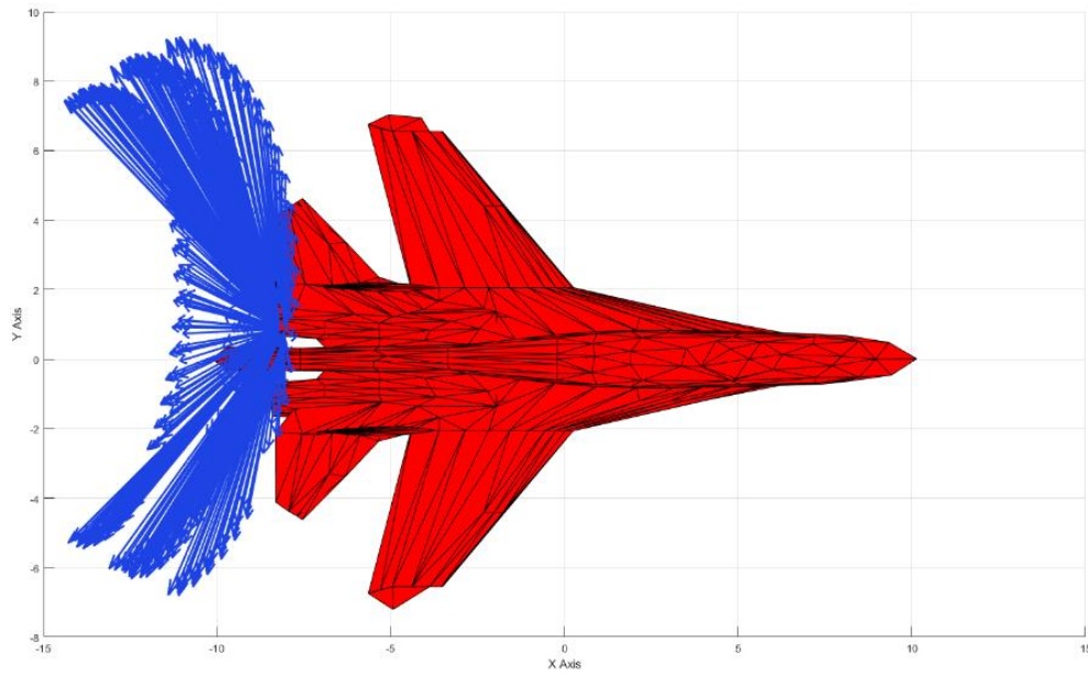
Figure 3.14: Scattering of Striking Fragments at Detonation Point 76 on XY Axis for the 2 nd Scenario
