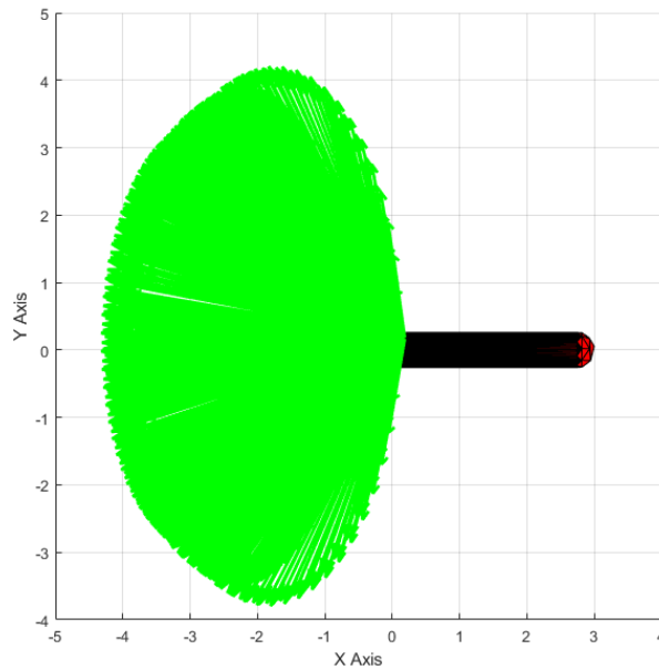
Figure 3.7: Scattering of All Fragments at Detonation Point 12 on XY Axis for the 1 st Scenario
