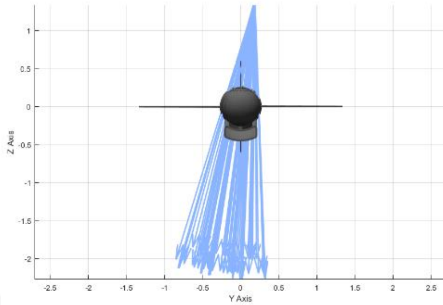
Figure 3.30: Scattering of Striking Fragments at Detonation Point 22 on YZ Axis for the 1 st Scenario by Using the Sphere Tool
