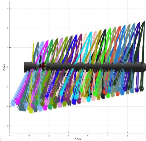
Figure 3.26: Scattering of Striking Fragments at All Detonation Points on XZ Axis for the 1 st Scenario by Using the Sphere Tool
