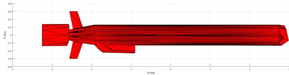
Figure 2.11: The Side View of the Cruise Missile with 500 Triangles in Total
