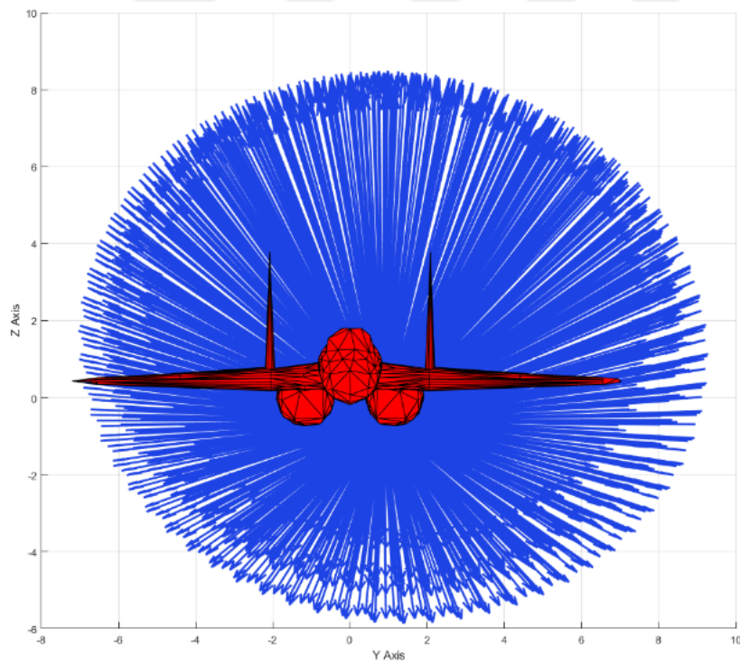
Figure 3.19: Scattering of All Fragments at Detonation Point 76 on YZ Axis for the 2 nd Scenario
