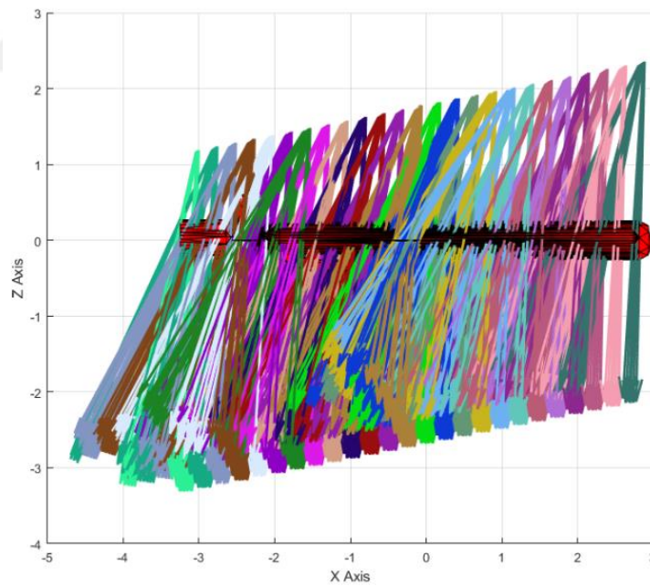
Figure 3.2: Scattering of Striking Fragments at All Detonation Points on XZ Axis for the 1 st Scenario
