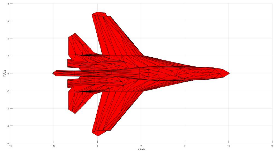
Figure 2.31: The Top View of the Fighter with 1000 Triangles in Total
