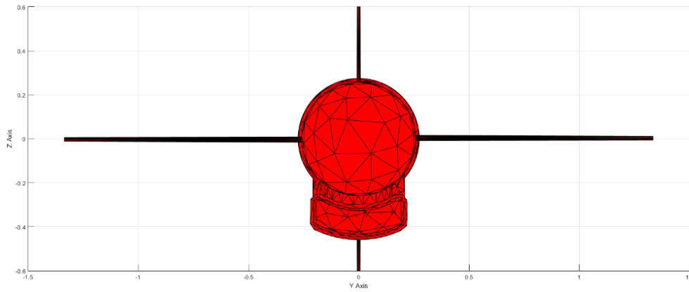
Figure 2.21: The Front View of the Cruise Missile with 2000 Triangles in Total
