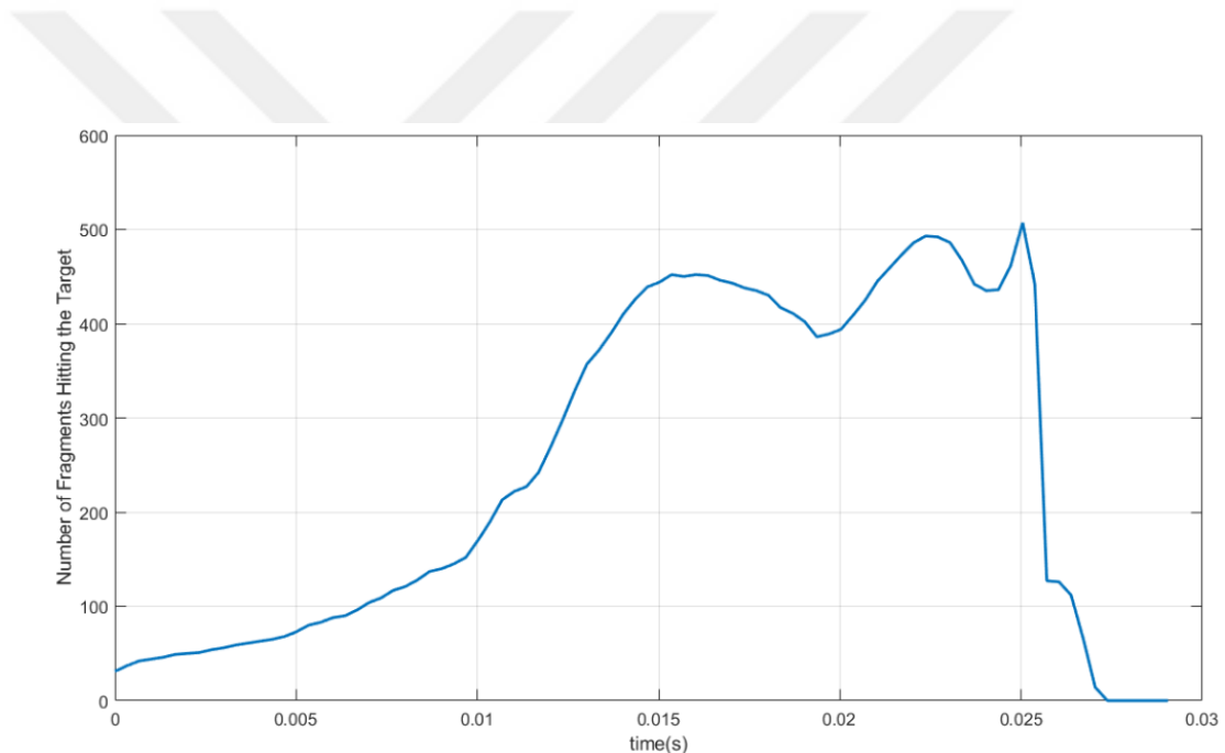
Figure 3.20: The Number of Fragments Hitting The Target vs Time for the 2 nd Scenario
