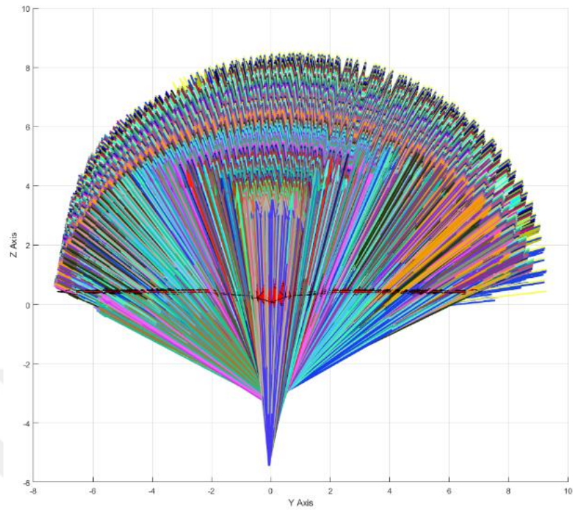
Figure 3.13: Scattering of Striking Fragments at All Detonation Points on YZ Axis for the 2 nd Scenario
