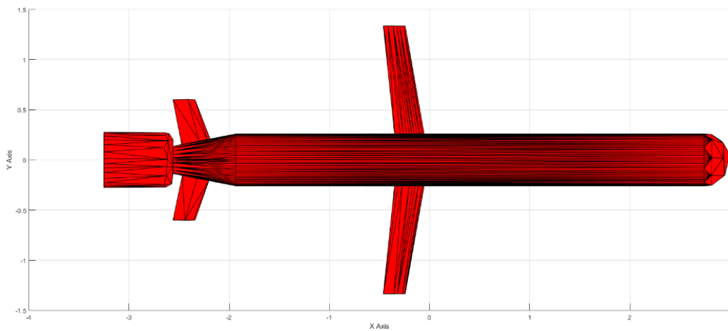
Figure 2.13: The Top View of the Cruise Missile with 1000 Triangles in Total
