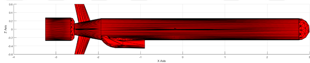
Figure 2.20: The Side View of the Cruise Missile with 2000 Triangles in Total
