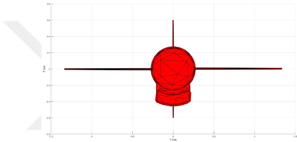
Figure 2.15: The Front View of the Cruise Missile with 1000 Triangles in Total
