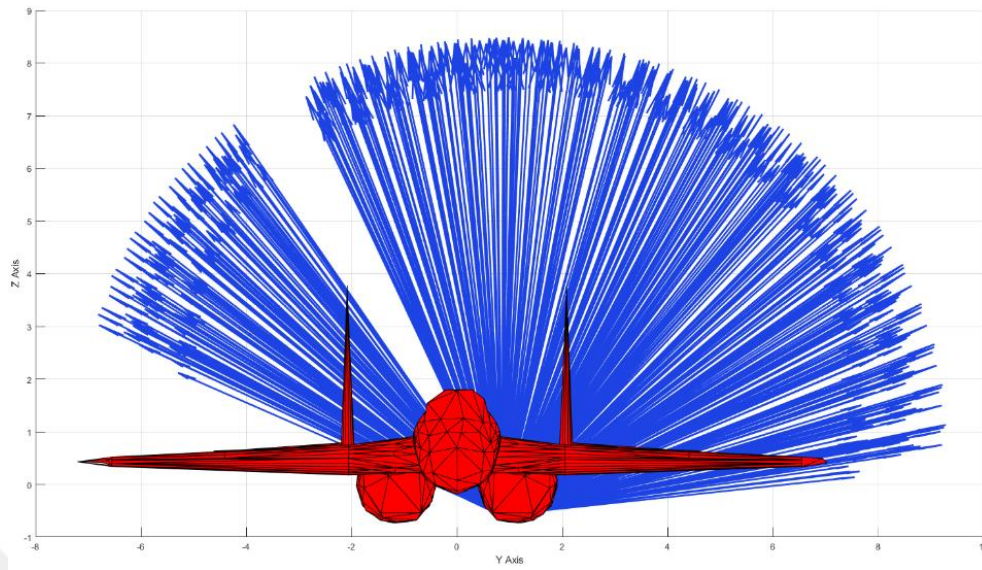
Figure 3.16: Scattering of Striking Fragments at Detonation Point 76 on YZ Axis for the 2 nd Scenario
