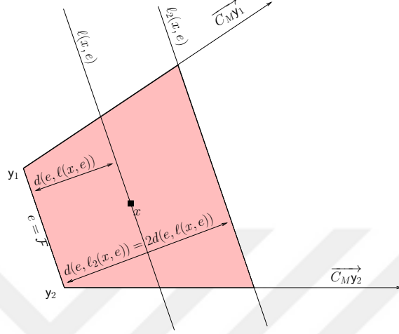
Figure 3.2: The proportional-edge proximity region, \mathcal{N}_{PE}(x, r = 2) (shaded), in an outer triangle \mathcal{F} \subseteq \mathbb{R}^2 .
