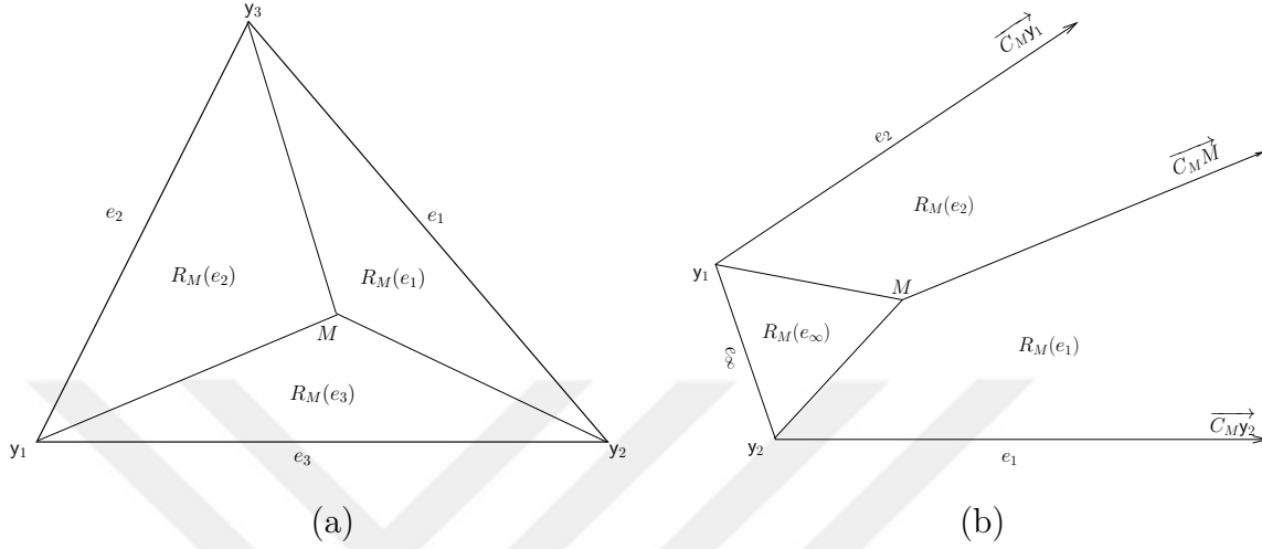
Figure 2.4: (a) Edge regions of an acute inner triangle T(\mathcal{Y}) = T(y_1, y_2, y_3) with a center M \in T^o . (b) Edge regions of an outer triangle T(\mathcal{Y}) = T(y_1, y_2) with a center M \in T^o .
