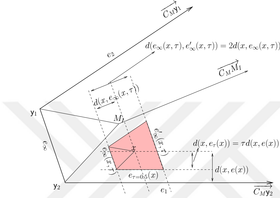
Figure 3.4: The central-similarity proximity region (shaded) of an outer simplex, N_{CS}(x, \tau = 0.5) in \mathbb{R}^2 .
