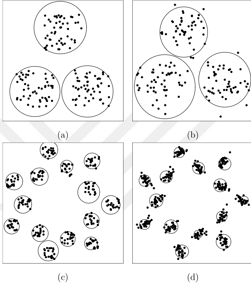
Figure 6.5: Four different settings with 3 or 14 classes, and the results of R-CCD algorithm. Each covering ball represents a cluster. (a) Three class setting with F_1 = U([0, 1]^2) , F_2 = U([3, 4] \times [0, 1]) and F_3 = U([0.5, 3.5] \times [3, 4]) . (b) Three class setting with F_1 = N(\mu_1, I_2) , F_2 = N(\mu_2, I_2) and F_3 = N(\mu_3, I_2) where \mu_1, \mu_2, \mu_3 \in \mathbb{R}^2 and I_2 is the identity matrix of size 2. (c) 14 classes where each are uniformly distributed in some square regions from \mathbb{R}^2 (d) 14 classes where each are normally distributed in \mathbb{R}^2 .
