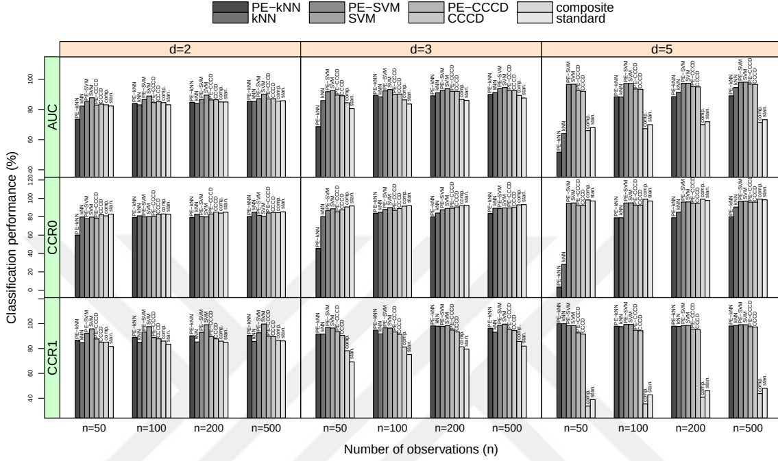
Figure 5.9: AUCs and CCRs of the two cover, three hybrid PE-PCD classifiers with expansion parameter r = 2.2 , and k -NN, SVM and CCCD classifiers. The composite covers are indicated with “comp.” and standard covers with “stan.”. Here, the classes are drawn as \mathcal{X}_0 \sim U([0, 1]^d) and \mathcal{X}_1 \sim U([0.3, 0.7]^d) with several simulation settings based on number of observations n = 50, 100, 200, 500 and dimensionality d = 2, 3, 5 .
