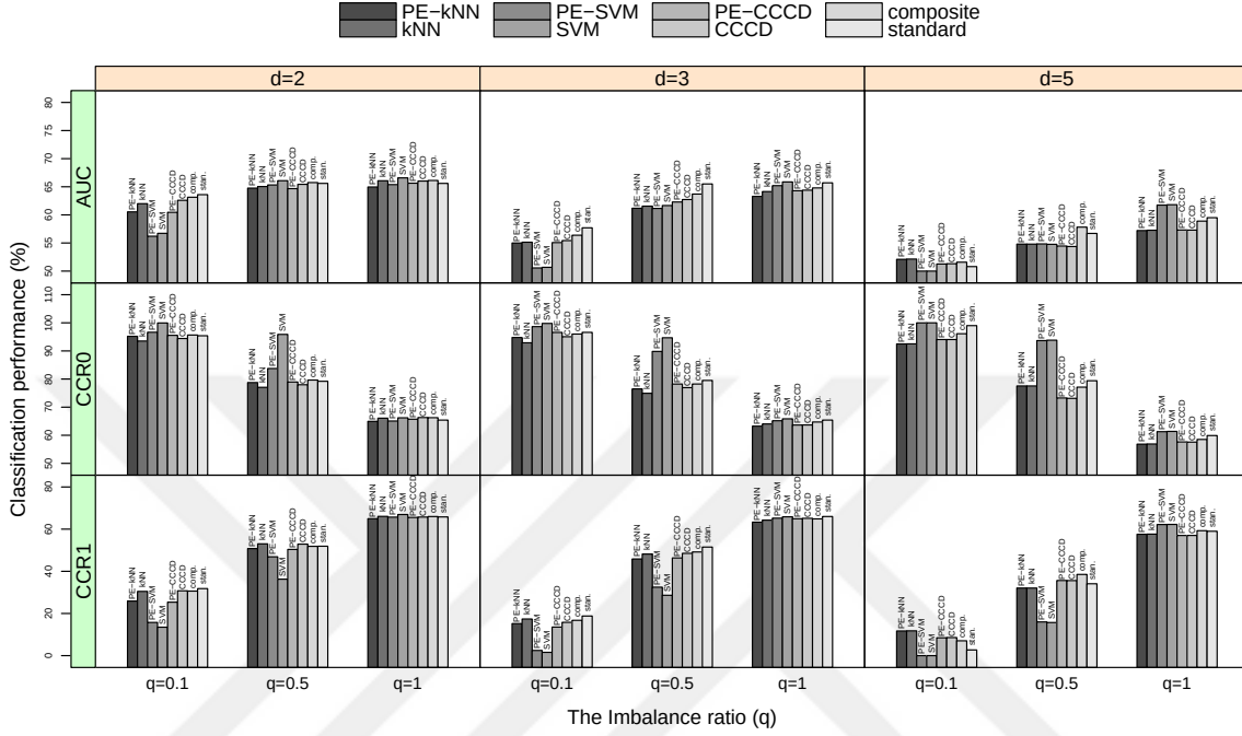
Figure 5.7: AUCs and CCRs of the two cover, three hybrid PE-PCD classifiers with expansion parameter r = 3 , and k -NN, SVM and CCCD classifiers. The composite covers are indicated with “comp.” and standard covers with “stan.”. Here, the classes are drawn as \mathcal{X}_0 \sim U([0, 1]^d) and \mathcal{X}_1 \sim U([\nu, 1 + \nu]^d) with several simulation settings based on \zeta = 0.5 , imbalance level q = 0.1, 0.5, 1 and dimensionality d = 2, 3, 5 .
