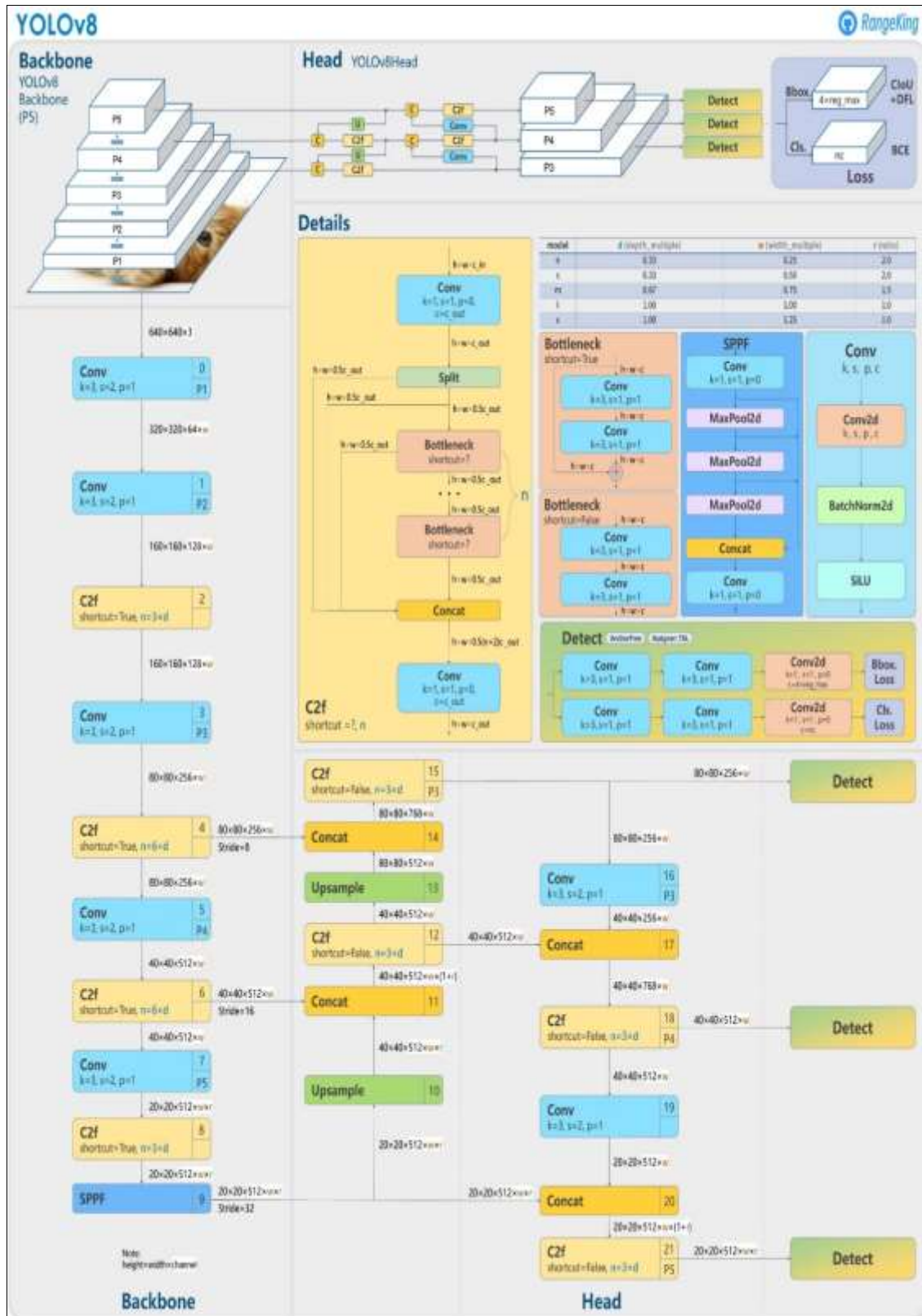
Figure 3.4: YOLOv8 Architecture.
