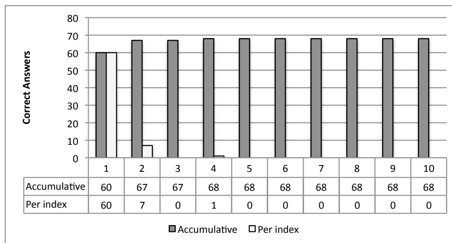
Figure 7.39: Correct answers returned by combining methods without answer type with answer re-ranking
