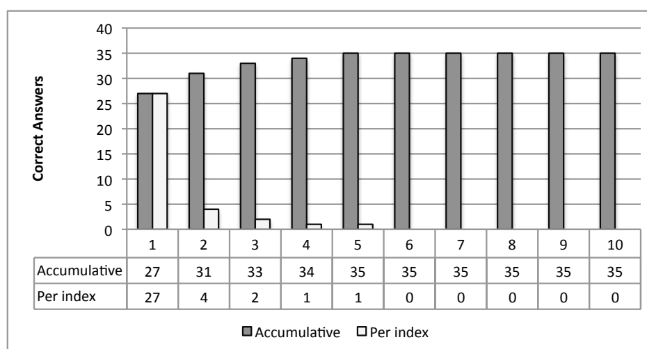
Figure 7.4: Correct answers returned by Stemmed String method
