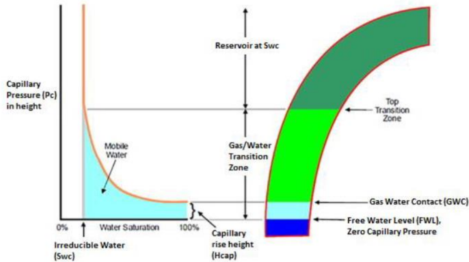
Figure 2: Typical capillary pressure curve (Malik, 2017)
