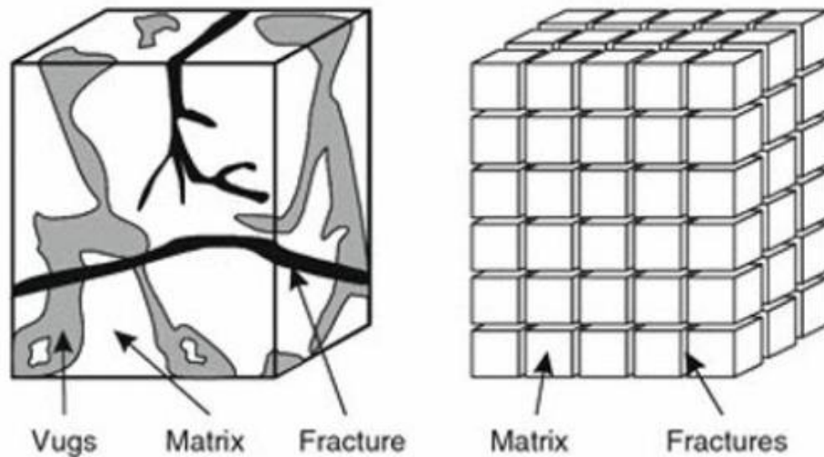
Figure 7: Dual-porosity, dual-permeability model(Warren & Root, 1963)
