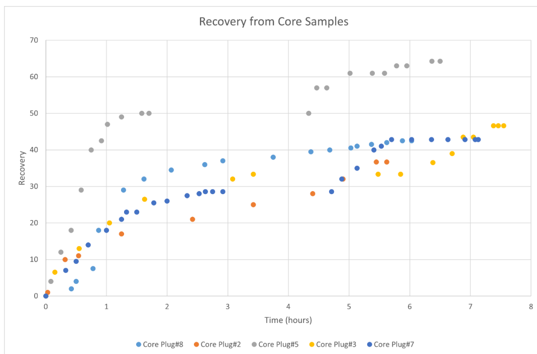
Figure 21: Recovery vs Time plot of core samples
