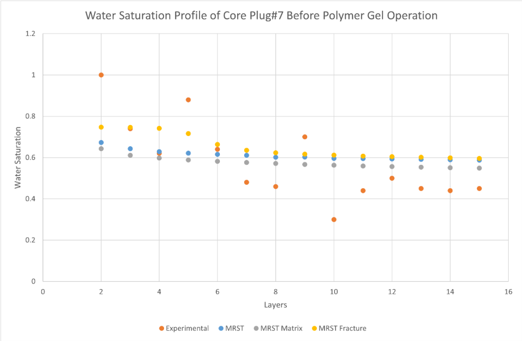
Figure 70: Water saturation profile of core plug#7 before polymer gel treatment
