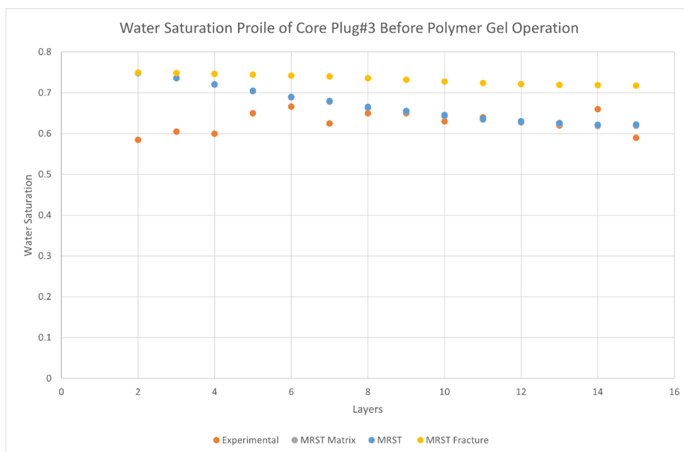
Figure 62: Water saturation profile of core plug#3 before polymer gel treatment
