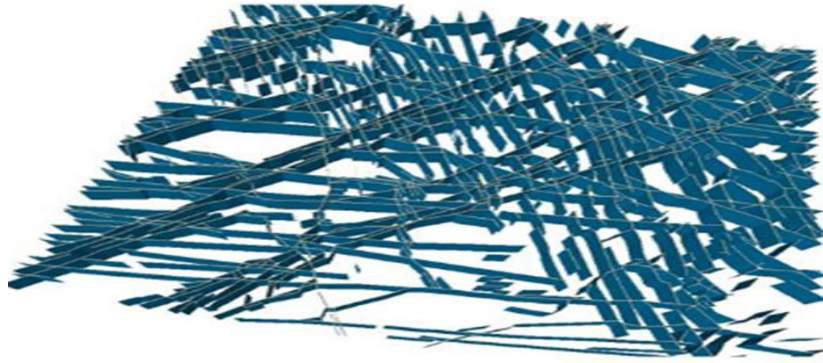
Figure 8: Discrete Fracture Model (DFM)
