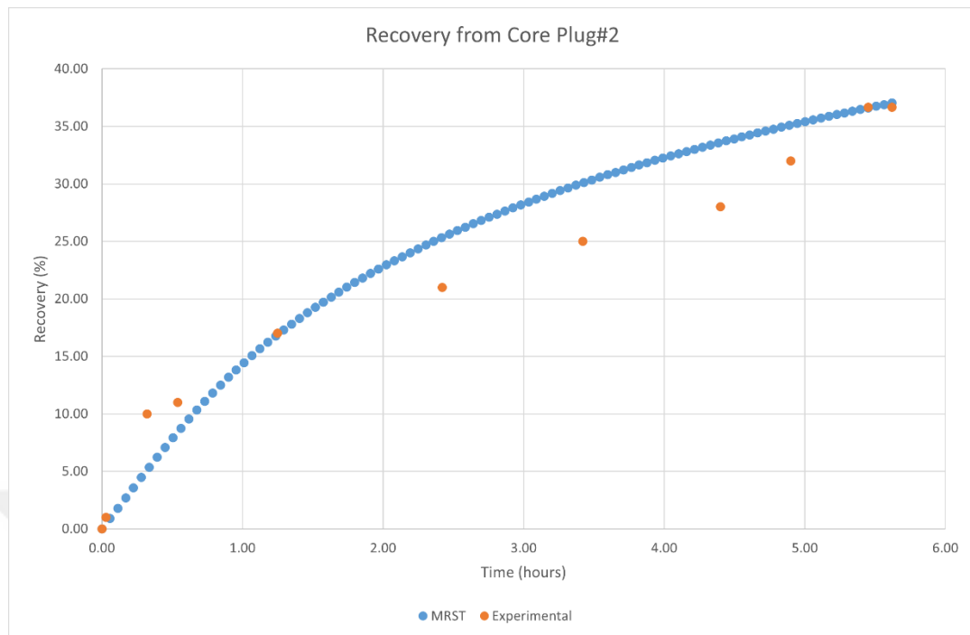
Figure 59: Recovery vs Time plot of core plug#2
