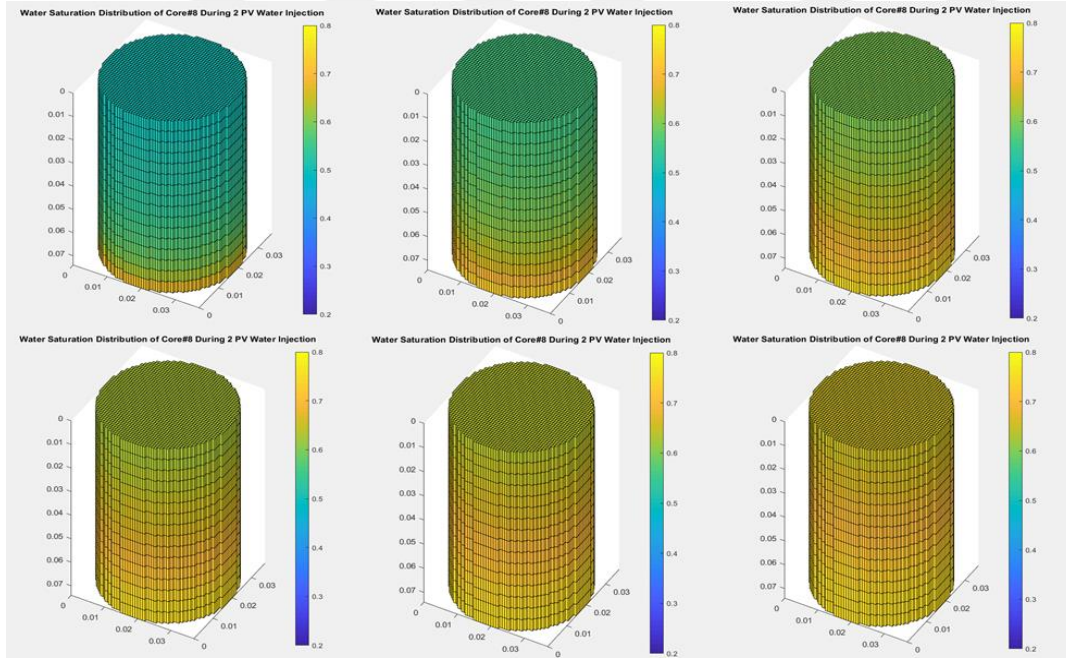
Figure 53: Water saturation distribution of core plug#8 (top left 0.2 PV, top middle 0.5 PV, top right 1 PV, bottom left 1.4 PV, bottom middle 1.7 PV and bottom right 2.0 PV)
