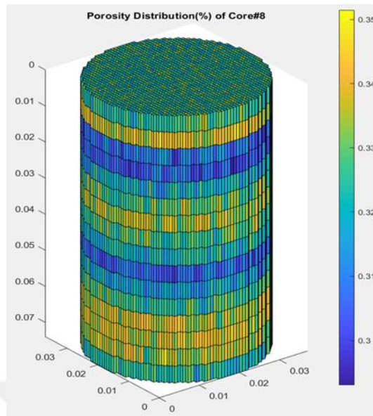
Figure 29: Porosity distribution of core plug#8
