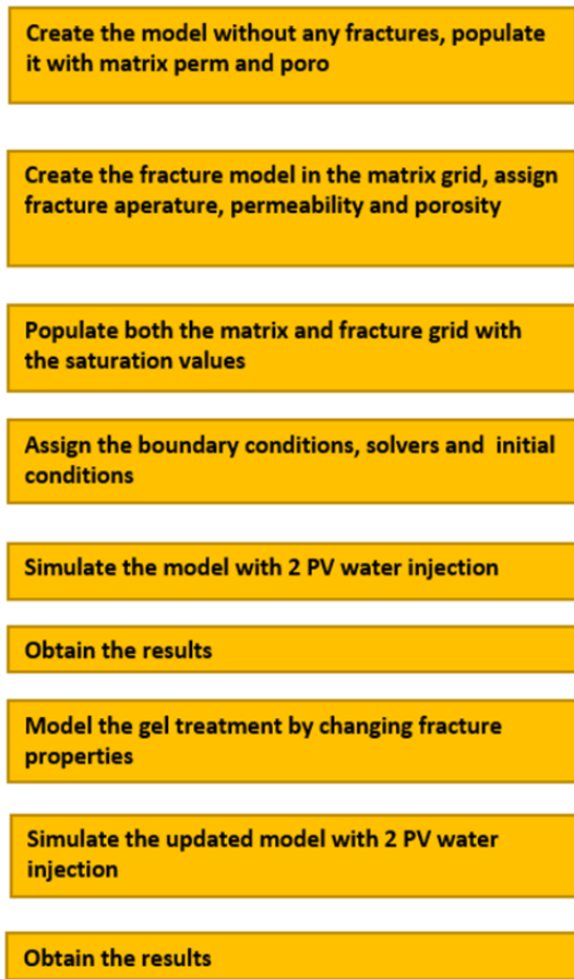
Figure 35: Procedure for fractured and gel-treated core plug modelling
