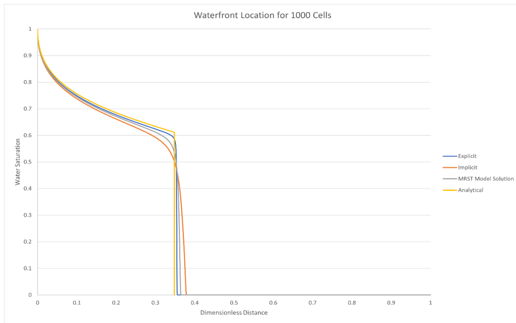
Figure 46: Waterfront location for different solution methods (1000 cells)
