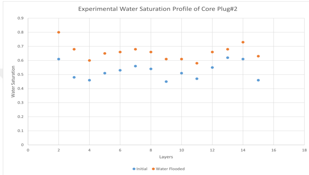
Figure 16: Experimental water saturation profile of core plug#2
