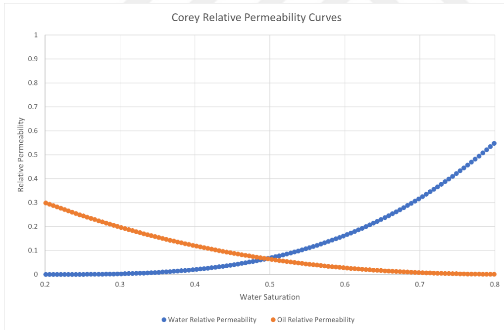
Figure 3: Corey type relative permeability curves
