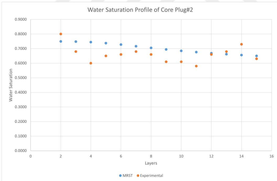
Figure 58: Water saturation profile of core plug#2
