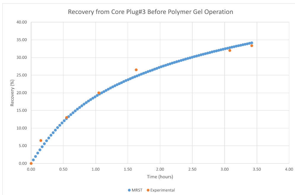
Figure 63: Recovery vs Time plot of core plug#3 before polymer gel treatment
