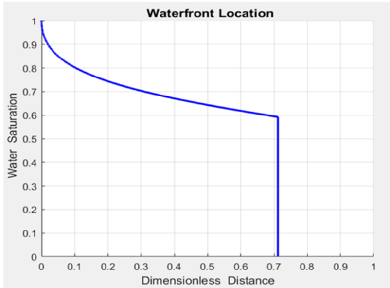
Figure 40: Analytical solution of the waterfront location
