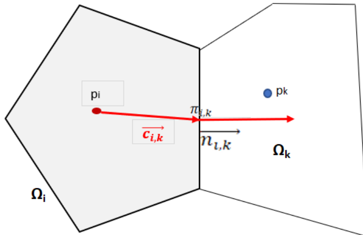
Figure 25: Schematic visualization of TPFA
