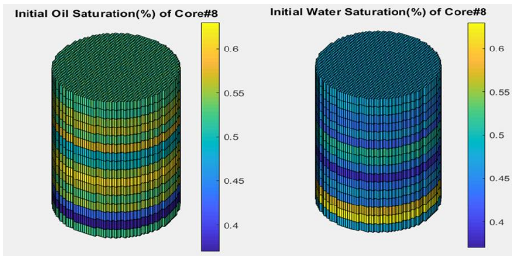
Figure 31: Initial oil and water saturation distributions for core plug#8
