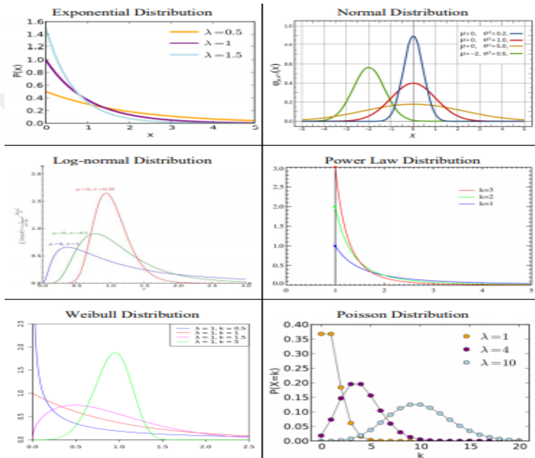
Figure 11: PDF's for different distribution methods (Shiriyev, 2013)
