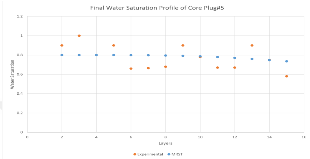
Figure 82: Final water saturation profile of core plug#5
