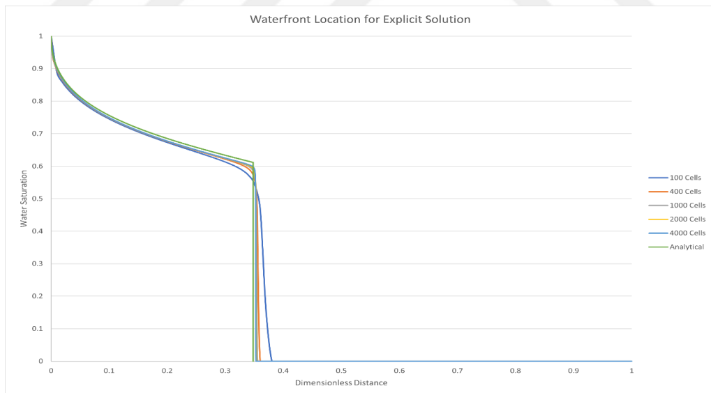
Figure 49: Waterfront location for explicit solution vs analytical solution for different cell numbers
