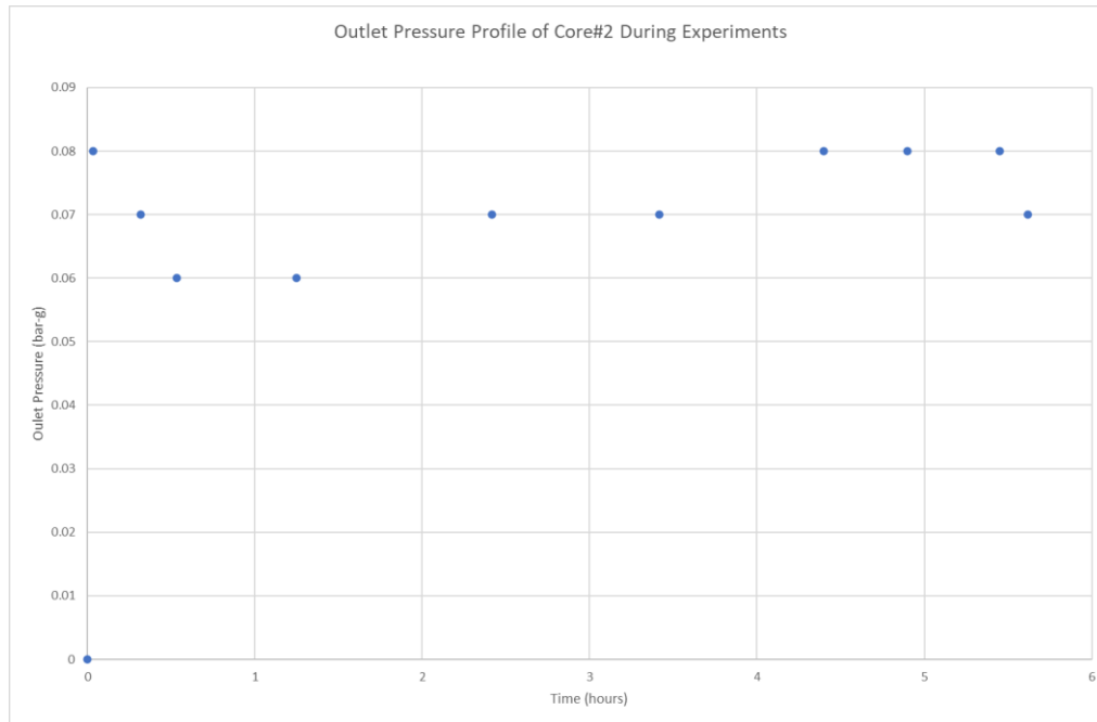
Figure 15: Outlet pressure profile of core plug#2
