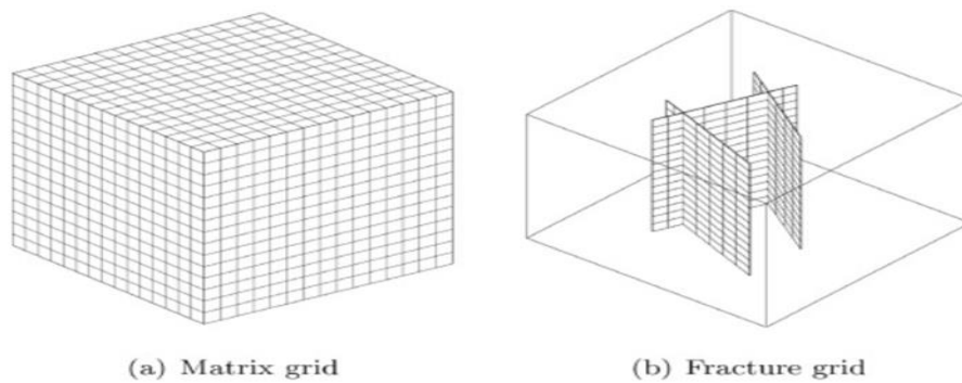
Figure 10: Embedded Discrete Fracture Model (EDFM) (Tene et al., 2017)
