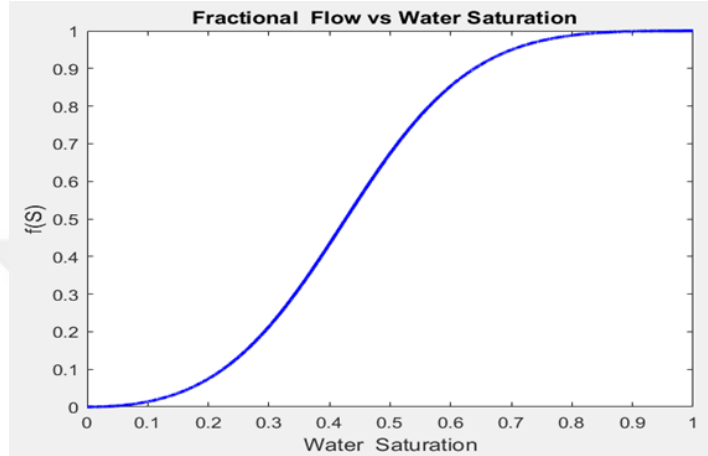
Figure 38: Water saturation vs fractional flow
