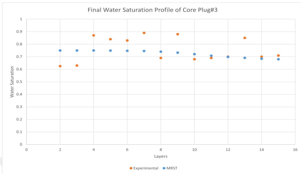
Figure 66: Final water saturation profile of core plug#3 after polymer gel treatment
