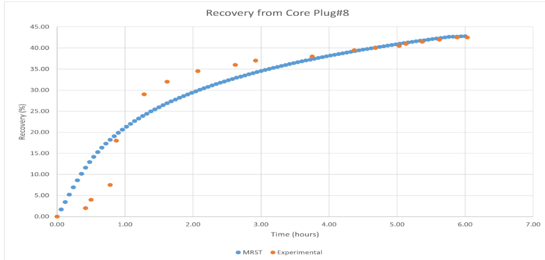
Figure 55: Recovery vs Time plot of core plug#8
