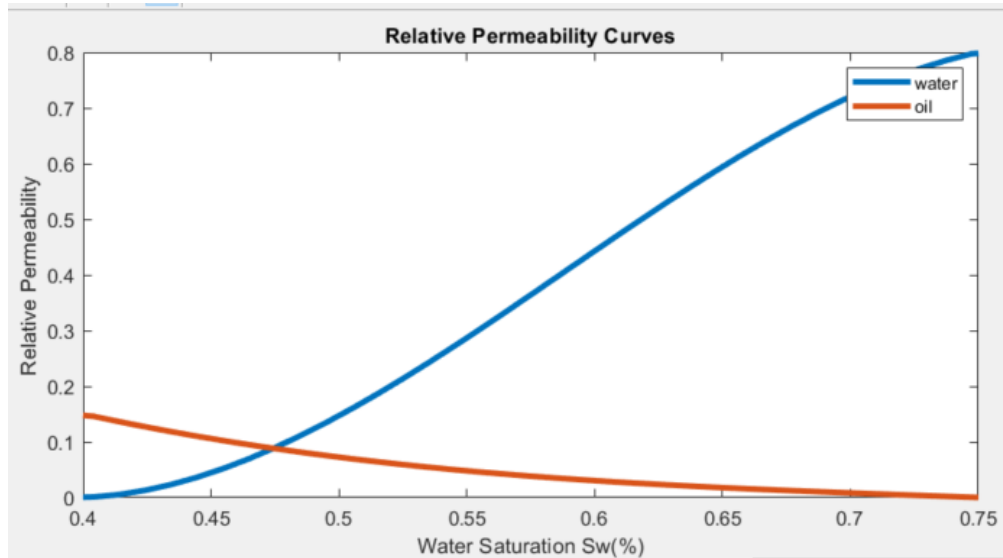
Figure 30: Relative permeability curves for the core plug#8
