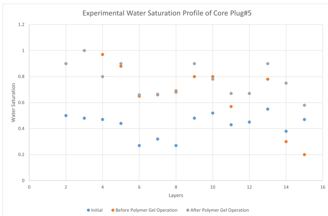
Figure 18:Experimental water saturation profile of core plug#5
