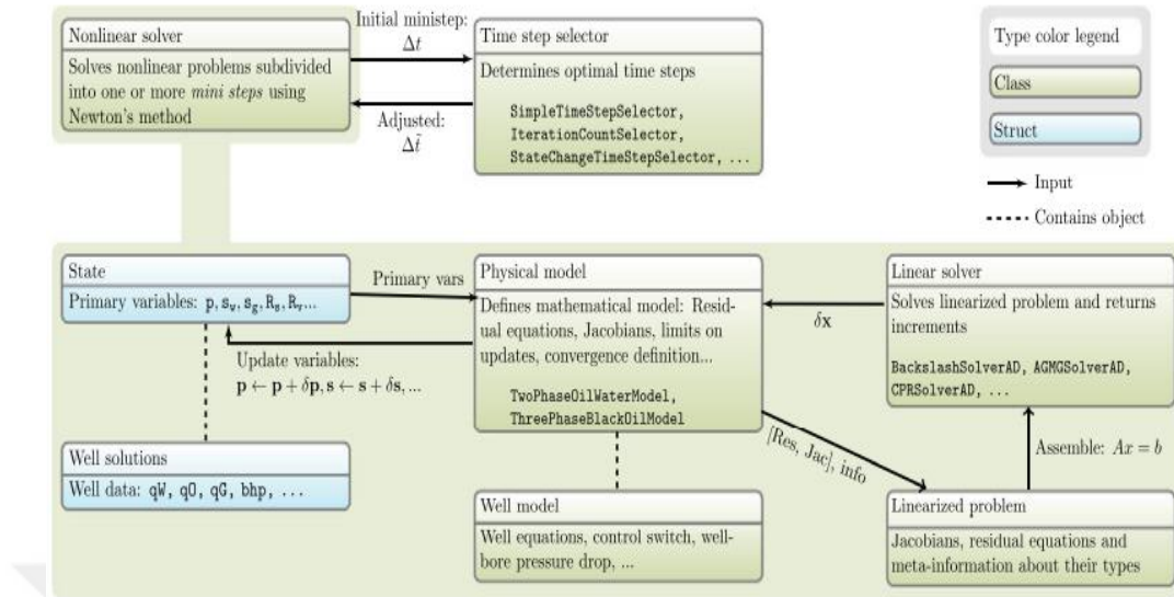
Figure 24: Mini-step solution procedure of AD (Lie, 2019)
