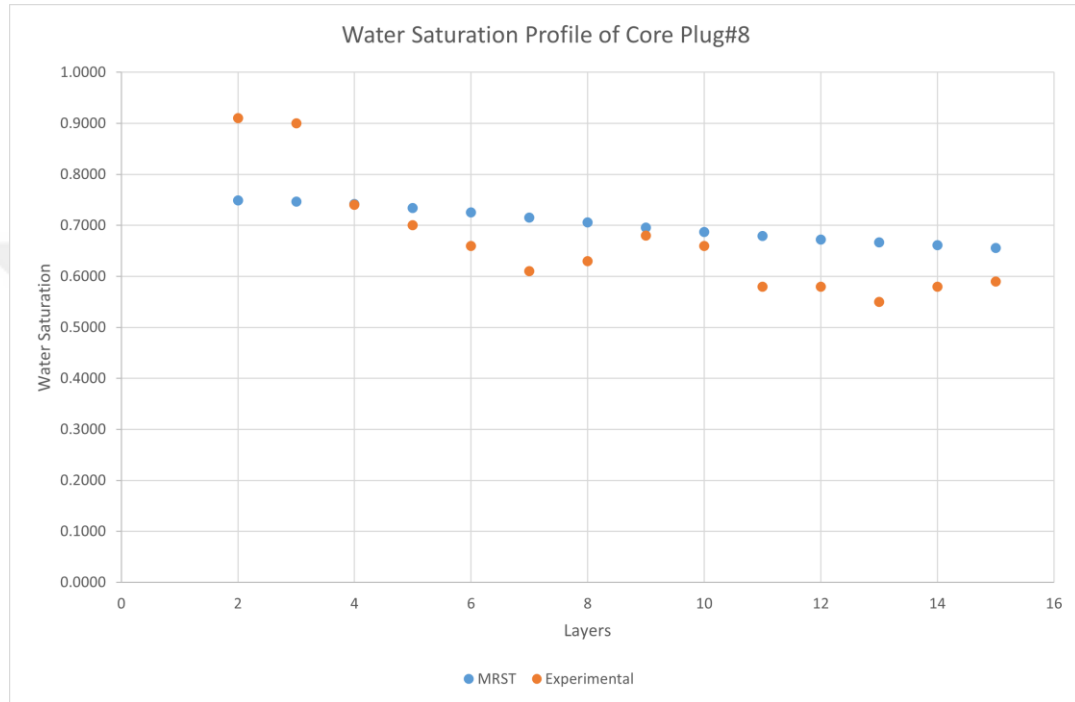
Figure 54: Water saturation profile of core plug#8
