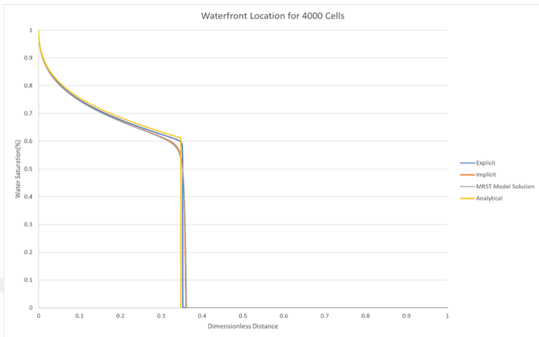
Figure 44: Waterfront location for different solution methods (4000 cells)
