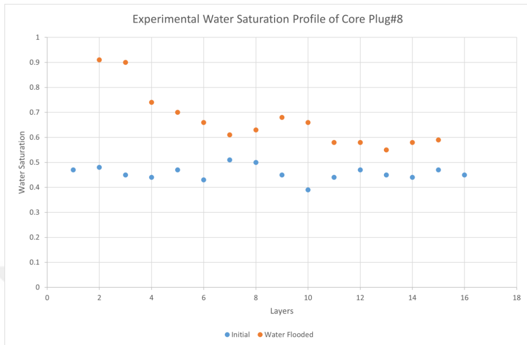
Figure 20: Experimental water saturation profile of core plug#8
