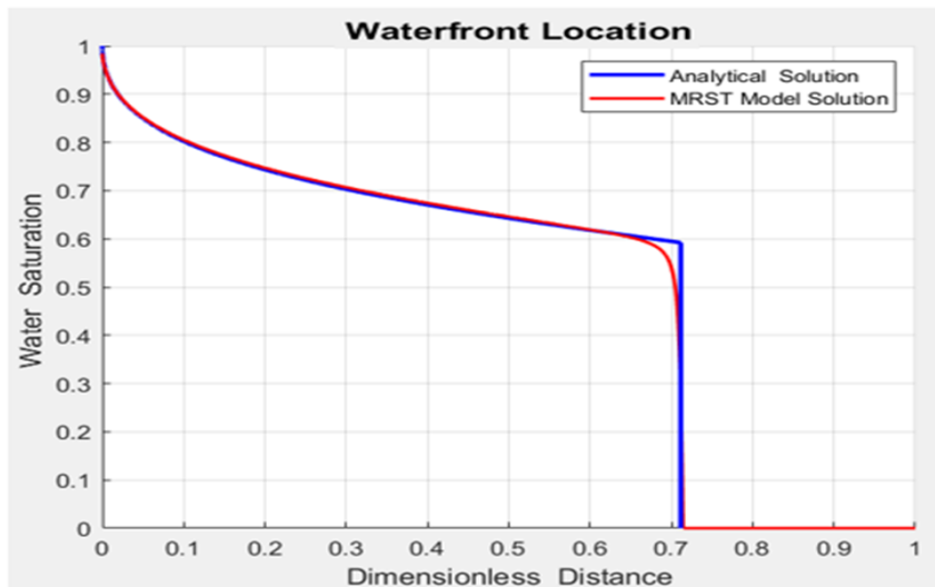
Figure 41: Comparison of the analytical and MRST model solution
