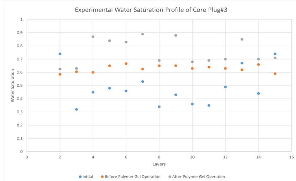
Figure 17: Experimental water saturation profile of core plug#3
