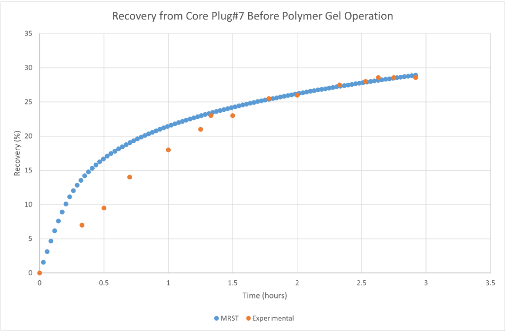
Figure 71: Recovery vs Time plot of core plug#7 before polymer gel treatment
