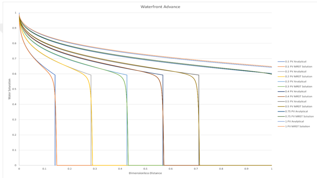
Figure 42: Overall comparison of analytical and MRST solution for the waterfront advance
