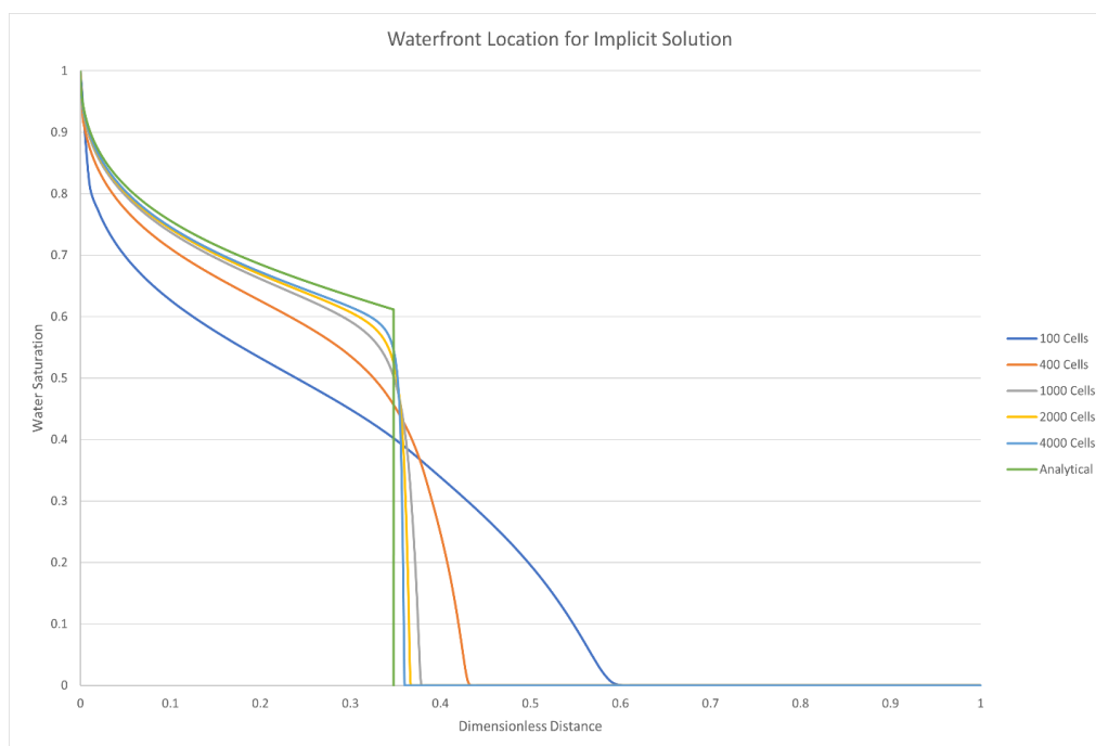
Figure 50: Waterfront location for implicit solution vs analytical solution for different cell numbers
