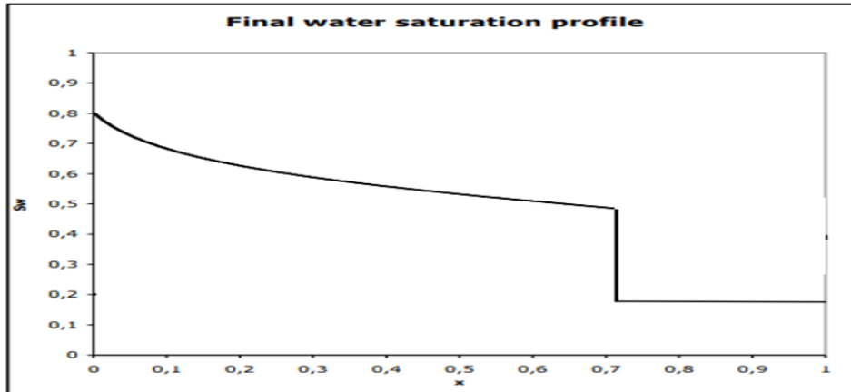
Figure 37: Typical frontal advance profile for waterflooding
