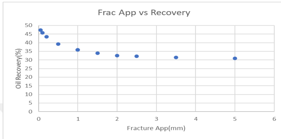
Figure 84: Change in oil recovery for different fracture aperture values when fracture permeability is constant
