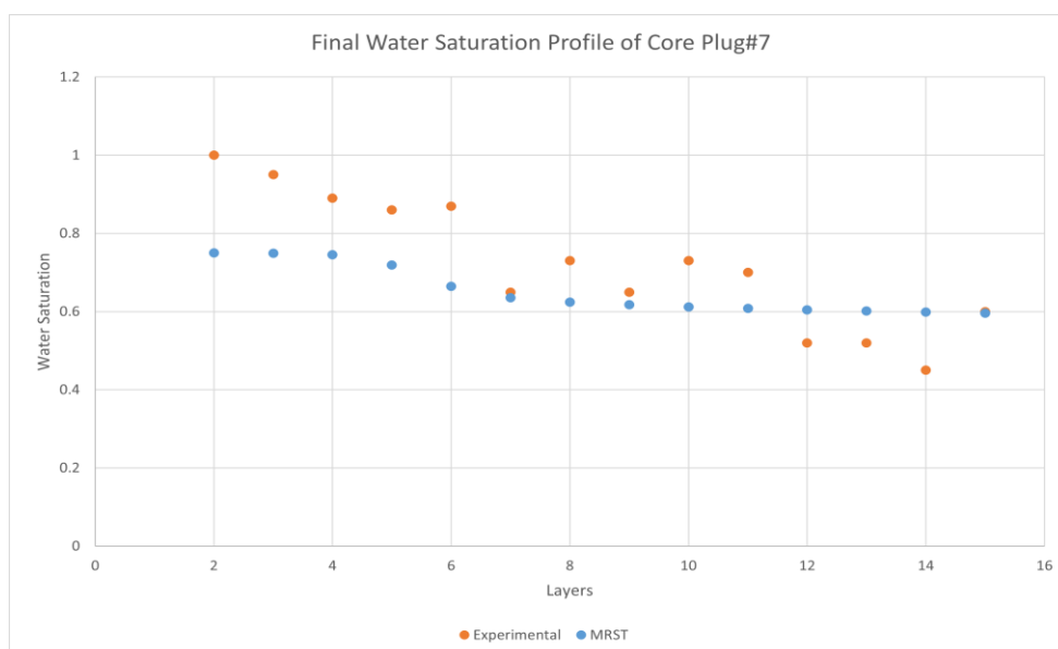
Figure 74: Water saturation profile of core plug#7 after polymer gel treatment
