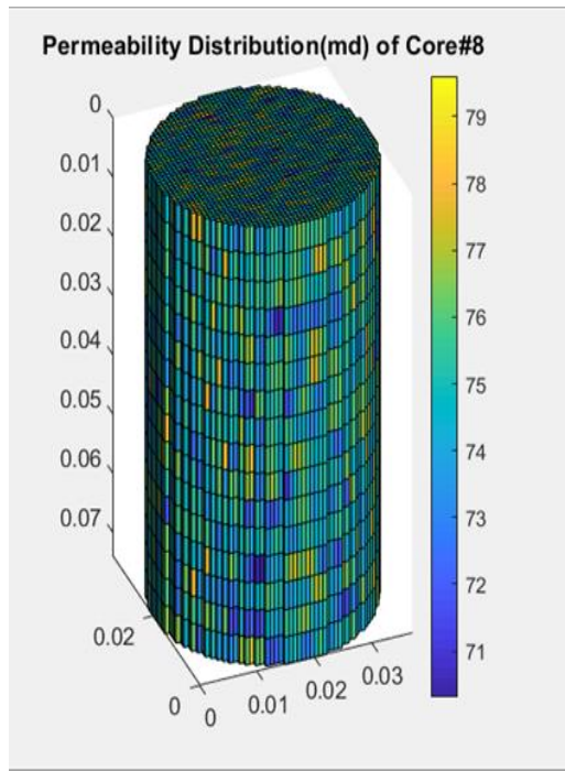
Figure 28: Permeability distribution of core plug#8
