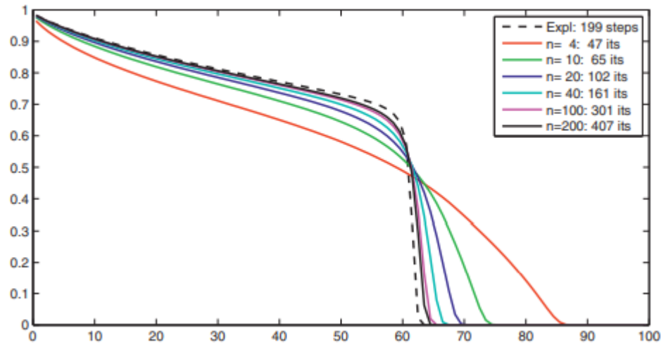
Figure 43: Approximate solutions computed by the explicit transport solver and the implicit transport solver with n time steps
