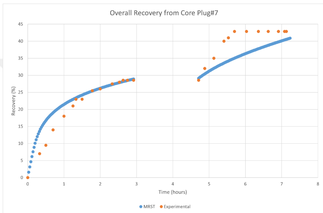
Figure 75: Overall recovery vs time plot of core plug#7
