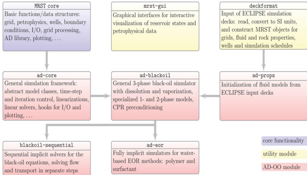
Figure 23: General framework of MRST (Lie, 2019)
