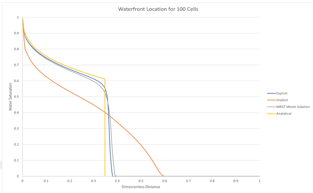
Figure 48: Waterfront location for different solution methods (100 cells)
