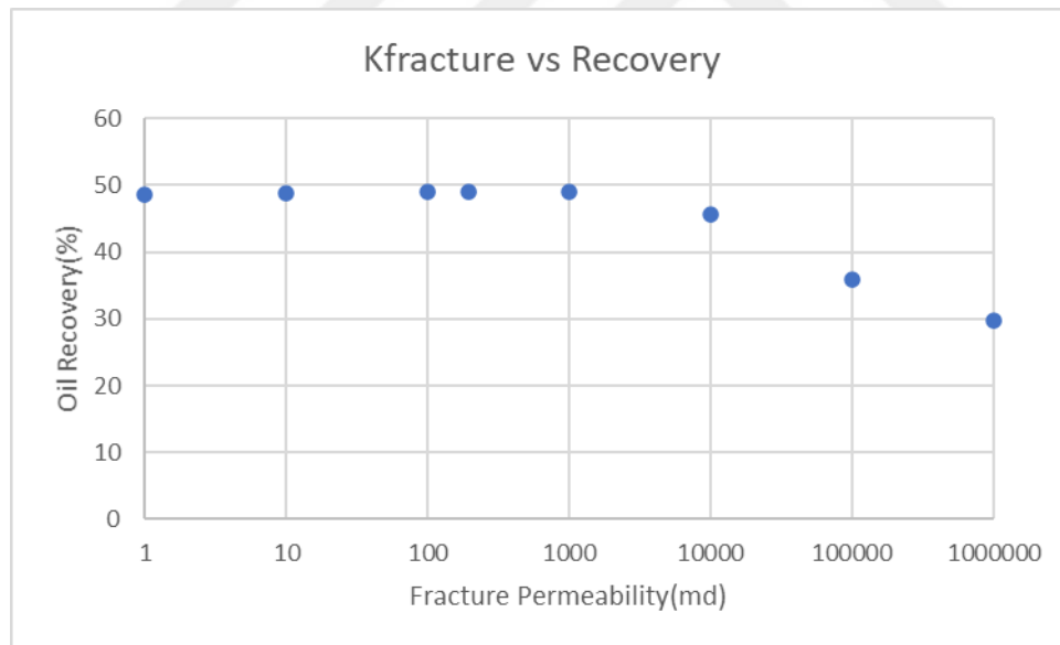
Figure 85: Change in oil recovery for different fracture permeability values when fracture aperture is constant
