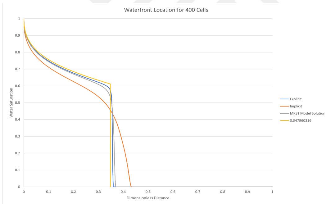
Figure 47: Waterfront location for different solution methods (400 cells)
