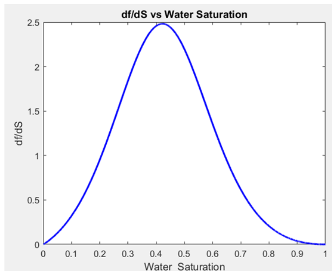
Figure 39: Derivative term vs water saturation
