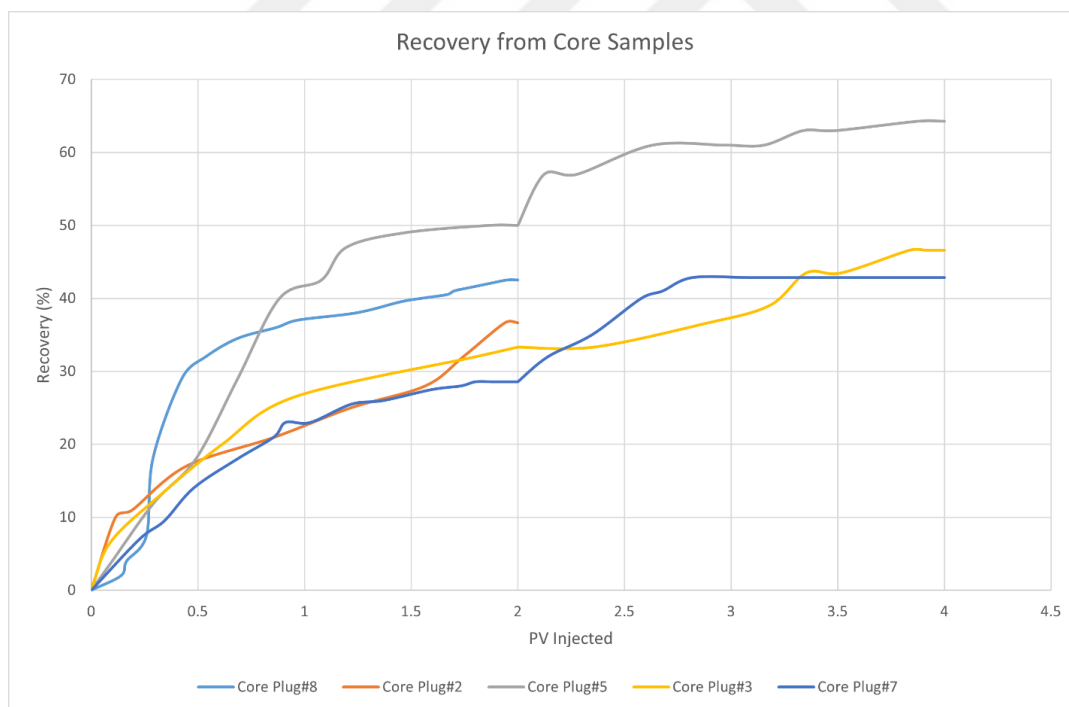
Figure 22: Recovery vs PV Injected plot of core samples
