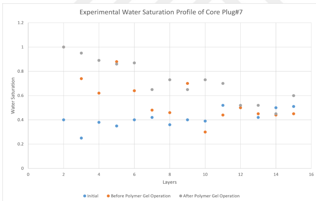
Figure 19:Experimental water saturation profile of core plug#7
