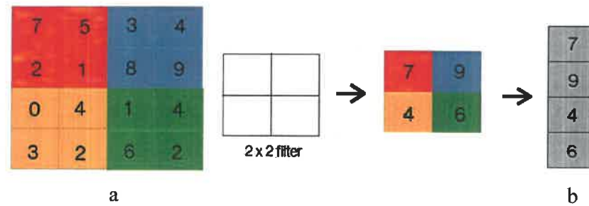
Figure 3.7. Max pooling (a) and Flatting (b) process
