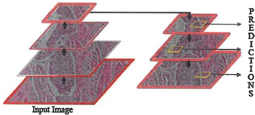
Figure 3.22. b. FPN Architecture
