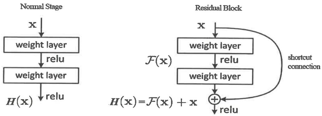
Figure 3.11. Representation of residual block (Adapted from He et al. 2016)
