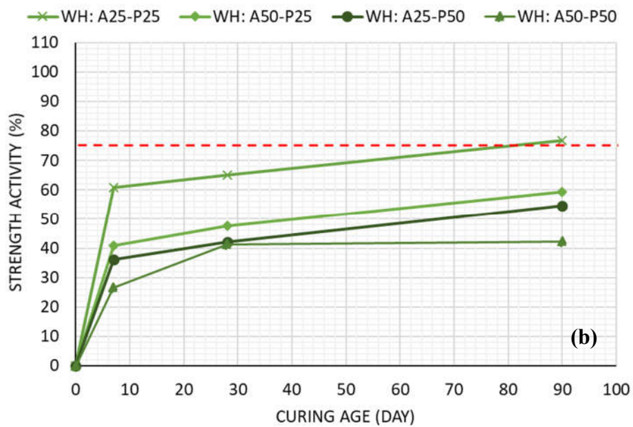
Figure 4.18 Compressive Strength Evolution vs. Age for Combined Usage Mortars with DHBA (a) and WHBA (b)
