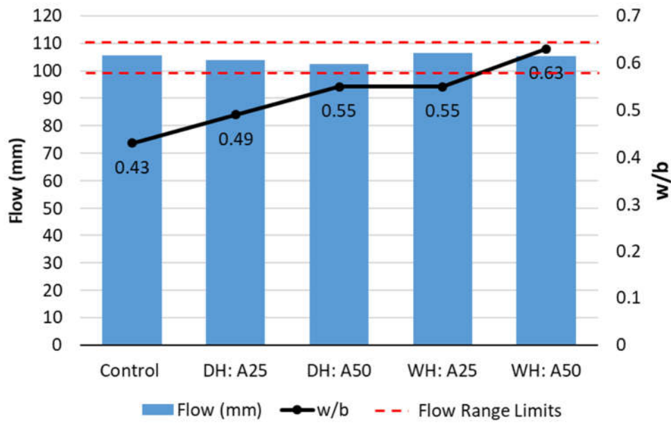
Figure 4.5 Flow and w/b for the Mechanical Test Mortars of Usage as FA
