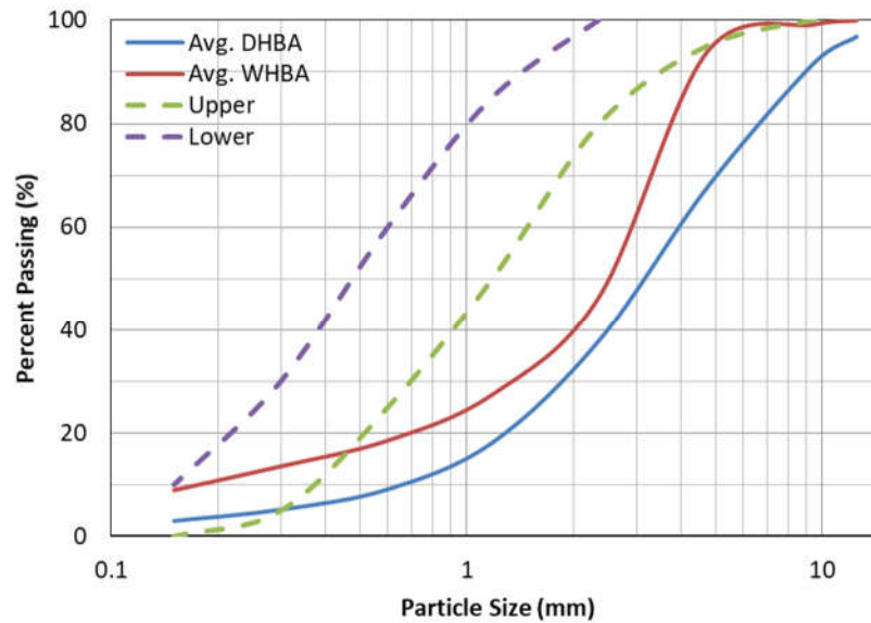
Figure 3.12. PSD of the as-is DHBA and WHBA (Upper and Lower Limit Zones [55])
