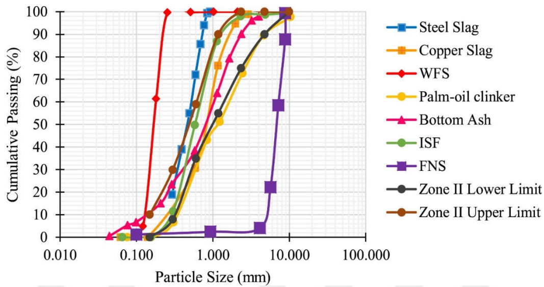
Figure 2.5. Particle Size Distribution of Industrial By-Products [18] (WFS: Waste Foundry Sand, ISF: Imperial Smelting Furnace, FNS: Ferro-Nickel Slag, Zone Limits Refer to IS 383-2016)
