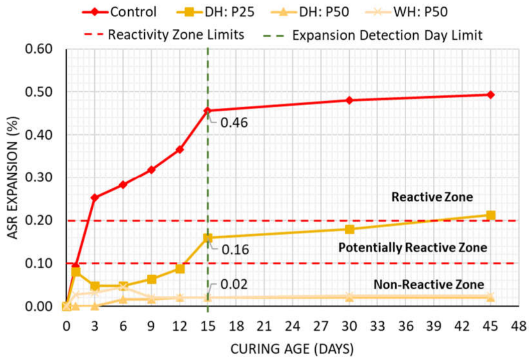
Figure 4.24 ASR Expansions of Usage as SCM Mortars.
