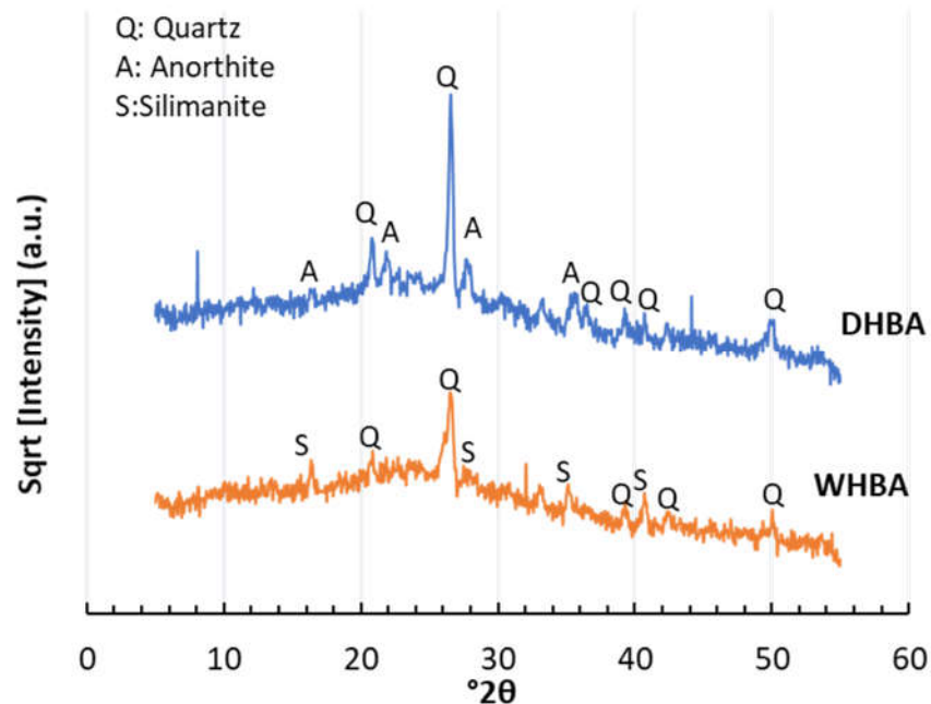
Figure 3.3. XRD Pattern of DHBA and WHBA Ashes
