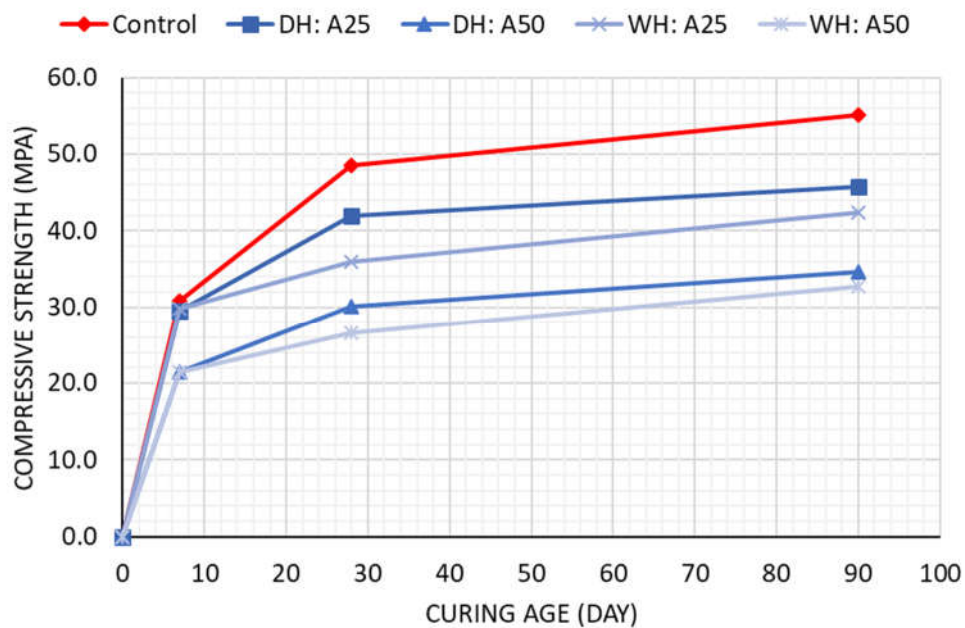
Figure 4.13 Compressive Strength vs. Age of Usage as FA Mortars
