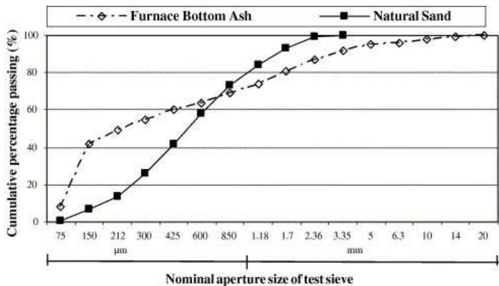
Figure 2.6. Comparison of the Particle Distribution of FBA and Natural Sand [25]
