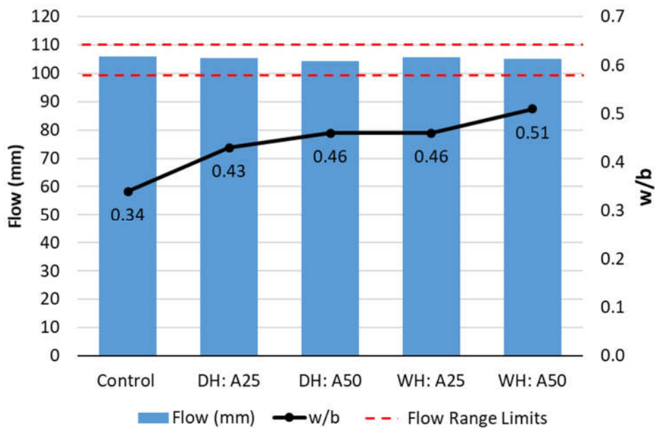
Figure 4.6 Flow and w/b for the Durability Test Mortars of Usage as FA
