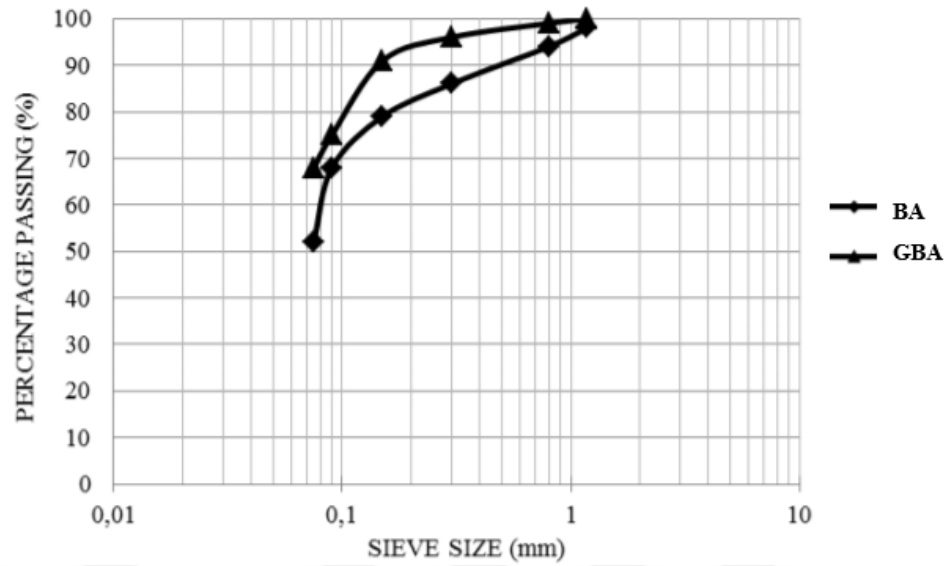
Figure 2.7. Comparison of the PSD as-is Bottom Ash, BA, and Ground Bottom Ash, GBA [41]
