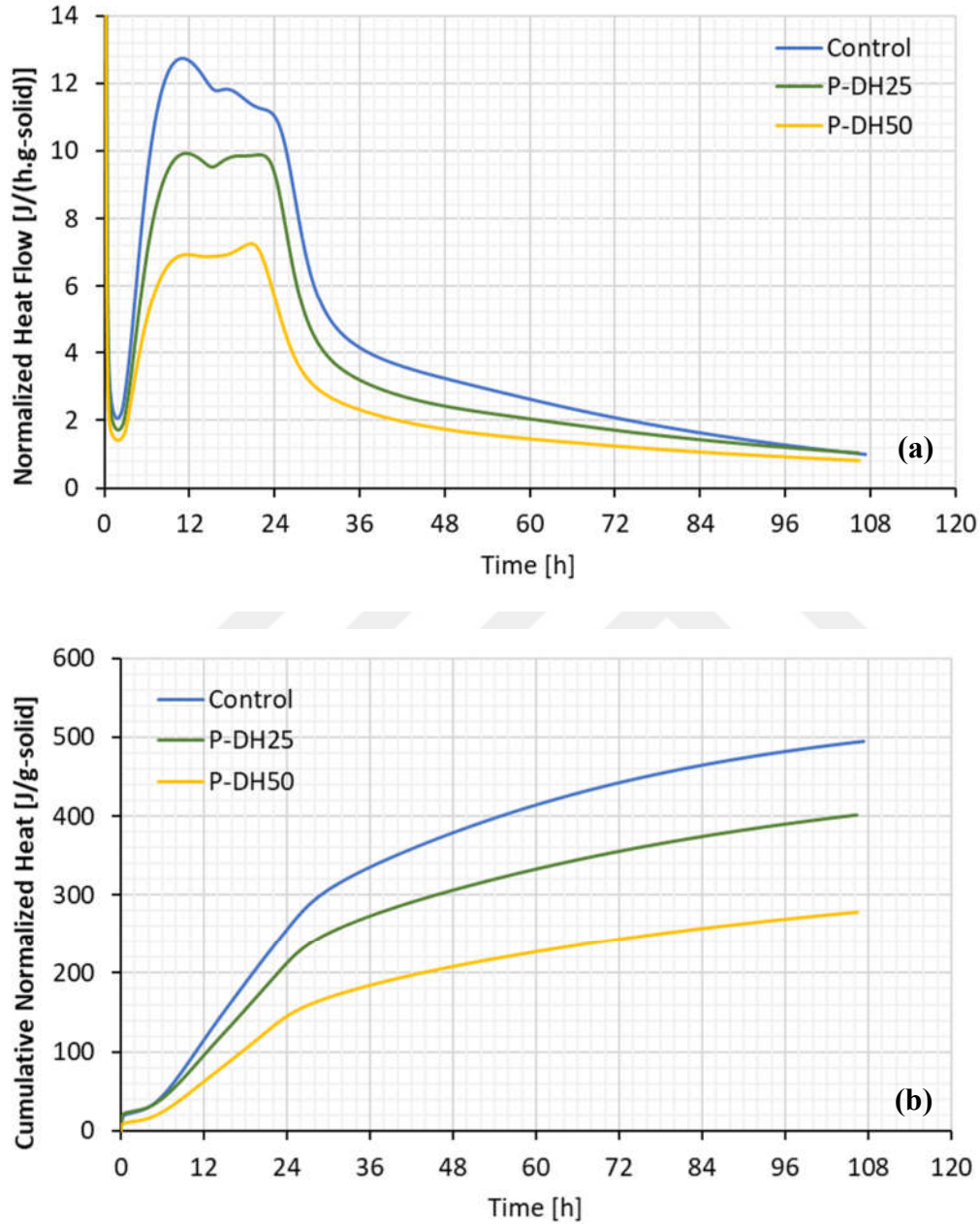
Figure 4.1 Hydration Heat of Control and P-DH25 & P-DH50 Pastes (a) Hydration Heat Evolution Rate, (b) Cumulative Hydration Heat / Solid
