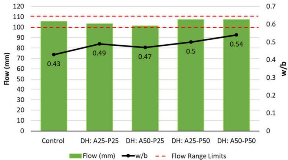
Figure 4.9 Flow and w/b for the Mechanical Test Mortars (DHBA) of Combined Usage
