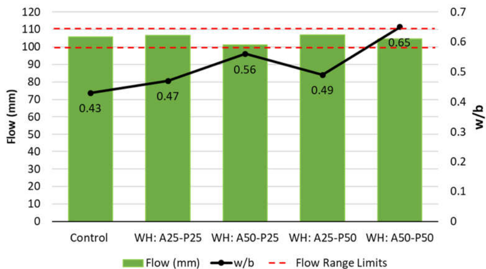
Figure 4.11 Flow and w/b for the Mechanical Test Mortars (WHBA) of Combined Usage
