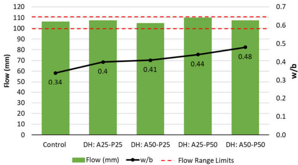
Figure 4.10 Flow and w/b of the Durability Test Mortars (DHBA) of Combined Usage
