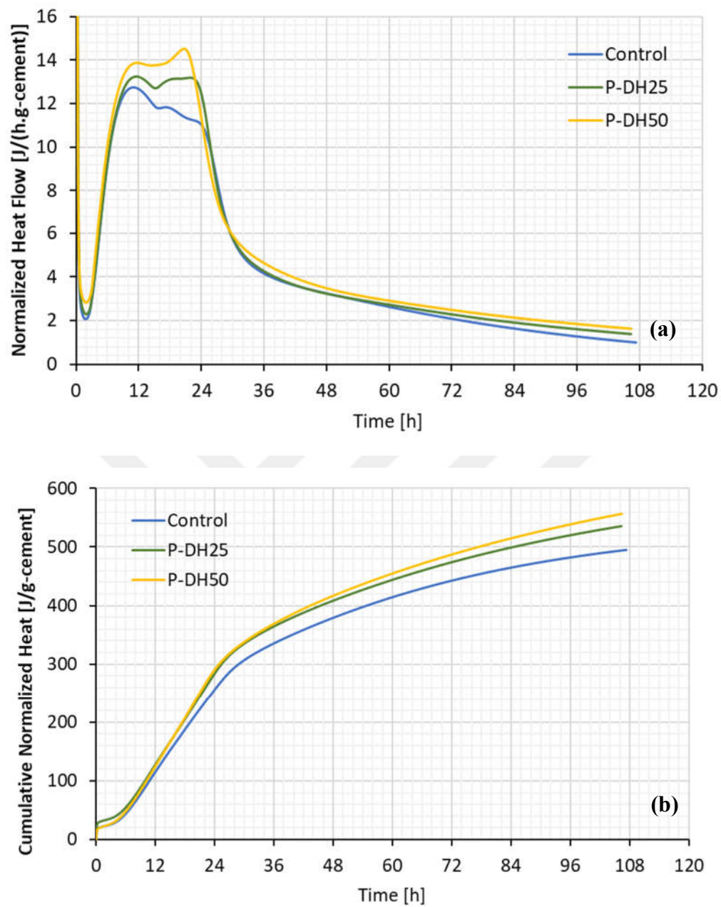
Figure 4.3 Hydration Heat of Control and P-DH25 & P-DH50 Pastes (a) Hydration Heat Evolution Rate, (b) Cumulative Hydration Heat / Cement
