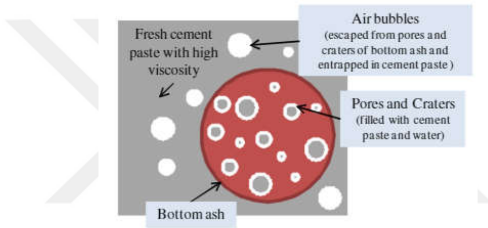
Figure 2.9. Generation of Air Bubbles in Cement Paste [44]
