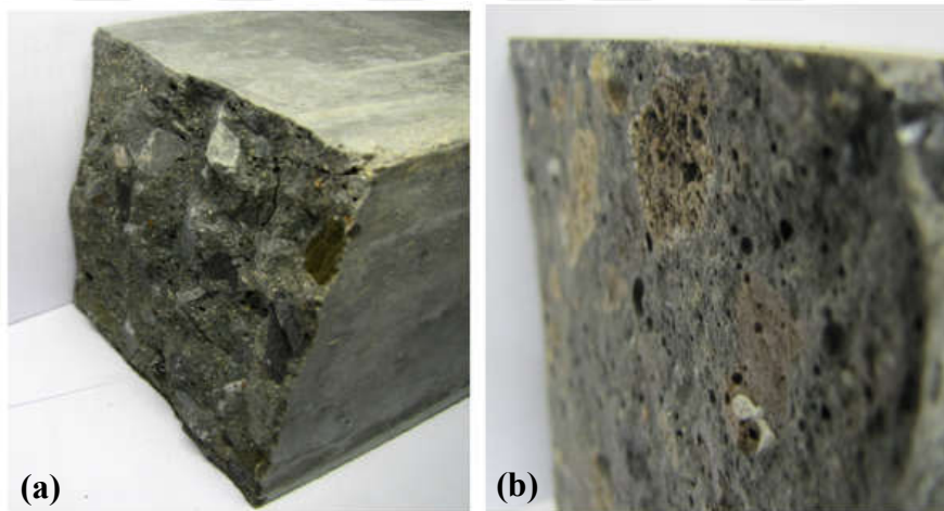
Figure 2.12. Fracture Sections of High-Strength Concrete with Normal (a) and Bottom Ash (b) Aggregates [44]
