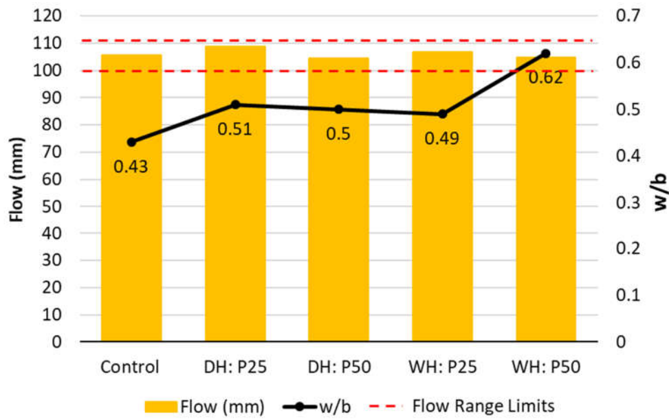
Figure 4.7 Flow and w/b of the Mechanical Test Mortars of Usage as SCM
