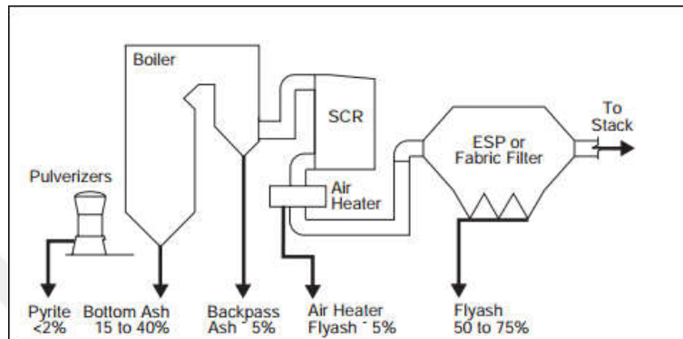
Figure 2.1. Typical Pulverized Coal-Fired Boiler Ash Discharge Locations and Approximate Amounts [11]
