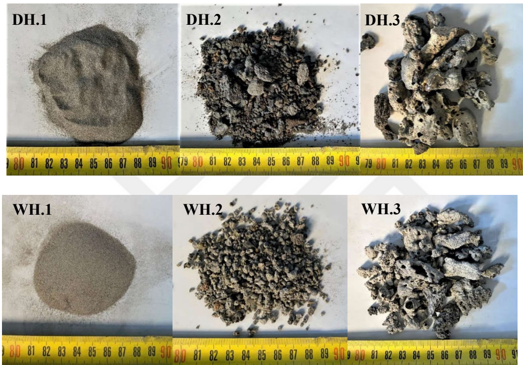
Figure 3.11. Different Size of DHBA (DH.1, DH.2 and DH.3) and WHBA (WH.1, WH.2 and WH.3) as-is Conditions
