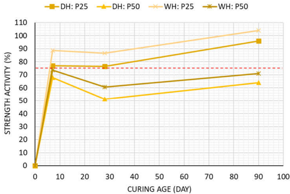
Figure 4.16 Compressive Strength Evolution vs. Age of Usage as SCM Mortars
