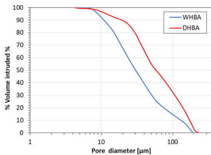
Figure 3.10. Volume vs. Pore Diameter Distributions of BAs
