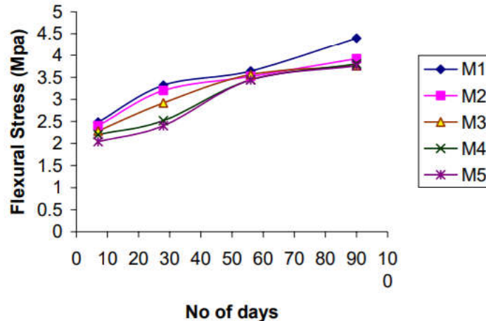
Figure 2.13. Effect of Bottom Ashes on the Flexural Strength [36]
