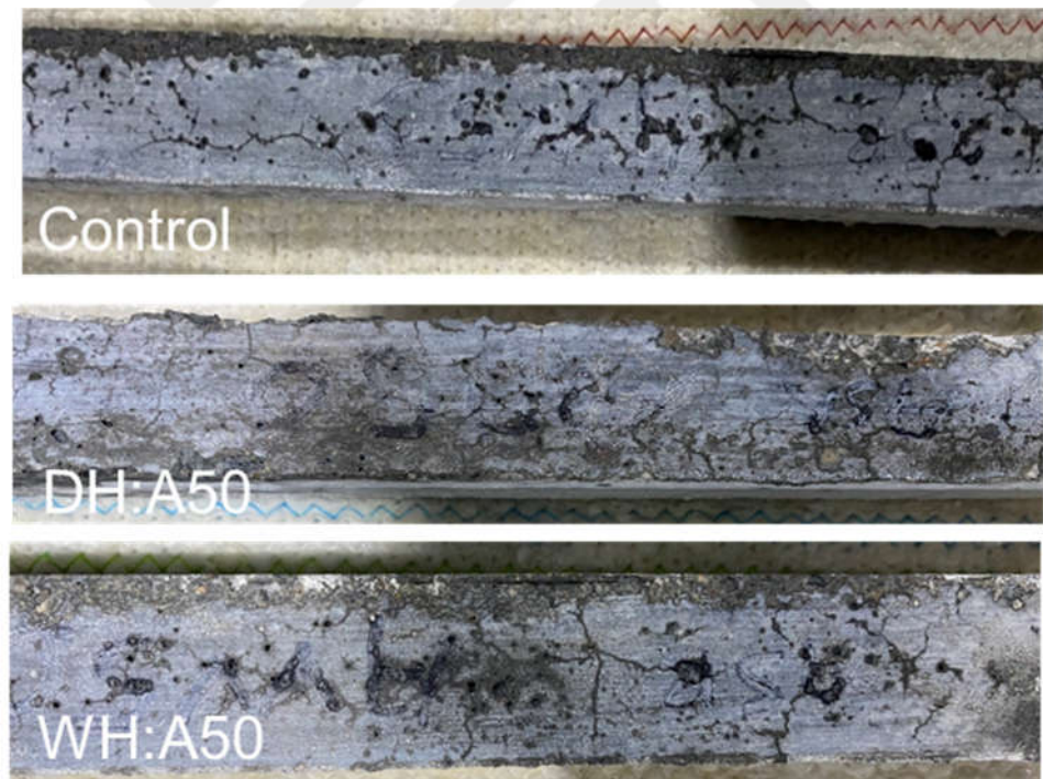
Figure 4.23 ASR Map Cracking Formation on Control, DH: A50 & WH: A50
