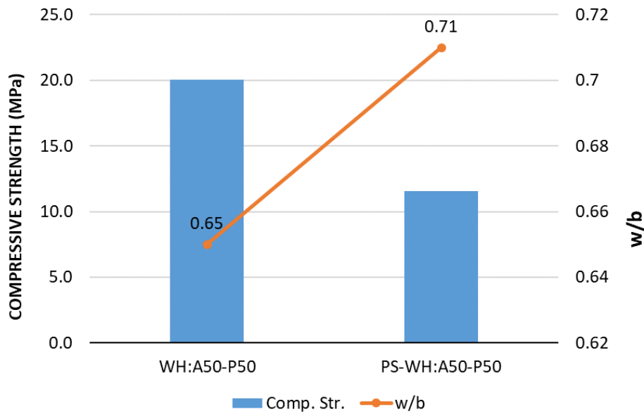
Figure 3.17 Comparison of the WH: A50-P50 Mixture and Pre-Soaking
