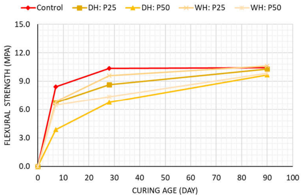
Figure 4.20 Flexural Strength Evolution vs. Age of Usage as SCM Mortars
