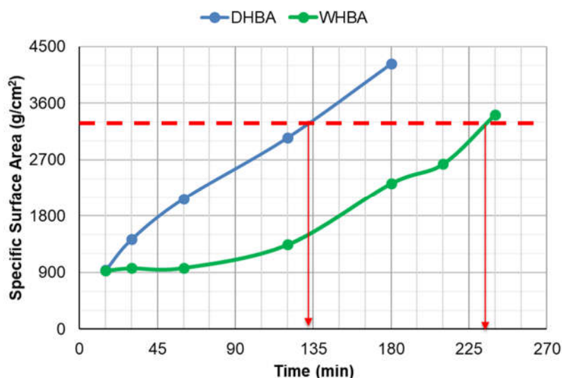
Figure 3.16. SSA vs. Grinding Time Graph of the both DHBA & WHBA
