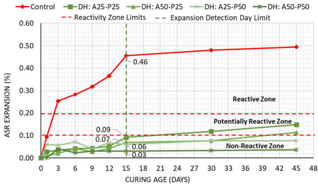
Figure 4.25 ASR Expansions of Combined Usage with DHBA Mortars
