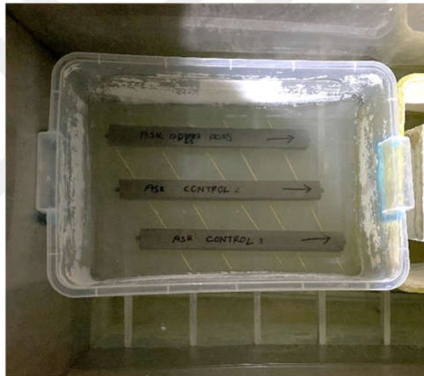
Figure 3.20 Oven Curing at 80°C with NaOH Solution of The Specimens
