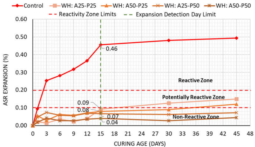
Figure 4.26 ASR Expansions of Combined Usage with WHBA Mortars
