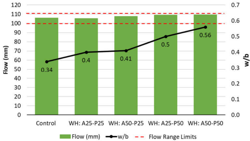
Figure 4.12 Flow and w/b for the Durability Test Mortars (WHBA) of Combined Usage
