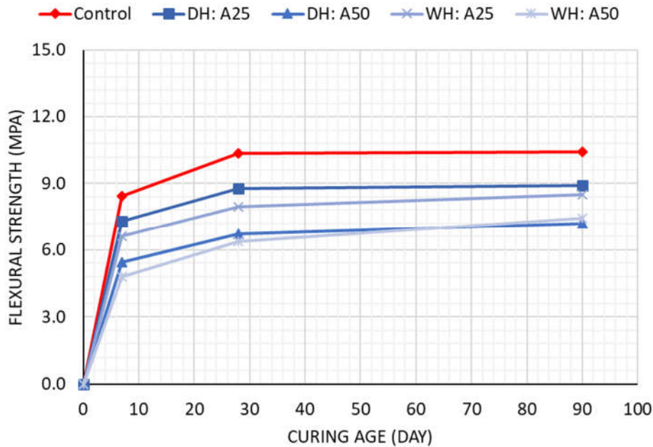
Figure 4.19 Flexural Strength Evolution vs. Age of Usage as FA Mortars
