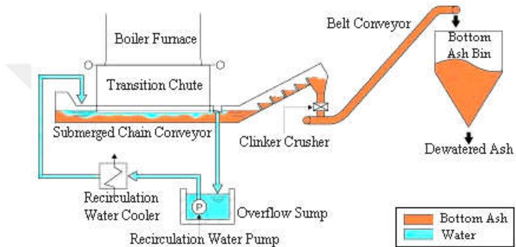
Figure 2.3. Typical SSC system [13]
