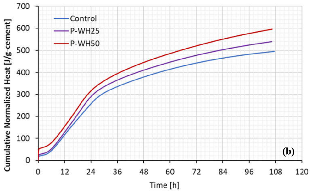
Figure 4.4 Hydration Heat of Control and P-WH25 & P-WH50 Pastes (a) Hydration Heat Evolution Rate, (b) Cumulative Hydration Heat / Cement
