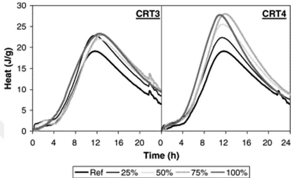
Figure 2.10. Evolution of Heat for Series CRT3, Lower Cement Content, and CRT4, Greater Cement Content [29]
