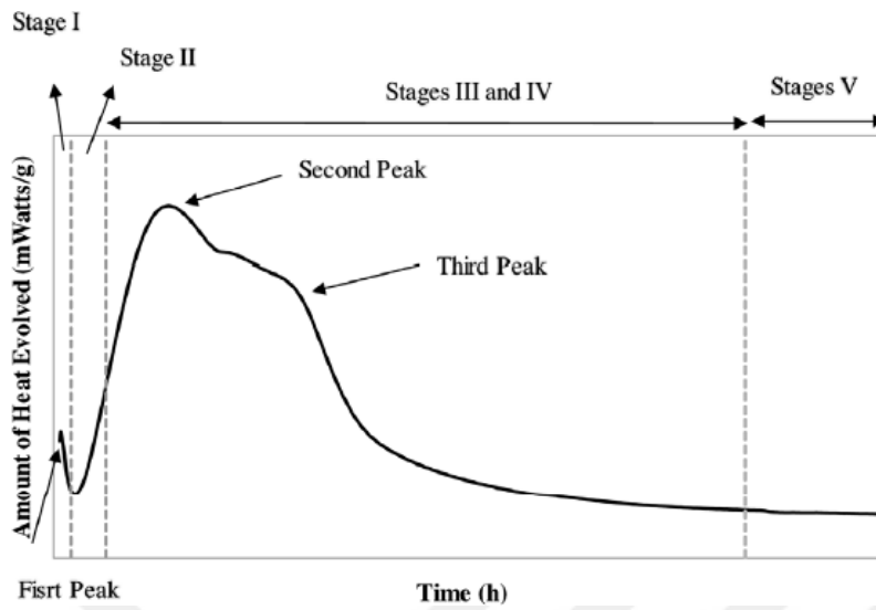
Figure 3.18 Common Cement Heat Evolution Curve [65]
