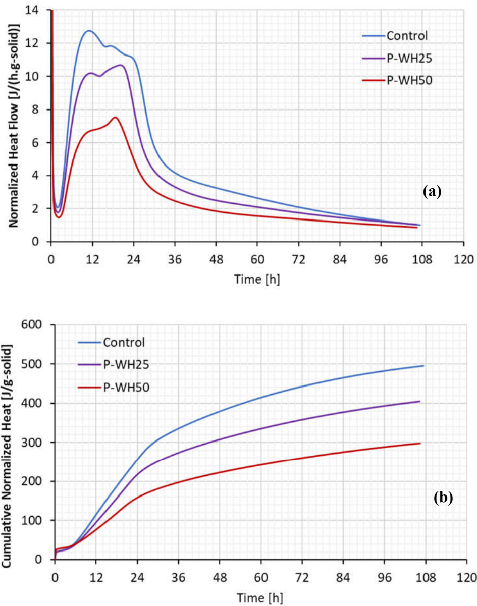
Figure 4.2 Hydration Heat of Control and P-WH25 & P-WH50 Pastes (a) Hydration Heat Evolution Rate, (b) Cumulative Hydration Heat / Solid
