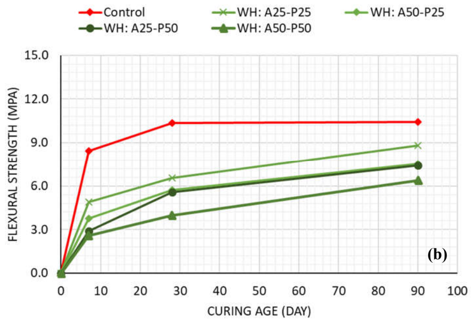
Figure 4.21 Flexural Strength Evolution vs. Age of Combined Usage Mortars with DHBA (a) and WHBA (b)
