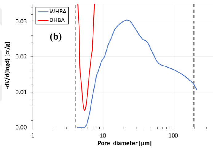
Figure 3.9. PSD of DHBA (a) and WHBA (b) by MIP ( 4 \mu\text{m} \leq d \leq 200 \mu\text{m} )
