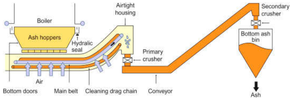
Figure 2.4. Dry- Bottom Ash Hopper Arrangement [9]
