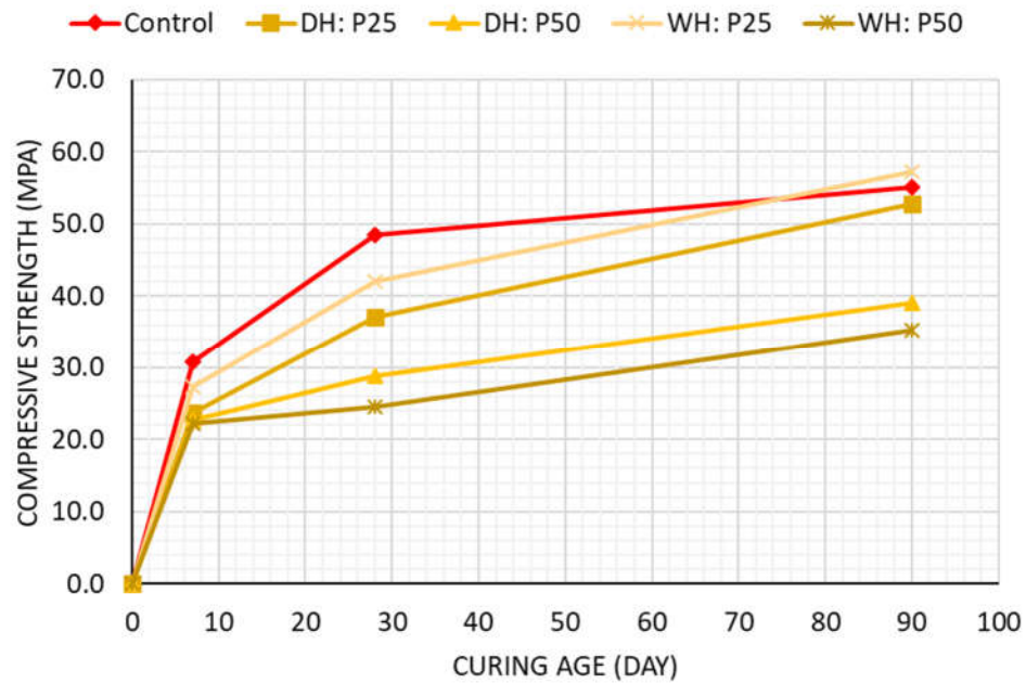
Figure 4.15 Compressive Strength vs. Age of Usage as SCM Mortars
