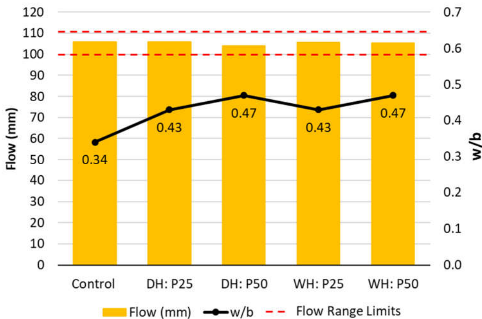
Figure 4.8 Flow and w/b for the Durability Test Mortars of Usage as SCM
