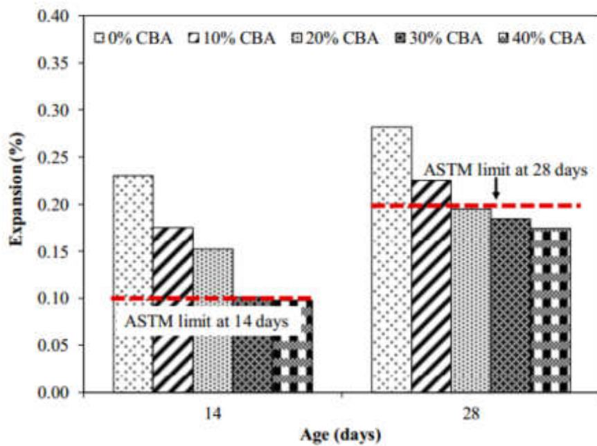
Figure 2.14. Expansion Results and ASTM Limits for Mixture with Various Proportions of CBA [50]
