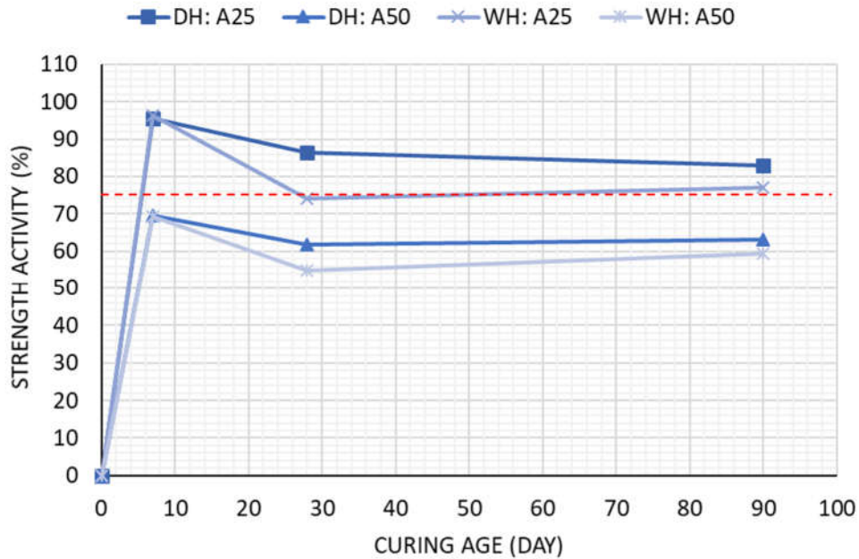
Figure 4.14 Compressive Strength Evolution vs. Age of Usage as FA Mortars
