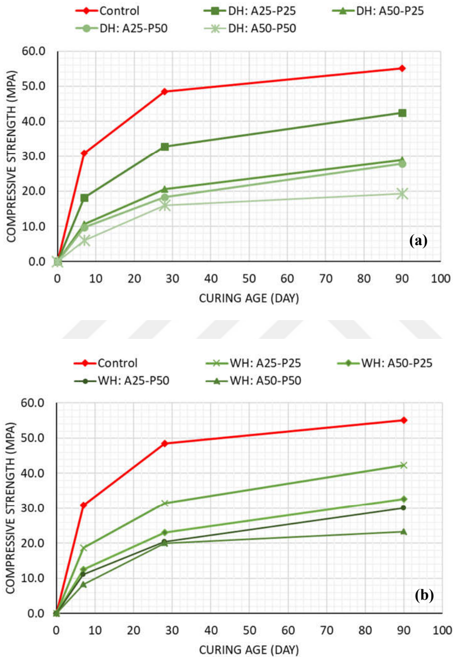
Figure 4.17 Compressive Strength vs. Age for Combined Usage Mortars with DHBA (a) and WHBA (b)
