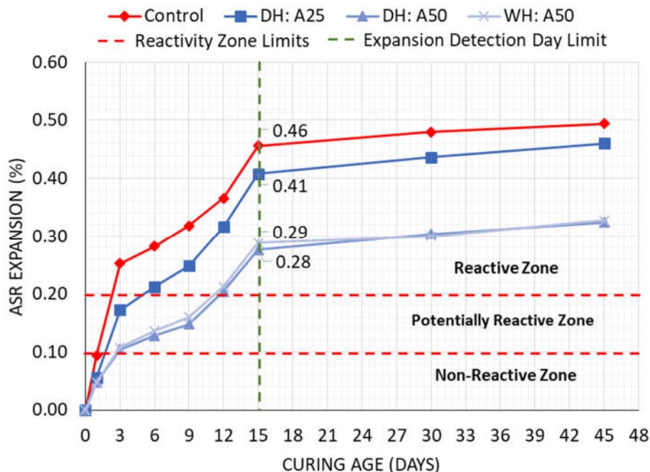
Figure 4.22. ASR Expansions of Usage as FA Mortars
