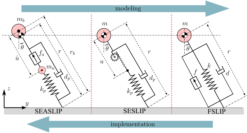
Figure 3.1: A hierarchy of progressively simpler templates for planar running behaviors starting from the anchor model with series elastic actuation on the left (SEASLIP) to the lossy SLIP template with parallel force actuator (FSLIP) on the right.
