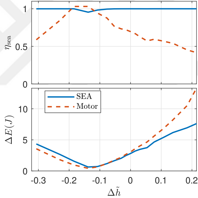
Figure 4.12: Efficiency of SEA work as a function commanded height change.
