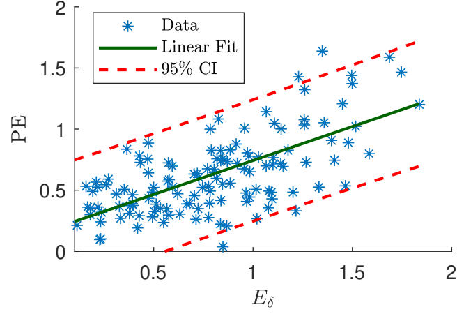
Figure 4.11: Dependence of PE on SEA tracking error where a linear model (green solid) can be fitted to the data (blue star) with 95% confidence intervals (dashed red) and R^2 = 0.56 .
