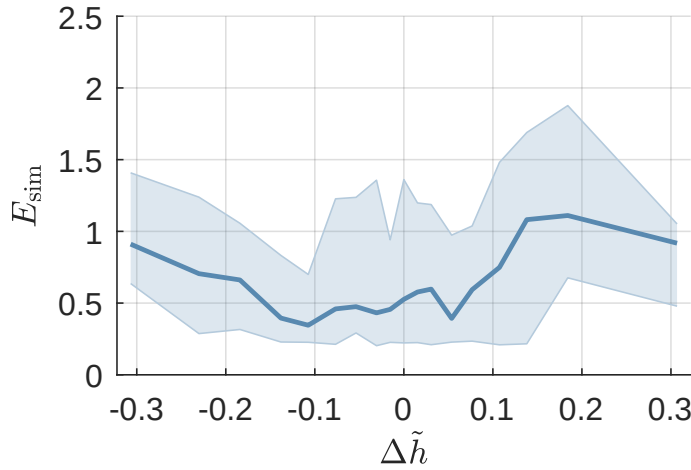
Figure 4.8: Prediction error of RM simulations compared to the physical implementation. Solid blue line corresponds to the mean error, and the shaded area is defined by the minimum and maximum error values, thus representing the entire set of experiments.
