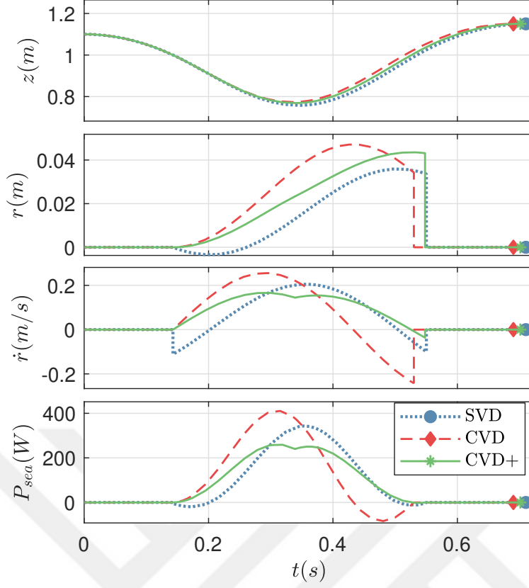
Figure 4.3: A simulation example with the IM, using SVD (dotted-blue), CVD(dashed-red), and CVD+(solid green) policies to realize the same desired apex state within a single stride starting from the same initial condition.
