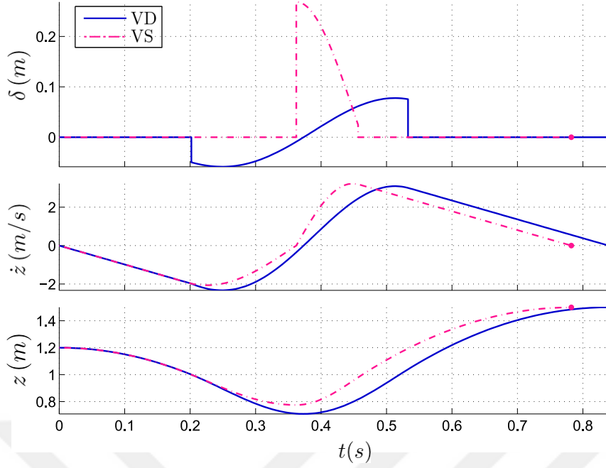
Figure 2.4: Example simulation plots of actuator input (top), vertical velocity (middle) and vertical position (bottom) with constant d throughout stance (solid blue) and step stiffness change at bottom (dot-dashed red). End of the stride in each case is marked with a colored dot.
