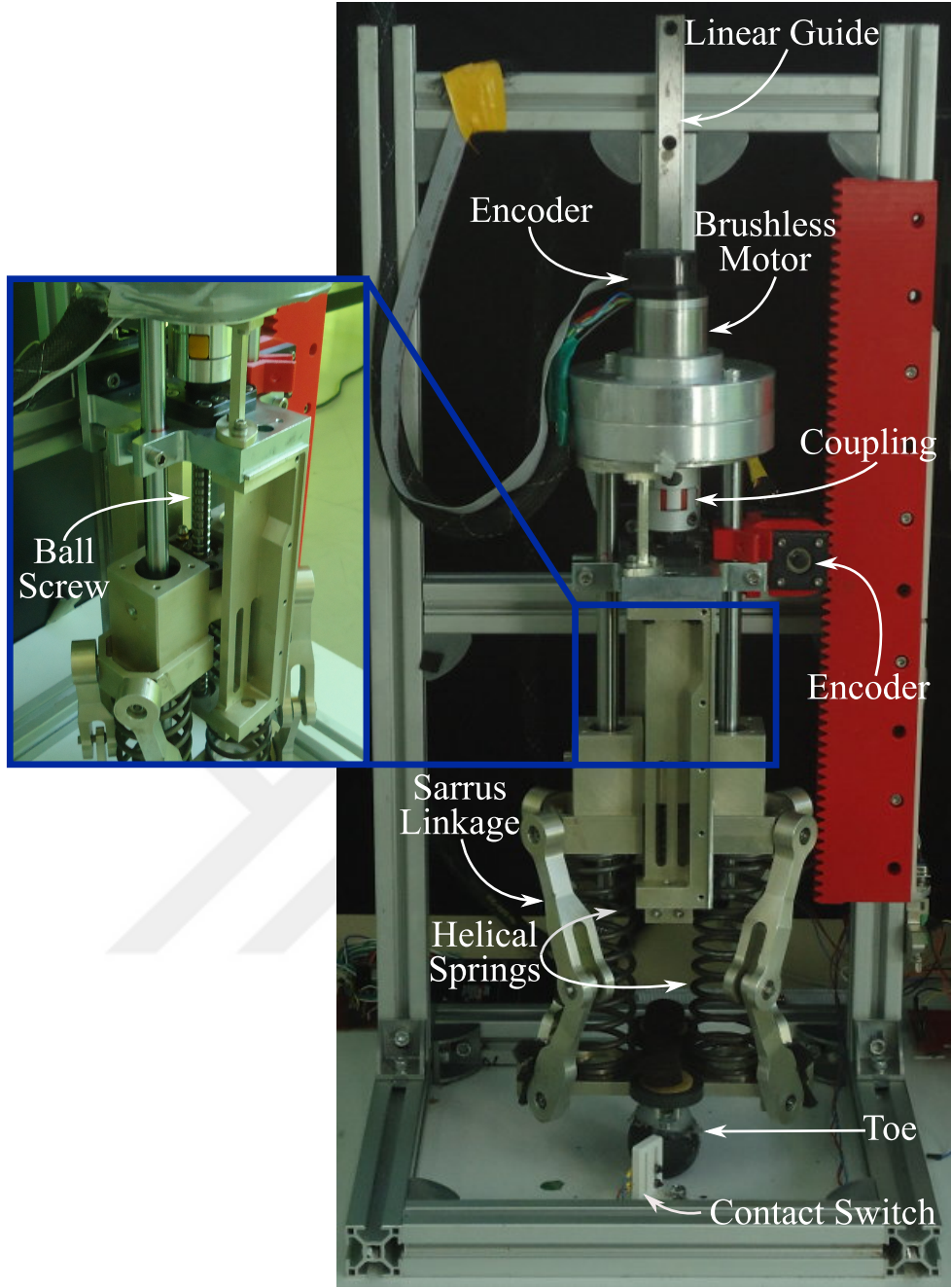
Figure 4.5: Our robot is a 5.5 kg vertical hopper with series elastic actuator consisting of a motor and ball screw.
