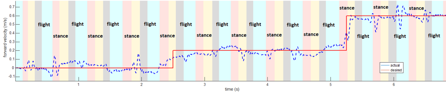
Figure 5.5: An example experiment showing commanded (solid-red) and actual (dashed-blue) forward velocities ranging from in-place hopping to 0.6 m/s.
