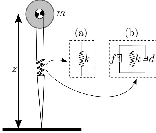
Figure 4.1: Lossless SLIP (a) and FSLIP (b) models of hopping.
