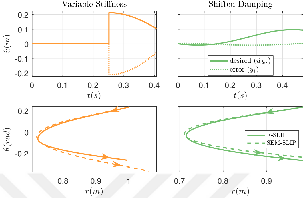
Figure 3.5: Stabilization of transverse dynamics (top) and the phase portrait for the zero dynamics (bottom) during a single stance phase with SEASLIP, embedding the template model FSLIP controlled with Variable Stiffness (left) and Shifted Damping (right) control strategies.
