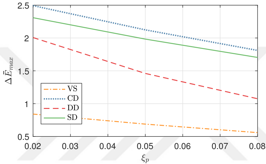
Figure 3.3: The maximum amount of normalized energy that can be injected into the system in a single stride for different control strategies as a function of the physical damping ratio \xi_p .
