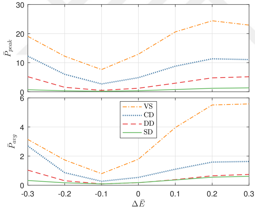
Figure 3.6: Peak (top) and average (bottom) power requirements for all deadbeat control strategies as a function of commanded change in the apex energy level, averaged over different initial conditions, model parameters and velocity commands.
