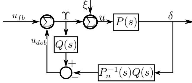
Figure 4.6: Block diagram of feedback linearized system augmented with disturbance observer.
