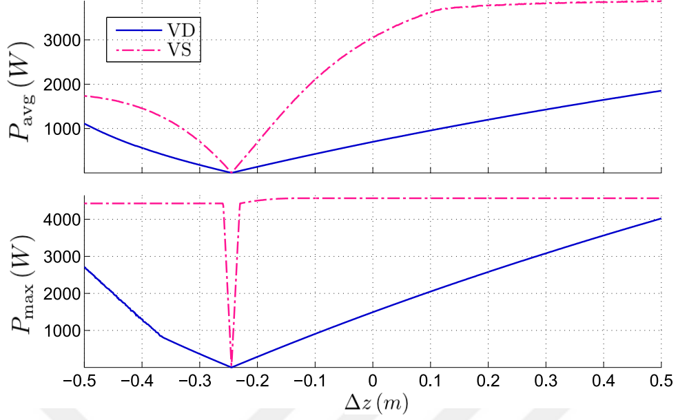
Figure 2.7: Dependence of average (top) and maximum (bottom) actuator power on the commanded height difference for different controllers. Simulations were run for a particular leg with k = 10000N/m and d_p = 100Ns/m and an initial height z(0) = 1.6m . Note that power data are saturated for visibility purposes.
