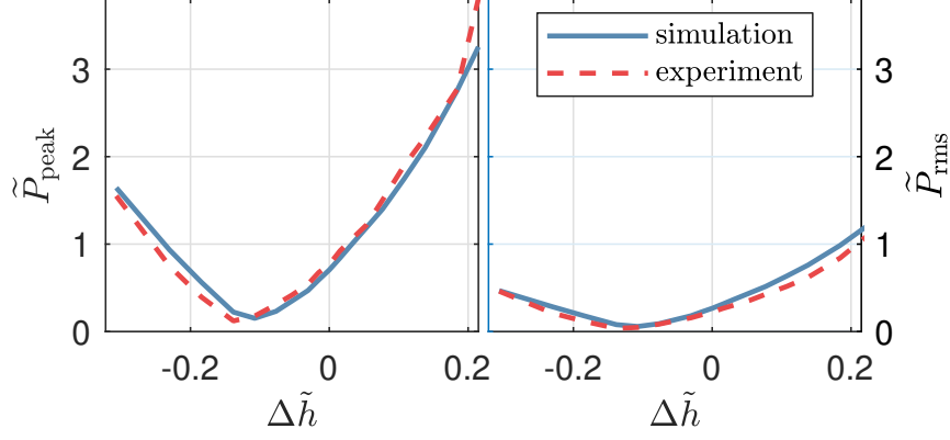
Figure 4.9: Nondimensional peak (left) and RMS (right) power consumption of RM simulations (solid blue) and experiments (dashed red) in a single step for various commanded changes in apex height.
