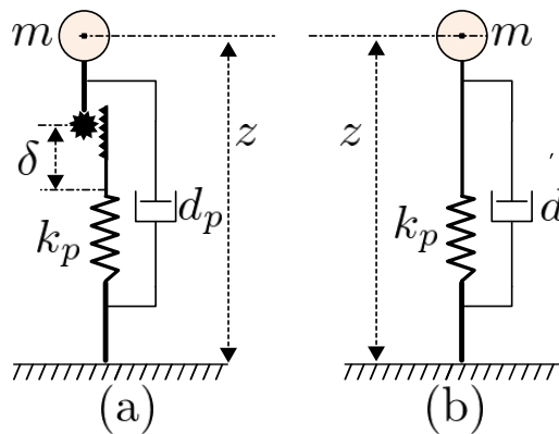
Figure 2.1: (a) VA-SLIP: Vertical SLIP model with linearly actuated compliant leg and physical damping coefficient d_p , (b) VD-SLIP: Vertical SLIP template with a tunable, possibly negative, damping coefficient d .
