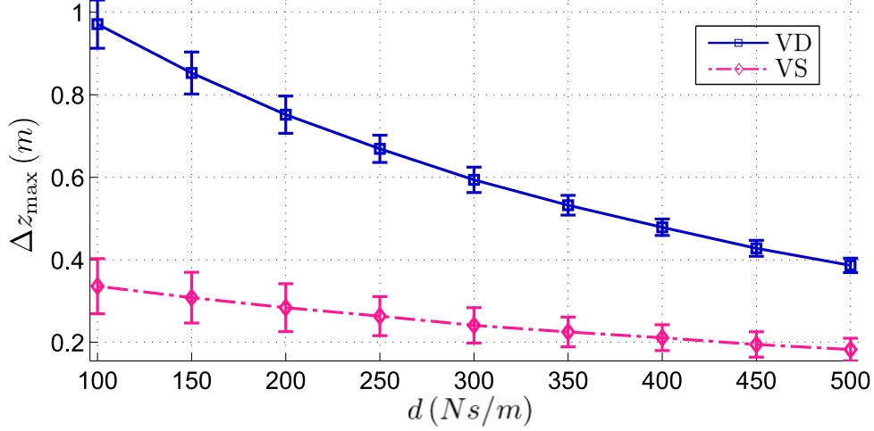
Figure 2.5: Maximum height gain \Delta y = z^* - z(0) that can be achieved using different control strategies as a function of the physical leg damping d_p with \delta_{\max} = 0.2m , averaged over z(0) \in [1.1, 2.5]m , k \in [10, 40]kN/m . Error bars correspond to the standard deviation across different initial conditions and spring stiffness values.
