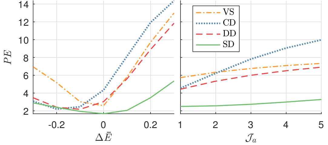
Figure 3.4: Average percentage errors in apex states for single-stride deadbeat control of the SEASLIP model for different controllers as a function of commanded change in normalized energy (left) and reflected actuator inertia (right).
