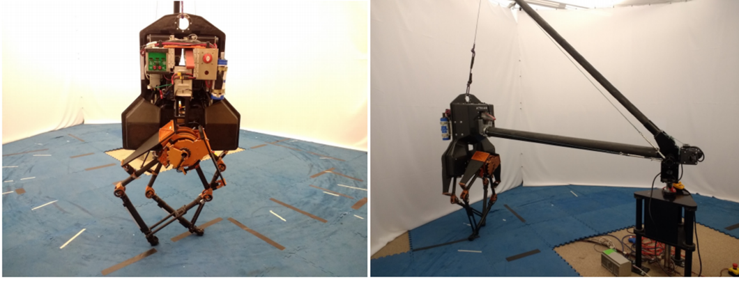
Figure 5.2: The robot is constrained to sagittal plane with a boom.
