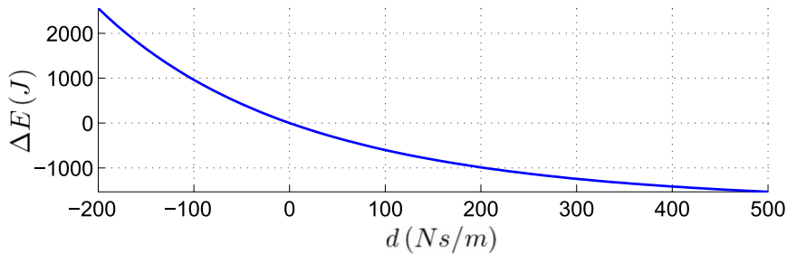
Figure 2.2: Monotonic dependence of the change in VD-SLIP energy, \Delta E on the virtual damping coefficient d .
