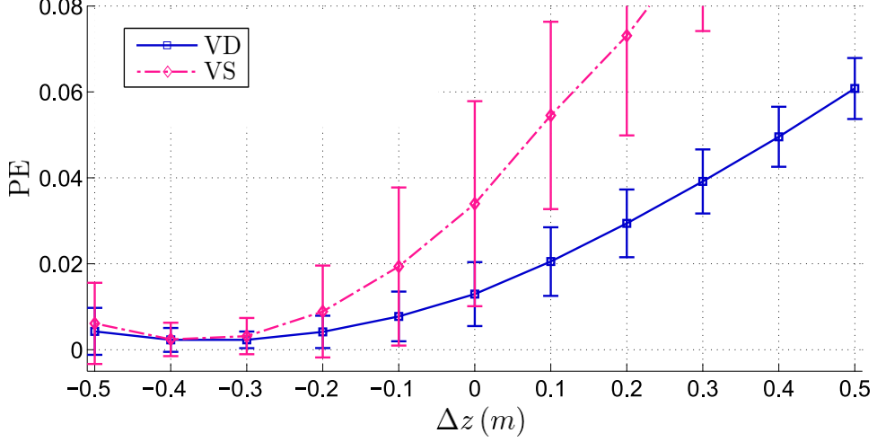
Figure 2.6: Percentage height tracking error using different control strategies with \delta_{\max} = 0.2m , \dot{\delta}_{\max} = 2m/s and F_{\max} = 10kN/m , averaged across d_p \in [100, 500]Ns/m , z(0) \in [1.1, 2.5]m , k \in [10, 40]kN/m . Error bars correspond to the standard deviation across different initial conditions and parameter values.
