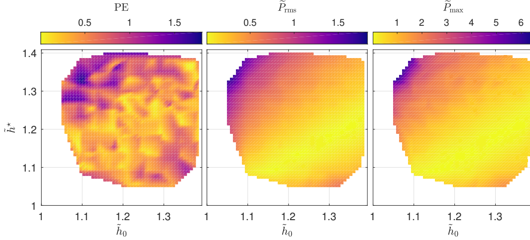
Figure 4.10: Dependence of percentage control error (left), RMS power consumption (middle), and peak power consumption (right) as a function of initial and desired apex heights.
