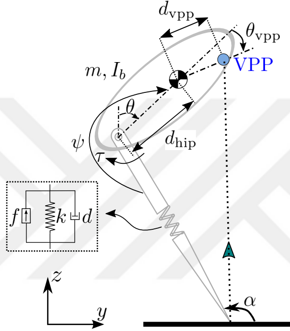
Figure 5.4: FSLIP-VPPC model redirects GRF toward the VP pivot point on the body.
