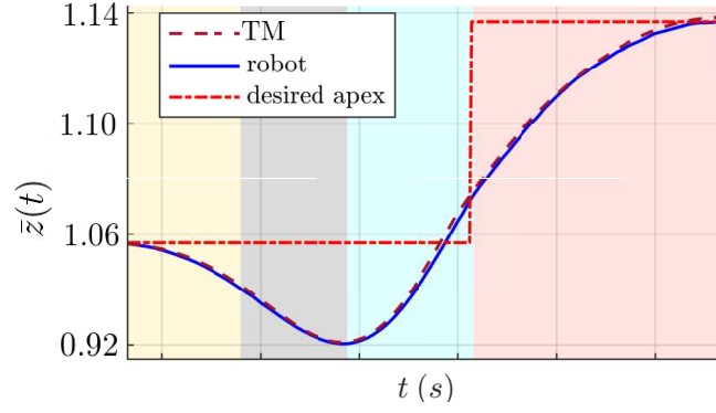
Figure 4.7: Single step trajectories of target model (TM - dashed maroon) and physical robot (RM - solid blue) for a change in desired apex height (dash-dotted red).
