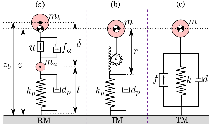
Figure 4.2: A hierarchy of models for vertical hopping starting from the RM to the TM to be realized via an IM.
