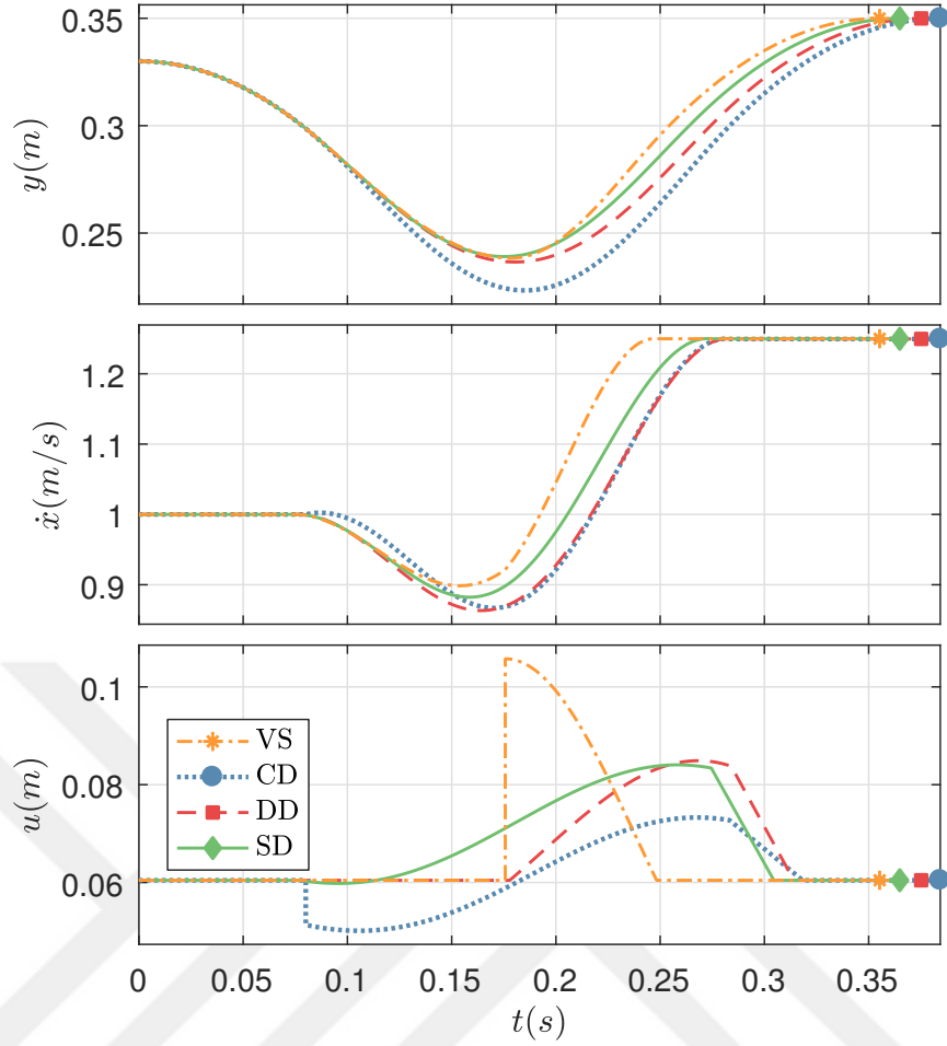
Figure 3.2: An example SESLIP simulation, using the Variable Stiffness (VS), Constant Damping (CD), Decompression-only tunable Damping (DD) and Shifted Tunable Damping (SD) methods to realize a desired apex state within a single stride starting from the same initial condition. After liftoff, the actuator is position retracted to u_0 in a fixed amount of time.
