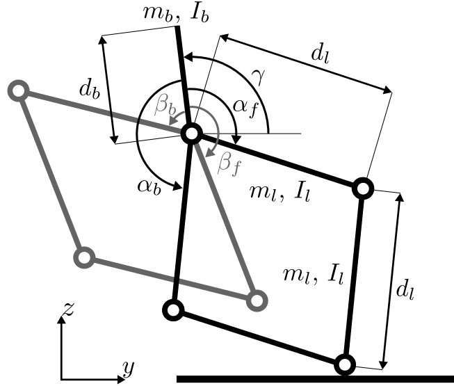
Figure 5.3: Planar model of ATRIAS robot.
