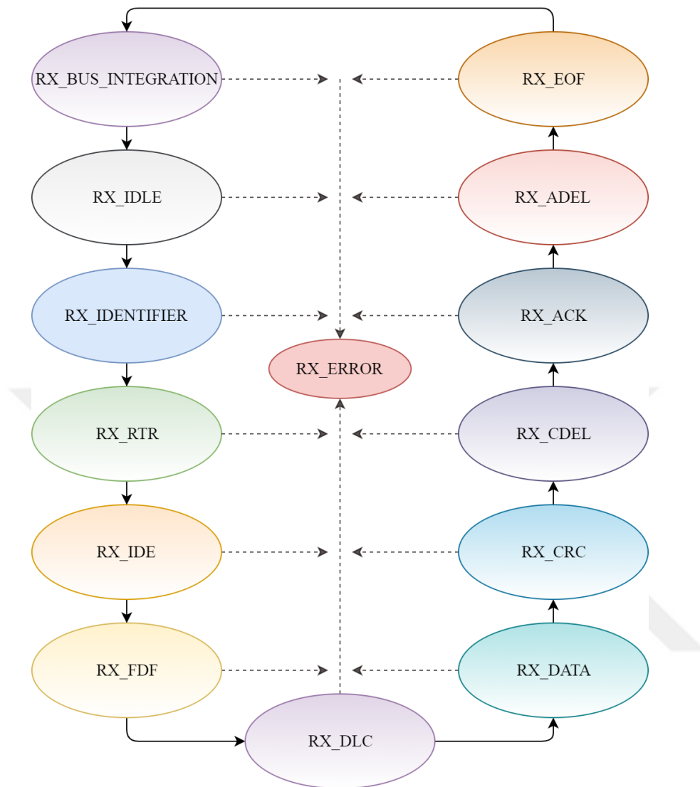
Figure 3.3: SDCC MAC Layer RX Finite State Automata
