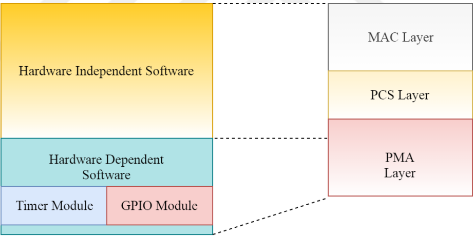
Figure 3.6: Software-Defined CAN Controller Hardware Dependency
