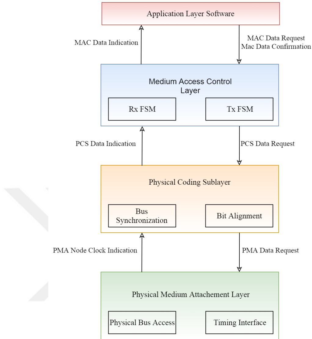
Figure 3.2: Software-Defined CAN Controller Primitives
