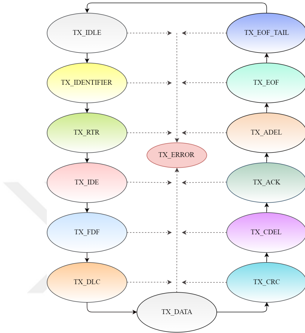
Figure 3.4: SDCC MAC Layer TX Finite State Automata
