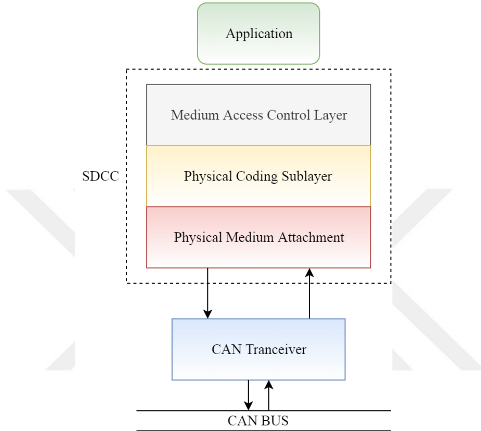
Figure 3.1: Software-Defined CAN Controller Architecture
