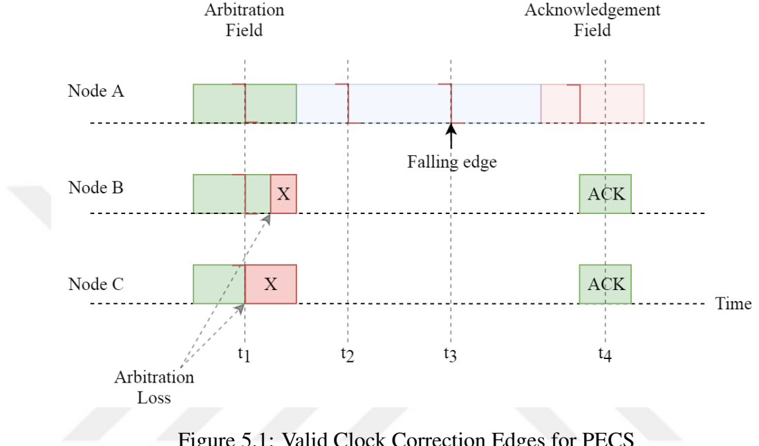
Figure 5.1: Valid Clock Correction Edges for PECS
