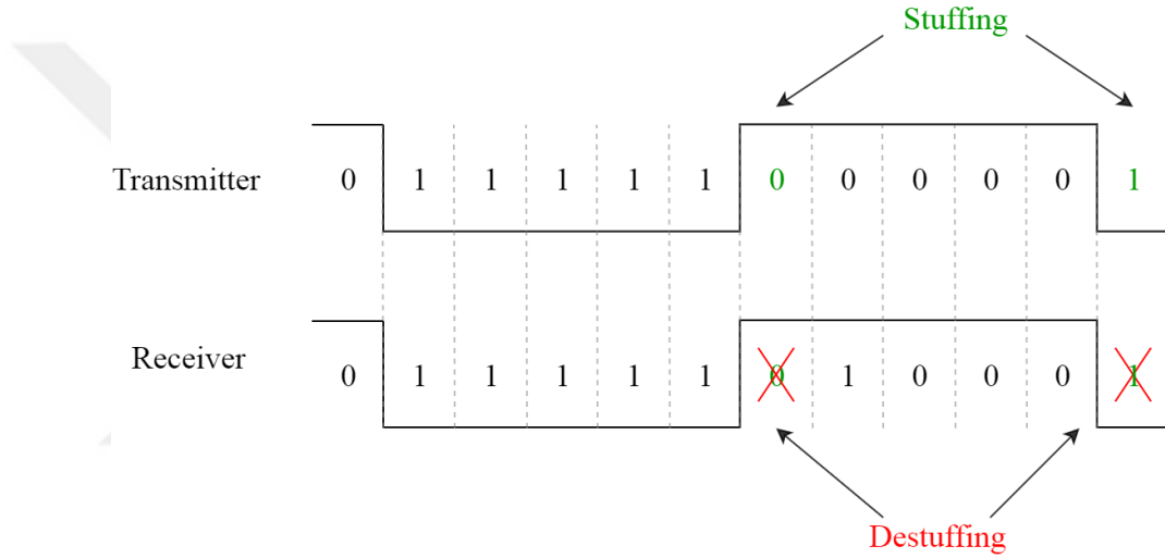
Figure 2.7: Bit Stuffing and Destuffing in CAN
