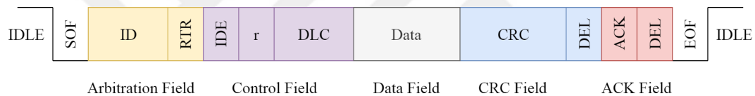
Figure 2.2: A Typical Controller Area Network Frame
