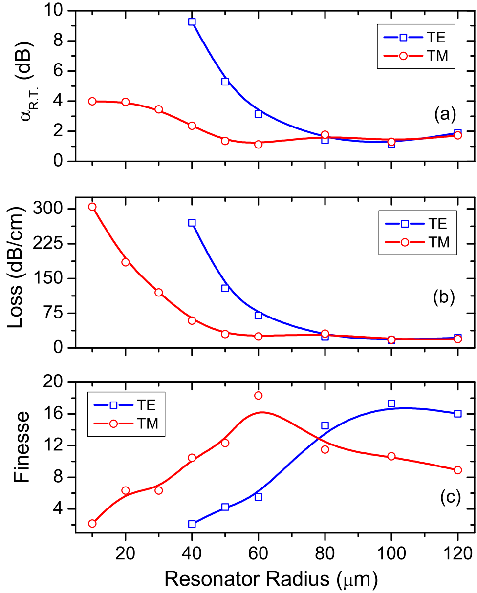
Figure 5.13: (a) Resonator round trip loss (b) effective propagation loss and (c) finesse values for TE and TM polarizations
