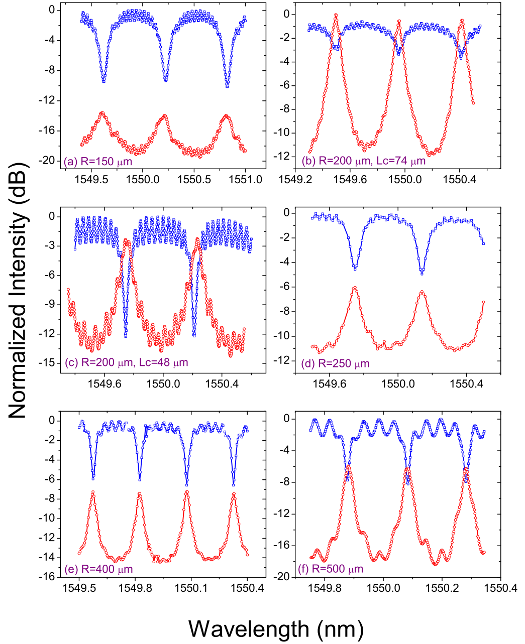
Figure 5.20: Measured TE transmission and drop spectra of the characterized double bus resonators.
