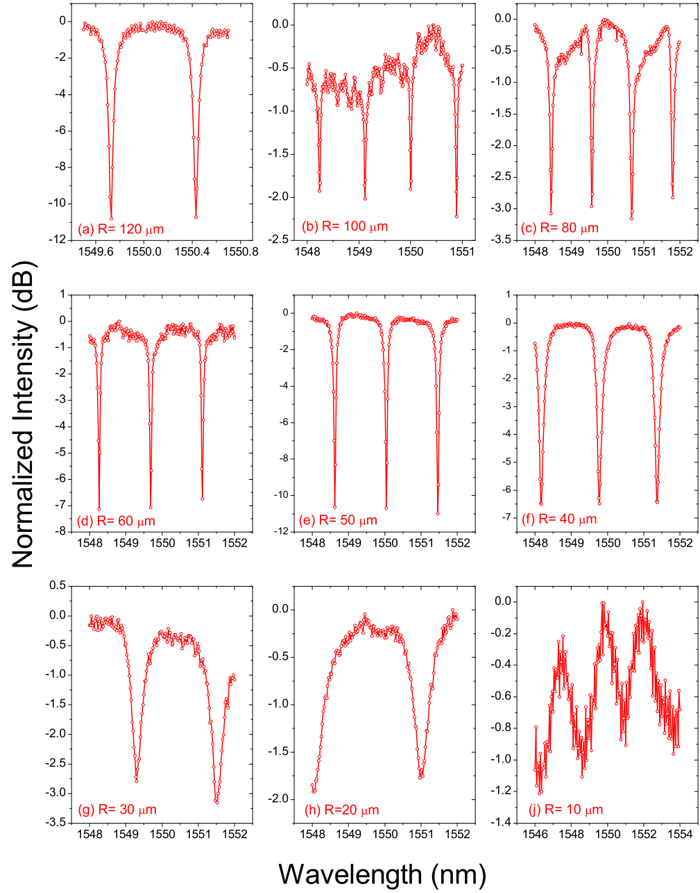
Figure 5.11: Measured TM transmission spectra of the characterized resonators.
