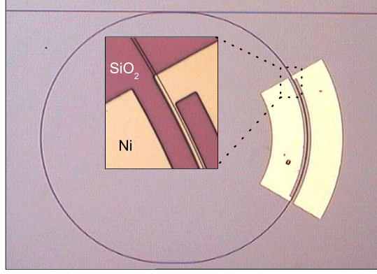
Figure 5.15: (a) Optical micrographs showing top view of a fabricated racetrack resonator and overlaying metal heater.
