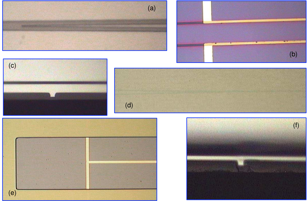
Figure 6.7: Optical micrographies taken during the fabrication of M-Z modulator:(a)Y-junction after first photolithography (b) Ni heaters defined on each arm (c) After planarization using BCB (d) Y-junction seen from backside after layer transfer. (e) Openings for electrical contact (f) Input waveguide facet after cleavage.
