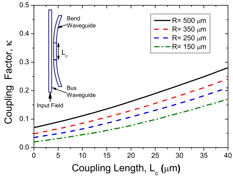
Figure 4.9: Power coupled from bus waveguide to racetracks with various radii for TE polarization as a function of straight section length for gap of 0.8\ \mu\text{m} .
