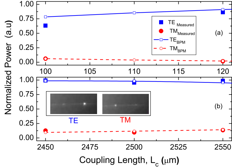
Figure 3.6: Normalized polarized optical power measured at the output port 2 for both TE and TM input signals for (a) gap=0.7 \mu\text{m} and (b) gap=1.4 \mu\text{m} . Lines are drawn to guide the eye.
