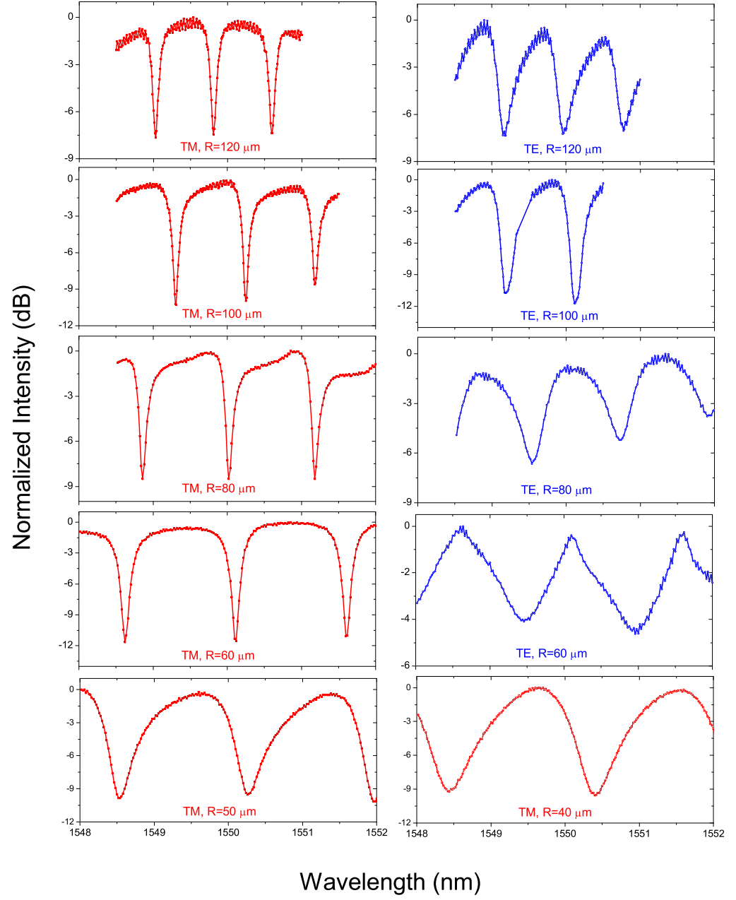
Figure 5.5: Measured TM and TE transmission spectra of the fabricated silicon-on-insulator rib waveguide racetrack resonators for radii of 40 to 120 \mu\text{m} .
