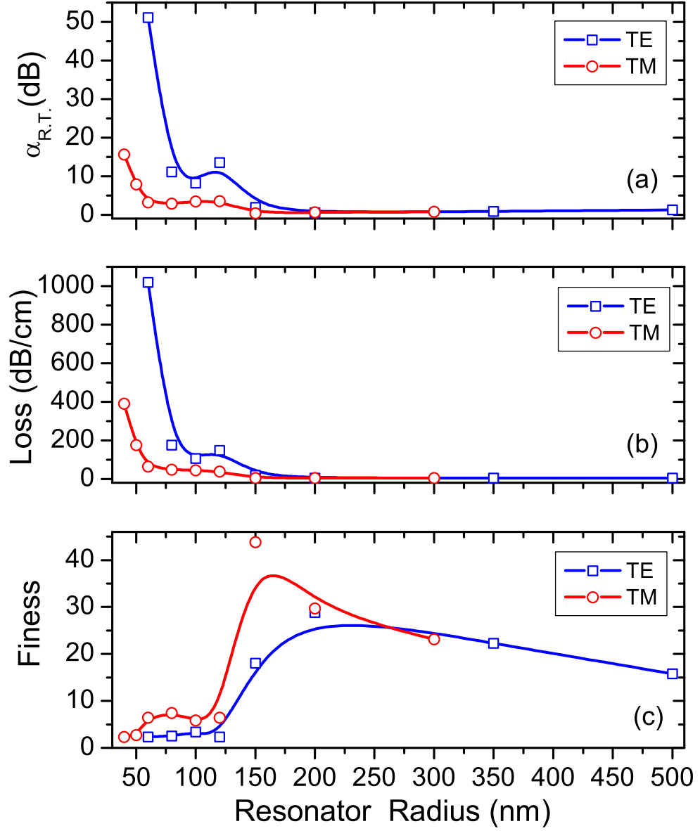
Figure 5.7: The extracted (a) resonator round trip and (b) effective propagation losses and (c) measured finesse values for TE and TM polarizations. The solid lines are to guide the eye.
