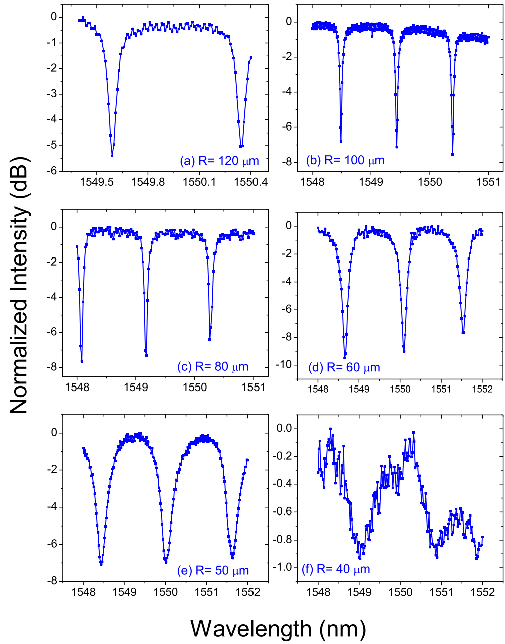
Figure 5.10: Measured TE transmission spectra of the characterized resonators.
