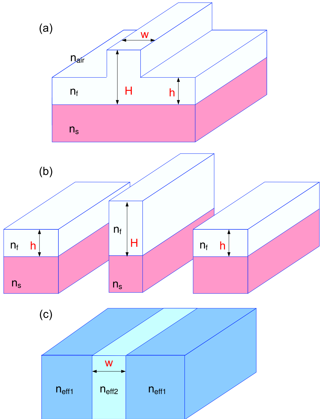
Figure 2.3: Effective index analysis for a rib waveguide of air cladding. (a) The rib waveguide with its critical dimensions. (b) Three slab waveguides constructed from the rib waveguide. (c) Artificially constructed slab waveguide using effective index of three slabs.
