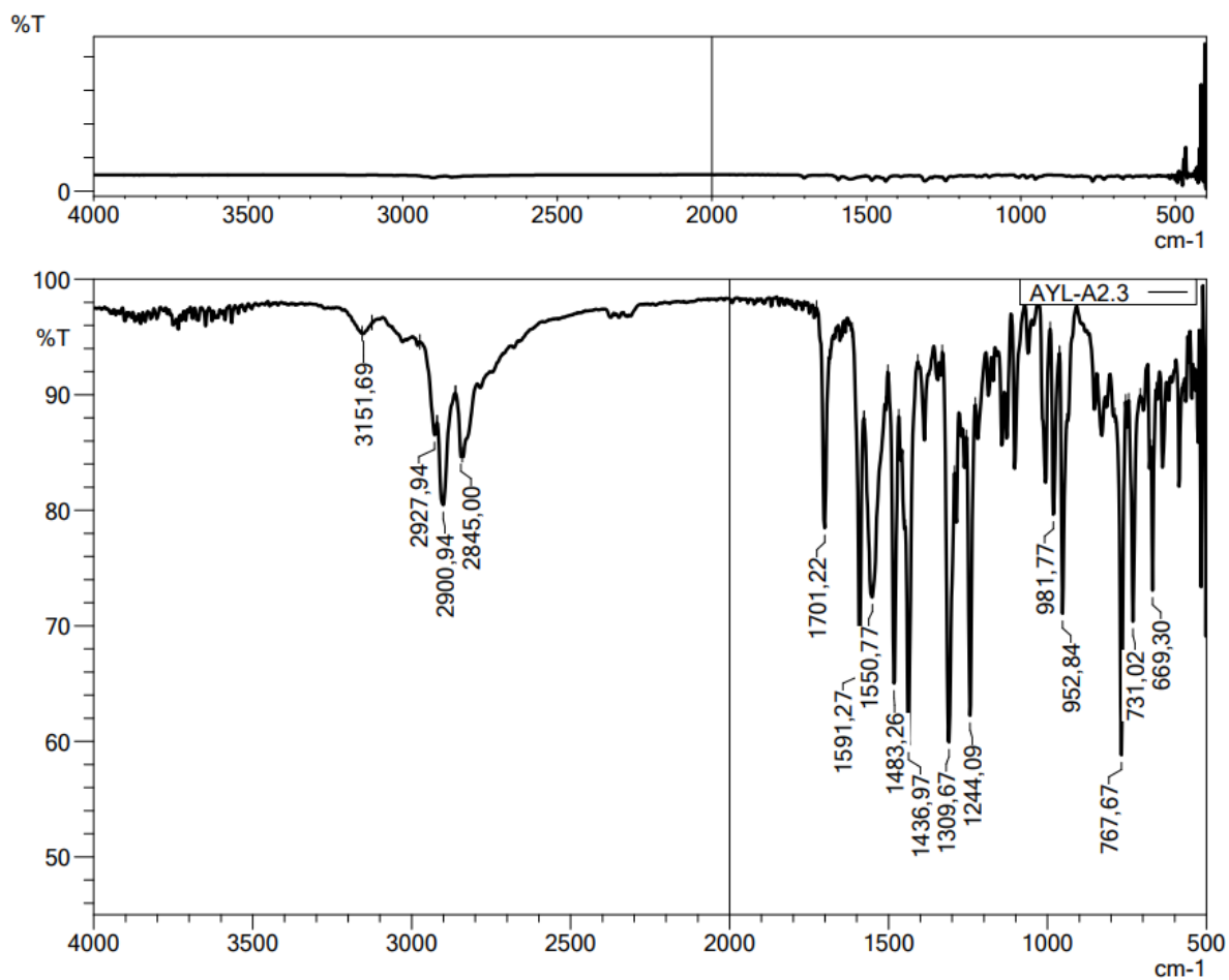
Figure 5.11. IR spectrum of compound 3b
