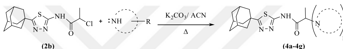
Figure 4.5. Synthesis of N -(5-(adamantan-1-yl)-1,3,4-thiadiazol-2-yl)-2-substituted-propanamide derivatives (Method E)
