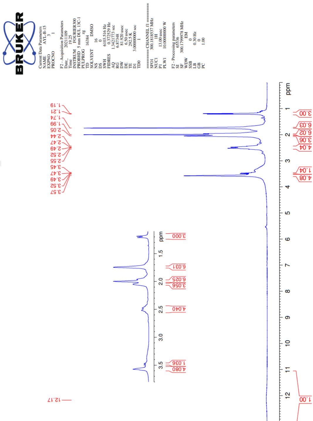
Figure 5.88. ^1\text{H} -NMR spectrum of compound 4g
