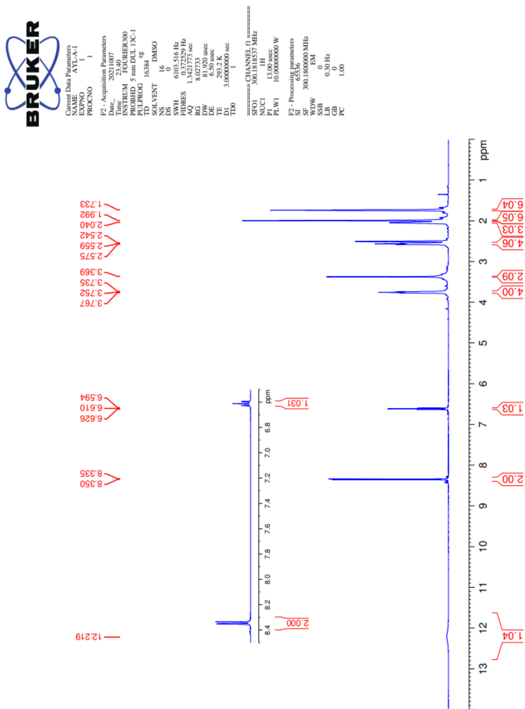
Figure 5.7. ^1\text{H} -NMR spectrum of compound 3a
