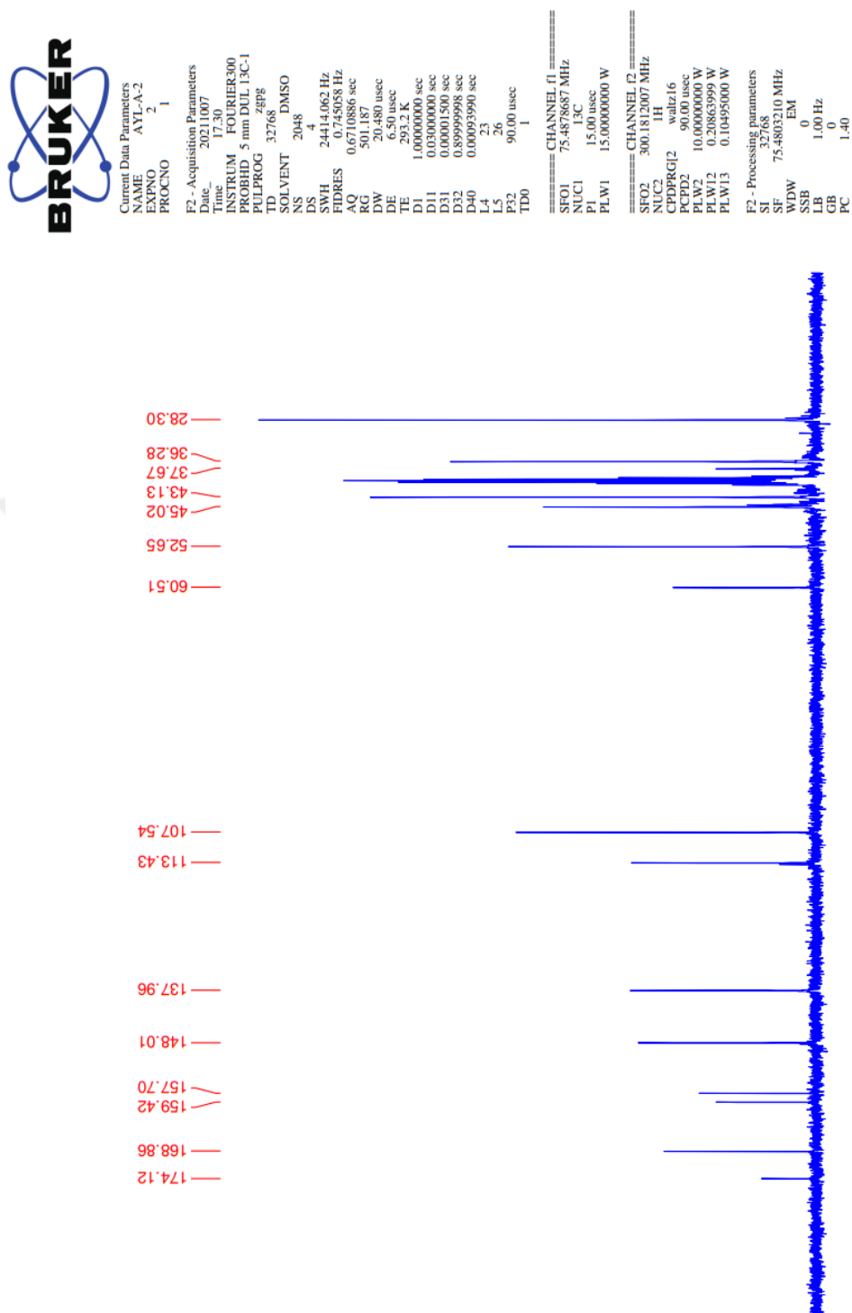
Figure 5.13. ^{13}\text{C} -NMR spectrum of compound 3b
