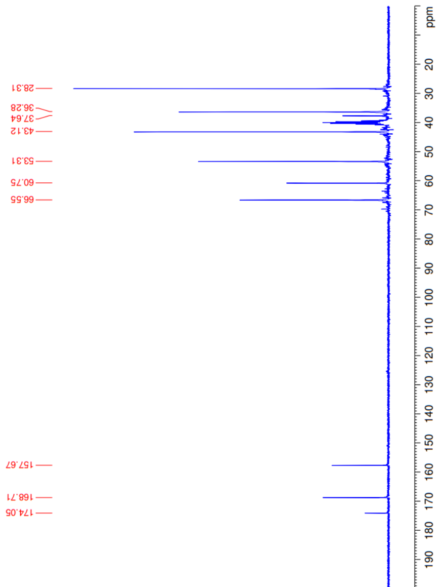
Figure 5.48. ^{13}\text{C} -NMR spectrum of compound 3i
