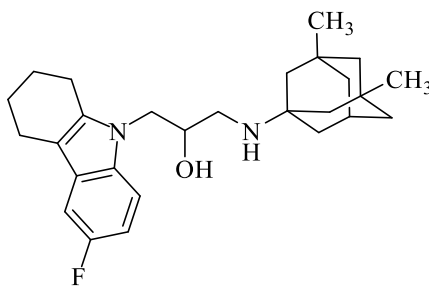
Figure 2.51. Tetrahydrocarbazoles-aminoadamantane conjugate
