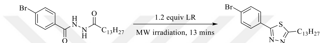
Figure 2.16. Synthesis of 2,5-disubstituted-1,3,4-thiadiazole from N, N' -diacyl hydrazine by using LR
