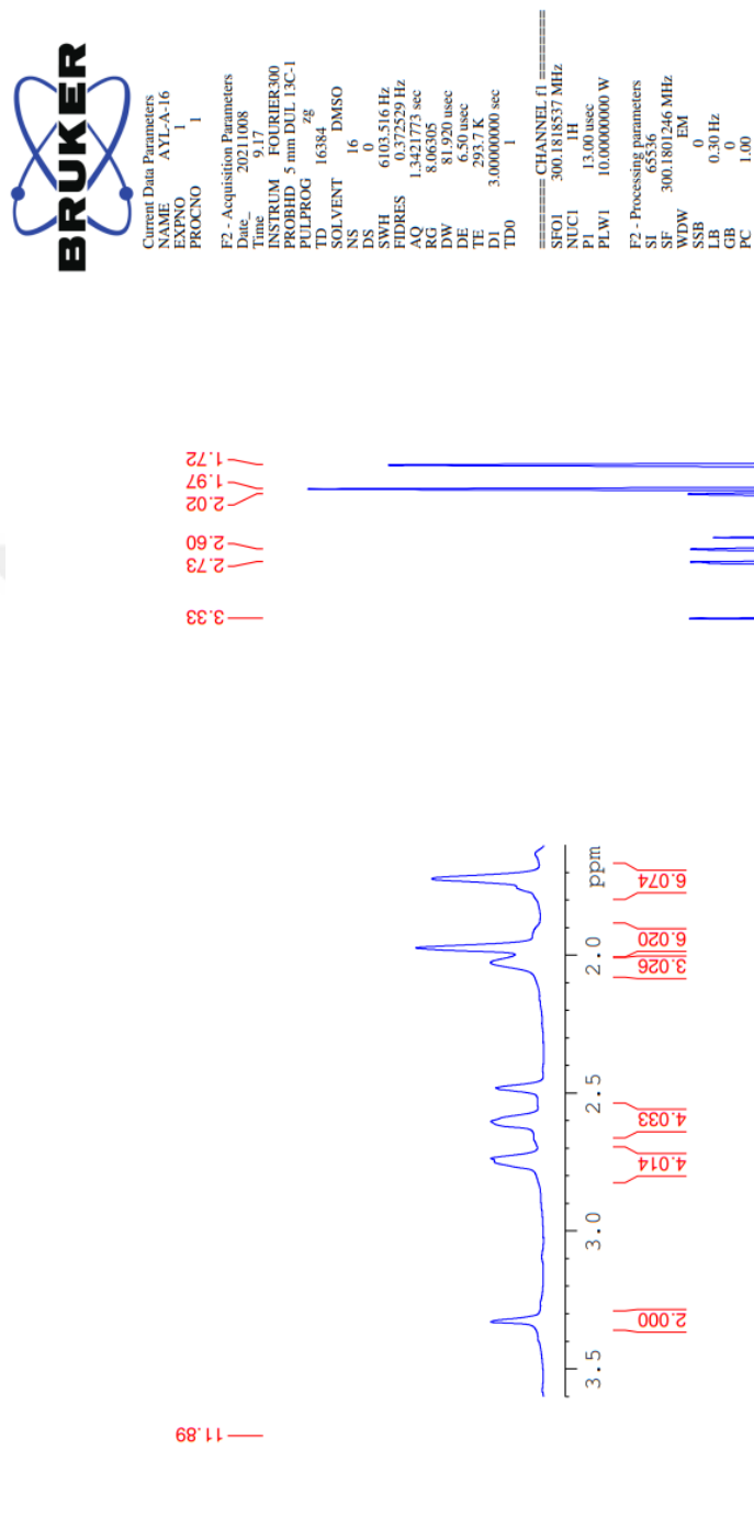
Figure 5.52. ^1\text{H} -NMR spectrum of compound 3j
