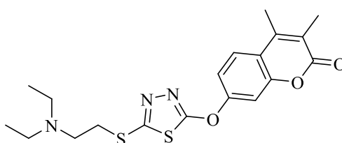
Figure 2.39. 7-[(5-[(2-(Diethylamino)ethyl)thio]-1,3,4-thiadiazol-2-yl)oxy]-3,4-dimethyl-2H-chromen-2-one
