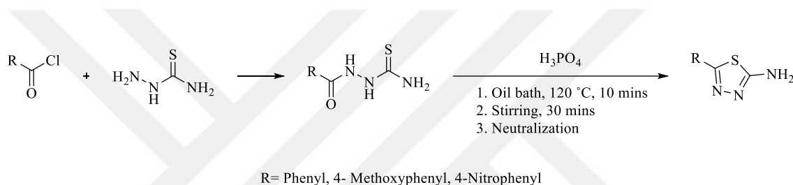
Figure 2.8. Synthesis of 2-amino-5-substituted 1,3,4-thiadiazole from thiosemicarbazide and benzoyl chloride derivatives by using phosphoric acid
