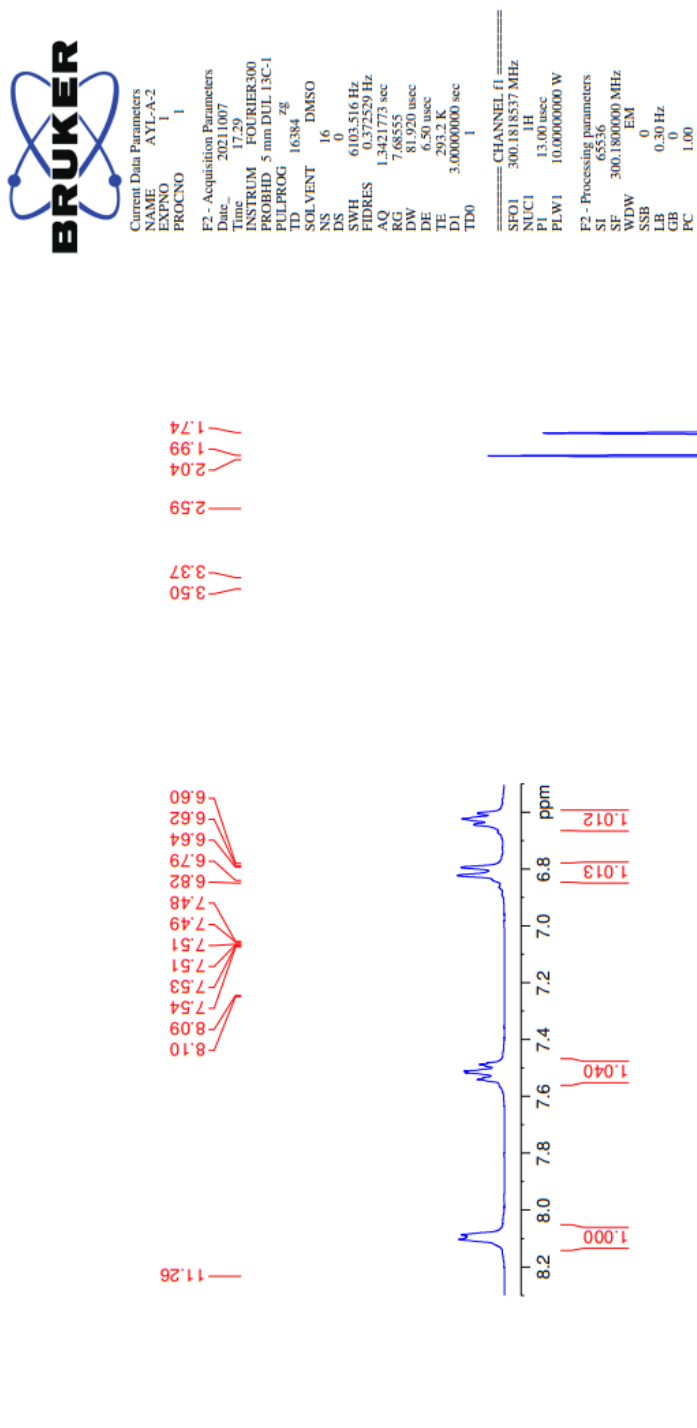
Figure 5.12. ^1\text{H} -NMR spectrum of compound 3b
