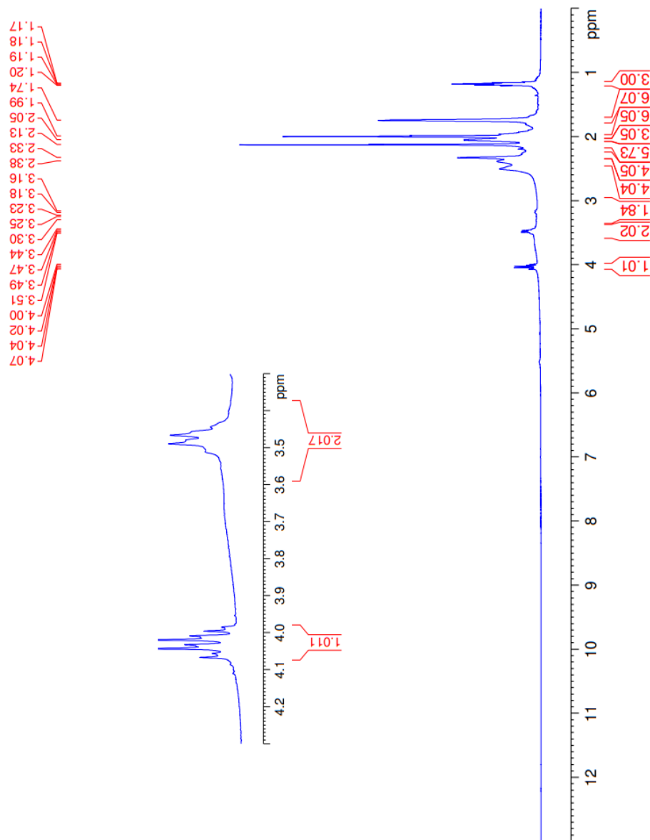
Figure 5.78. ^1\text{H} -NMR spectrum of compound 4e
