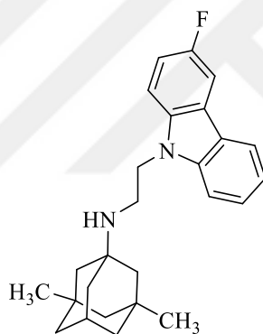
Figure 2.52. N -(2-(6-fluoro-9H-carbazol-9-yl)ethyl)-3,5-dimethyladamantan-1-amine
