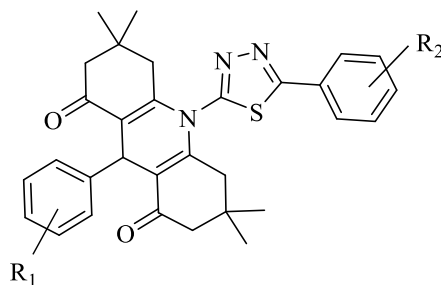
Figure 2.36. Acridine-1,3,4-thiadiazole derivatives. ( R_1 = 2,4\text{-diCl} , R_2 = 4\text{-Cl} for 4d, R_1 , R_2 = 4\text{-NO}_2 for 4i, R_1 = \text{H} , R_2 = 3\text{-NO}_2 for 4j, R_1 = 3\text{-OCH}_3 , R_2 = 3\text{-Cl} for 4k)
