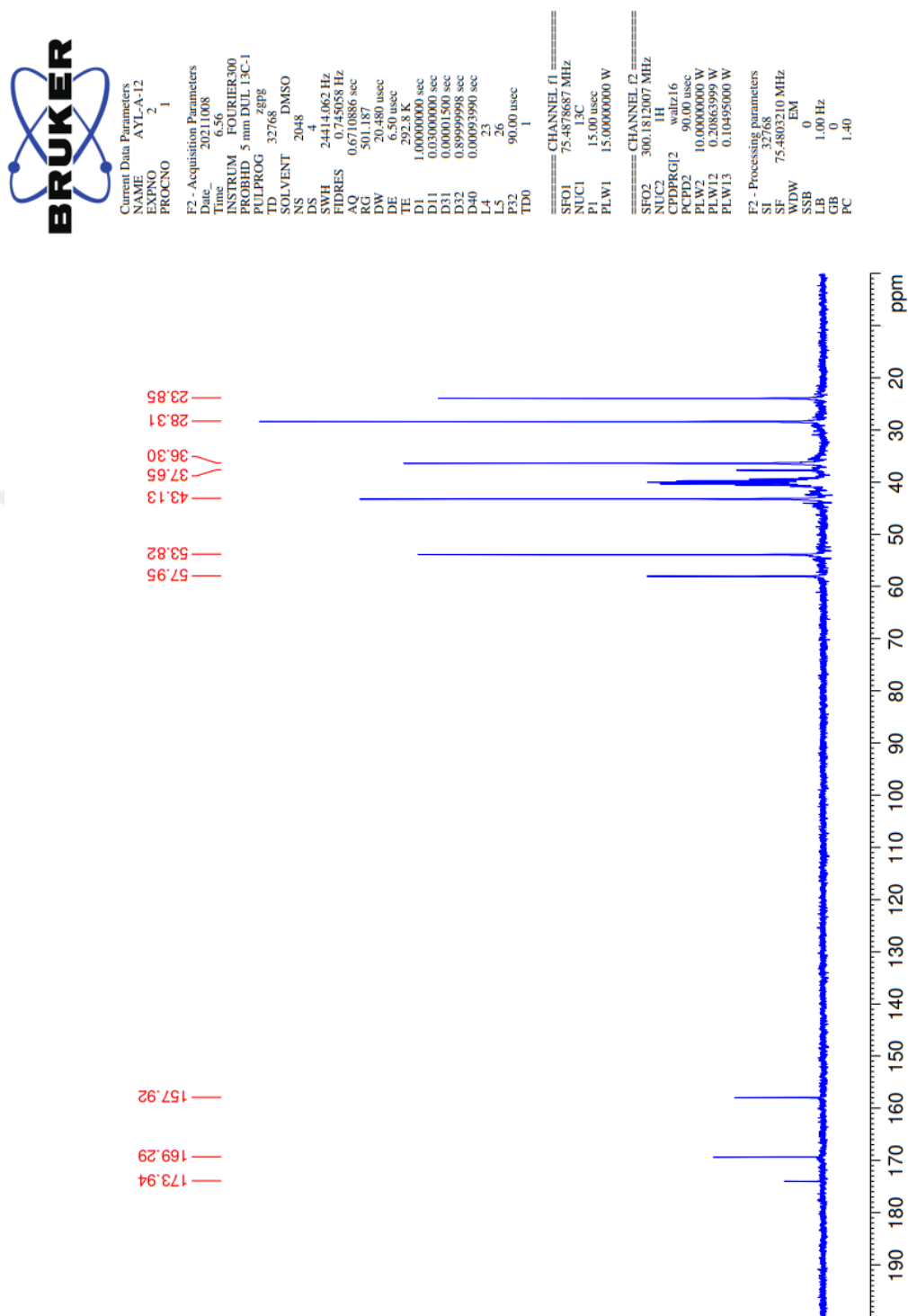
Figure 5.38. ^{13}\text{C} -NMR spectrum of compound 3g
