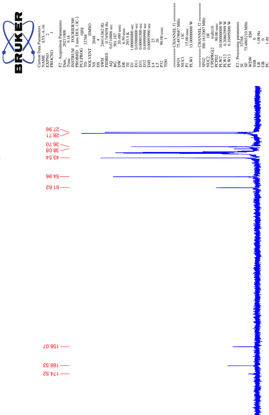
Figure 5.53. ^{13}\text{C} -NMR spectrum of compound 3j
