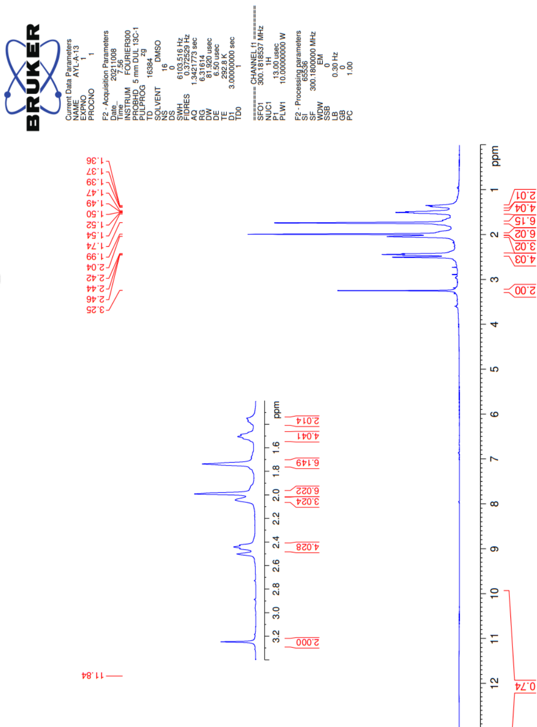
Figure 5.42. 1 H-NMR spectrum of compound 3h
