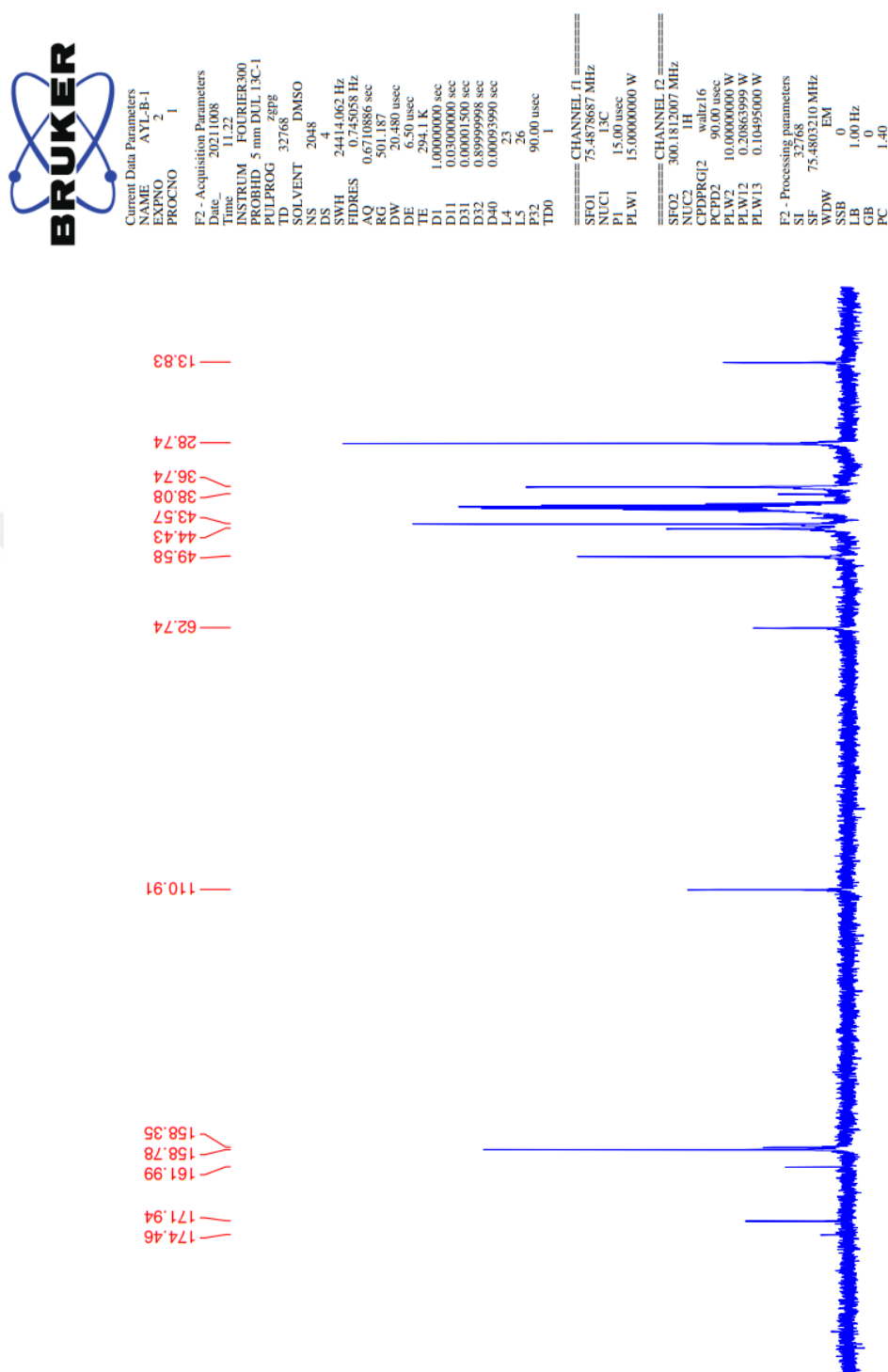
Figure 5.59. ^{13}\text{C} -NMR spectrum of compound 4a
