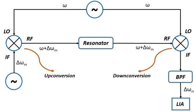
Figure 3.7: Open Loop Frequency Sweep Scheme
