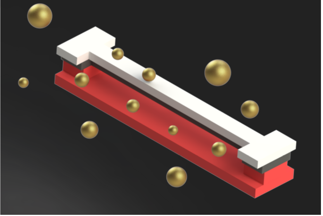
Figure 1.1: Depiction of particle adhesion on doubly clamped NEMS
