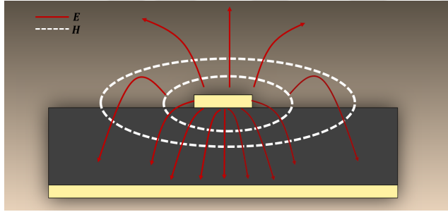
(a) Electric and magnetic field distribution in a cross-section of a microstrip TL
