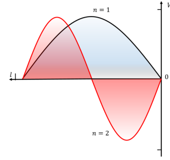
(b) Voltage profile along a microstrip TL resonator
