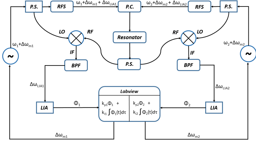
Figure 3.6: The experiment circuit
