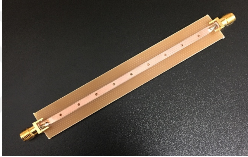
Figure 2.8: The PCB resonator with drilled holes used in pipette experiments
