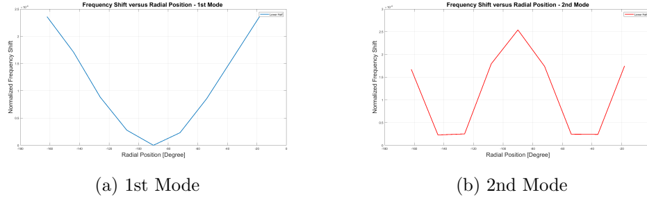
Figure 2.6: Simulated frequency shifts due to particle presence in a ring resonator
