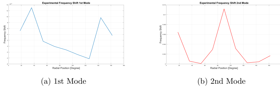
Figure 2.12: Experimental frequency shifts due to analyte presence in a ring resonator
