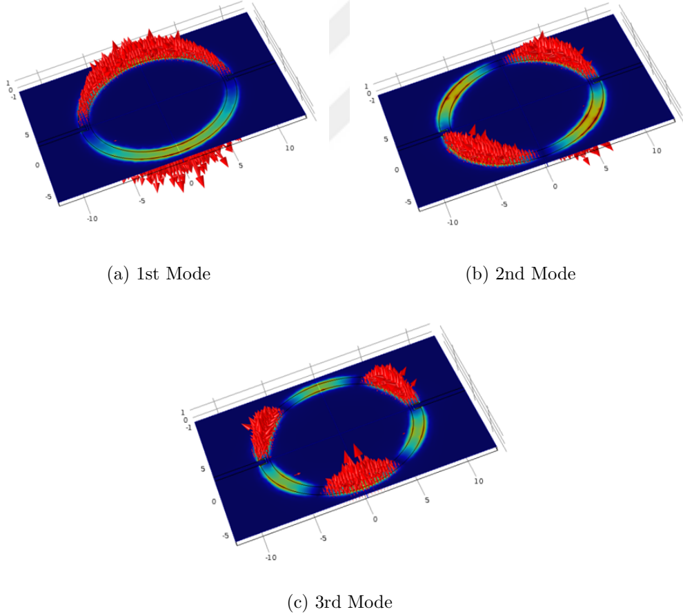
Figure 2.5: First three consequent mode shapes of a ring resonator
