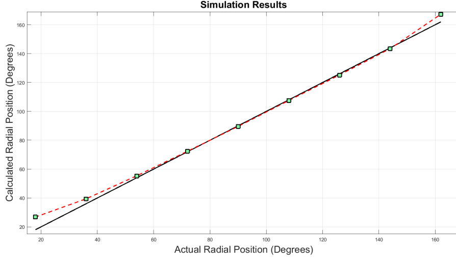
Figure 2.7: Angular position calculation with experimentally obtained frequency shifts in ring resonator case
