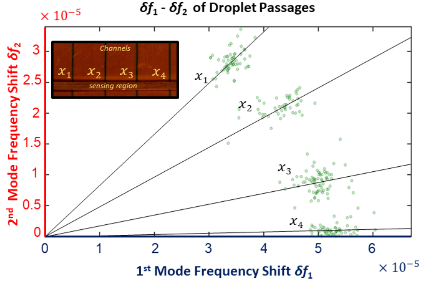
Figure 4.6: Position dependent frequency shifts on \delta f_1 - \delta f_2 plane. Reprinted with permission of Royal Society of Chemistry, Lab on a Chip Journal, Issue 3, 2018.
