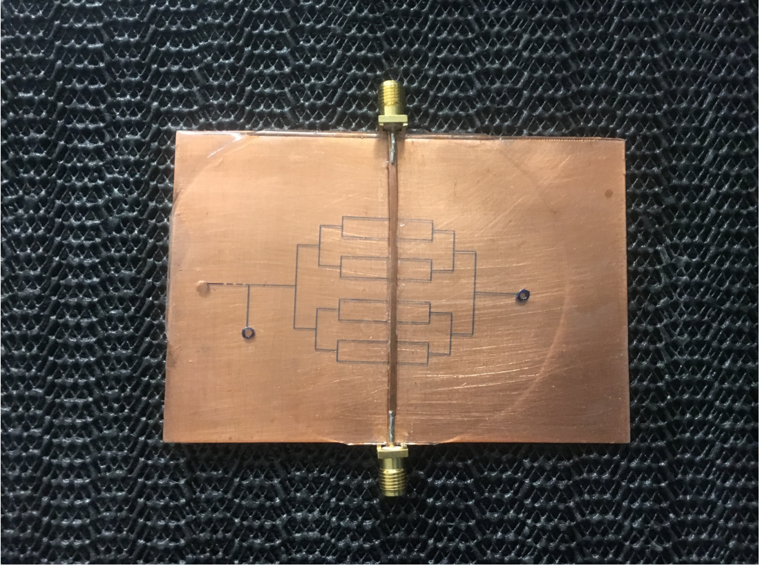
Figure 4.3: Microfluidic channel embedded microwave TL resonator
