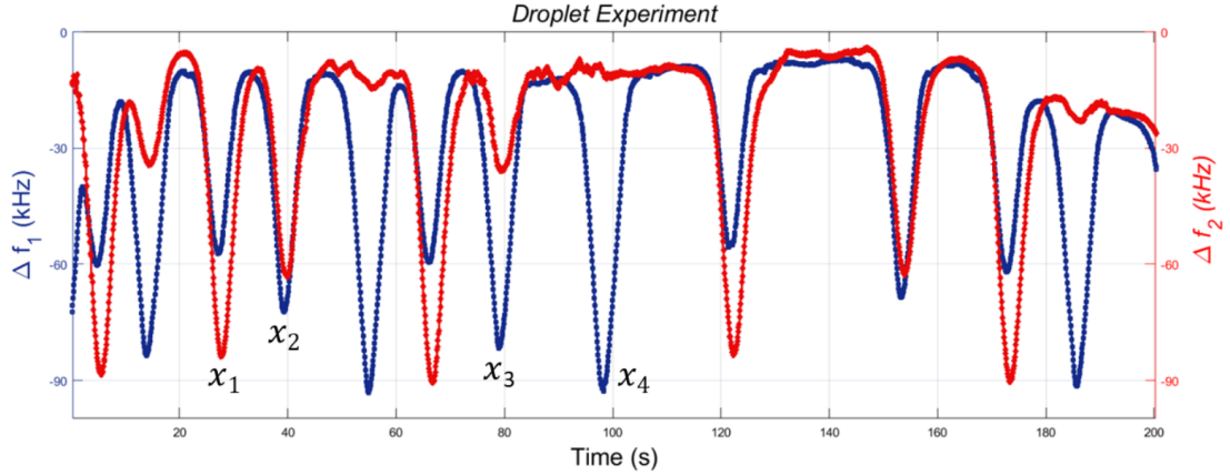
Figure 4.4: Frequency shifts due to the droplet passages
