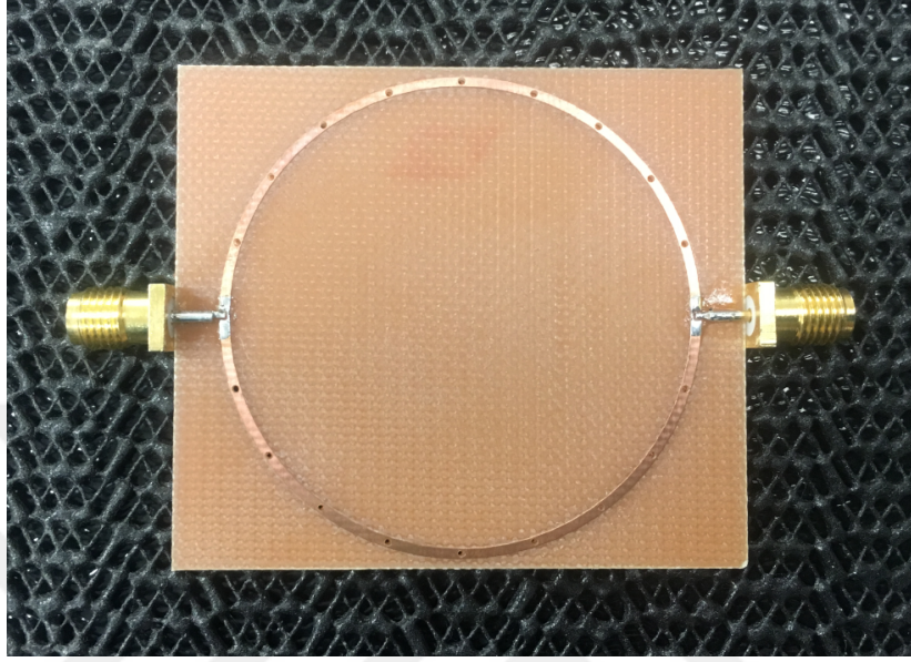
Figure 2.11: The PCB ring resonator with drilled holes used in pipette experiments
