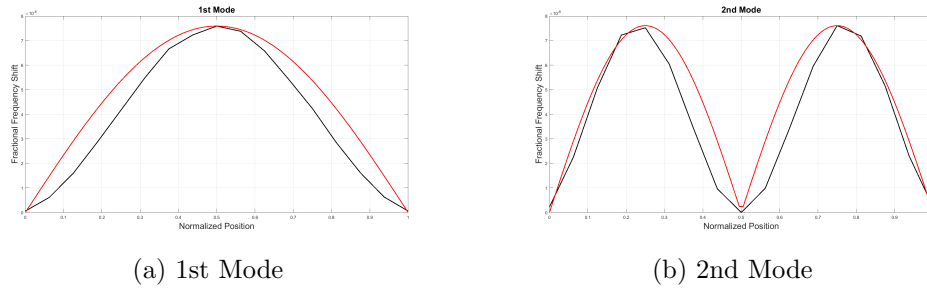
Figure 2.3: Frequency shifts and theoretical shifts with respect to mode shapes for the first two modes
