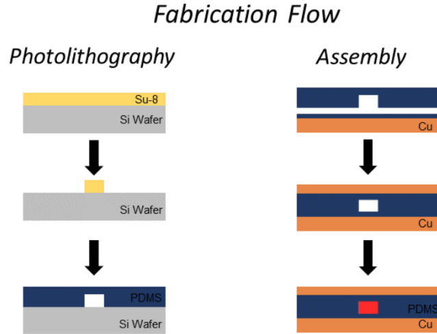
Figure 4.1: Fabrication flow of the microwave resonators containing microfluidic channels
