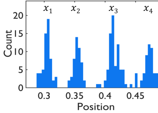
Figure 4.7: Calculated positions of the droplets. Reprinted with permission of Royal Society of Chemistry, Lab on a Chip Journal, Issue 3, 2018.
