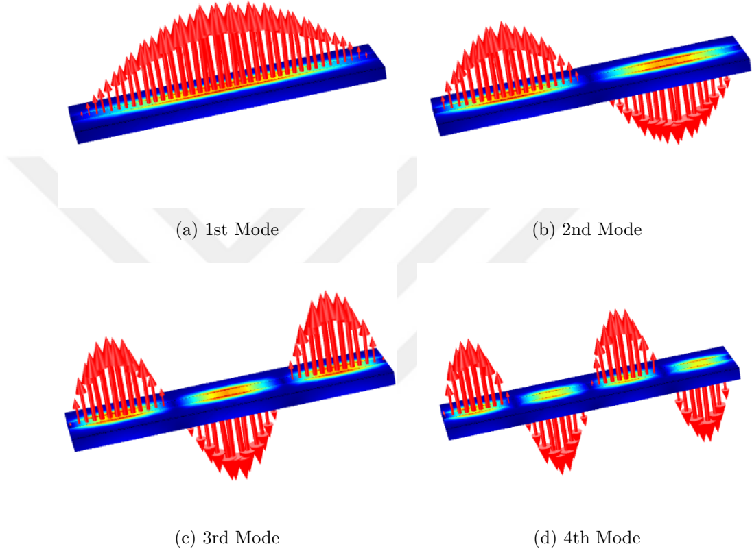
Figure 2.2: First four consequent mode shapes of a microwave TL resonator
