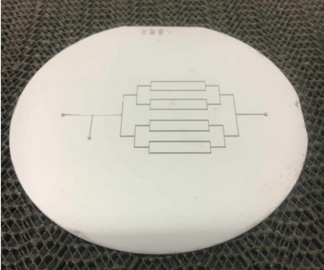
Figure 4.2: The silicon wafer mask after photolithography to transfer the features to PDMS substrate
