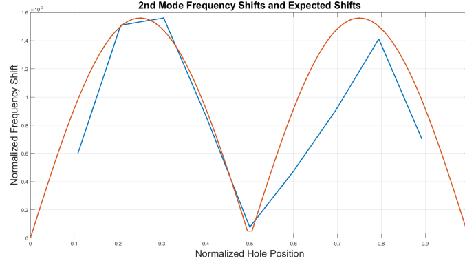
(b) Expected frequency shift profile and experimental frequency shift for the 2nd mode
