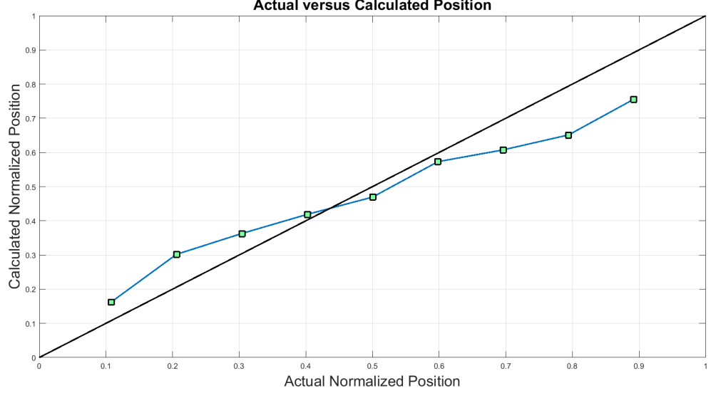
Figure 2.10: Position calculation through experimentally obtained frequency shifts
