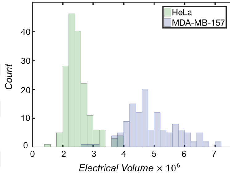
Figure 4.10: Calculated electrical volume of the cell lines HeLa and MDA-MB-157 during the experiments. Reprinted with permission of Royal Society of Chemistry, Lab on a Chip Journal, Issue 3, 2018.
