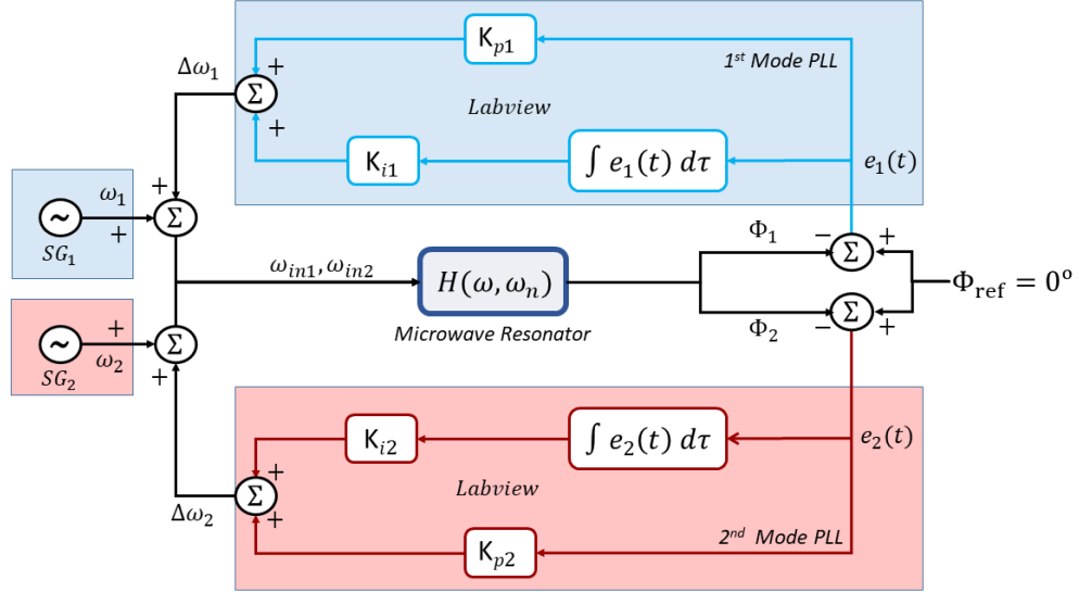
Figure 3.9: Interplay of control scheme embedded in labview with microwave circuitry
