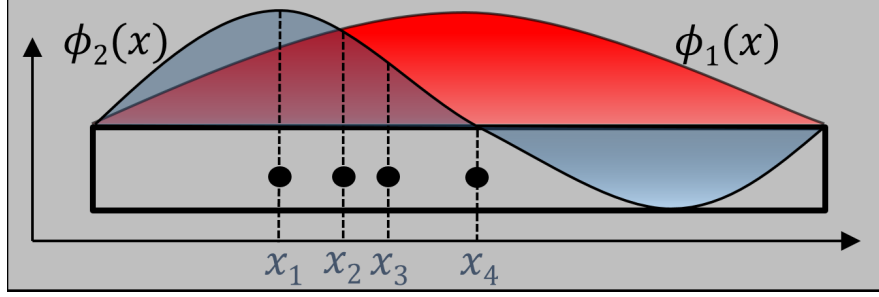
Figure 4.5: Position dependent frequency shifts due to mode shapes
