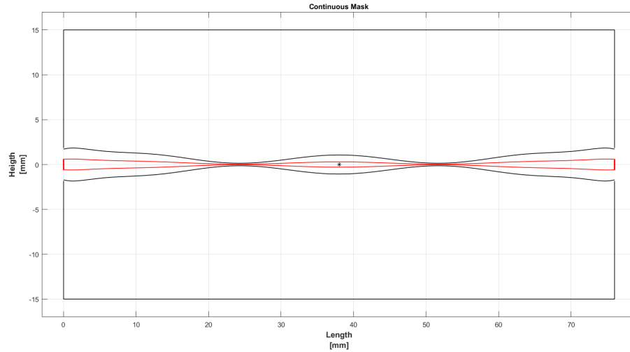
Figure 4.11: Tapered CPW structure for cell sensing applications
