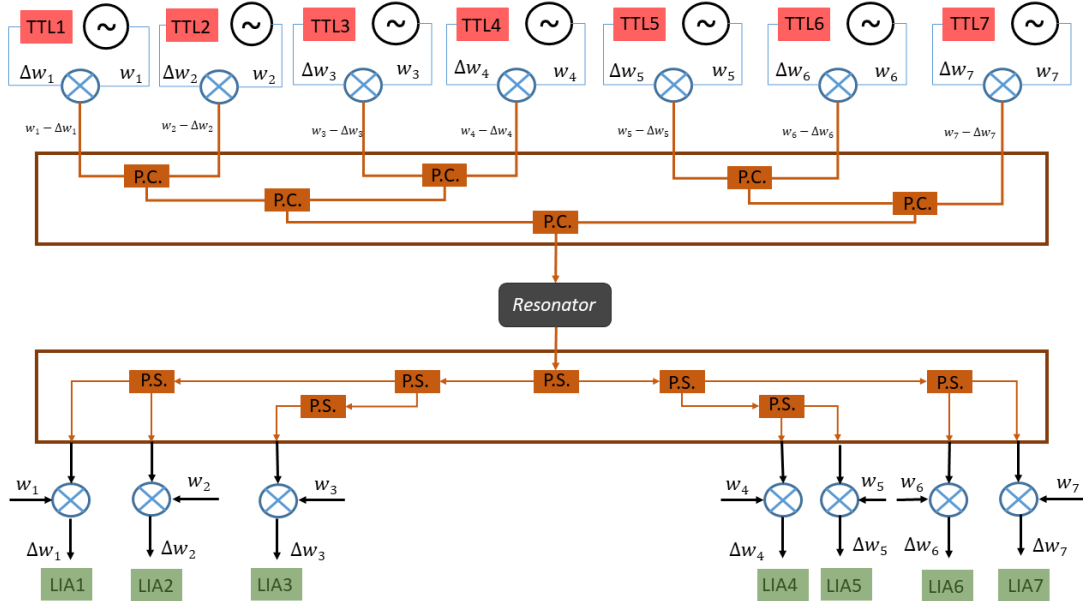
Figure 4.12: Microwave circuit for seven-mode measurement
