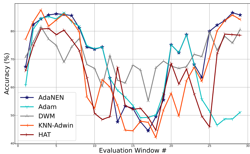
Figure 6.6: 20NG-Gradual.
