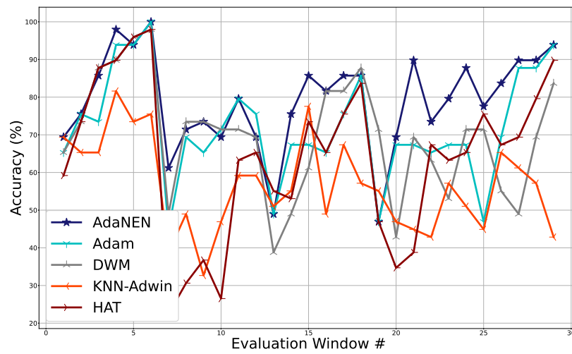
Figure 6.3: Usenet.
