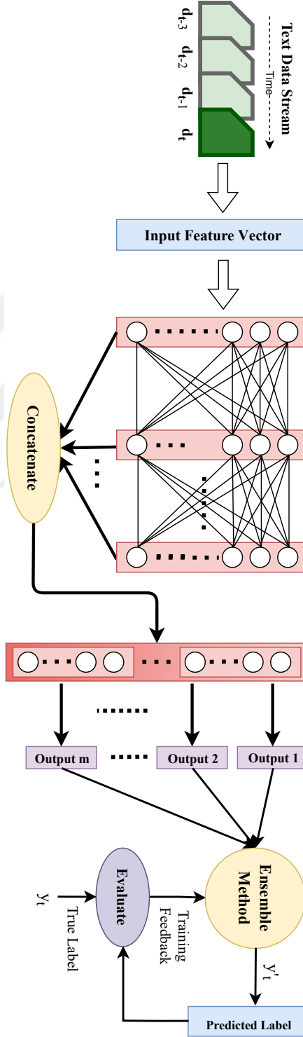
Figure 4.1: Overall schema of our Adaptive Neural Ensemble Network (AdaNEN) for evolving text stream classification.
