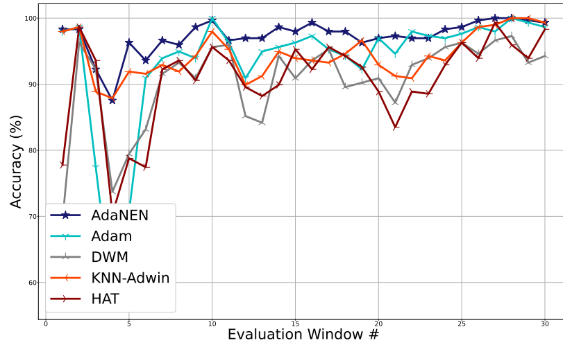
Figure 6.2: Spam.
