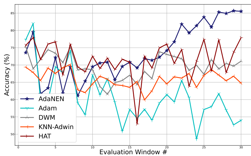
Figure 6.7: AGNews-Abrupt.
