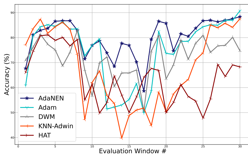
Figure 6.5: 20NG-Abrupt.
