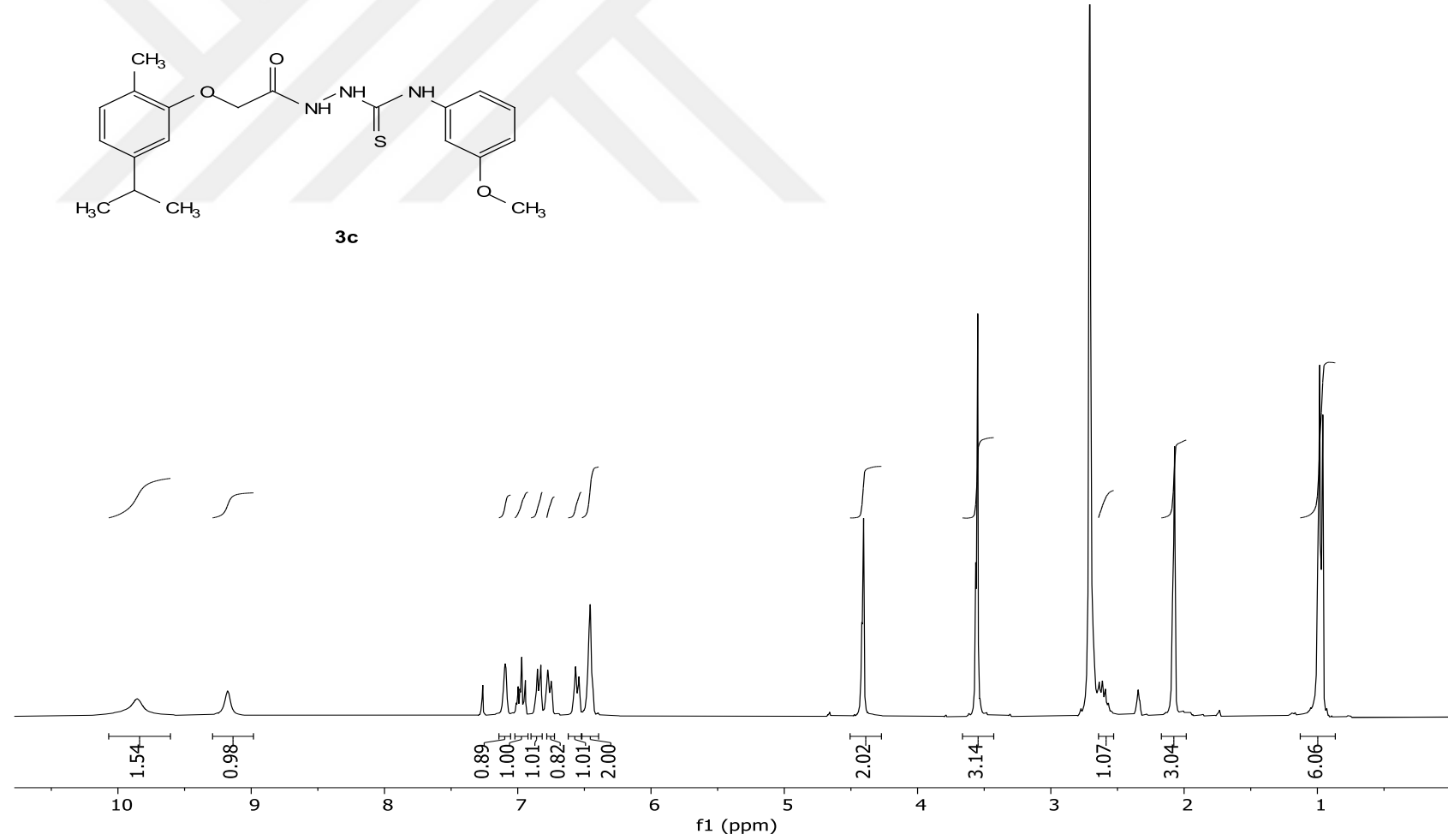
EK-9. (3c) bileşiminin ^1\text{H} NMR spektrumu (300 MHz, \text{CDCl}_3 + \text{DMSO-d}_6 )
